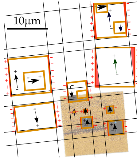
Figure 3.24: Explanation of the ferroelectric orientation. The orientation of \mathbf{P}_e is caused by a charge accumulations at the edges of the pattern due to the missalignment of the squares with respect to the diagonals of the crystal axis (black lines).
