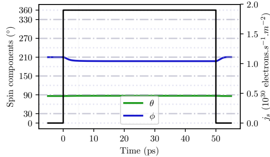
Figure 2.9: STT just above threshold. A STT of 1.9 \times 10^{30} electrons. m^{-2}.s^{-1} (black curve) is above the threshold value to initiate a switch, but a pulse duration of 50ps is still not sufficient to achieve the switch (the blue curve goes back to its initial dashed line, and not to the next one). The higher the STT, the faster the switch.
