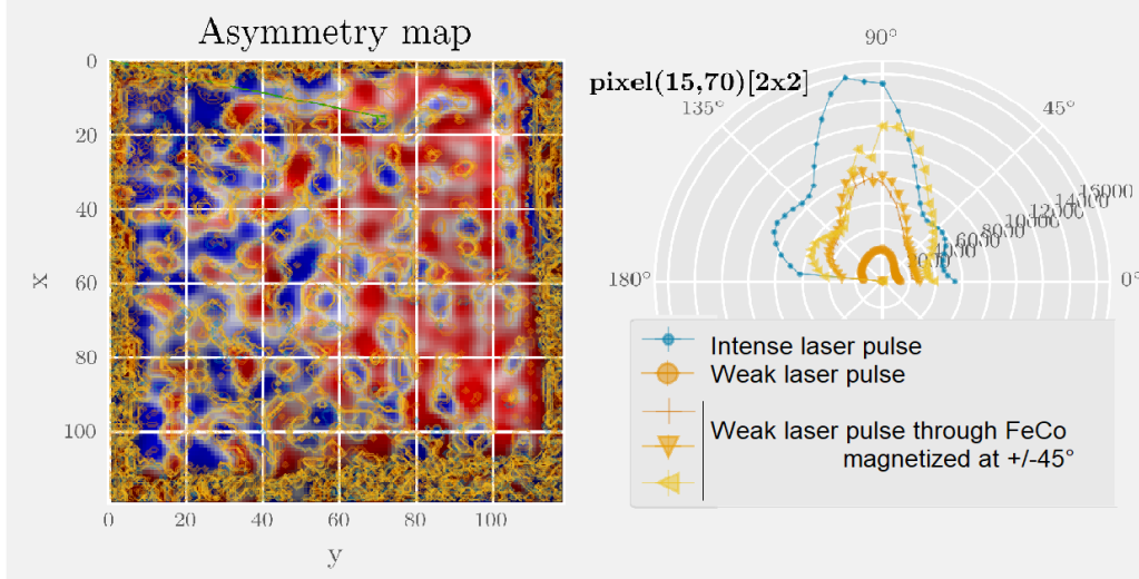
Figure 4.29: Comparison between intense femtosecond laser pulse and THz emission on the SHG signal of BiFeO 3 . The THz emitters modify the second harmonic generation angular dependence in a similar way as an intense laser pulse does.
