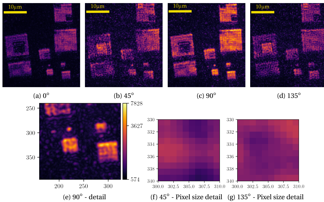
Figure 3.16: Second harmonic intensities for different incident light polarization angles.
