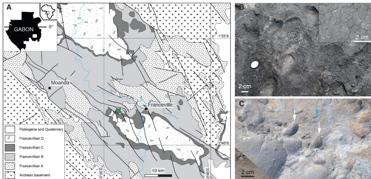
Figure 30: Geological map and field photographs of the FB 2 Member outcrops, Gabon. (A) Geological map of the Francevillien basin adapted from Bouton et al. (2009b). The studied area is the Moulendé Quarry (green star). (B) Elephant-skin texture on the bedding plane of coarse-grained sandstones. Inset box shows reticulate patterns. (C) Micrometer-thick microbial mat laminae (blue arrow) on the bedding plane of sandstones with rounded pits (white arrows).
