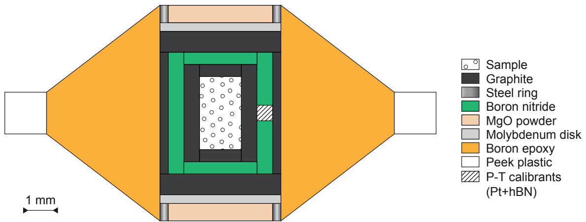
Figure 2.7 – Paris-Edinburgh press experimental assembly.
