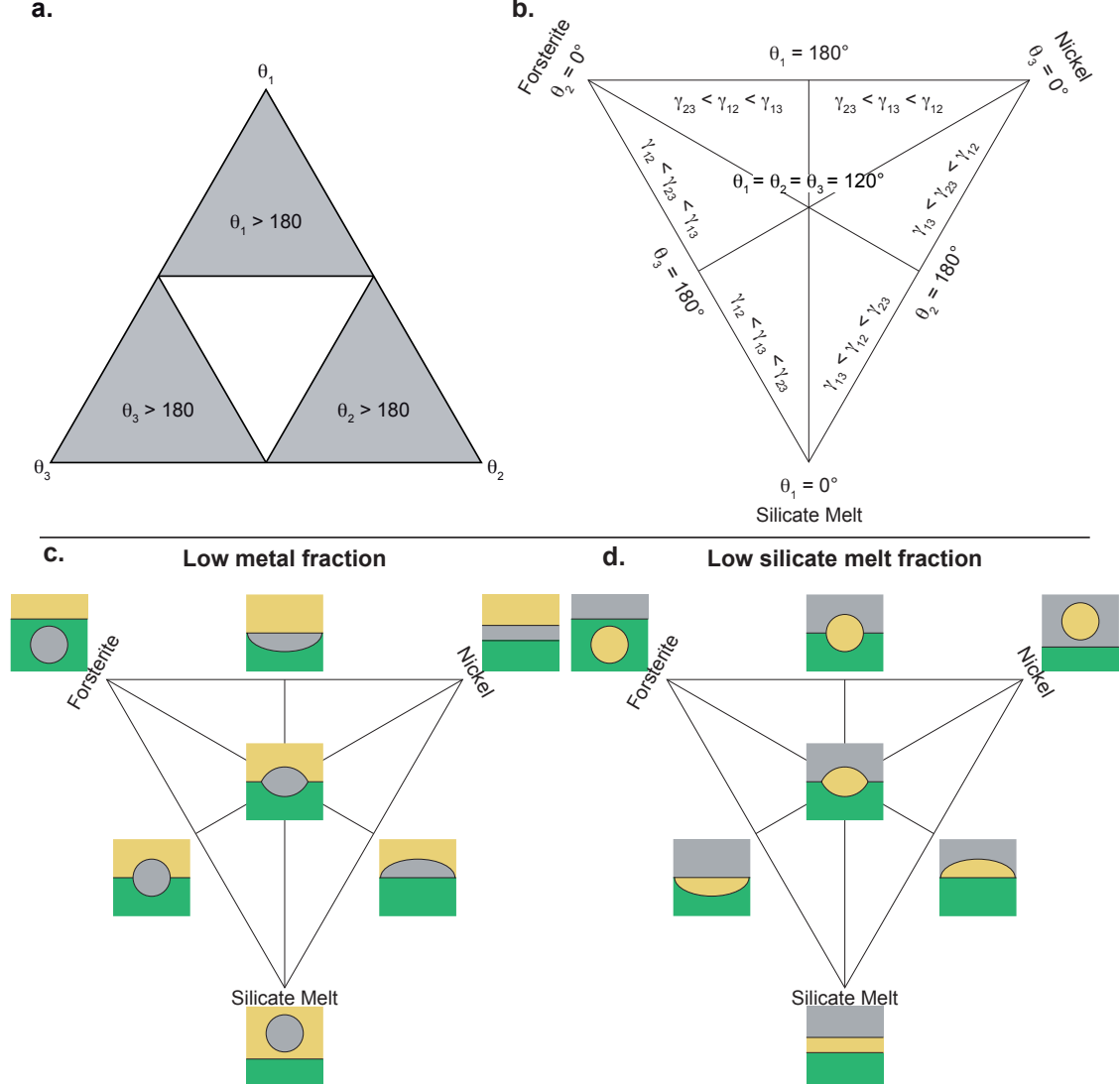
Figure 3.4 – (a.) Ternary diagram showing the inner triangle of possible space given the conditions \theta > 0^\circ and \theta < 180^\circ . (b.) Reduced ternary diagram showing the different energetic regimes delimited by equation 3.3. Full lines separate these regimes and represent equality between two interfacial energies. Sketches explaining the geometry in remarkable points of the ternary diagram are represented in (c.) and (d.). Two end-member cases are considered: (c.) metal is the minor phase, (d.) silicate melt is the minor phase. If one angle is equal to 180^\circ , the phase either forms a sphere or a film. When the dihedral angle is equal to 0^\circ , the phase is highly wetting, its contact is punctual or inexistant, and this phase prevents the two others from being in contact with each other.
