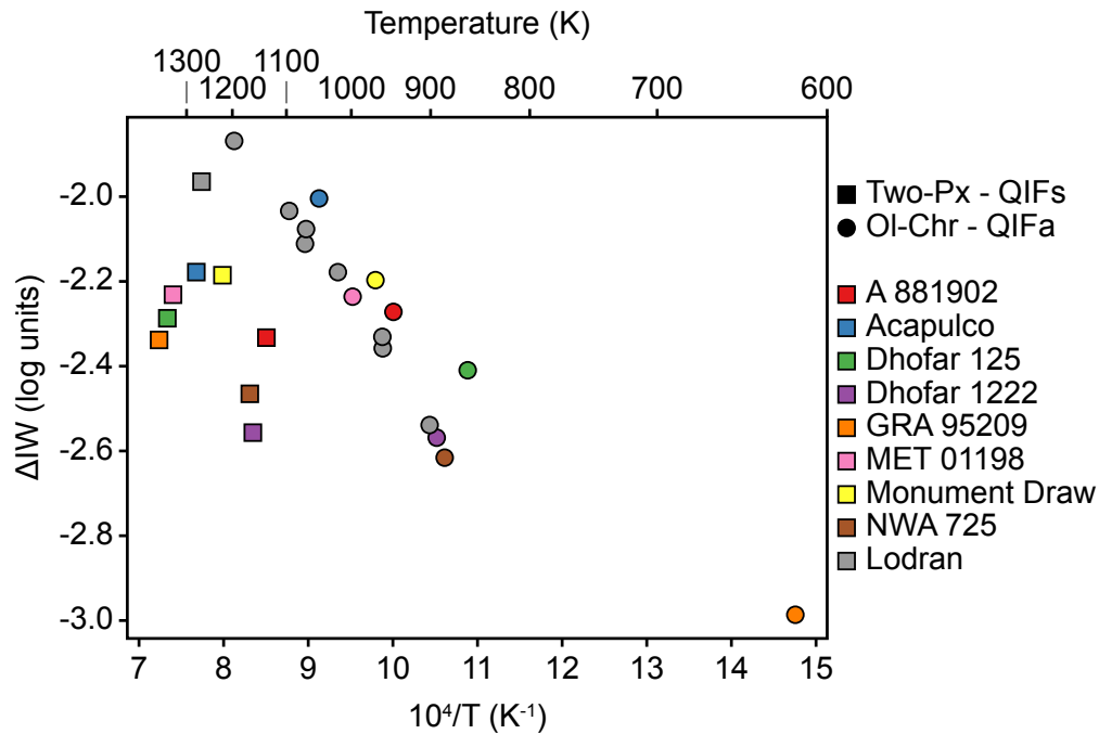
Figure 6.16 – Oxygen fugacity (expressed as deviation from the IW buffer in log units) as a function of the closure temperature calculated. Squares correspond to the pyroxene equilibrium while circles correspond to the olivine equilibrium.
