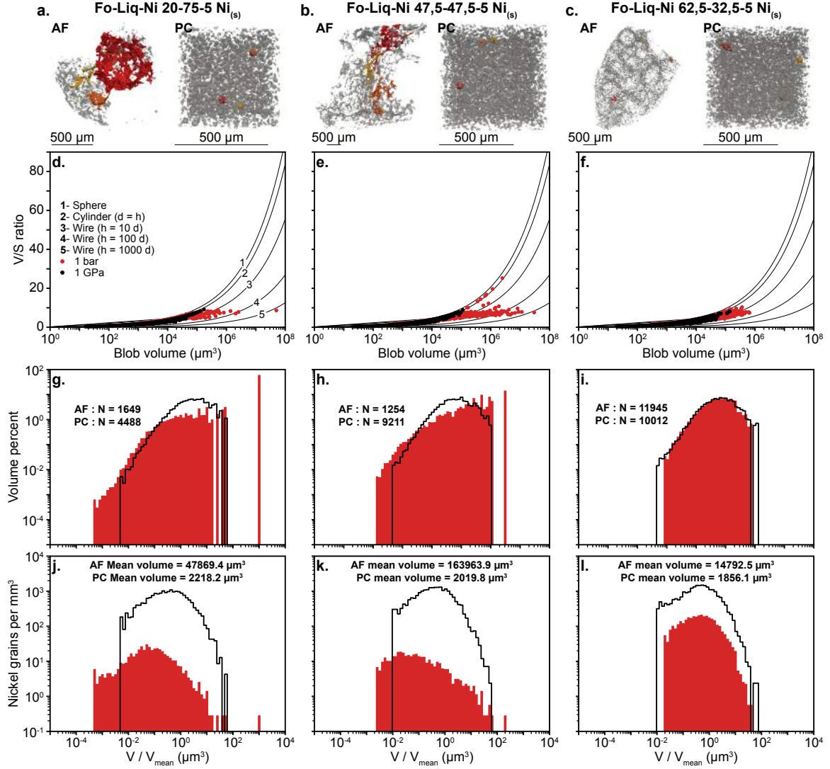
Figure 4.1 – Textures comparison of nickel phase (5 vol% in all samples) between stirred by gas bubbles samples (1-bar furnace, AF) and immobile samples (piston cylinder, PC) for different proportions of silicate melt in the system and after 24 hours (AF) and 5 hours (PC) of experiments at 10-15 K below the melting point of nickel. (a-c) show images of the 3D X-ray microtomograms. In gray is represented all the nickel of the sample. The three biggest blobs of nickel are represented in red, orange and yellow in each sample. (d-f) represent the volume to surface ratio ( V/S ) as a function of blob volume, with data points for AF experiments in red and data points for PC experiments in black. Normalized distributions ( V/V_{\text{mean}} ), in volume or in number are represented in (g-i) and (j-l), respectively. Here also, AF data are plotted in red and PC data in black.
