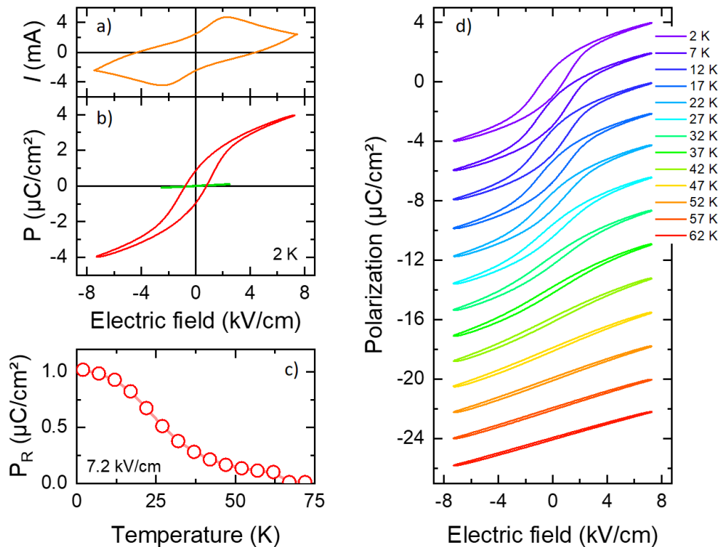
FIG. 4.16: Ferroelectric properties. a) Current vs voltage curves measured on a \text{STOAl}(1.8 \text{ nm}) sample. b) Corresponding polarization loop (red curve). The green curve corresponds to the polarization loop measured with a maximum field of 2.5 \text{ kV/cm} . c) Temperature dependence of the remanent polarization. d) Polarization loops at different temperatures. The curves are shifted by 2 \mu\text{C/cm}^2 for clarity.
