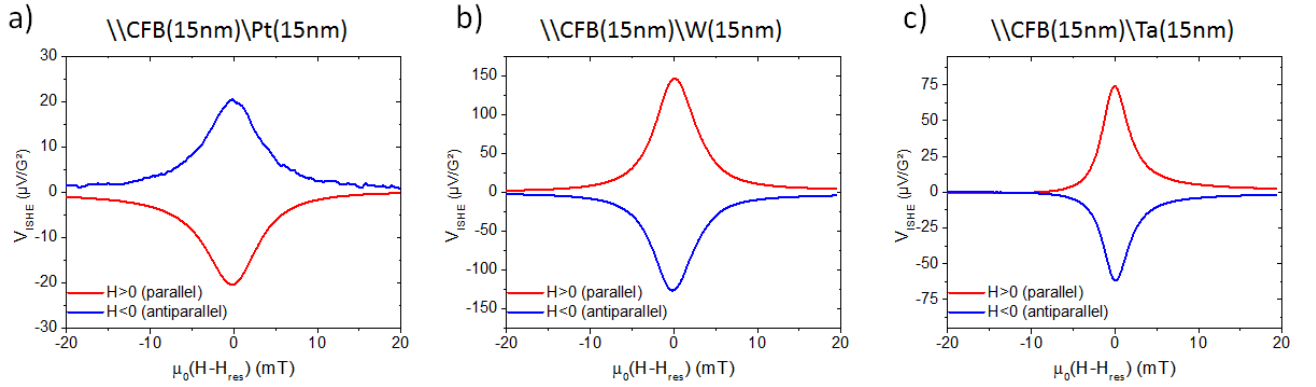
FIG. 3.1: Spin pumping ISHE signals measured in different bilayers in the parallel and antiparallel configurations using CoFeB as the ferromagnetic layer: a) CoFeB(15)\Pt(15) b) CoFeB(15)\W(15) and c) CoFeB(15)\Ta(15). Thicknesses are in nanometers.
