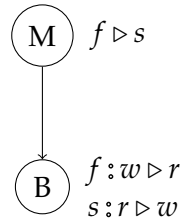
FIGURE 2.1: Lucy's CP-net.
