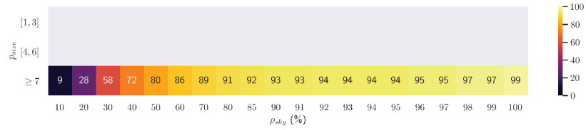
(b) U, Brown, W_5 , tpr
