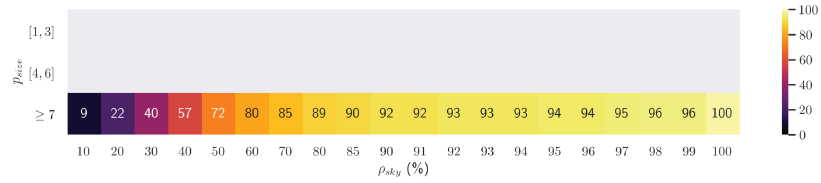
(a) U, Brown, W_3 , tpr
