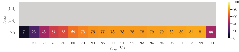
(c) U, Brown, W_7 , score
