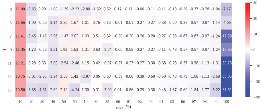
(b) U, Brown, intercept
