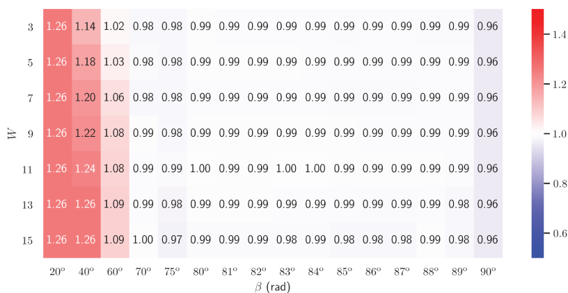
(a) H, Brown, slope
