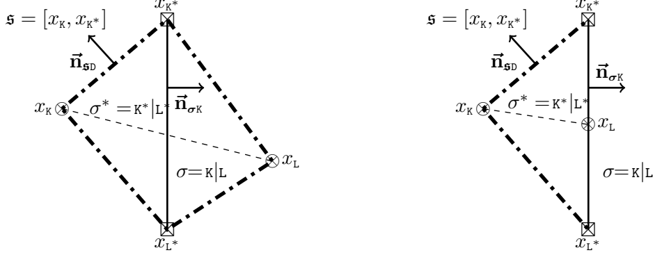
Fig. III.2 Left : A diamond \mathfrak{D} = \mathfrak{D}_{\sigma, \sigma^*} with \sigma \subset \mathcal{E}_{int} . Right : A diamond \mathfrak{D} = \mathfrak{D}_{\sigma, \sigma^*} with \sigma \in \partial\Omega .
