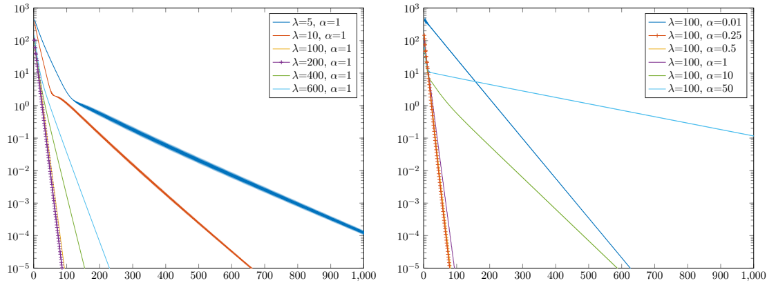
Fig. IV.9 Test 1, Mesh 1 1 , first Schwarz algorithm. Left : optimization of \lambda , with \alpha = 1 . Right : optimization of \alpha , with \lambda = 100 .
