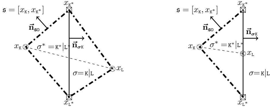
Fig. IV.1 Left : A diamond \mathfrak{D} = \mathfrak{D}_{\sigma, \sigma^*} with \sigma \subset \mathcal{E}_{int} . Right : A diamond \mathfrak{D} = \mathfrak{D}_{\sigma, \sigma^*} with \sigma \in \partial\Omega .
