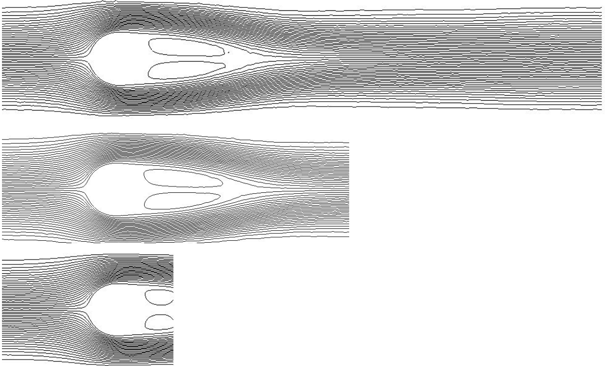
Fig. 3 Streamline of Test case 2 at T = 3.5 , Re = 250 . On the top: \Omega = [0, 5] \times [0, 1] , NbCell=12118 . In the middle: \Omega' = [0, 3] \times [0, 1] , NbCell=8636 . On the bottom: \Omega'' = [0, 1.5] \times [0, 1] , NbCell=6534 .
