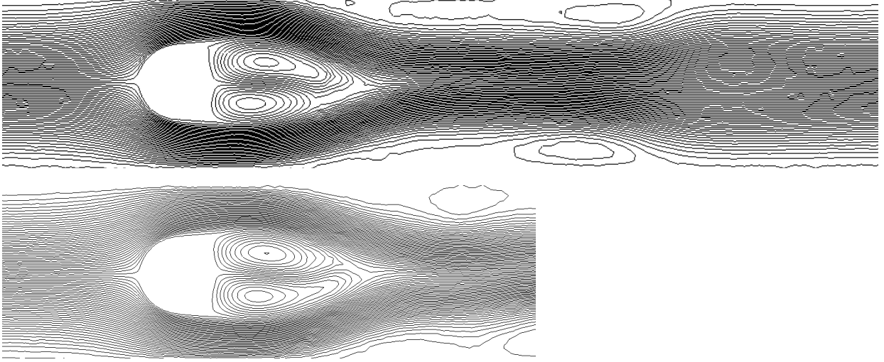
Fig. III.9 Streamline of Test case 2 at T = 3.5 , Re = 1000 , \delta t = 0.035 . On the top: \Omega = [0, 5] \times [0, 1] , NbCell= 12118. On the bottom: \Omega' = [0, 3] \times [0, 1] , NbCell=8636.
