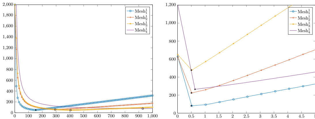
Fig. IV.12 Test 1, (\text{Mesh}_m^1)_m , m = 1, 2, 3, 4 . Left: optimization of \lambda to obtain an error of order 10^{-5} , with \alpha = 1, \beta = 10^{-1} . Right: optimization of \alpha to obtain an error of order 10^{-5} , with \lambda = 100, \beta = 10^{-1} .
