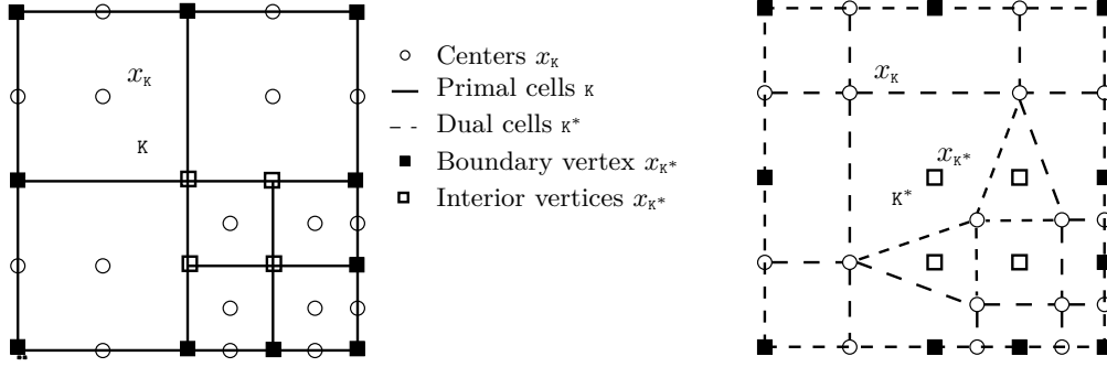
Fig. I.2 DDFV mesh \mathfrak{T} .
