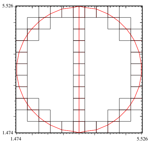
Fig. 4 Example of reconstruction of an interface between three materials, with two triple points configurations.
