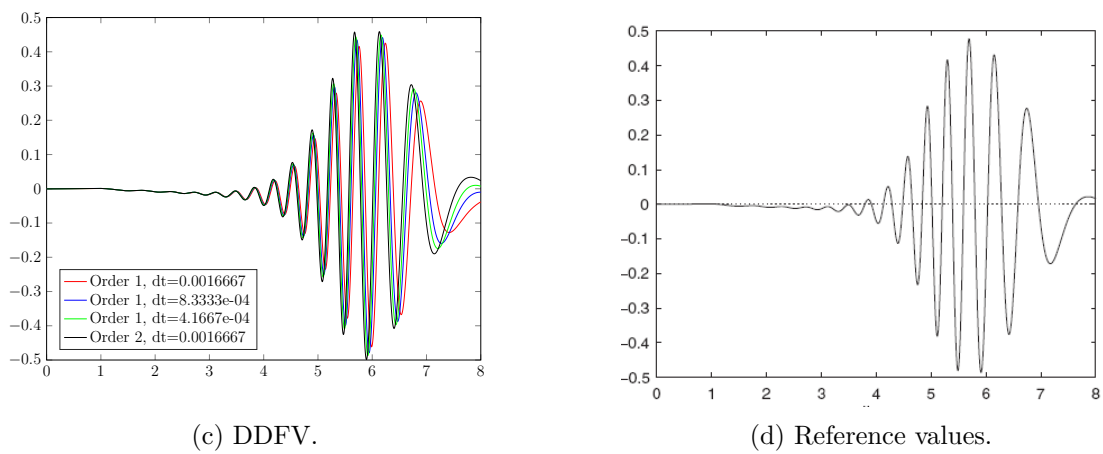
Evolution of the lift coefficient c_l^n
