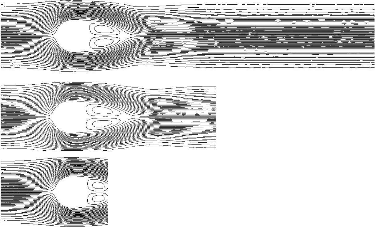
Fig. III.6 Streamline of Test case 2 at T = 1.5 , Re = 250 , \delta t = 0.035 . On the top: \Omega = [0, 5] \times [0, 1] , NbCell= 12118. In the middle: \Omega' = [0, 3] \times [0, 1] , NbCell=8636. On the bottom: \Omega'' = [0, 1.5] \times [0, 1] , NbCell=6534.
