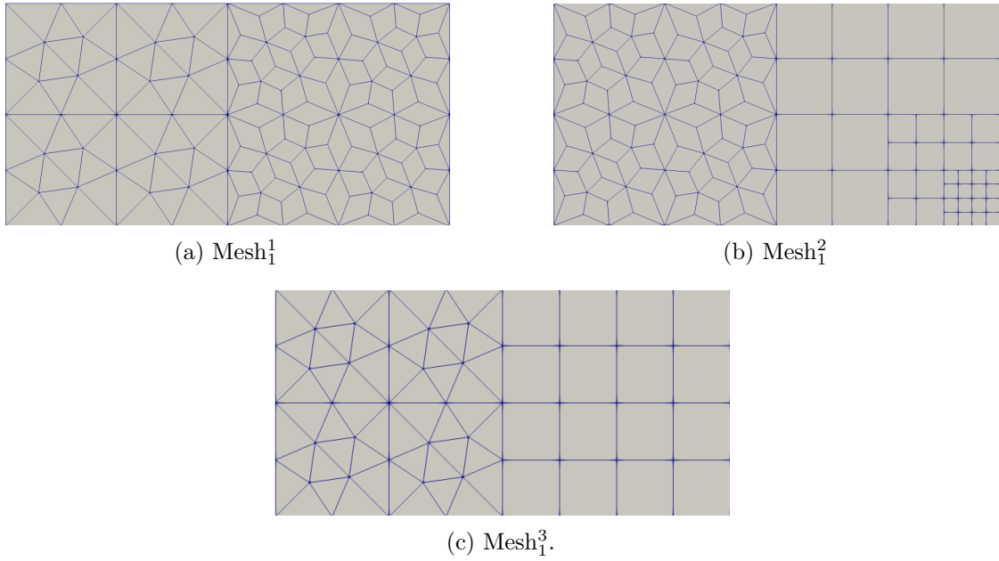
Fig. IV.5 Coarse level of refinement of the composite meshes on \Omega , \text{Mesh}_1^k .
