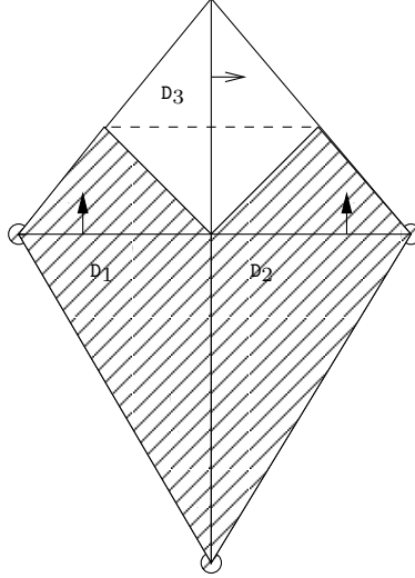
Fig. I.7 Degenerate case
