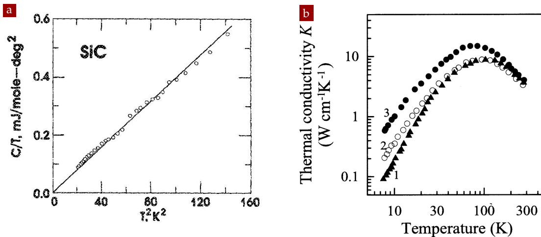
FIGURE 3.2 – (a) Specific heat of SiC between 4 and 12 K. Data from [123]. (b) Thermal conductivity of SiC as a function of the temperature, data from [219]; at low temperature different polytypes behave differently (1 \rightarrow 4H-SiC, 2 \rightarrow 3C-SiC, 3 \rightarrow 6H-SiC)
