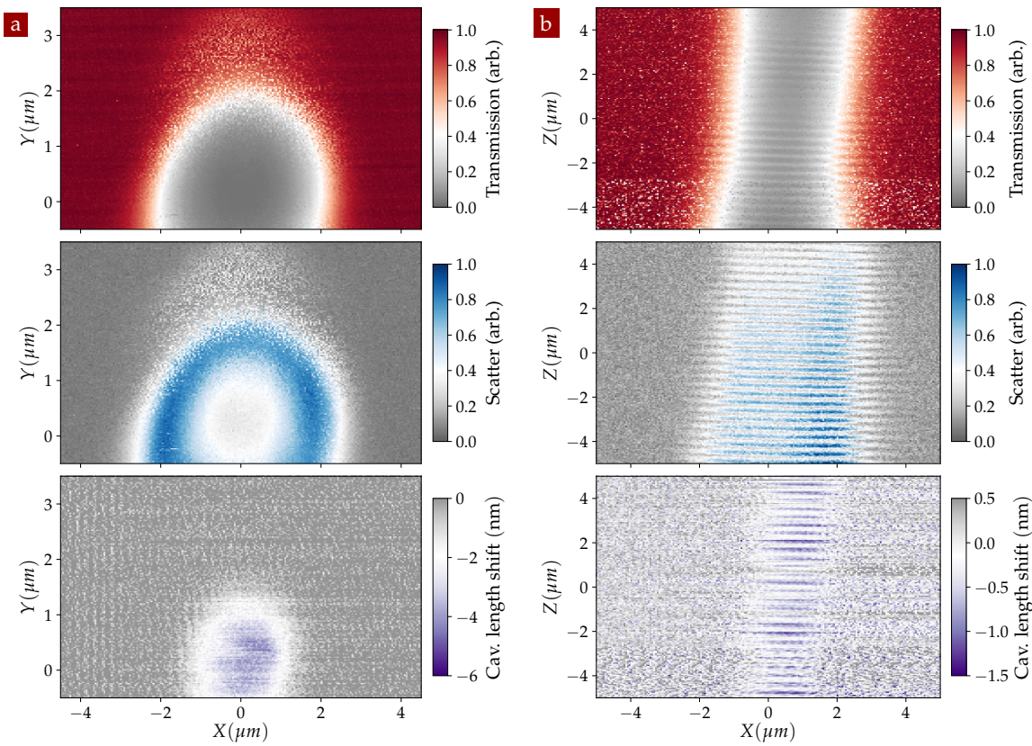
FIGURE 5.10 – (a) Cross-section imaging of the TM_{00} mode in the transversal XY plane. (b) Imaging of the TM_{00} mode in the XZ plane, spanning over a long distance in the Z direction: the variation of the waist dimension as well as the isophase profile can be imaged in this configuration.
