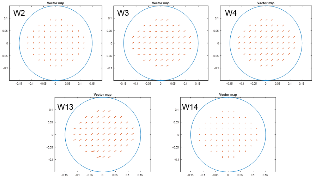
Figure 30: Misalignment wafer map for five wafers (Pitch= 3.42\mu\text{m} )
