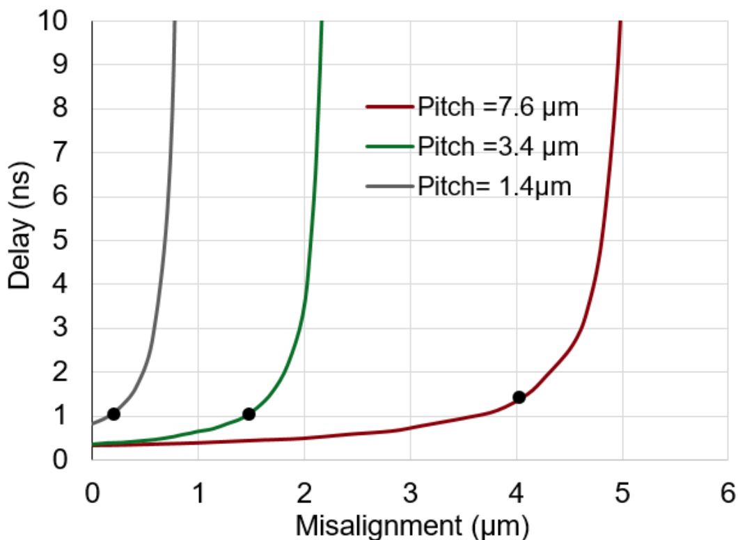
Figure 62: Delay variation of a daisy chain (10,000 Cu-Cu pads) (pitch: 7.6, 3.45 and 1.4 \mu\text{m} ) as a function of the misalignment
