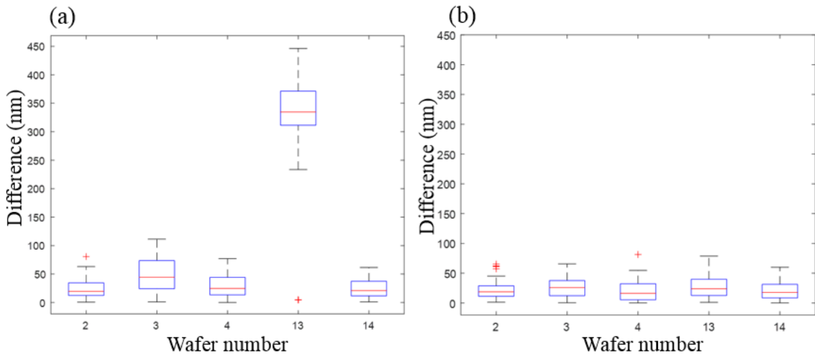
Figure 35: Comparison of test structure results ( 3.42\mu\text{m} pitch) and overlay measurements in X and Y direction
