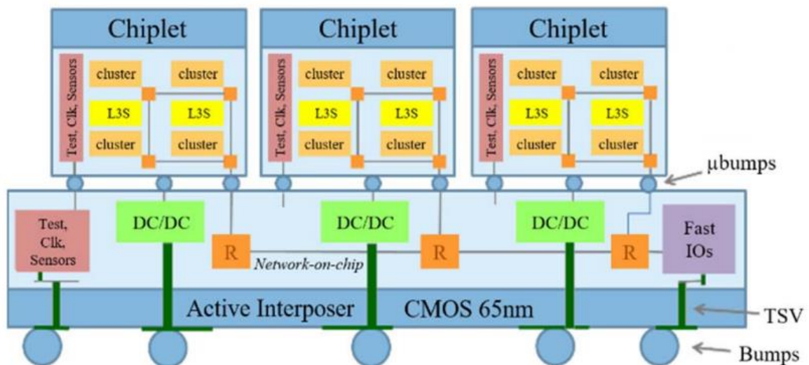
Figure 12: Intact system architecture overview (source [38])
