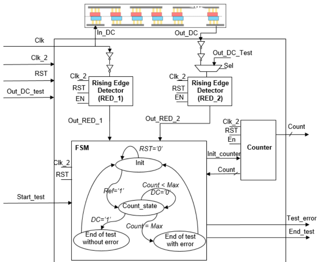
Figure 60: BIST delay architecture
