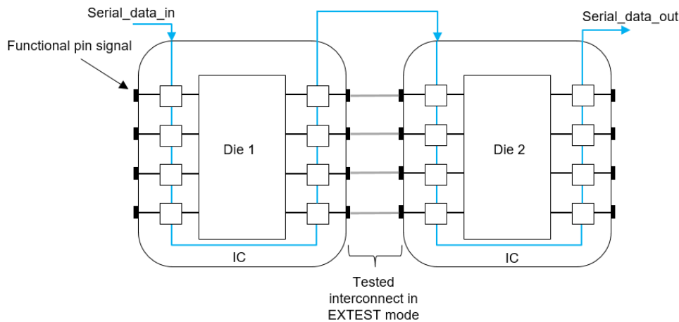
Figure 40: IEEE 1149.1 boundary scan test
