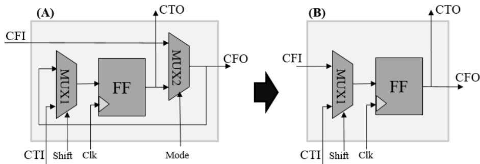
Figure 52: Dedicated (a) and (b) shared wrapper cell
