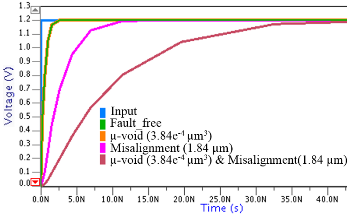
Figure 64: Simulation of the electrical equivalent model of daisy chain (10,000 Cu-Cu pads; pitch= 3.45 \mu\text{m} )
