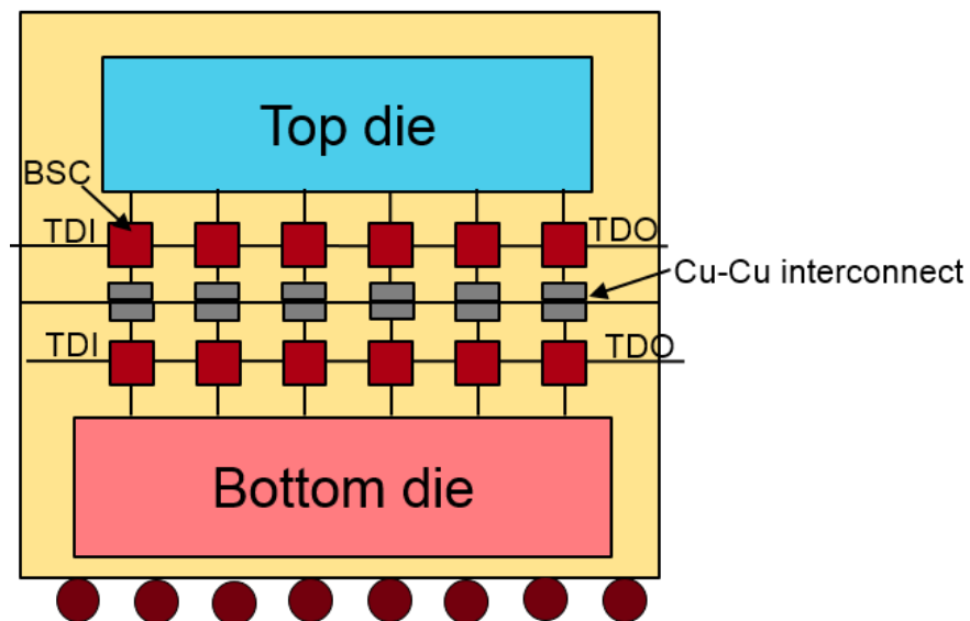
Figure 15: Test of 3D-IC interconnects at system level
