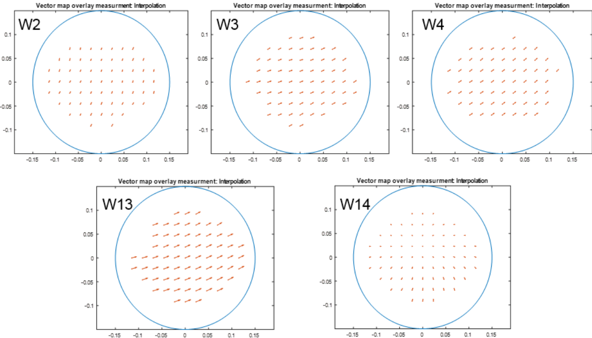
Figure 34: Wafer map results using overlay measurements
