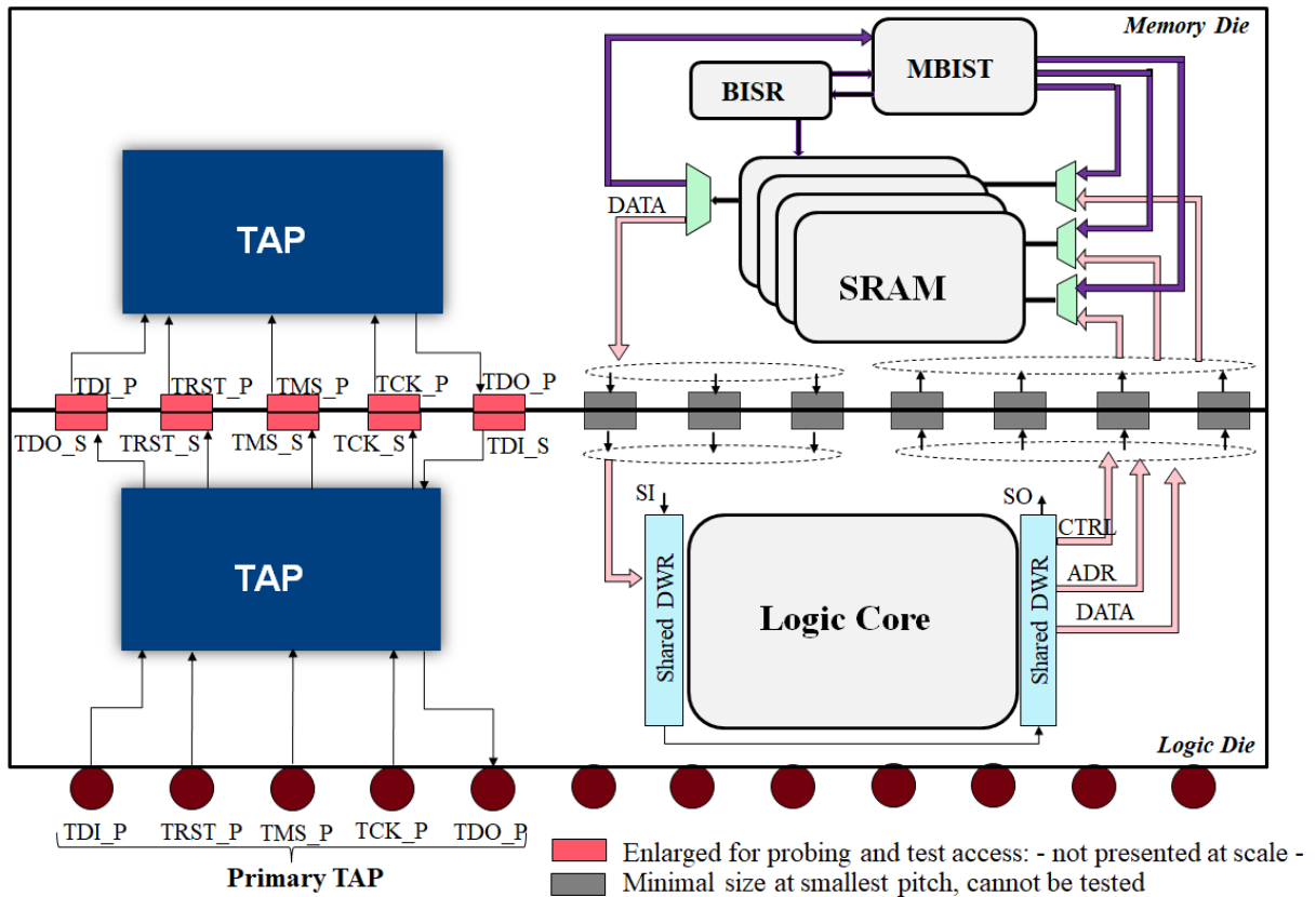
Figure 53: Optimized DFT architecture for SRAM/Logic 3D-IC
