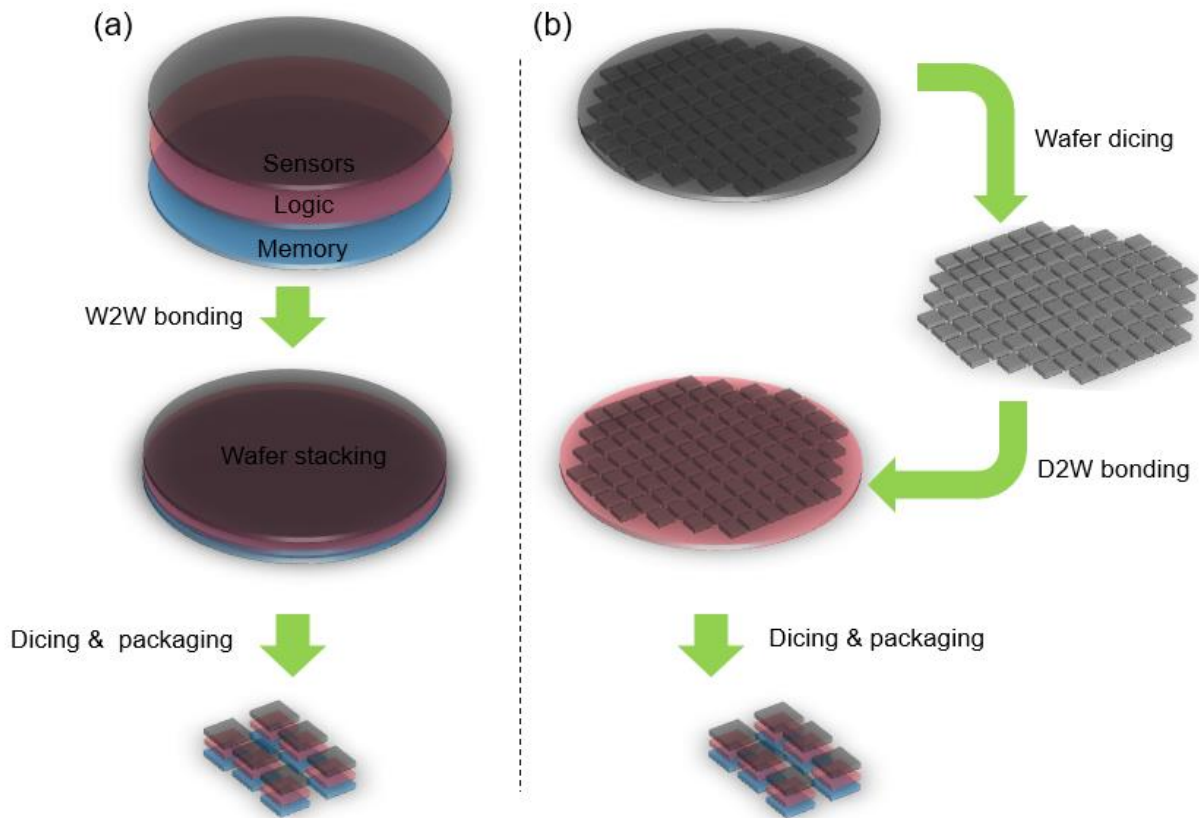
Figure 3: 3D stacking options: (a) W2W, (b) D2W
