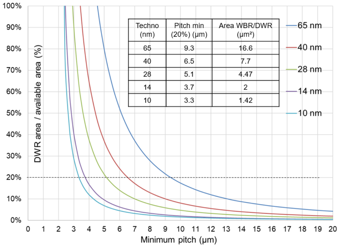
Figure 51: Variation of the ratio between the area of WBR/DWR and the available area as a function of pitch (Face-to-Back)
