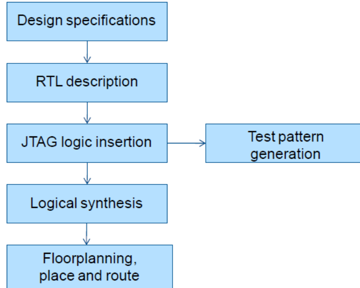
Figure 65: Design flow of the test chip circuit
