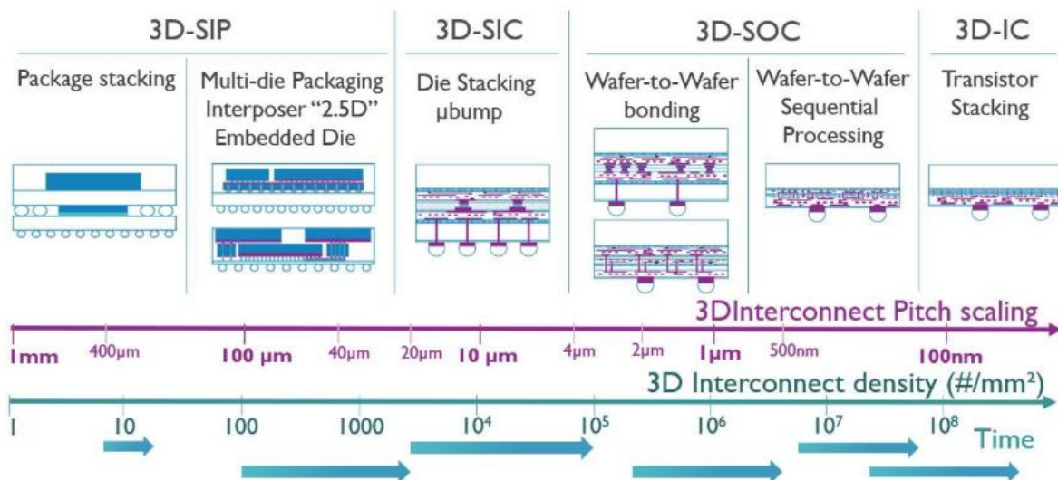
Figure 2: Evolution of 3D integration (source [8])
