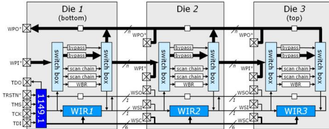
Figure 45: 3D DFT architecture based on IEEE 1500 (source [62])
