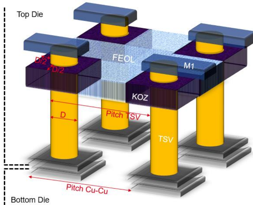
Figure 50: 3D view of 3D-IC interconnects (Face-to-Back stacking mode)
