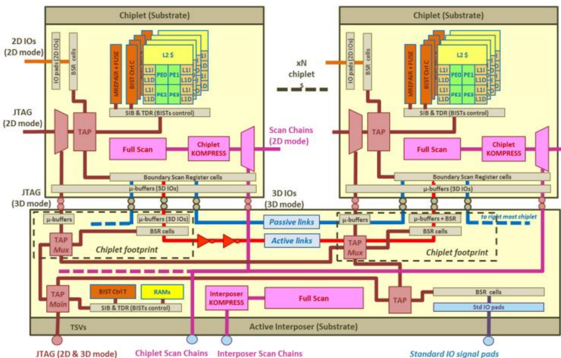
Figure 47: 3D DFT architecture based on IEEE P1687 (source [64])
