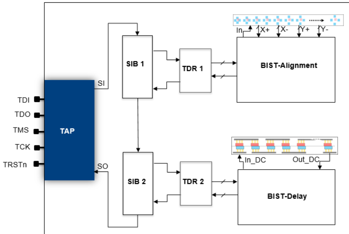
Figure 61: BIST's architecture integration within IJTAG infrastructure
