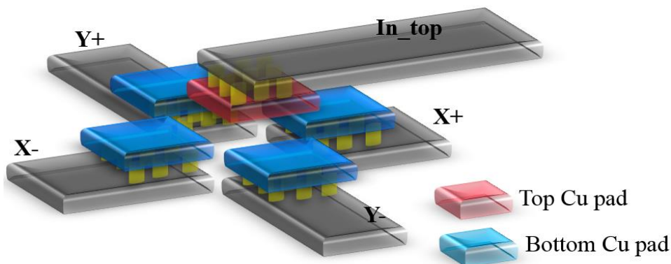
Figure 25: The reference pattern of misalignment test structure
