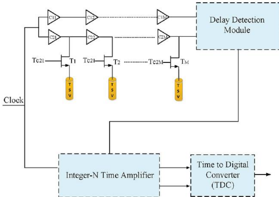
Figure 55: Example of delay measurement method (source [71])
