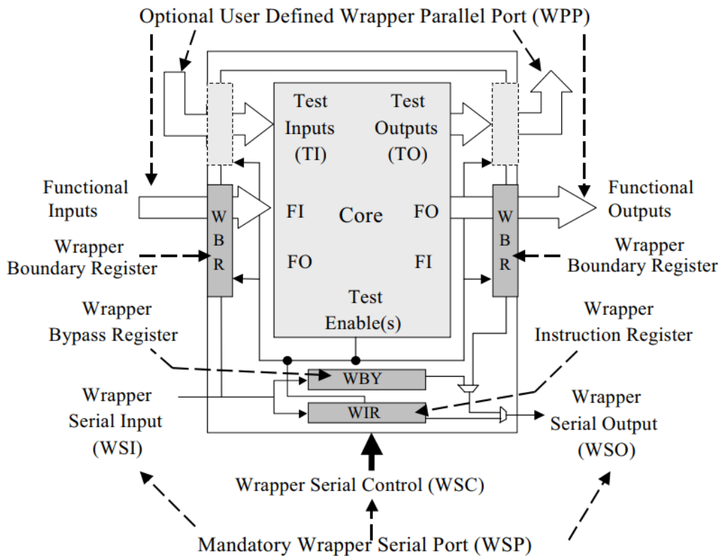
Figure 43: IEEE Std 1500 wrapper components (source [58])
