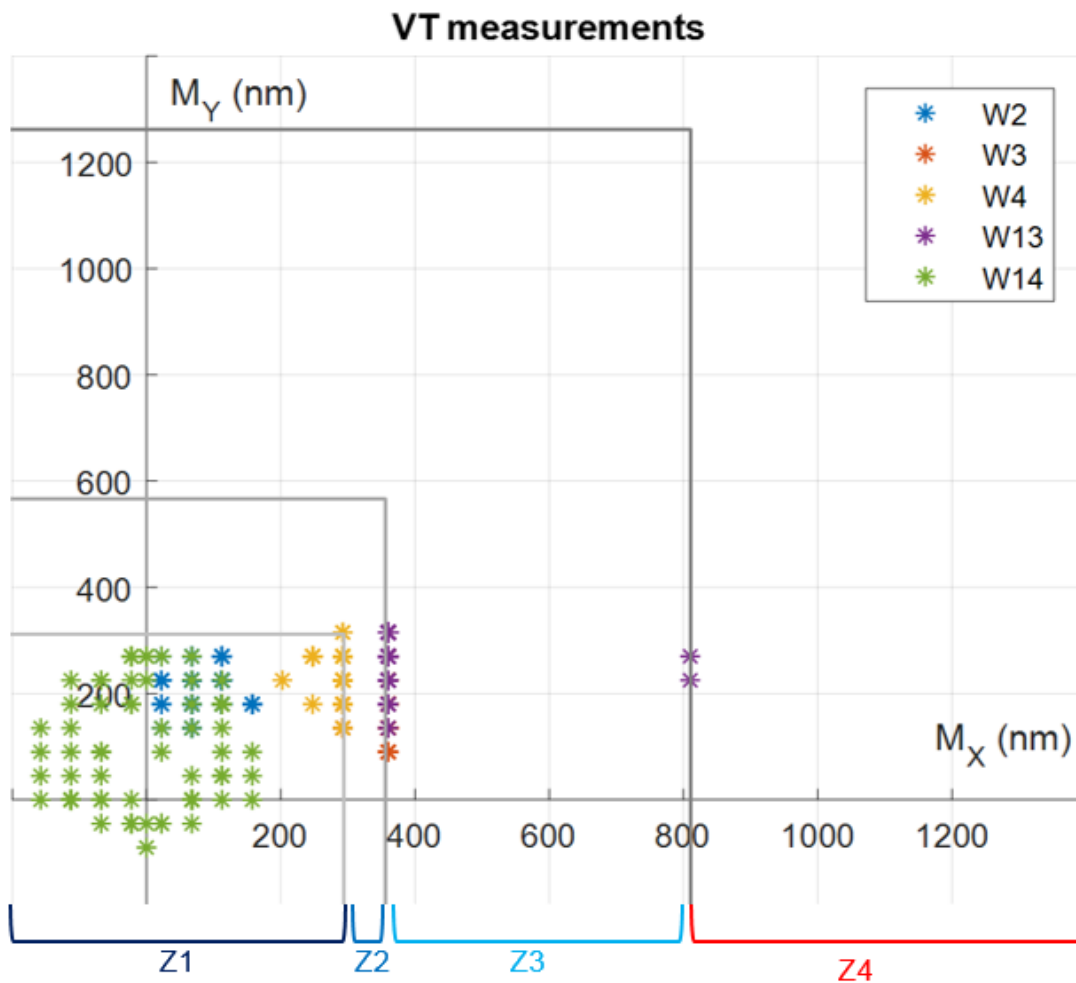
Figure 29: Misalignment test structure results (Pitch= 3.42\mu\text{m} )
