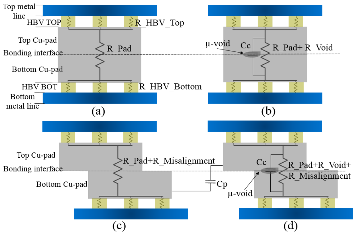
Figure 17: Impact of Cu-Cu interconnect defect on electrical characteristics
