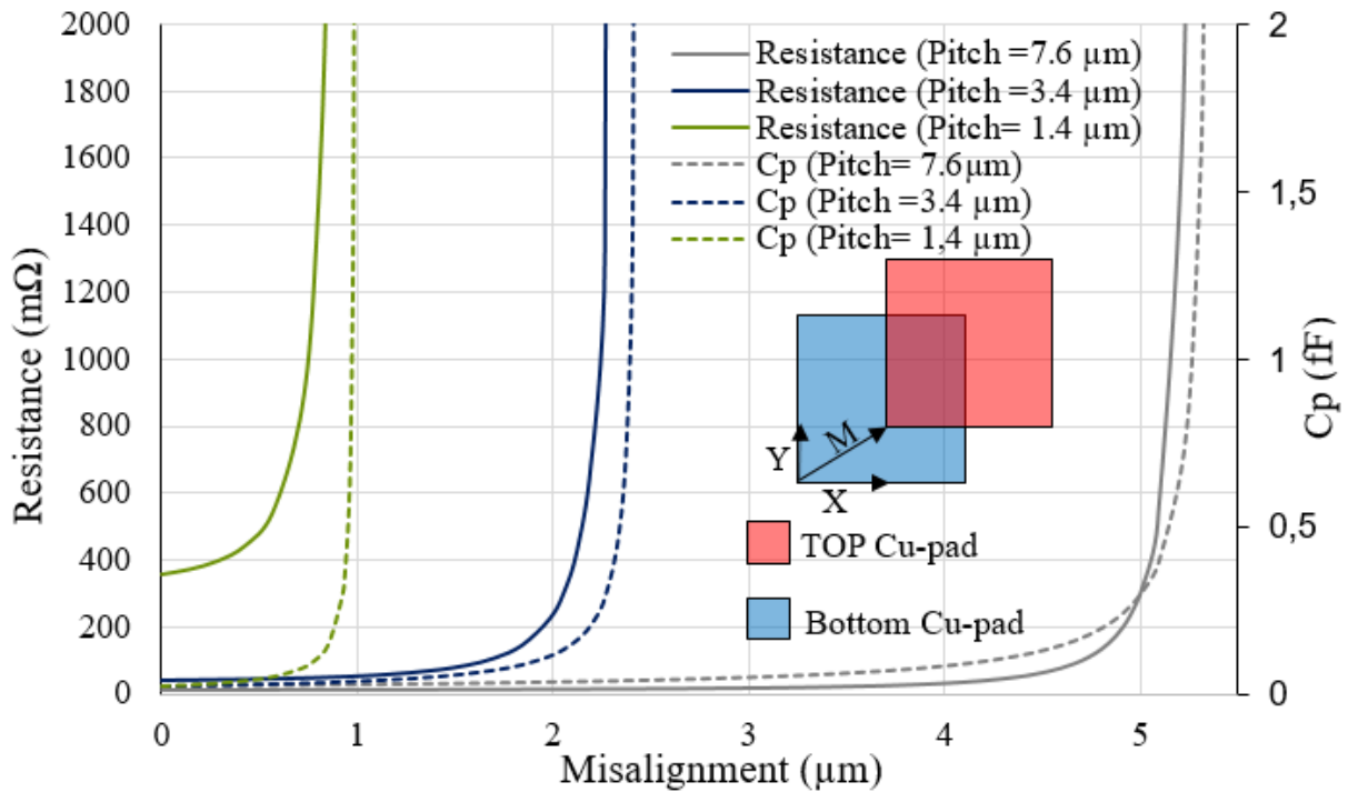
Figure 19: Variation of the resistance and parasitic capacitance of a Cu-Cu pad (pitch: 7.6, 3.45 and 1.4 \mu\text{m} ) as a function of misalignment.
