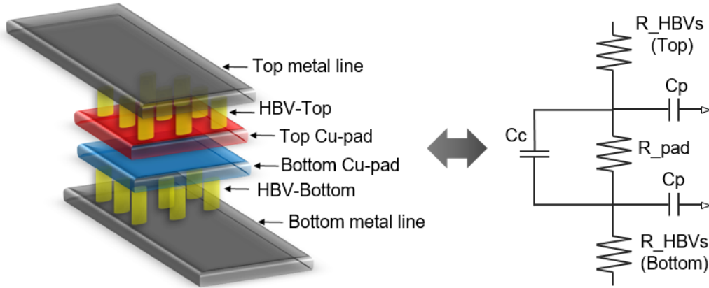
Figure 16: Equivalent electrical model of Cu-Cu interconnects
