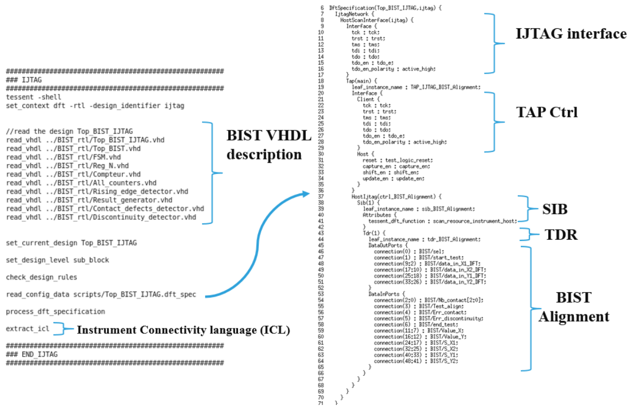
Figure B.5: DFT specification and ICL extraction
