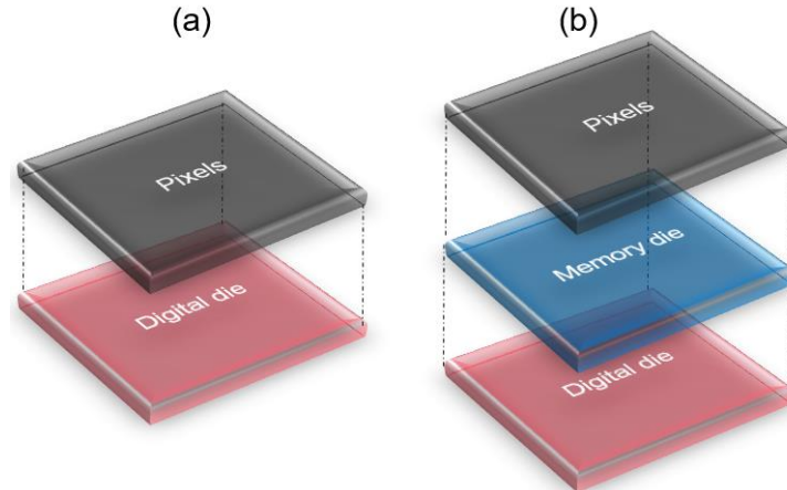
Figure 8: Structure of stacked CMOS image sensor: (a) two layers, (b) three layers
