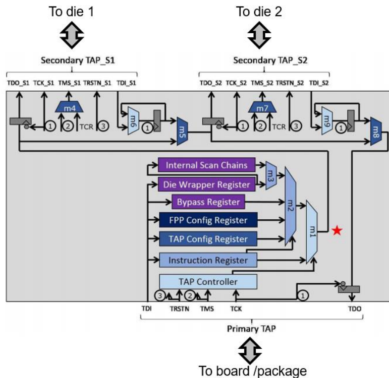
Figure 48: Serial control mechanism (SCM) (source: [68])
