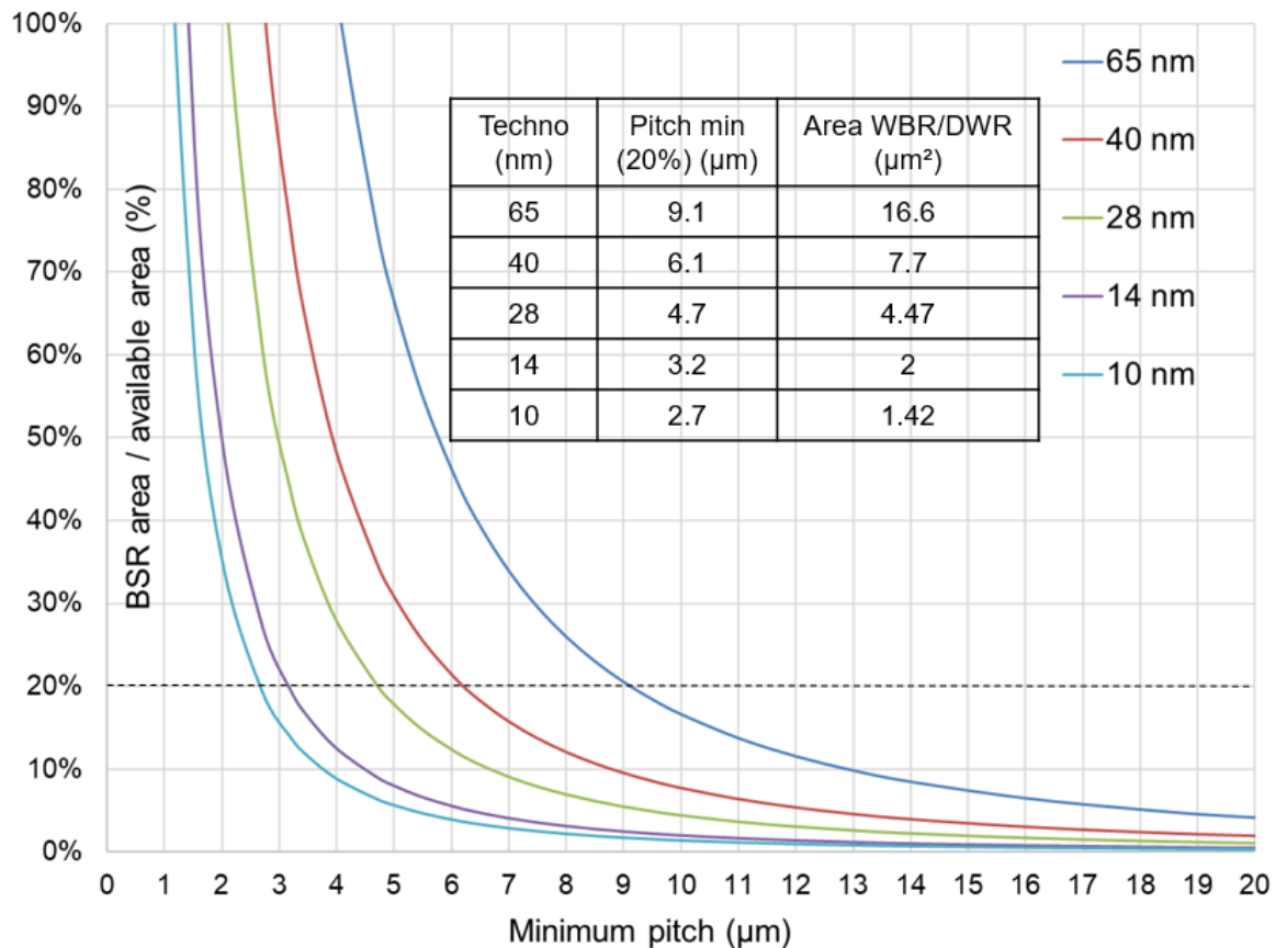
Figure 49: Variation of the ratio between the area of WBR/DWR and the available area as a function of the minimum pitch (Face-to-Face)
