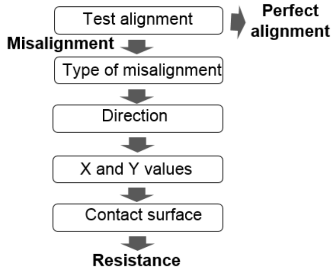
Figure 37: Overall test misalignment flow
