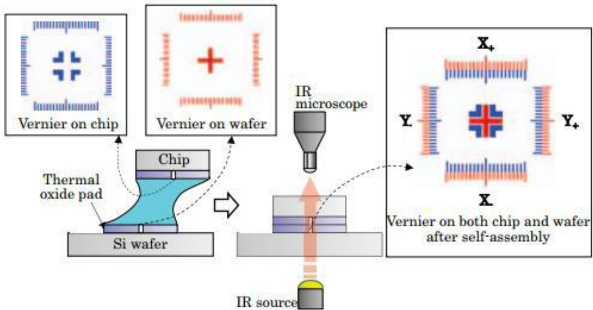
Figure 21: IR metrology tool principle (source [50])
