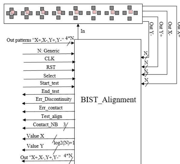
Figure B.1: BIST Alignment architecture
