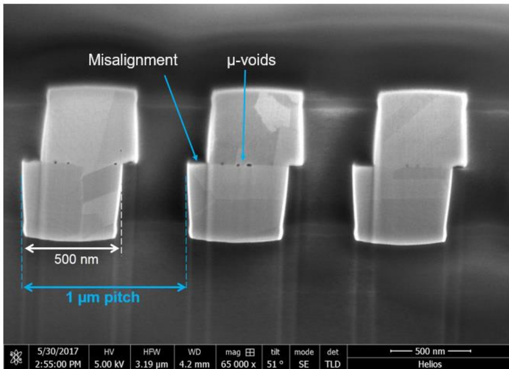
Figure 13: \mu -voids and misalignment defect in Cu-Cu interconnects
