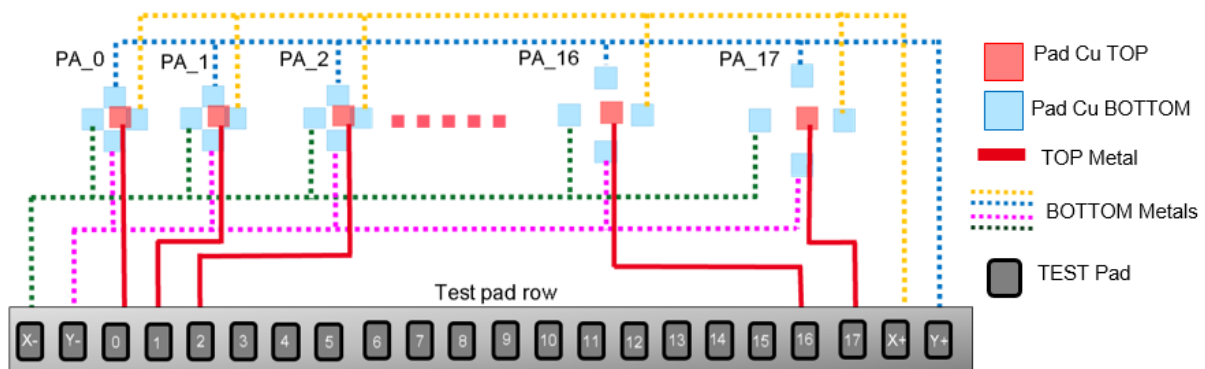
Figure 27: Misalignment test structure architecture
