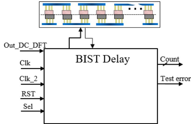
Figure B.2: BIST Delay architecture
