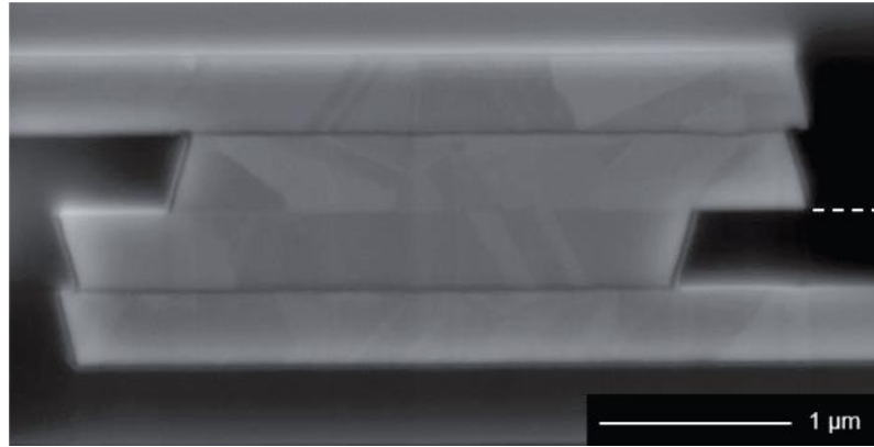
Figure 22: Example of SEM image of Cu-Cu interconnect (source [55])
