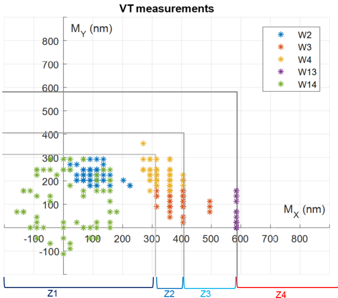
Figure 31: Misalignment test structure results (Pitch= 1.44\mu\text{m} )
