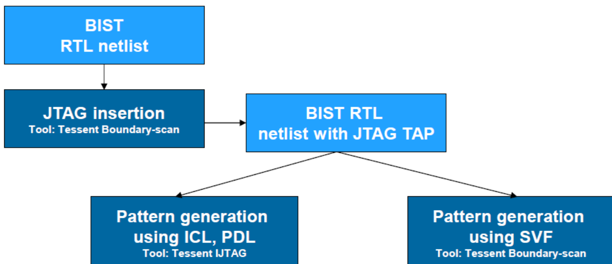
Figure B.3: DFT insertion step
