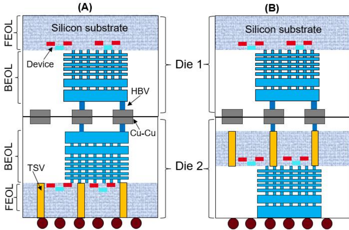
Figure 5: Cross-sectional view of high density 3D-IC structures: (a) F2F, (b) F2B
