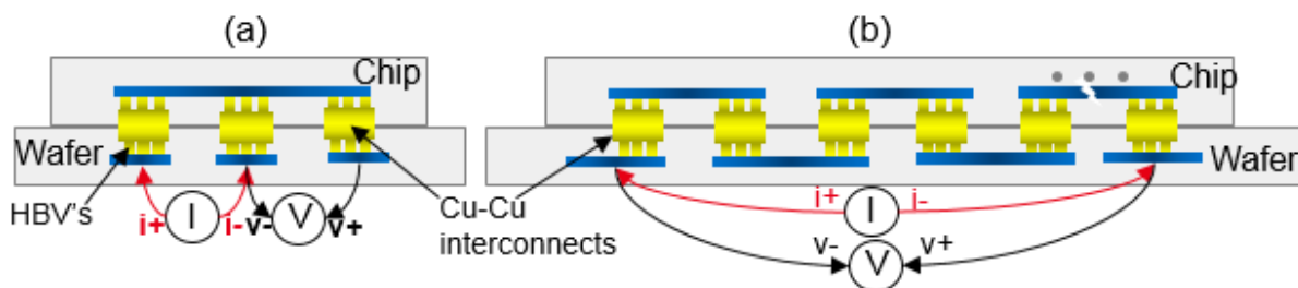
Figure 23: Electrical measurement test vehicle: (a) Kelvin, (b) Daisy chain
