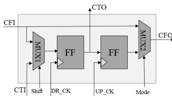
Figure 41: Boundary-Scan-Register (BSR) architecture
