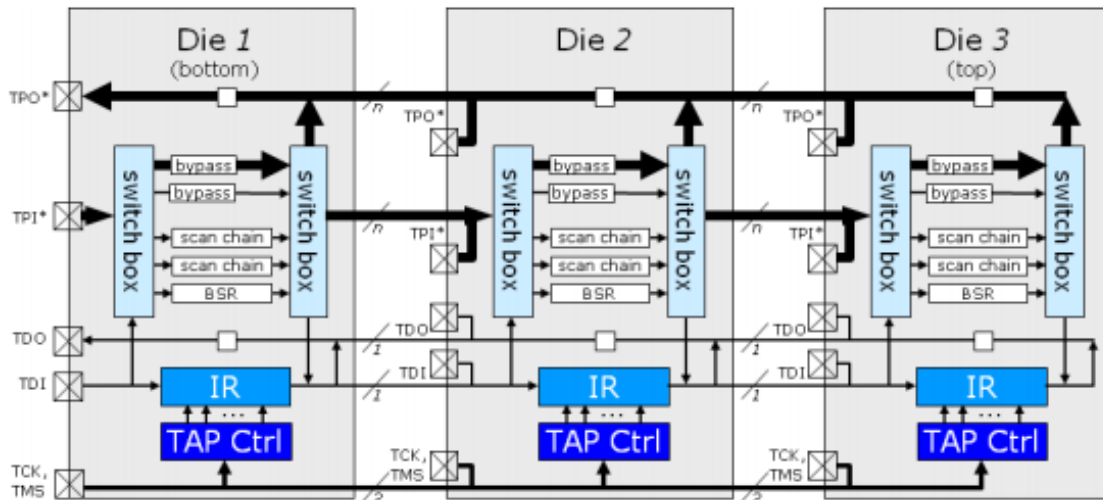
Figure 42: 3D DFT architecture based on IEEE 1149.1 (source [62])
