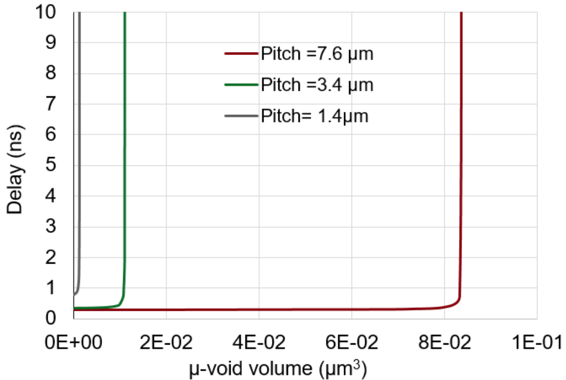
Figure 63: Delay variation of a daisy chain (10,000 Cu-Cu pads) (pitch: 7.6, 3.45 and 1.4 \mu\text{m} ) as a function of \mu -void volume
