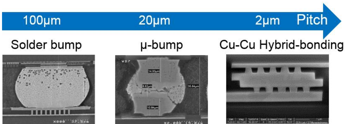
Figure 4: Evolution of inter-dies interconnects
