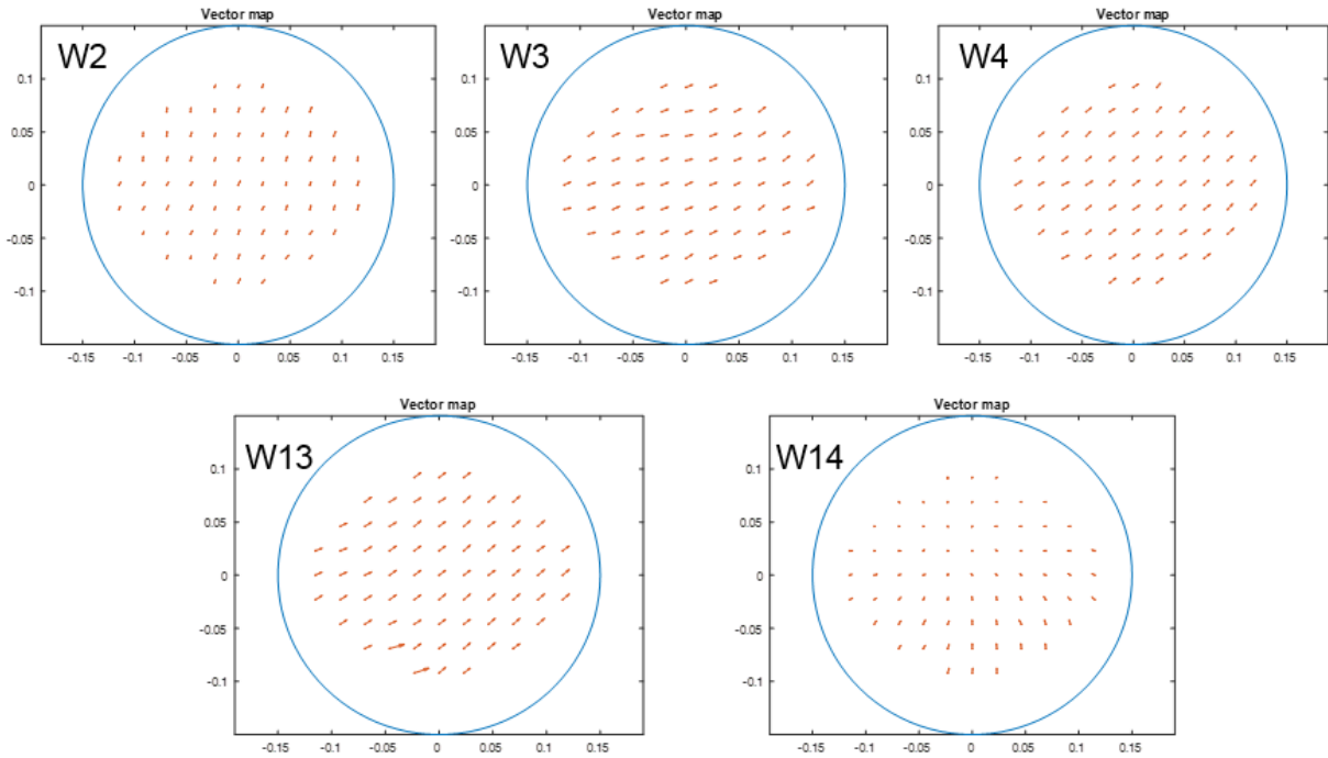
Figure 32: Misalignment wafer map for five wafers (Pitch= 1.44 \mu m)
