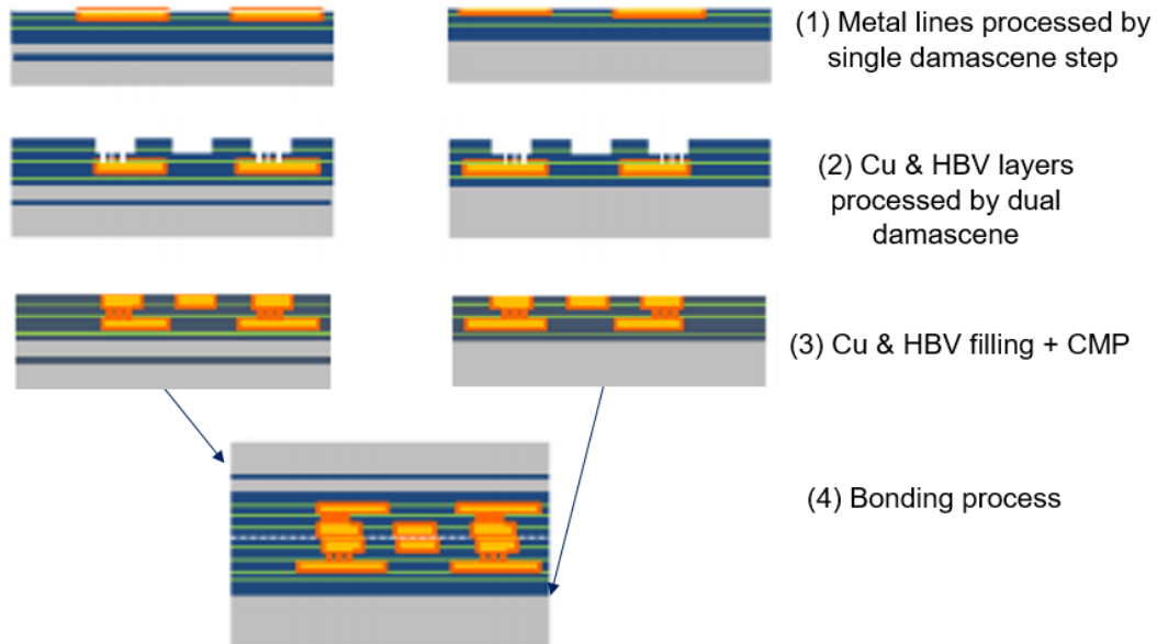
Figure 6: Example of hybrid bonding process flow (source [15])
