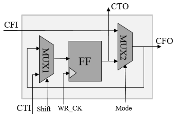
Figure 44: Wrapper-Boundary-Register (WBR) architecture
