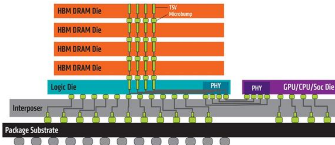
Figure 11: AMD Fury: HBM and CPU/GPU implementation using a passive interposer (source [34])
