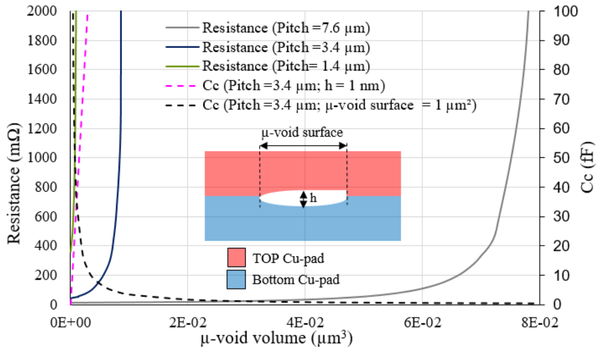
Figure 20: Variation of the resistance and coupling capacitance of a Cu-Cu pad (pitch: 7.6, 3.4 and 1.4 \mu\text{m} ) as a function of \mu -void volume.
