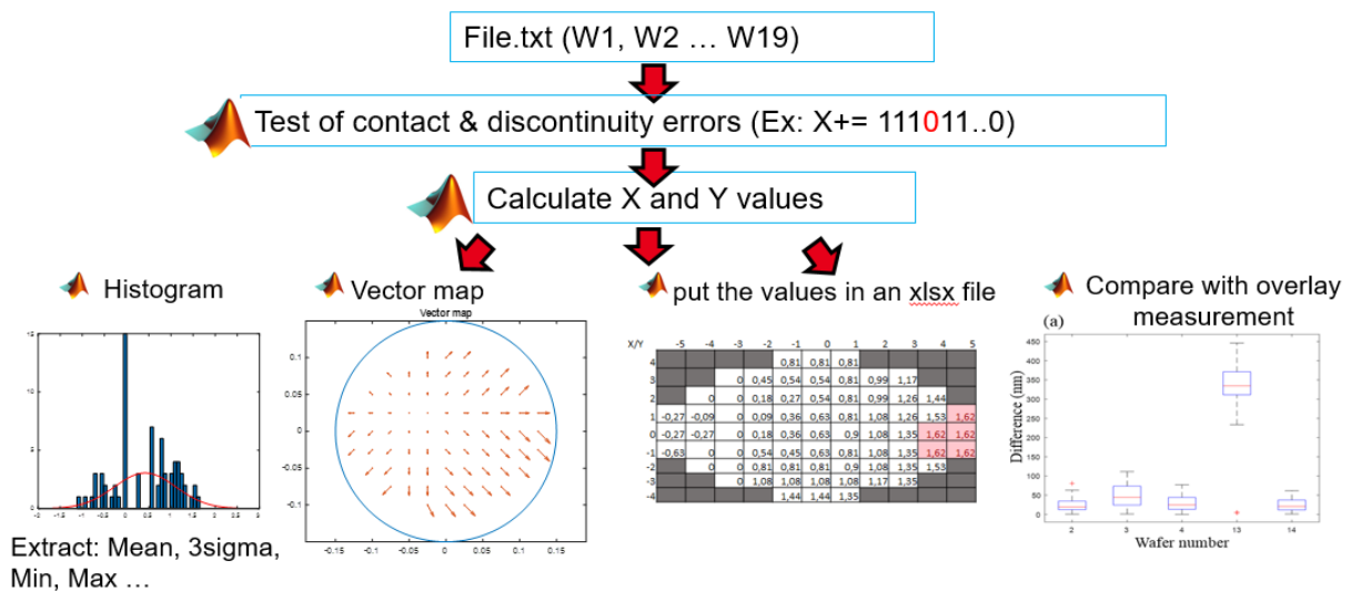
Figure A.1: principle of the developed virtual wafer vector map tool
