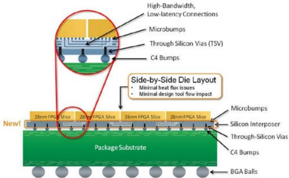
Figure 10: architecture of Virtex-7 HT (source [31])
