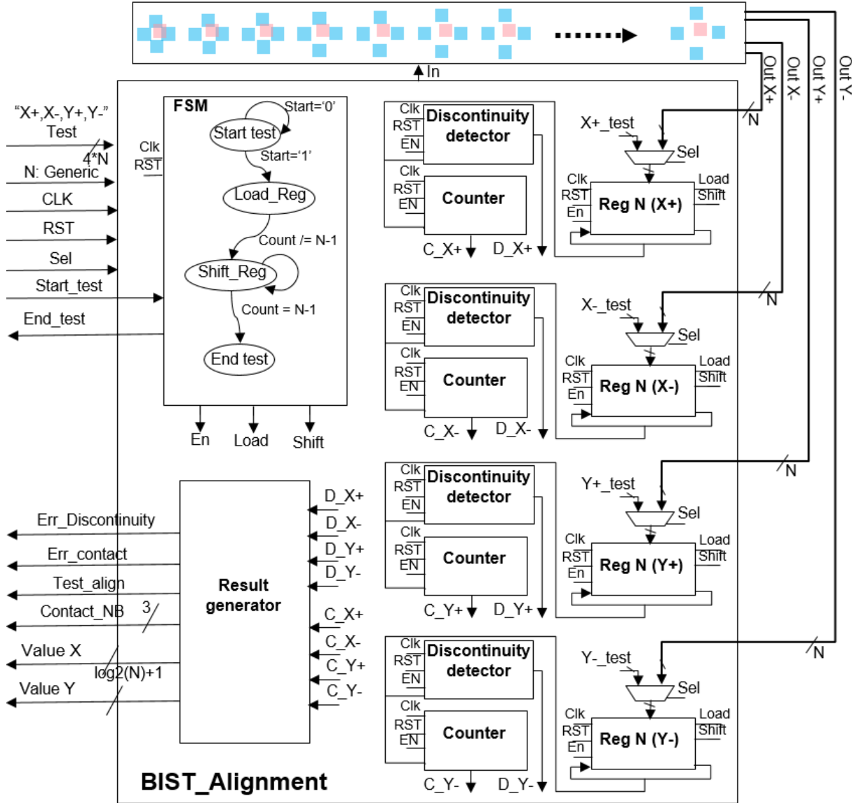
Figure 58: Proposed structural test flow for Cu-Cu interconnects
