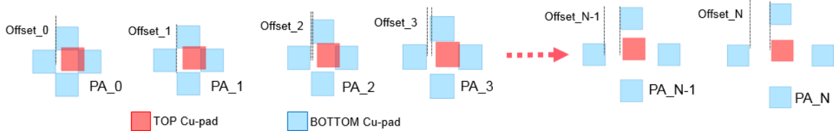
Figure 26: N patterns using different “offset” values
