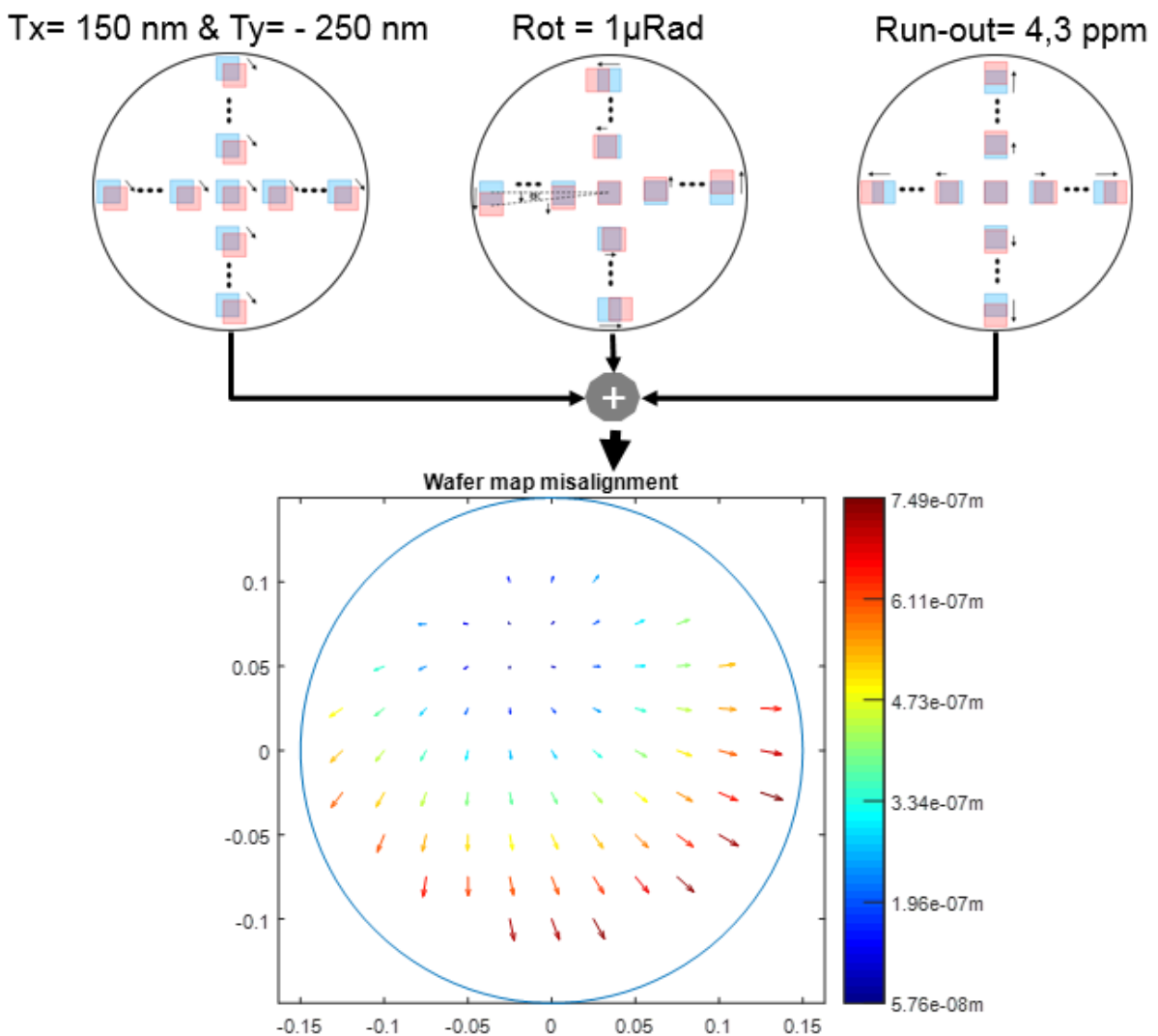
Figure 24: Wafer map: example of misalignment simulation
