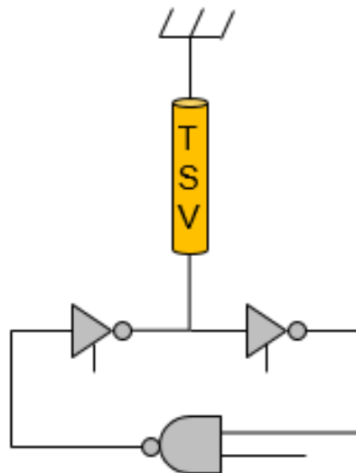
Figure 56: Test TSV using ring oscillator example
