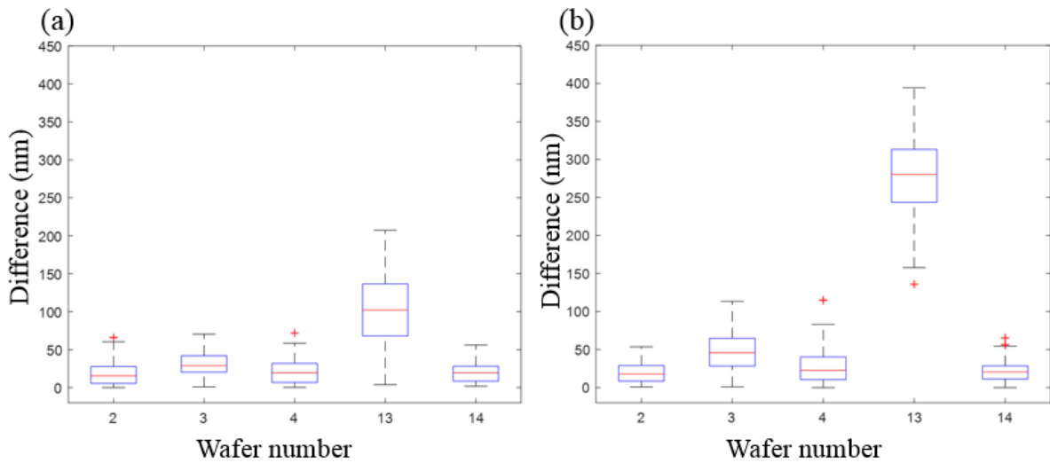
Figure 36: Comparison of test structure results ( 1.44\mu\text{m} pitch) and overlay measurements in X and Y direction
