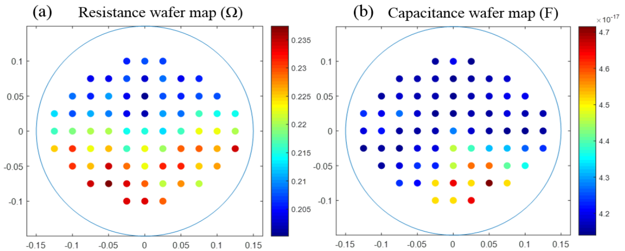
Figure 38: Resistance and capacitance values distribution (W14 with a pitch=1.44 \mu m)
