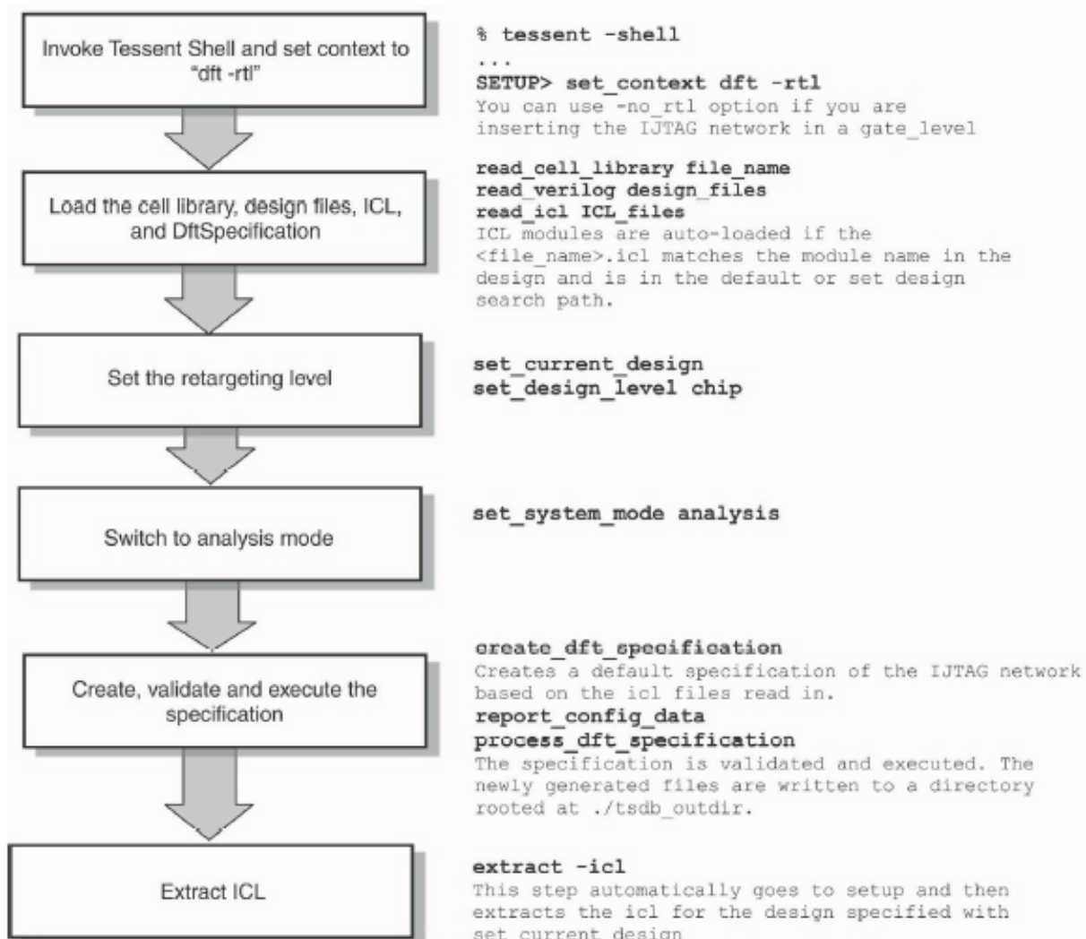
Figure B.4 DFT insertion flow
