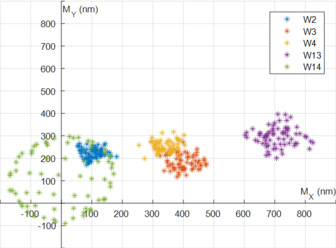
Figure 33: Overlay measurements distribution
