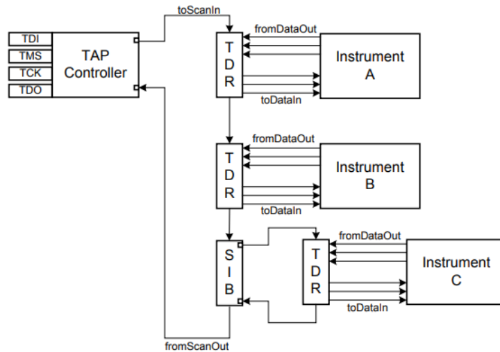
Figure 46: Conceptual IEEE 1687 network
