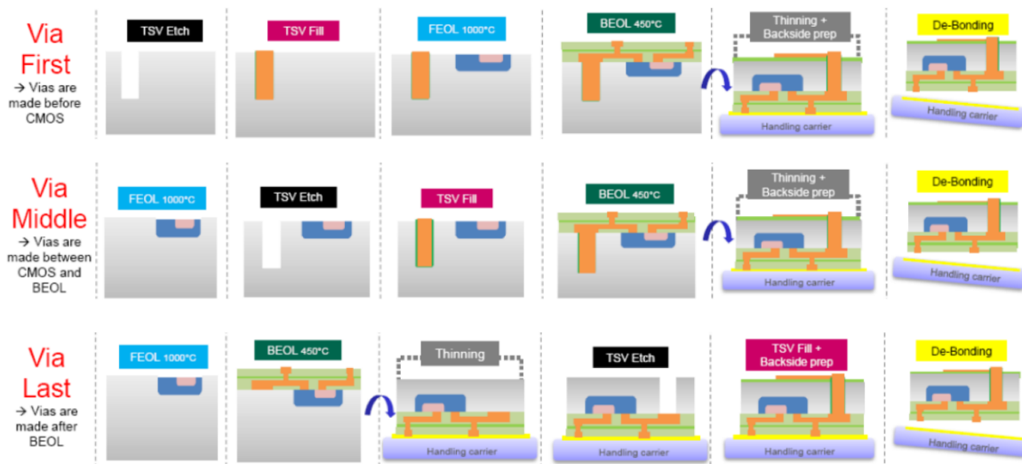
Figure 7: Via-first, via-middle and via-last illustration (source [16])
