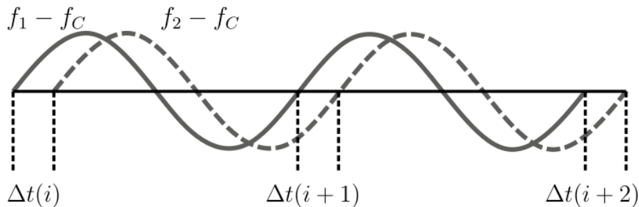
Figure 45. DMTD block diagram presented in (Allan & Daams, 1975) and time diagram showing the time difference measured between beat signals.
