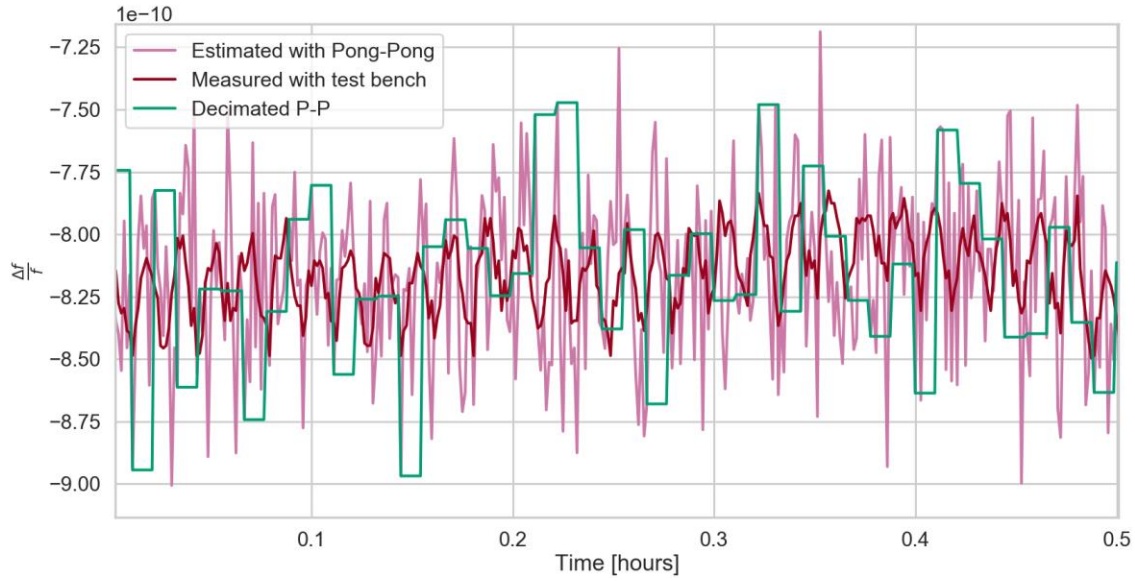
Figure 67. Decimated Pong-Pong transmissions. In pink: estimated clock drift with Pong-Pong technique, in red: clock drift measured with the test bench and in green: decimated Pong-Pong transmissions every 8 Soundings.
