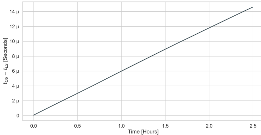
Figure 60. Accumulated time error for start events from the data of the test bench. The test included 2 Syrlinks clocks measured for 2.5 hours.
