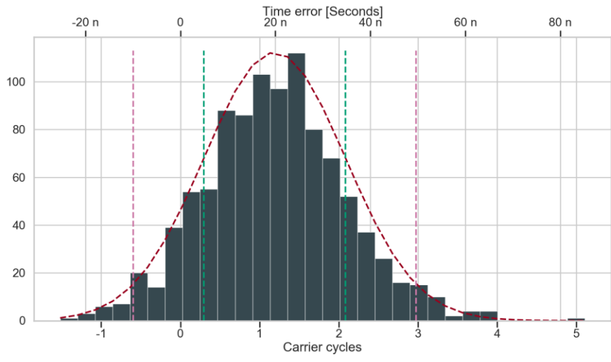
Figure 76. Distribution after 1 hour for 1000 realizations with the time between Pongs being 1 second. \sigma = 1.48 \times 10^{-8} , \mu = 1.98 \times 10^{-8} in carrier cycles.
