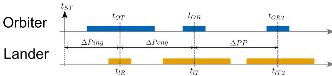
Figure 24. Pong-Pong technique. Two transmissions back from Lander to Orbiter will permit to measure the clock drift between clocks.
