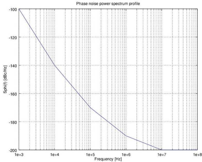
Figure 91. Phase noise profile
