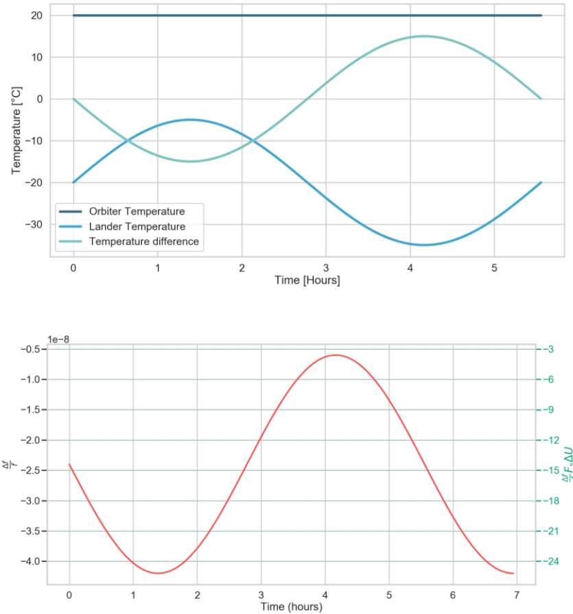
Figure 32. Temperature conversion to the frequency difference. Top: varying temperature for the Lander, constant temperature for the Orbiter and the difference between these two. Bottom: the conversion of the temperature difference to frequency difference using a linear model.
