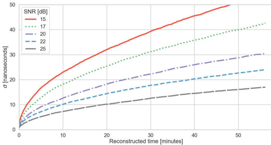
Figure 79. The standard deviation of the accuracy of time reconstruction for different SNR with 1 second between transmissions for 1 hour.
