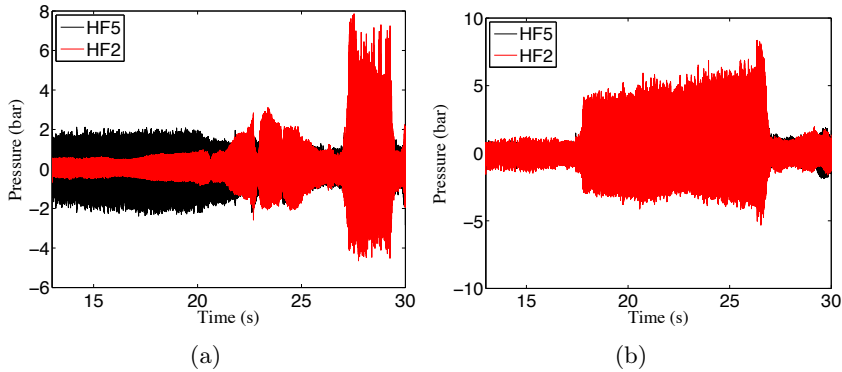
Figure 4.1: (a) PF2 during LFM2. The first six seconds correspond to a monofrequency excitation on the 1T mode (1840 Hz), there is no growth of the acoustic amplitude - (b) PF2 during CWM3 at the 1T2L mode. The amplitude increases from 4 bar to 6 bar during this 8 seconds test.
