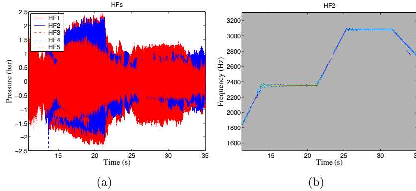
Figure 3.81: PF_4 during CWM1 at SP2 (2350 Hz) and SP4 (3070 Hz) - (a) Response of the HF transducers - (b) Temporal evolution of the HF2 power spectral density. The second frequency does not respond to the excitation as expected.
