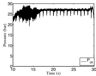
Figure 3.29: PF2 during OWM - Evolution of mean pressure. Before nominal pressure is reached, a low frequency instability is triggered (between 10 and 15 s after the test start) and is finally damped.
