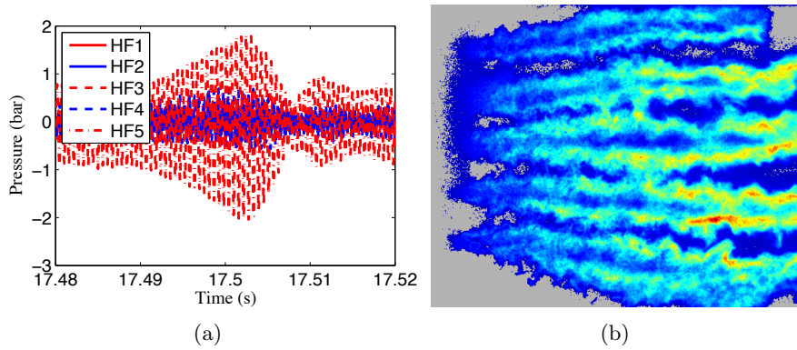
Figure 3.12: PF1 during the LFM at SP1 ( f = 1770 Hz) - (a) Response of the HF transducers signals near the spectral peak - (b) Instantaneous OH^* emission of the flames excited near the peak.
