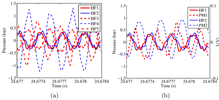
Figure 3.17: PF1 during the LFM at SP3 ( f = 2700 Hz) - (a) Response of the HF transducers - (b) Near injection pressure sensors HF1 and HF2 plotted with the PM signals.
