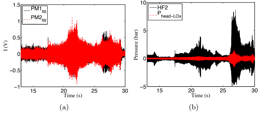
Figure 3.59: PF3 during LFM - (a) Filtered PM signal evolution during the frequency sweep - (b) HF2 response during the frequency ramp plotted with the unsteady pressure in the LOx injection head.
