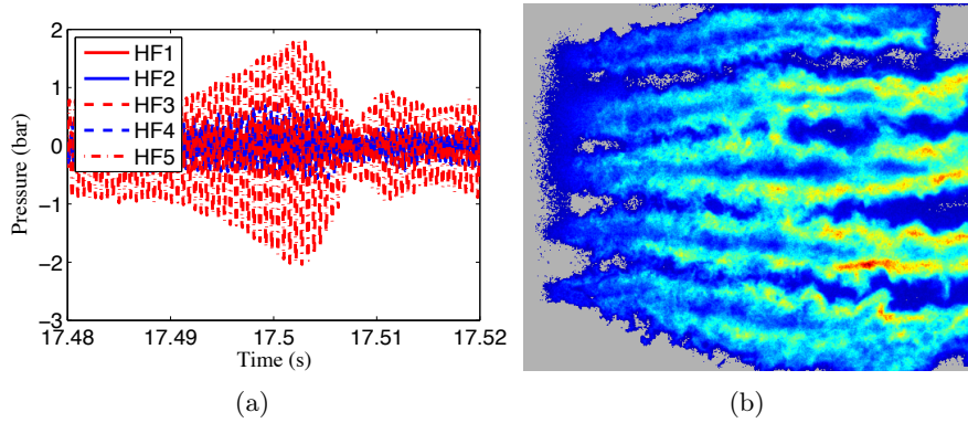
Figure 3.12: PF1 during the LFM at SP1 ( f = 1770 Hz) - (a) Response of the HF transducers signals near the spectral peak - (b) Instantaneous \text{OH}^* emission of the flames excited near the peak.
