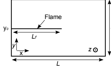
Figure 4.5: Schematic representation of the rectangular chamber with the reference frame of coordinates used in the analytical development. The initial flame position y_0 and its length L_f are also shown.
