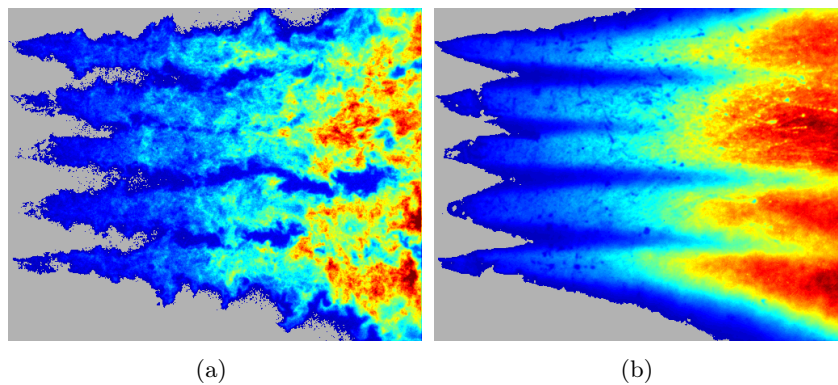
Figure 3.30: PF2 during OWM - (a) Instantaneous OH^* emission of the flames - (b) Averaged OH^* emission of the flames.
