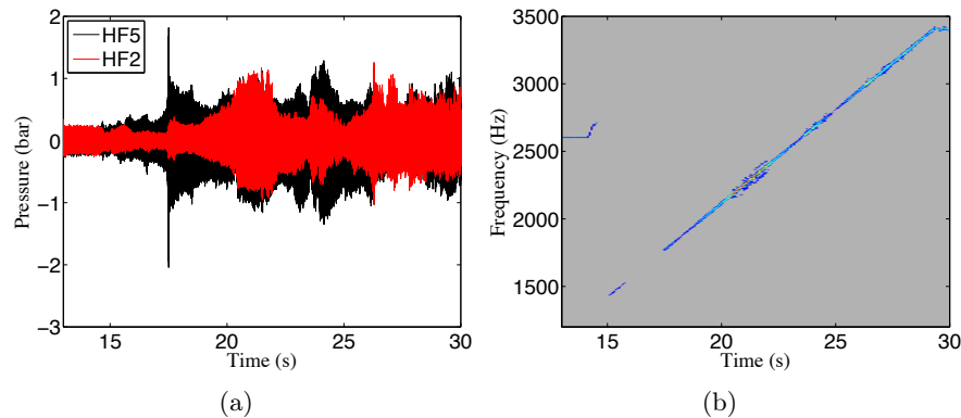
Figure 3.4: PF1 during the LFM - (a) Sensor responses during a frequency sweep. Four peaks emerge from the background noise - (b) Temporal evolution of HF2 power spectral density.
