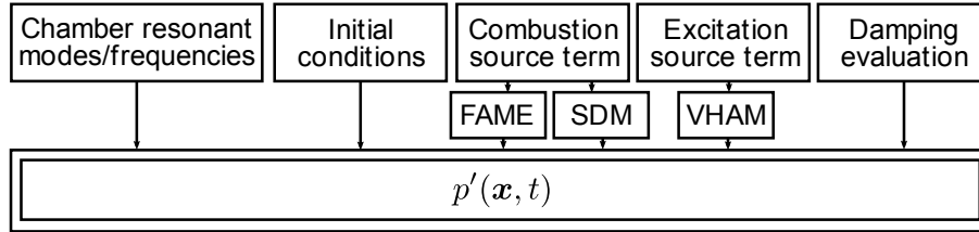
Figure 5.1: Principal constituents of the modeling tool STAability HF (STAHF).
