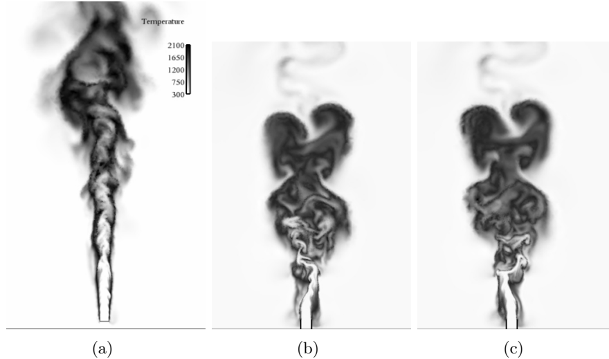
Figure 7.2: Cut of the temperature field - (a) Without excitation - (b) With excitation: \phi = 0 - (c) With excitation: \phi = \pi .
