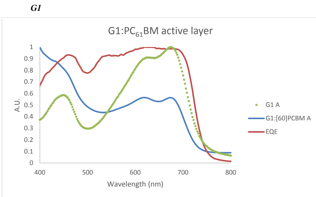
Figure 0-38: Comparison of the UV-visible optical absorption (A) of a G1 and G1:PC 61 BM film with the external quantum efficiency (EQE) of a solar cell with a G1:PC 61 BM active layer.
