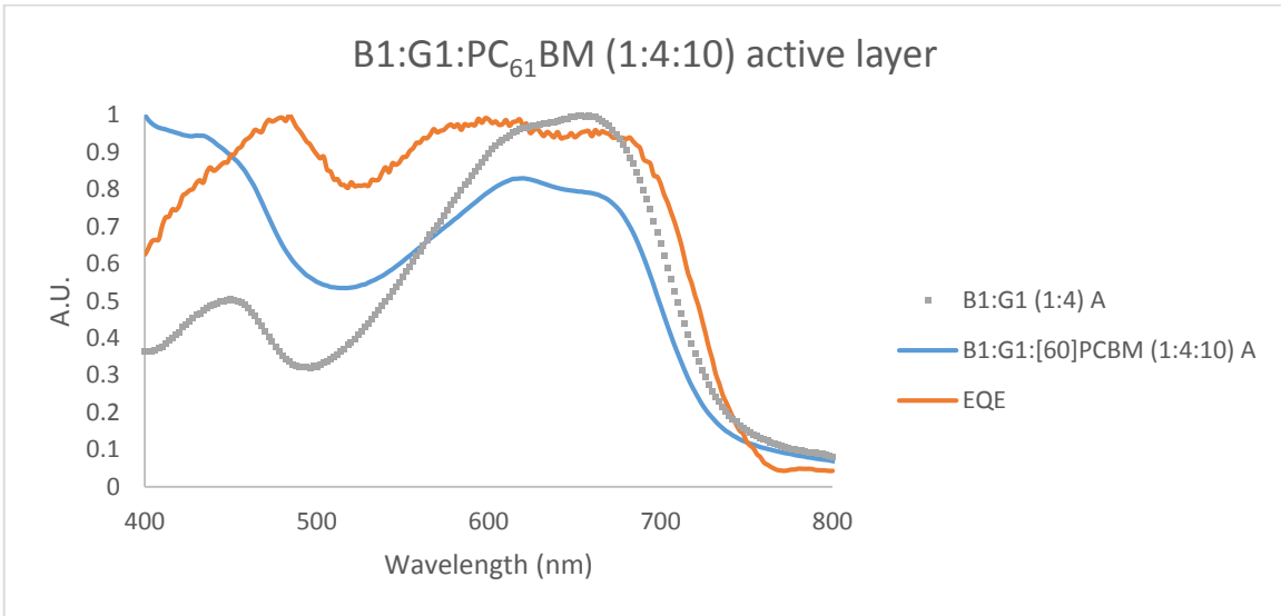
Figure 0-48: Comparison of the UV-visible optical absorption (A) of a B1:G1 (1:4) and B1:G1:PC 61 BM (1:4:10) film with the external quantum efficiency (EQE) of a solar cell with a B1:G1:PC 61 BM (1:4:10) active layer.
