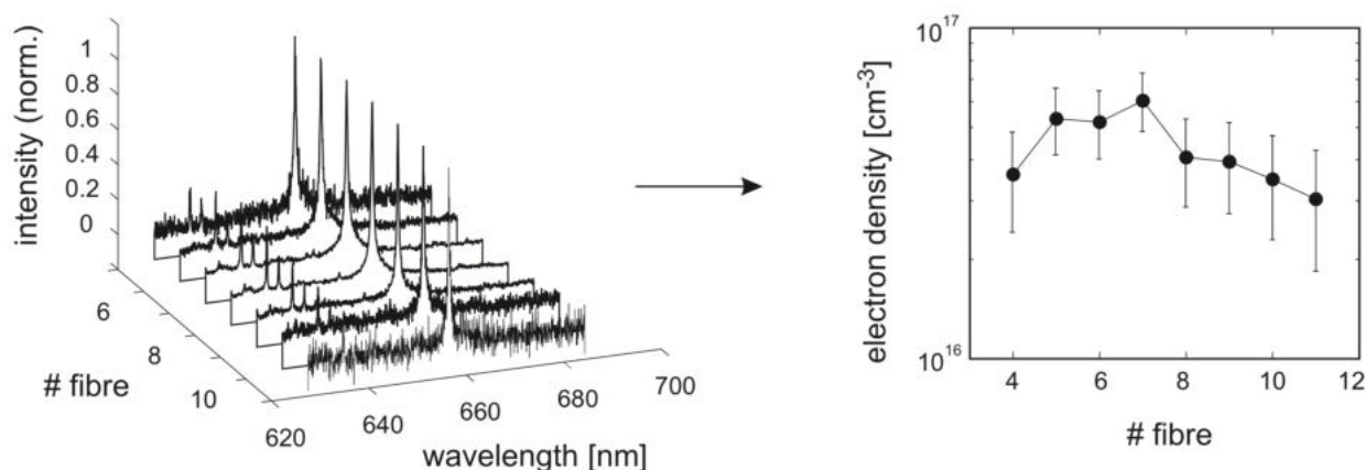
Figure 2.12: Vertical profile of the electron number density calculated from spatially-resolved H_{\alpha} broadening measurements. The spectra are normalized to the intensity of the H_{\alpha} line at 656.2 nm. The light measurement is time integrated over thousands of discharges (6 A, 100 \mu\text{s} , water, 600 \text{ g mm}^{-1} grating) [56].
