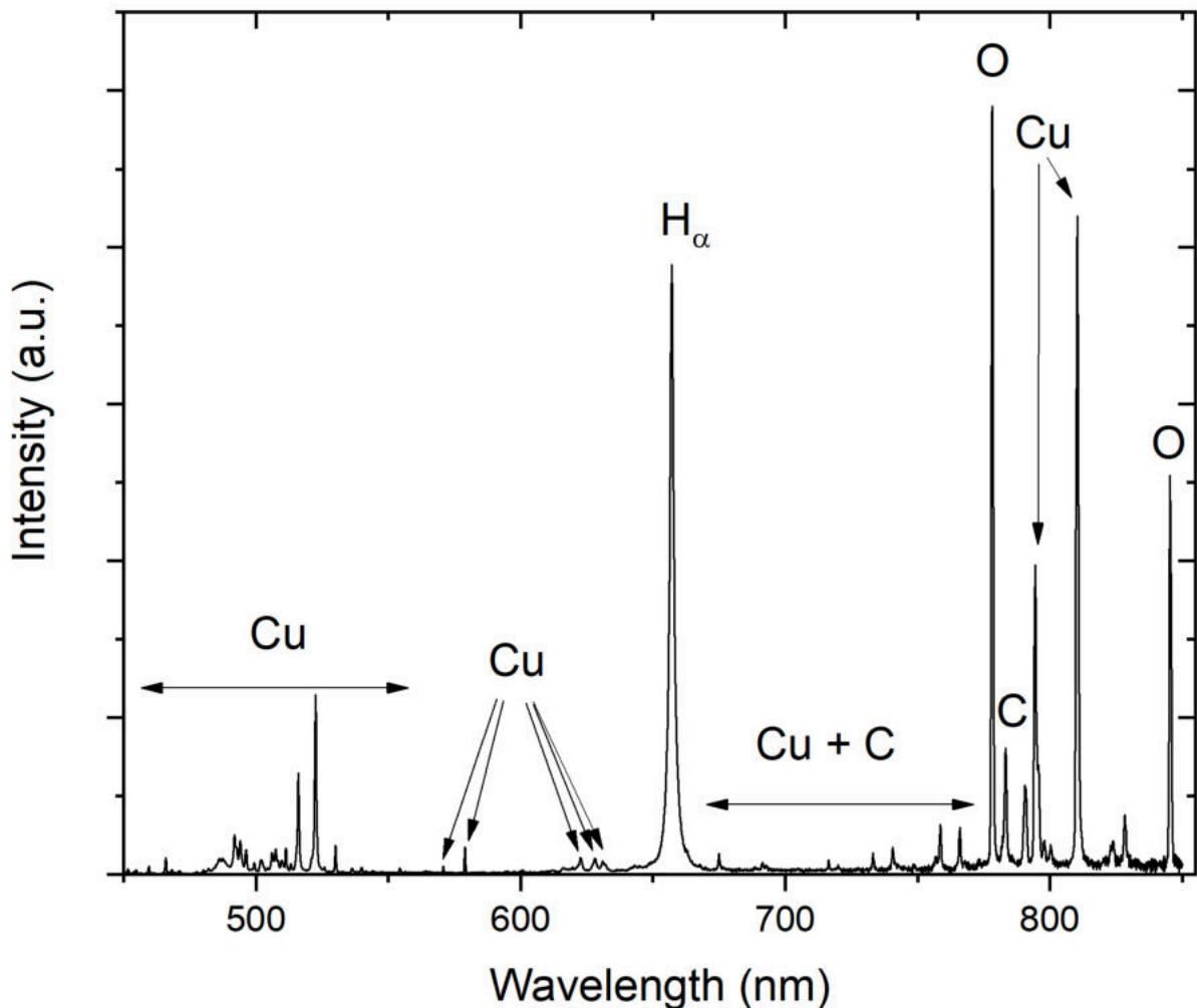
Figure 4.9: Typical emission spectrum of the underwater discharge plasma generated between copper granules: the peak pulse current of about \sim 520 A.
