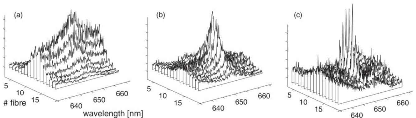
Figure 2.14: Time- and spatially-resolved spectra of the H_\alpha line (Cu/steel, 12 A, 50 \mu s, water; time resolution 2 \mu s, 600 g\ mm^{-1} grating): (a) 0–2 \mu s; (b) 4–6 \mu s; (c) 36–38 \mu s [60].
