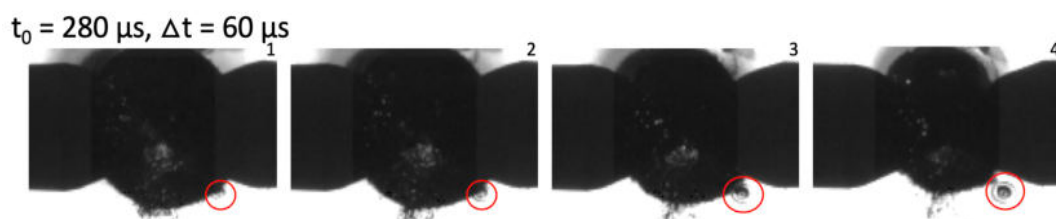
Figure 4.38: Creation of a small gas bubble and its separation from the main bubble surrounding the plasma: high-speed imaging of discharge generated between Cu electrodes in deionized water, peak pulse current of 600 A.
