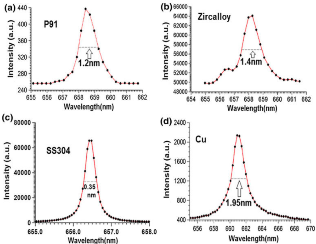
Figure 2.21: Recorded H_{\alpha} line profiles: (a) P91; (b) zircaloy; (c) SS304, and (d) copper anodes [57].
