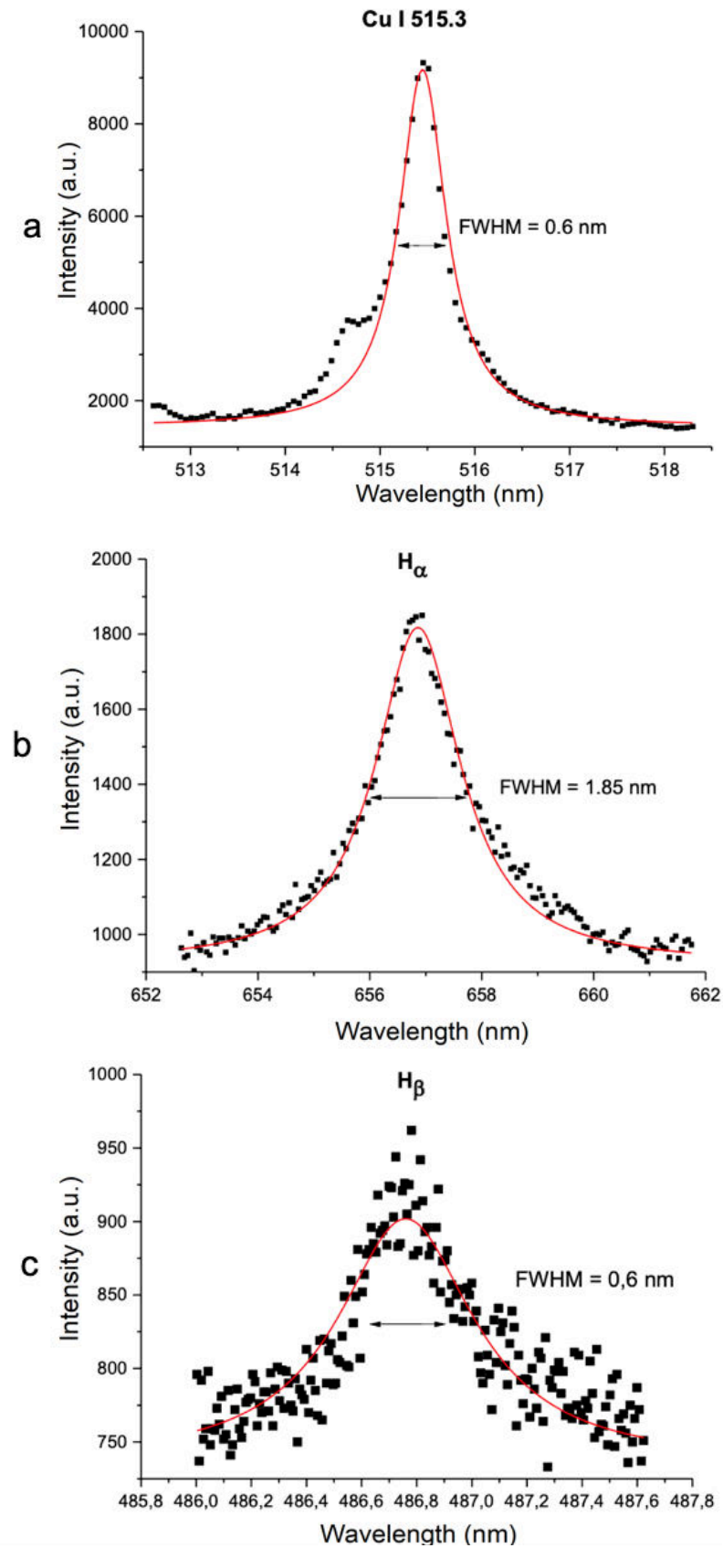
Figure 4.21: Line profiles and Voigt fit of the registered lines for current regime I = 1000 A, radial position r = 0 mm (discharge axis): (a) Cu I 515.3 nm line; (b) H \alpha line; (c) H \beta line [11].
