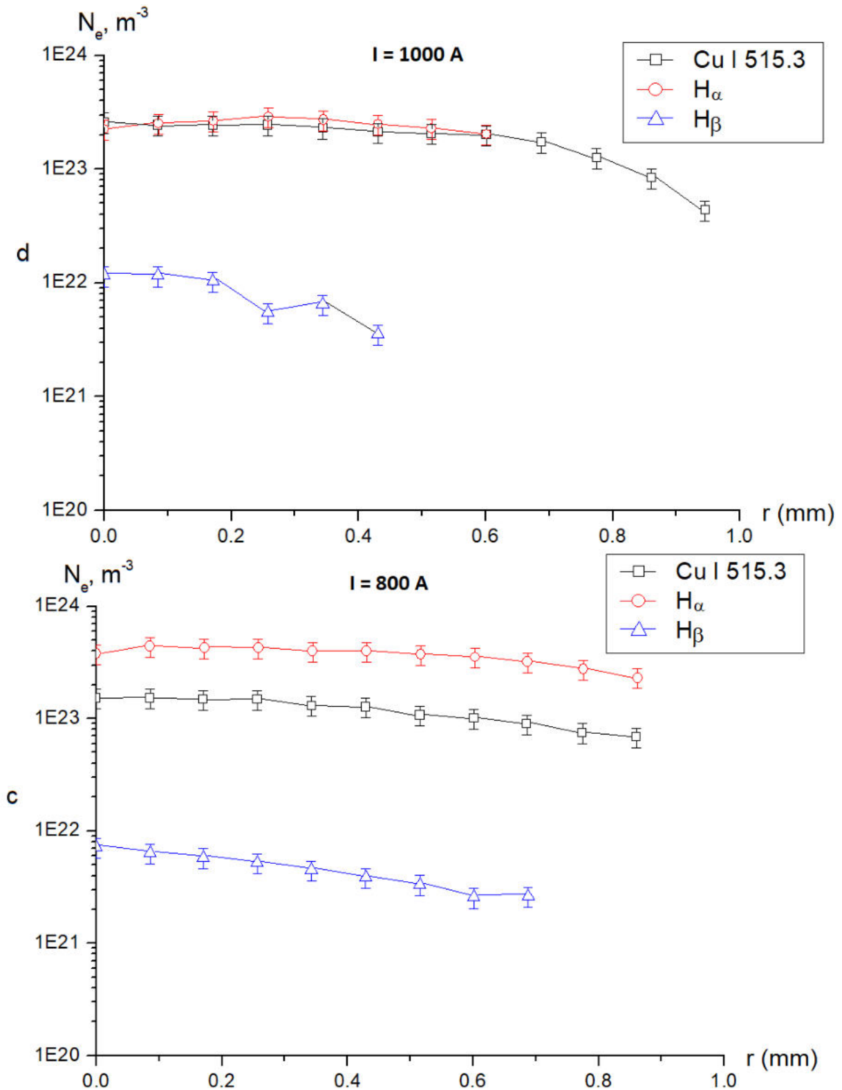
Figure 4.22: Radial profiles of the electron density calculated using broadening of the selected registered lines for different experimental current regimes: (a) I = 450 A , N_e calculated using Cu I 515.3 nm line and H_\alpha line; ( H_\beta line was not registered for this regime); (b) I = 660 A , N_e calculated using Cu I 515.3 nm, H_\alpha and H_\beta lines; (c) I = 800 A , N_e calculated using Cu I 515.3 nm, H_\alpha and H_\beta lines; (d) I = 1000 A , N_e calculated using Cu I 515.3 nm, H_\alpha and H_\beta lines [11].
