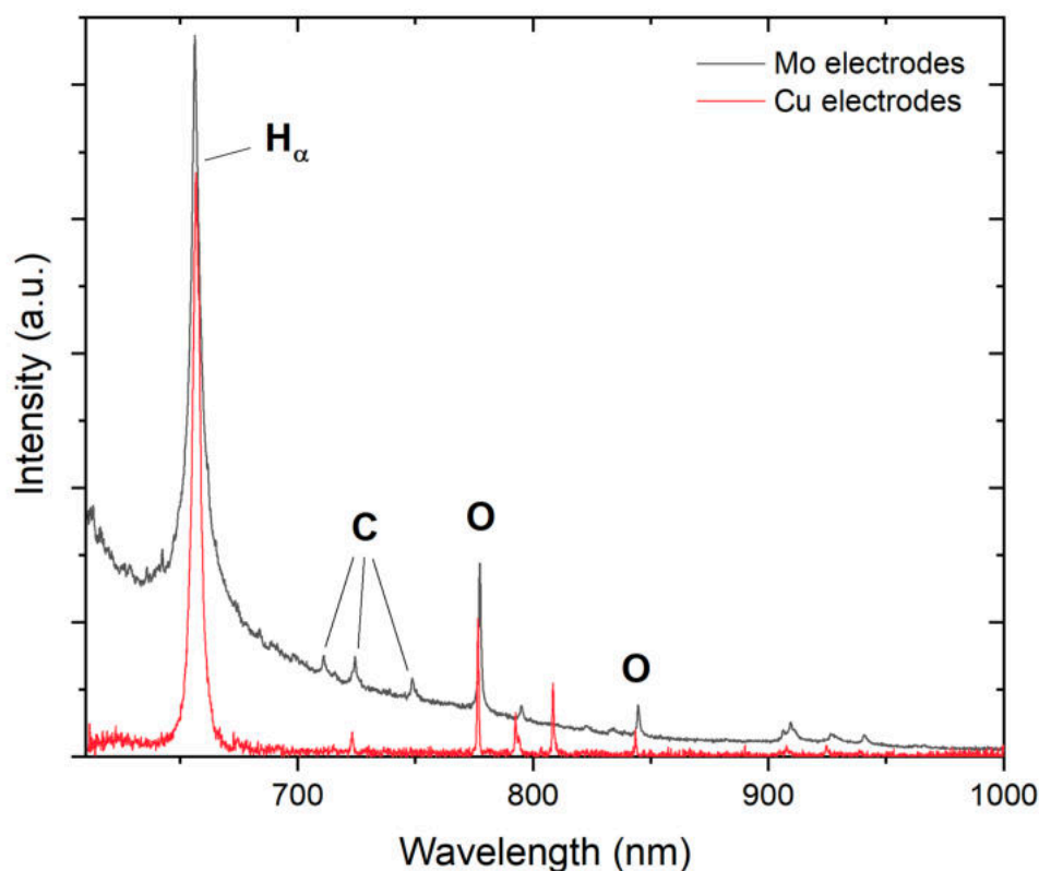
Figure 4.11: Continuum radiation in the emission spectrum of the underwater discharge plasma generated between molybdenum and copper granules: the peak pulse current of about \sim 520 A (fourth spectral range of the spectrometer).
