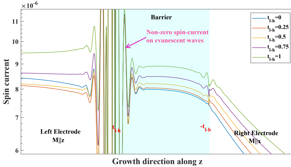
FIGURE 5.6: Profiles of the z -component of the spin current within (\text{Ga,Mn})\text{As}/\text{GaAs}/(\text{Ga,Mn})\text{As} junctions. The magnetization of the thick layer to the left is along z , whereas the one to the right is transverse that is along x for the calculation of the STT. The calculations have been performed with the energy of holes \epsilon = -0.03\text{eV} from the middle of the (\text{Ga,Mn})\text{As} band. Here, the necessary heavy hole - light hole mixing parameter t_{l-h} varies from 0 to 1. This coefficient is set naturally positive and negative at the respective right and left interface of the barrier due to the specific D_{2d} symmetry of the junction of a symmetric profile.
