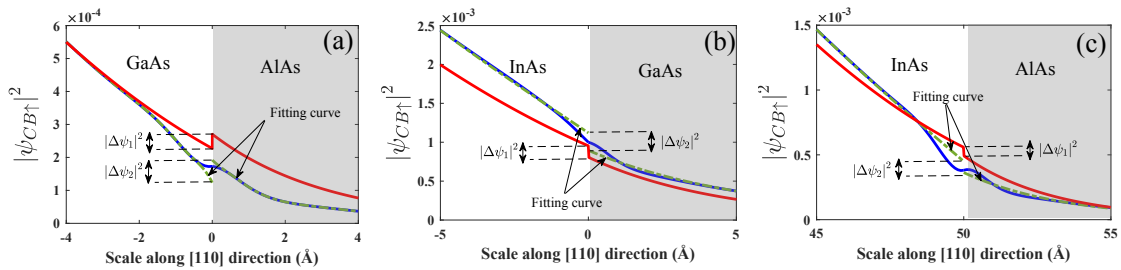
FIGURE 3.4: (a) The zoom in of the wave function in Fig 3.3a close to the interface between GaAs and AlAs showing the jump in both analytical formula \Delta\psi_1 and numerical calculations \Delta\psi_2 with 30 bands \mathbf{k}, \mathbf{p} Hamiltonian. The same calculations have been performed for wave function at InAs/GaAs interface (b) and InAs/AlAs interface (c).
