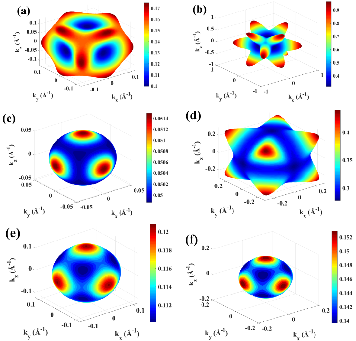
FIGURE 2.22: Fermi surface of heavy hole (a,c), light hole (b,d) and SO band (e,f) with E_f = -0.1\text{eV} (a,b), E_f = -1\text{eV} (b,d,e) and E_f = -1.5\text{eV} (f).
