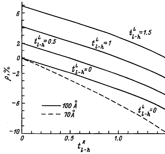
FIGURE 6.18: The anisotropy of optical matrix transition elements as a function of the mixing term parameter at right interface of quantum well originating from HH and LH with different values of mixing term parameter at left interface, taken from Ref.[409].
