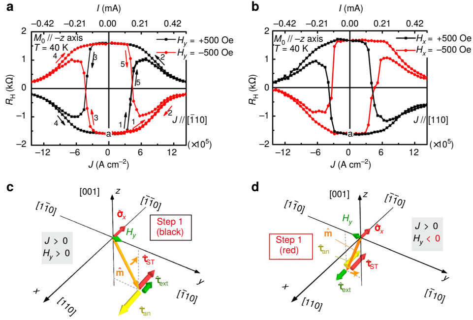
FIGURE 5.1: The SOT switching and the relevant switching mechanism; (a,b) Field-assisted SOT switching with J \parallel [\bar{1}10] and H_y = \pm 500 oe and with J \parallel [110] and H_x = \pm 500 oe. (c,d) illustrations of the torques exerted by the external field ( \tau_{ext} ), the anisotropy field ( \tau_{an} ) and the spin component along the x direction ( \tau_{ST} ) with J > 0 when H_y > 0 and H_y < 0 , here m lies in the y - z plane. Taken from [5].
