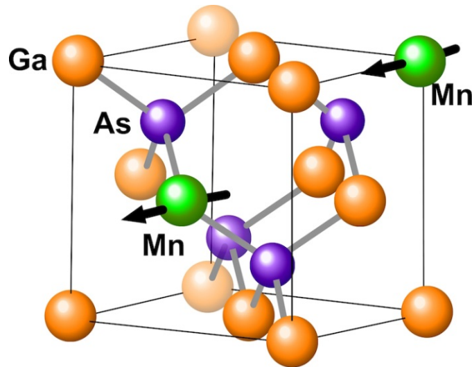
FIGURE 1.6: Crystal structure of (Ga,Mn)As. Mn ions substituting Ga possess a magnetic moment, and the magnetic moment of each Mn ion aligns along the same direction. This implies ferromagnetism of (Ga,Mn)As. Taken from Ref.[66].
