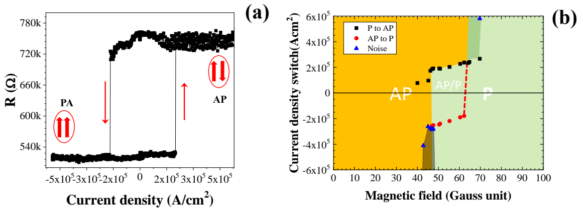
FIGURE 5.10: (a) Spin torque experiment performed on the same nanopillars revealing magnetic reversal for a critical current density of j_{c+} = 2.1 \times 10^5 \text{ A.cm}^{-2} and j_{c-} = -1.9 \times 10^5 \text{ A.cm}^{-2} respectively. The applied field is 55 Oe in the in-plane direction; (b) The magnetization diagram switching for this spin torque experiment.
