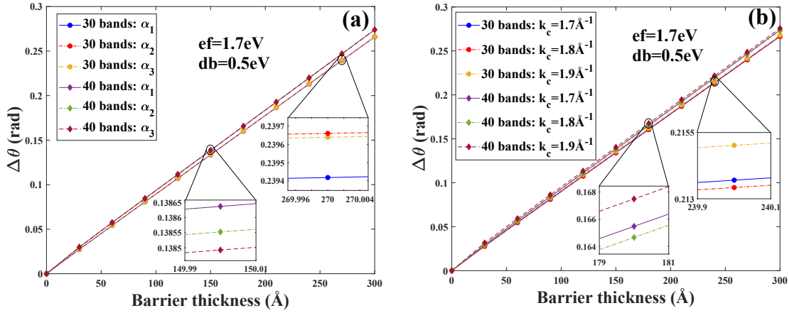
FIGURE 4.8: Spin rotation experienced by the outgoing electron transmitted through the [110] GaAs barrier for different as a function of barrier thickness with fixed barrier height db = 0.5\text{eV} and different ghost-band coupling strength \{\alpha\} (a) and at different k_c (b) showing small differences.
