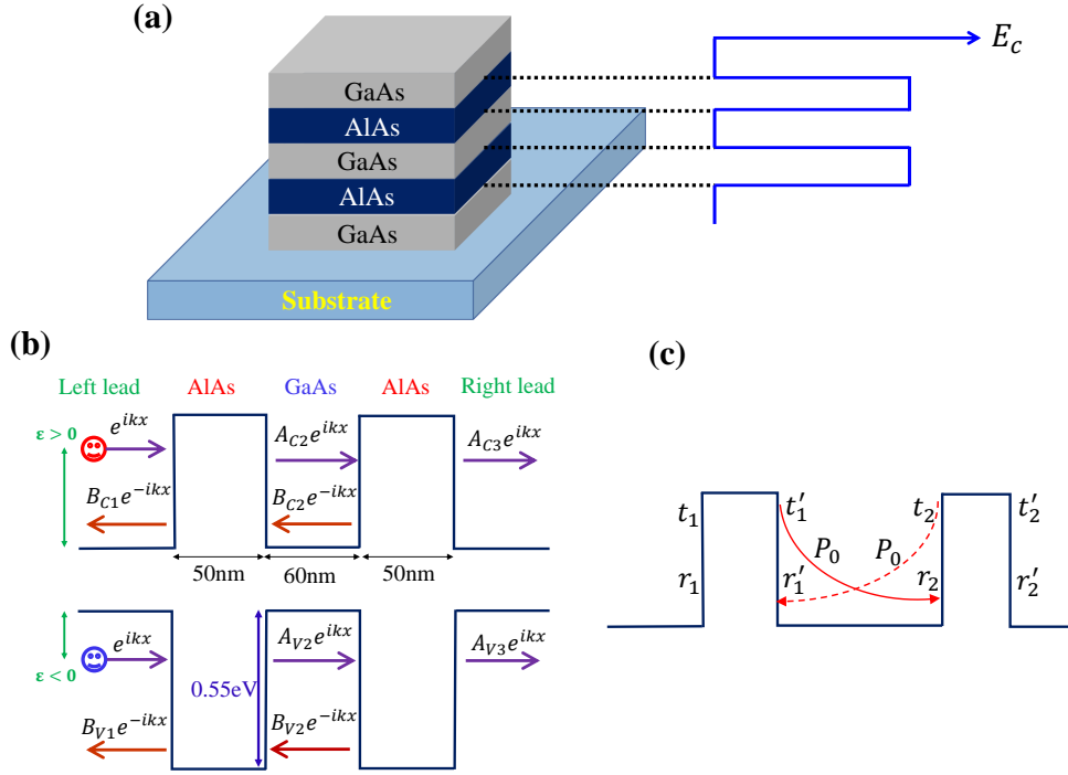
FIGURE 3.8: (a) Scheme of GaAs/AlAs quantum well structures by sandwiching the middle GaAs layer between two AlAs barriers. (b) Resonant tunneling through GaAs/AlAs quantum well structure together with the corresponding amplitude of the waves. (c) Indication of transmission and reflection coefficients as well as propagation inside the considered quantum well structure.
