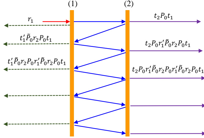
FIGURE C.5: Schematic of scattering process between two interface.
