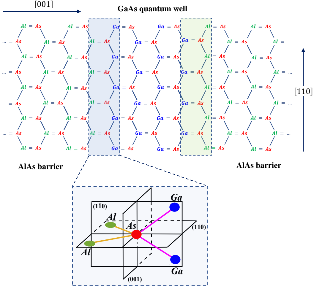
FIGURE 3.16: Schematics of the nearest neighbors of an As interface atom of GaAs/AlAs quantum well structure where the point symmetry C_{2v} of a single heterojunction contains the twofold rotation axis C_2 parallel to the growth direction [001] and two mirror planes [110] and [1\bar{1}0]
