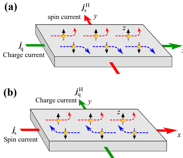
FIGURE 1.13: (a) Charge-current-induced Spin Hall effect (SHE) in which the charge current j_q along the x -direction induces the spin current j_s^H in the y -direction with the polarization parallel to the z -axis. (b) Inverse Spin Hall effect (ISHE) in which the spin current j_s flowing along the x -direction with the polarization parallel to the z -axis induces the charge current j_q^H in the y -direction, taken from Ref.[113].
