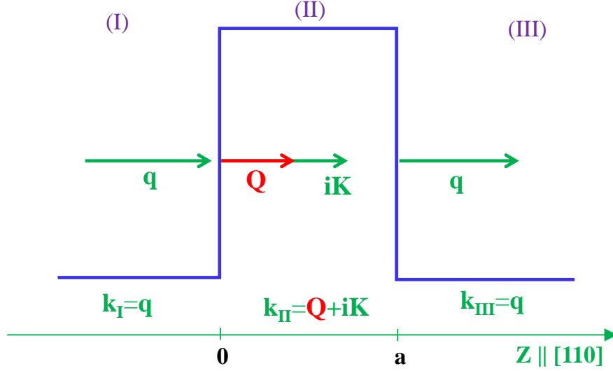
FIGURE 3.1: Sketch of the tunnel geometry with notations. The spin-orbit-split barrier material of thickness a (medium II is located between two free-electron like materials (media I and III). The tunnel axis, normal to the barrier, is the z axis. In the free-electron like materials, the real normal incident electron wave vector in the z direction is referred to as q . In the barrier material, the evanescent wave vector along the z axis is referred to as Q + iK , where Q and K are real quantities. The transverse wave-vector component is in the barrier plane. Then, the overall wave vectors in the three media are, respectively, k_I = k_{III} = q and k_{II} = Q + iK .
