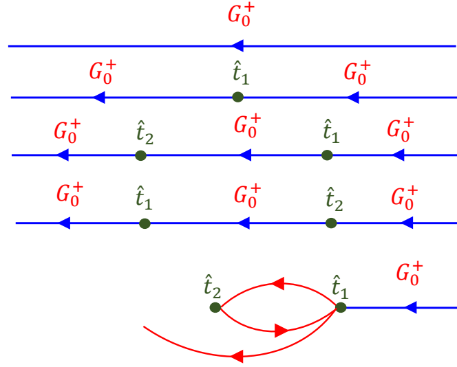
FIGURE 4.1: Scheme of Green function where \hat{t}_1 and \hat{t}_2 symbols design scattering evens at the interfaces of a heterostructure.
