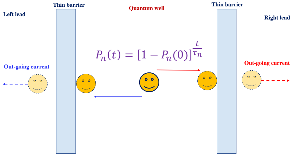
FIGURE 3.14: Scheme of a quasi-bound state in a quantum well structure. An electron with maximum occupation probabilities at the middle of quantum well decrease with time since each time the electron hits the barriers, it may tunnel through barrier with a small probability.
