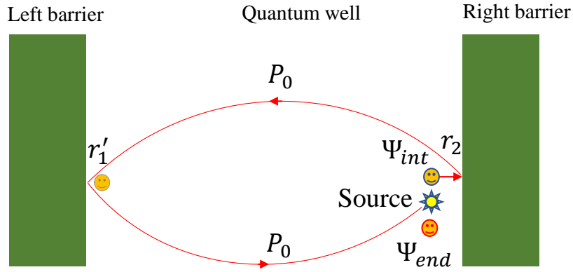
FIGURE 3.10: Scheme of bounded motion or bound state of an electron in a quantum well structure. \Psi_{int} is the initial wavefunction of the electron and \Psi_{end} is the ending wavefunction of the electron after one (or many) period of motion; r'_1 and r_2 are the reflection coefficient of the left barrier and right barrier, respectively; P_0 is the propagation within quantum well (thank to the inversion time symmetry, the propagation from left to right and from right to left are the same and denoted by P_0 ).
