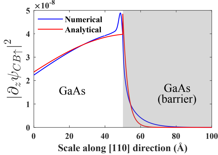
FIGURE 3.2: The derivative of wave function close to the interface between GaAs on the left and GaAs barrier (by adding a fictitious barrier height) one the right sides. This figure show the jumps of derivative wave function at the interface in a good agreement between analytical formula and numerical calculation.
