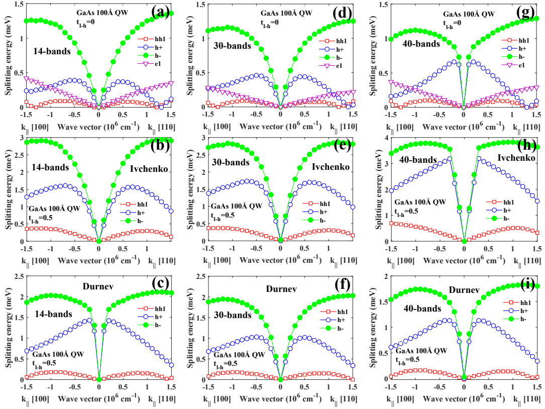
FIGURE 3.25: Splitting of valence subbands in GaAs/AlAs 10nm QW calculated with different k.p platforms (depicted in the figure), for two values of the mixing term t_{l-h} = 0 and t_{l-h} = 0.5 with two sets of boundary conditions proposed by Ivchenko et al. [30] and Durnev et al. [31].
