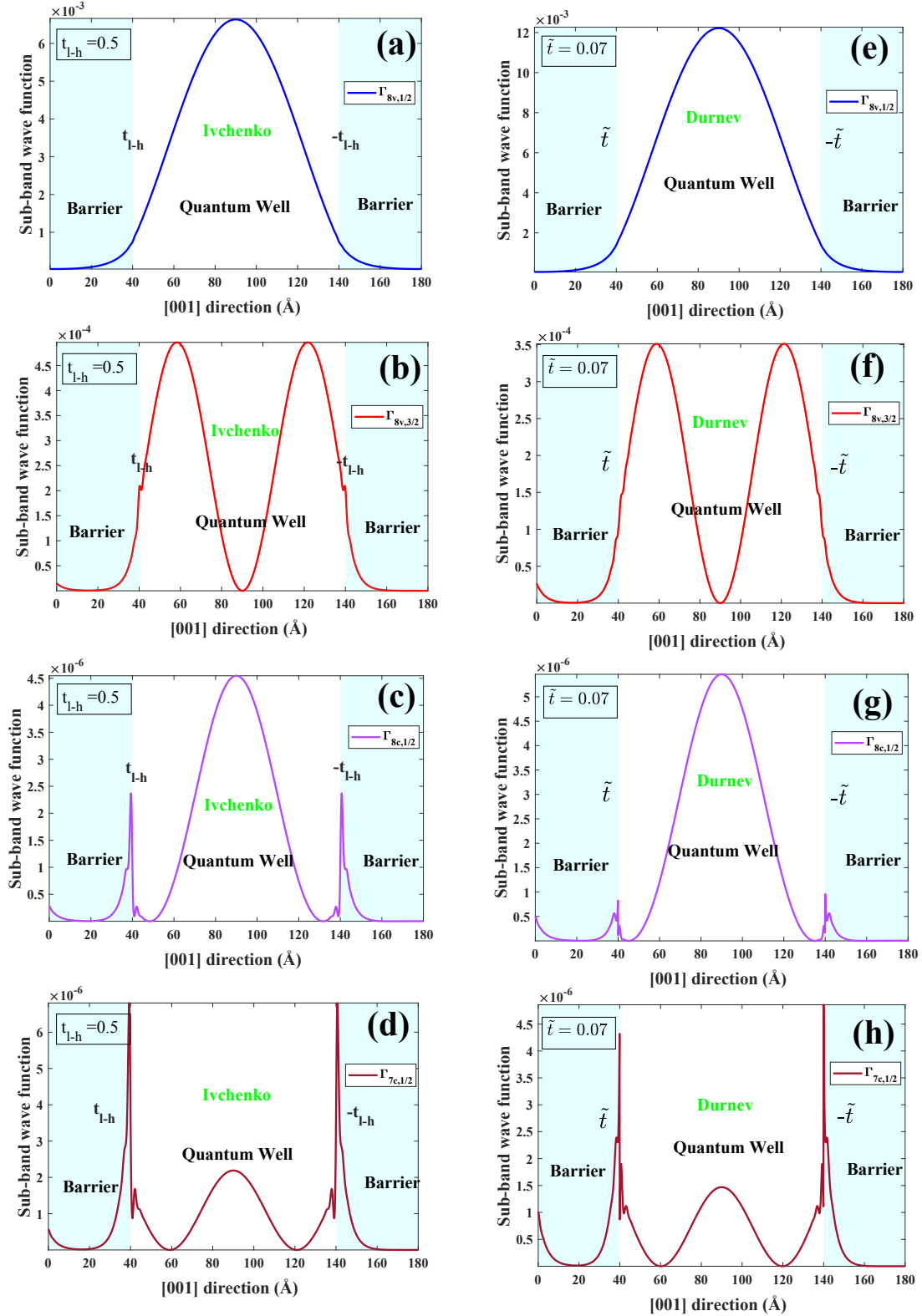
FIGURE 3.22: The envelope functions in a GaAs/AlAs quantum well calculated in the framework of 30-band k, p theory with Ivchenko's matching conditions t_{l-h} = 0.5 (a-d) and Durnev's matching condition \tilde{t} = 0.07 (e-h) with normal incidence k_{||} = 0 for corresponding LH_1 (h+) energy level. The calculated wavefunctions are the scattered waves propagating from left to right.
