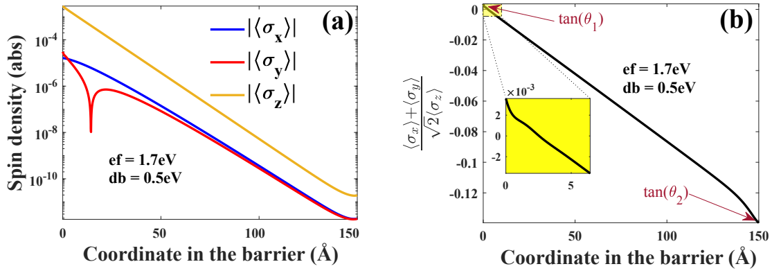
FIGURE 4.5: (a) Spin density profile \langle \sigma_i \rangle along the respective i = x, y, z directions (the [100]-, [010]- and [001]-direction respectively) calculated using our 30-band \mathbf{k} \cdot \mathbf{p} platform for an incoming electron crossing a [110] GaAs tunnel barrier with incoming spin aligned along the z direction; (b) Same calculations giving the ratio \frac{\langle \sigma_x \rangle + \langle \sigma_y \rangle}{\sqrt{2} \langle \sigma_z \rangle} showing the gradual rotation of the spin component in the {[001], [110]} plane. The rotation is a manifestation of the spin dephasing effect. A nonzero value of \theta at the interface (the positive value of \frac{\langle \sigma_x \rangle + \langle \sigma_y \rangle}{\sqrt{2} \langle \sigma_z \rangle} close to origin depicted in inset figure) shows the spin mixing conductance of interface.
