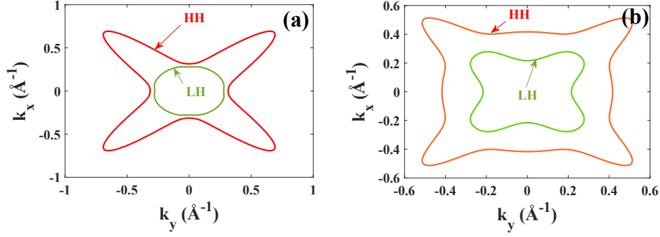
FIGURE 2.21: Constant energy surface of Heavy Holes (HH) and Light Holes (LH) in the GaAs band structure with E_f = -0.1 eV and E_f = -1 eV, Figure (a) and (b) respectively.
