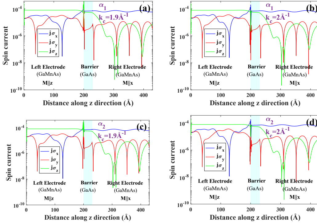
FIGURE 2.15: The 3 spin-current components through (Ga,Mn)As/GaAs/(Ga,Mn)As trilayer structure, the magnetization in the left and in the right electrode are aligned respectively along the z and x directions, within an extended 30-band \mathbf{k}\cdot\mathbf{p} framework calculated for strictly normal incidence ( k_{\parallel} = 0 ) and for different ghost-spurious coupling strength \alpha : \alpha_1 = 1.5 eV \cdot \text{\AA}^{-2} Figs. (a,b) and \alpha_2 = 2 eV \cdot \text{\AA}^{-2} Figs. (c,d) and at different coupling points k_c as depicted in the figure.
