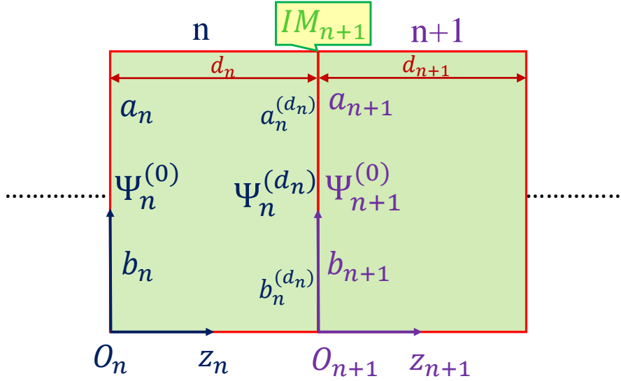
FIGURE C.1: The wave function in n^{th} layer and (n+1)^{th} layer. \Psi_n^{(0)} is the wavefunction at O_n point in n th layer, a_n and b_n are coefficients corresponding to \Psi_n^{(0)} ; \Psi_n^{(d_n)} is the wavefunction at d_n point in n th layer, a_n^{(d_n)} and b_n^{(d_n)} are coefficients corresponding to \Psi_n^{(d_n)} ; \Psi_{n+1}^{(0)} is the wavefunction at O_{n+1} point in n th layer, a_{n+1} and b_{n+1} are coefficients corresponding to \Psi_{n+1}^{(0)} . Here O_i z_i is the proper coordinate in i^{th} layer where O_i was chosen as the point at the interface between (i-1)^{th} and i^{th} layer.
