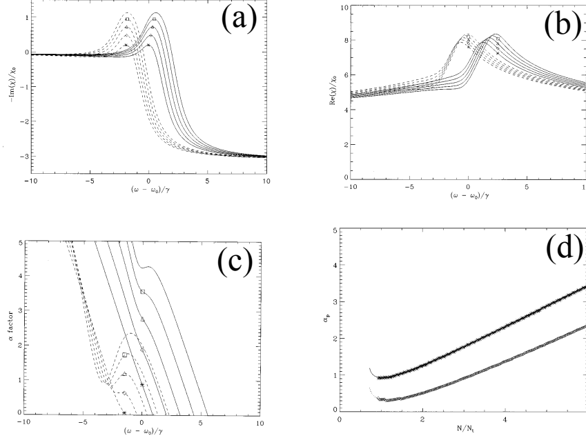
FIGURE 6.19: (a) Normalized imaginary part of the susceptibility as a function of the normalized frequency deviation from the nominal band-gap frequency (\omega - \omega_0) / \gamma , for increasing carrier densities N/N_t = 1.2 (star), 1.5 (diamond), 1.8 (triangle), 2.1 (square), and 2.4 (no symbol). Solid lines correspond to \sigma = 0.2 , while dashed lines correspond to \sigma = 2 ; (b) Normalized real part of the susceptibility as a function of the normalized frequency deviation from the nominal band-gap frequency (\omega - \omega_0) / \gamma for the same carrier densities and \sigma values as in figure a; (c) Line width enhancement factor \alpha as a function of the normalized frequency deviation from the nominal band-gap frequency, (\omega - \omega_0) / \gamma for carrier densities n/N_t = 1.17 (star), 2.37 (diamond), 3.57 (triangle), 4.77 (square), and 5.97 (no symbol). Solid lines correspond to \sigma = 0.2 , while dashed lines correspond to \sigma = 2 ; (d) Line width enhancement factor at the gain peak, \alpha_p , as a function of the normalized carrier density N/N_t . The symbols denote value obtained numerically from the electrical susceptibility, while the solid line corresponds to equation (18) in Ref. [410]. Taken from Ref. [410]
