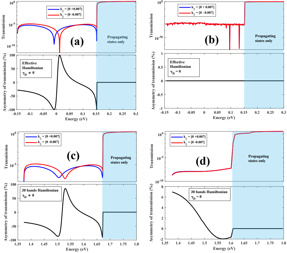
FIGURE 5.23: The transmission coefficient for plus and minus inplane wave vector k_{||} and transmission asymmetry for an electron in CB tunnels through exchange step junction with antiparallel configuration of magnetization. Figs (a, b) are calculations using effective Hamiltonian (without s-p hybridization) with and without Dresselhaus term \gamma_D \neq 0 ( \gamma_D = 0 ). (c, d) are calculations using 30 bands Hamiltonian (taking into account s-p hybridization) with and without Dresselhaus term \gamma_D \neq 0 ( \gamma_D = 0 ).
