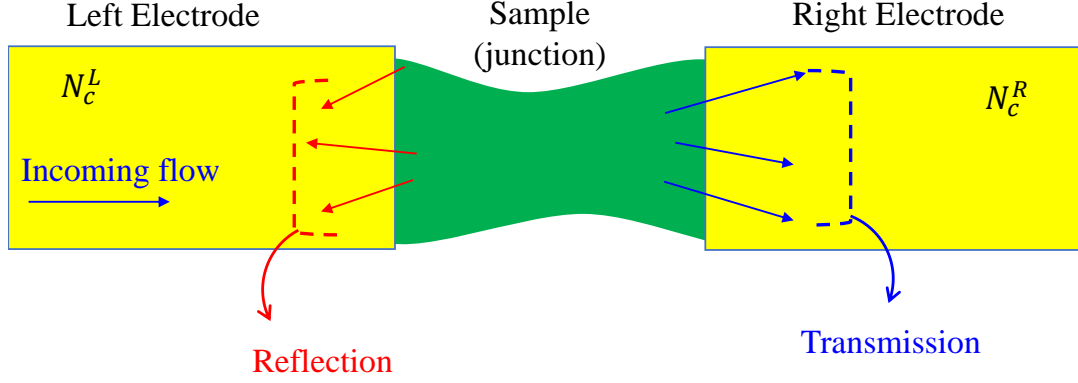
FIGURE 3.7: Reflected and transmitted wave at the junction.
