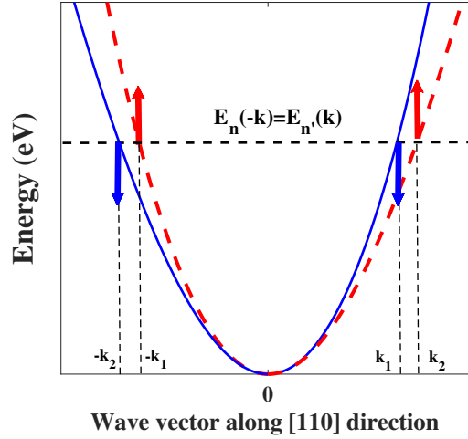
FIGURE 2.18: Energies of \uparrow spin (red line) and \downarrow spin (blue line) states generated by Dresselhaus terms.
