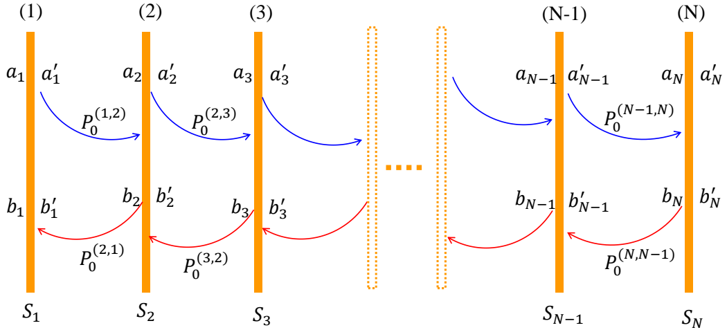
FIGURE C.3: Schematic of scattering process within a heterostructure with indications of wavefunction's amplitudes and interfacial scattering matrix S_i at each interface as well as the propagation between two interfaces of considering heterostructure.
