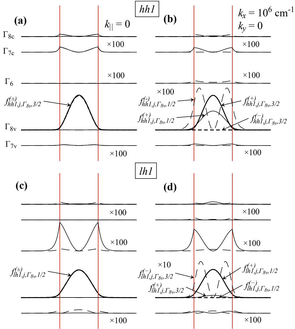
FIGURE 3.19: The envelope function |f_{n,j,N}^{(+)}|^2 (solid lines) and |f_{n,j,N}^{(-)}|^2 (dashed lines) for n = hh1(HH1) (a,b) and n = lh1(LH1) (c,d) in GaAs/Al_{0.35}Ga_{0.75}As 100 Å quantum well. Here, (+) and (-) are labeled for spin up and spin down and the calculations was done for k_{||} = [0 \ 0] (a,c) and k_{||} = [10^6 \text{ cm}^{-1} \ 0] (b,d) and for t_{l-h} = 0 for all. Taken from Ref. [249]
