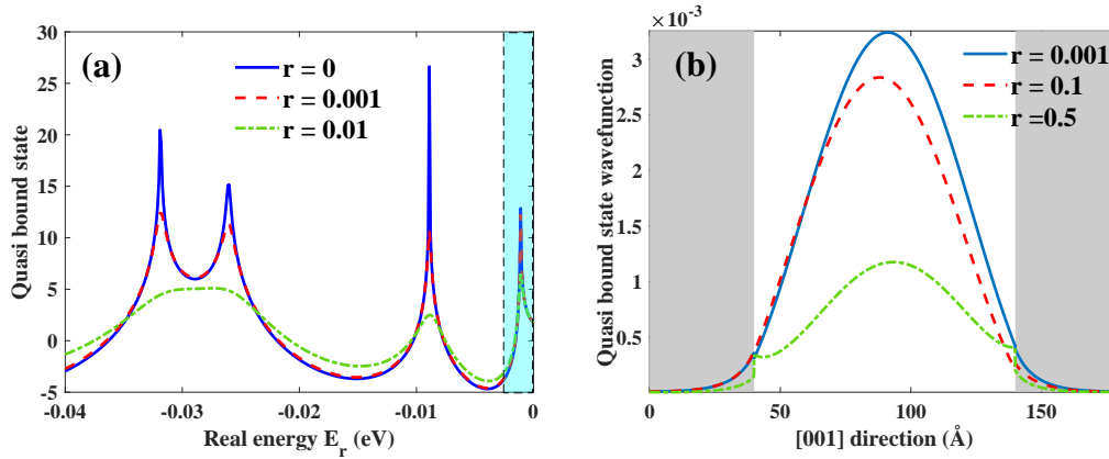
FIGURE 3.15: (a) The \text{Det}[S(0, N)] as function of energy with different ratios r = \frac{E_r}{E_i} where E_r and E_i are the real and imaginary part of generalized energy E , respectively, of an electron in (In,Ga)As/GaAs 10 nm quantum well structure. As the same as previous argument with bound state solutions, the first maximum of the curves here are not bound state solutions. (b) The quasi bound state wavefunction corresponding to the LH1 energy level in (In,Ga)As/GaAs 10 nm quantum well structure with different values of r .
