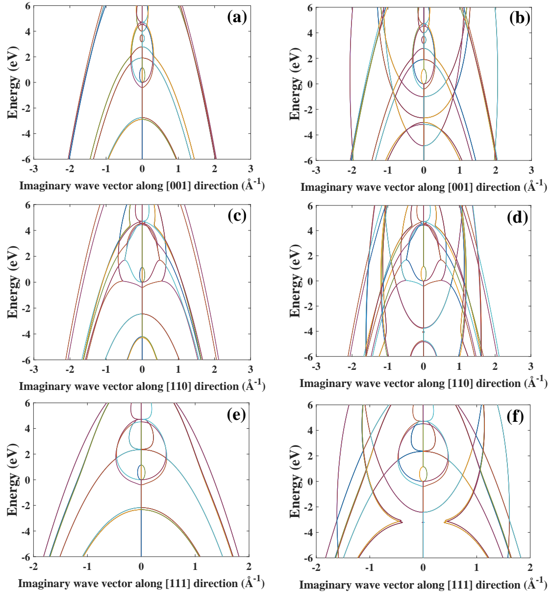
FIGURE A.5: Complex band structure of InGaAs via 30-band k \cdot p model before (a,c,e) and after (b,d,f) using our novel ghost-band method to remove spurious states.
