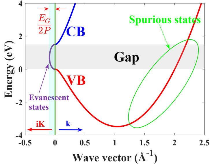
FIGURE 2.4: Spurious and Evanescent states in 2 band toy model. The spurious states cross the band gap at k = 2\hat{\text{A}}^{-1} and the evanescent states are located within K = [0, \frac{E_G}{2P}]
