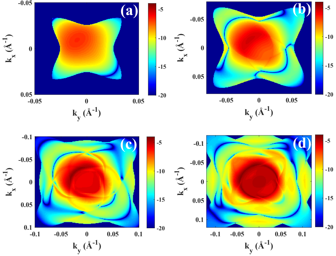
FIGURE 5.14: Transmission coefficient as function of k_{\parallel} wavevector for the maximum spin transfer torque configuration ( \theta = \pi/2 ) depicted in Fig. 5.11. The strong asymmetry in the transmission coefficient for the opposite incidence leads to a difference in the angular dependence of the torque upon two opposite incident direction depicted in Fig. 5.13(c-f).
