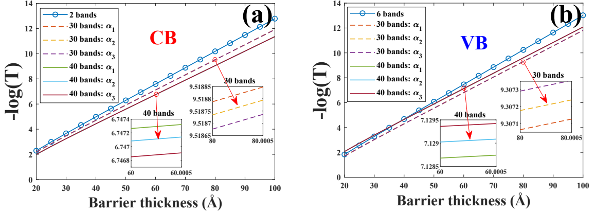
FIGURE 2.14: Transmission of carriers (in log. scale) vs. the barrier thickness d in fictitious GaAs/GaAs/GaAs trilayer barrier (a fictitious barrier height has been added in the central GaAs of -0.2\text{eV} ) calculated in the CB (Fig. (a)) and VB (Fig. (b)) within an extended 30- and 40- band k \cdot p framework for strictly normal incidence ( k_{\parallel} = 0 ). The slope of the transmission in log. scale vs d is related to the tunneling effective mass which remains robust under ghost-spurious coupling strength \alpha : \{\alpha_1 = 1\text{eV} \cdot \text{\AA}^{-2}; \alpha_2 = 1.5\text{eV} \cdot \text{\AA}^{-2}; \alpha_3 = 2\text{eV} \cdot \text{\AA}^{-2}\} for 30-band k \cdot p model and \{\alpha_1 = 1.5\text{eV} \cdot \text{\AA}^{-2}; \alpha_2 = 1.6\text{eV} \cdot \text{\AA}^{-2}; \alpha_3 = 1.7\text{eV} \cdot \text{\AA}^{-2}\} for 40 band k \cdot p model.
