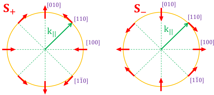
FIGURE 2.19: Quantized directions of \uparrow and \downarrow eigenstates as a function of the orientation of the in-plane electron wave vector k_{\parallel} . Taken from Ref.[54].
