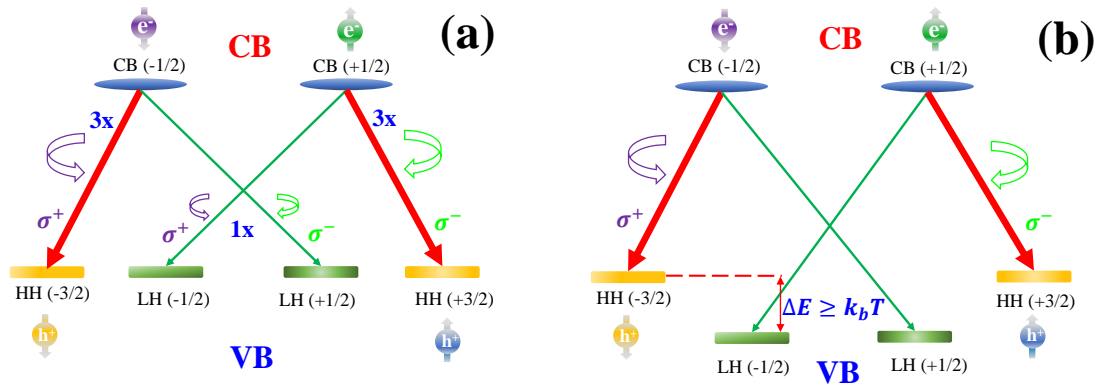
FIGURE 1.17: Optical selection rules for dipole radiation: (a) In the case of a bulk active medium, the HH-band and LH-band are degenerated and (b) The electron \rightarrow hole recombination in a quantum well structure, the epitaxial strain and quantum confinement lift the degeneracy between the HH-band and LH-band.
