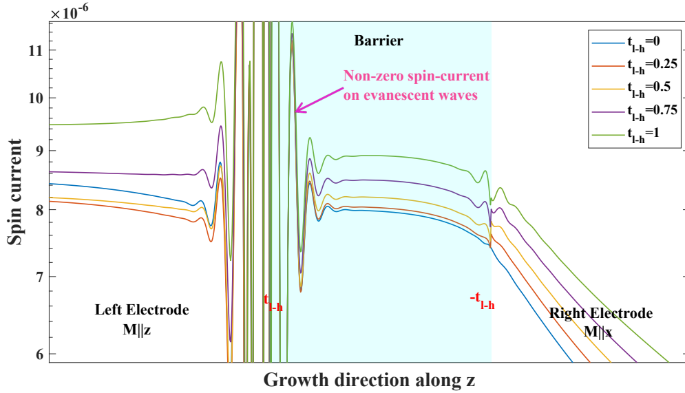
FIGURE 5.6: Profiles of the z -component of the spin current within (Ga,Mn)As/GaAs/(Ga,Mn)As junctions. The magnetization of the thick layer to the left is along z , whereas the one to the right is transverse that is along x for the calculation of the STT. The calculations have been performed with the energy of holes \epsilon = -0.03eV from the middle of the (Ga,Mn)As band. Here, the necessary heavy hole - light hole mixing parameter t_{l-h} varies from 0 to 1. This coefficient is set naturally positive and negative at the respective right and left interface of the barrier due to the specific D_{2d} symmetry of the junction of a symmetric profile.
