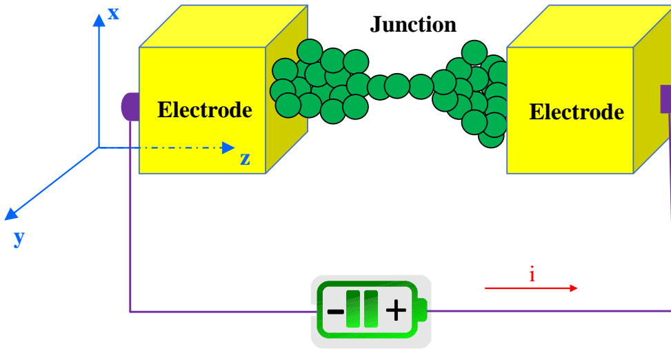
FIGURE 3.6: Scheme of a closed system, electron source plus electrode-junction-electrode structure. The electrodes are assumed to confine electrons in the x - y direction.
