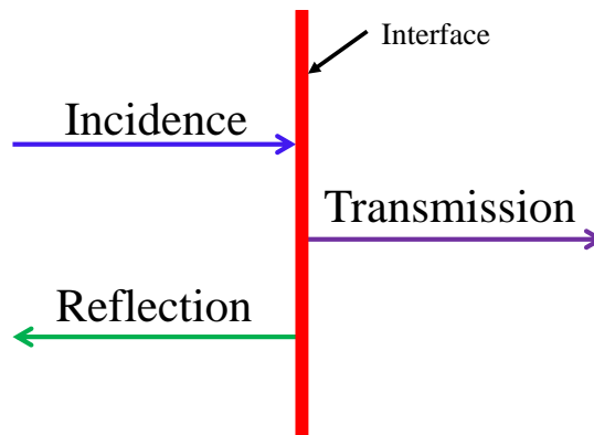
FIGURE 3.5: Scheme of continuity of wave current at the interface of heterostructure.
