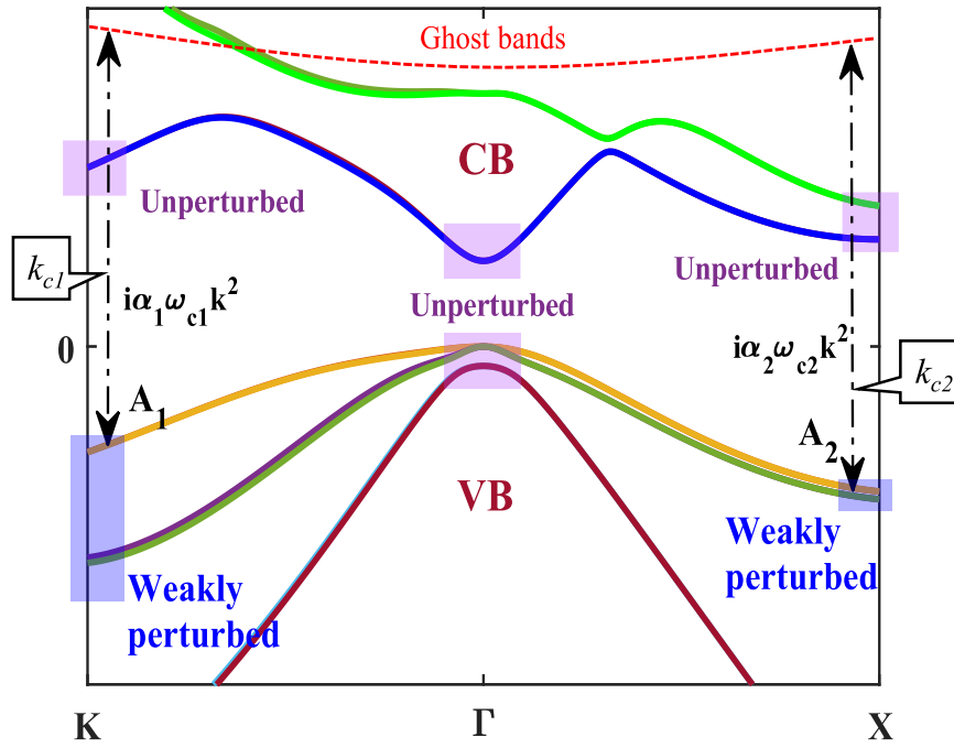
FIGURE 2.9: Schematic of band structure of Hamiltonian in Fig 2.8, the ghost bands are included at higher energy than the first conduction band for perturbation minimization. At the A_{(1,2)} point, the ghost bands only couple with the VBs to ensure that the band structure at \Gamma point is not affected. At the A_{(1,2)} points, the CBs is almost unaffected and VBs are weakly affected.
