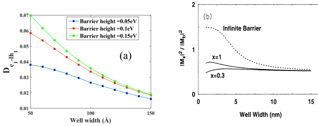
FIGURE 6.13: Dipolar matrix elements as function of quantum well width electron-light hole transitions with polarization along [100] direction calculated by our 30×30 band k.p code (a) compares with result of Kajikawa (b) taken from ref.[221].
