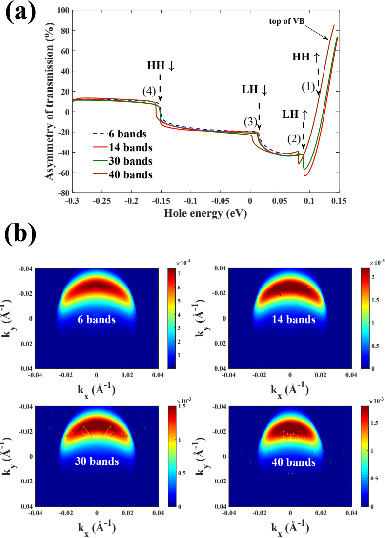
FIGURE 5.22: (a) Asymmetry coefficient \mathcal{A} vs. reduced energy calculated in the VB of (Ga,Mn)As/GaAs/(Ga,Mn)As 3 nm thick tunnel junction with AP magnetizations for k = 0.05 \text{ nm}^{-1} and (b) the transmission coefficient as function of in-plane wave vector k_{\parallel} = (k_x, k_y) . Carriers with plus k_y in-plane wavevector component are more easily transmitted than those carrying minus k_y . These calculations were done for VB within the different \mathbf{k} \cdot \mathbf{p} framework: 6-, 14-, 30-, and 40- band model and a good agreement among them showing that the numerical code is robust. The exchange strength is 0.3 eV and the total kinetic energy E = 0.23 \text{ eV} , the barrier thickness being 3 nm.
