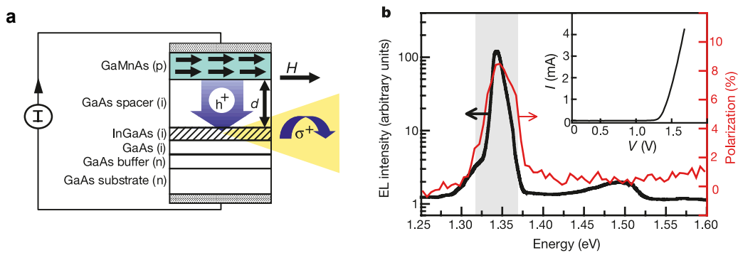
FIGURE 1.15: (a) Electrical spin injection in an epitaxially grown ferromagnetic semiconductor heterostructure, based on GaAs. Spontaneous magnetization develops below the Curie temperature T_C in the ferromagnetic p-type semiconductor (Ga,Mn)As, depicted by the black arrows in the green layer. Under forward bias, spin-polarized holes from (Ga,Mn)As and unpolarized electrons from the n-type GaAs substrate are injected into the (In,Ga)As quantum well (QW, hatched region), through a spacer layer with thickness d , producing polarized EL. (b) Total electro-luminescence (EL) intensity of the device ( d = 20 nm) under forward bias at temperature T = 6 K and magnetic field H = 1 Oe is shown (black curve) with its corresponding polarization (red curve). Current I = 1.43 mA. Note that the polarization is largest at the QW ground state ( E = 1.34 eV). The EL and polarization are plotted on semi-log and linear scales, respectively. Inset, a current-voltage plot characteristic of a 20-nm spacer layer device. Taken from [129].
