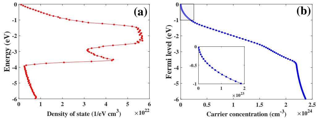
FIGURE 2.25: The density of states (DOS) and Fermi level vs carrier concentration calculated for GaAs in framework of 30-band k \cdot p method.
