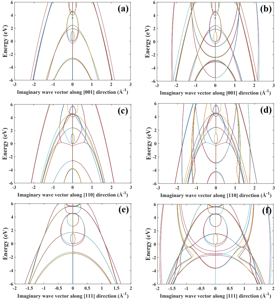
FIGURE 2.17: Evanescent band structure of GaAs within native 30-band (a), (c), (e) and 38-band (8 ghost-band) (b), (d) and (f) calculated for three characteristic direction [001], [110] and [111]. In comparison to native 30-band, there are additional evanescent bands at far away from \Gamma point in the calculation with 38-band method. As mentioned in Ref. [164], these additional bands are the consequences of converting the spurious solutions with large real k to the spurious solution with large imaginary k which, as commented earlier, are harmless in the calculations. The imaginary k landscape remains unchanged close to the \Gamma point.
