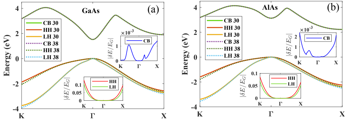
FIGURE 2.10: The band structure along K\Gamma X valleys calculated by native 30 bands \mathbf{k}\cdot\mathbf{p} Hamiltonian, E_{30} , (solid lines) and after using ghost-band method, E_{38} , (dot lines) for GaAs (a) and AlAs (b) materials. The inset figures show the relative errors \delta E/E_G induced by ghost bands for the first conduction band, heavy and light holes band respectively ( \delta E = E_{38} - E_{30} and E_G is energy gap).
