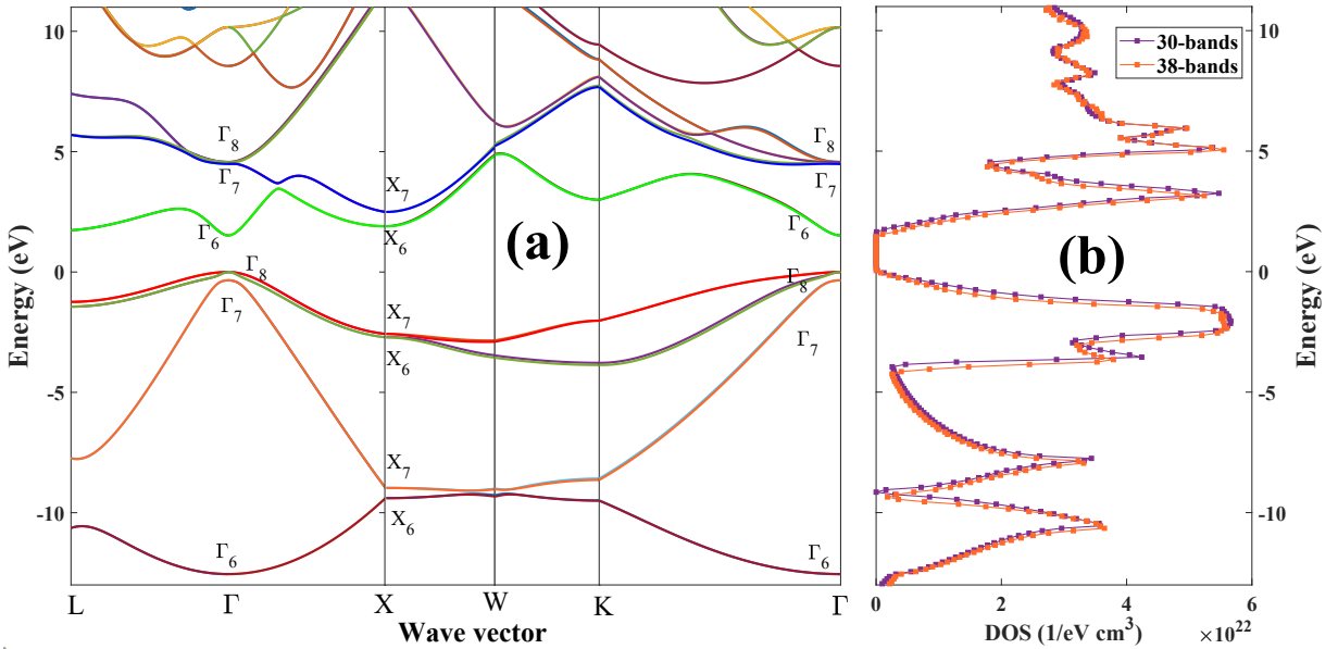
FIGURE 2.1: (a) Band structure of GaAs (belongs to T_d group) calculated in framework of 30-band k.p model. The energy at the top of the filled valance bands has been taken to be zero. (b) Density of states (DOS) calculated with native 30-band k.p method and 38-band (30 bands + 8 ghost-bands detailed hereafter) which shows that the ghost-band weakly affects the DOS which is in good agreement with the experimental results and numerical results, calculated by Density Functional Theory in Ref.[46].
