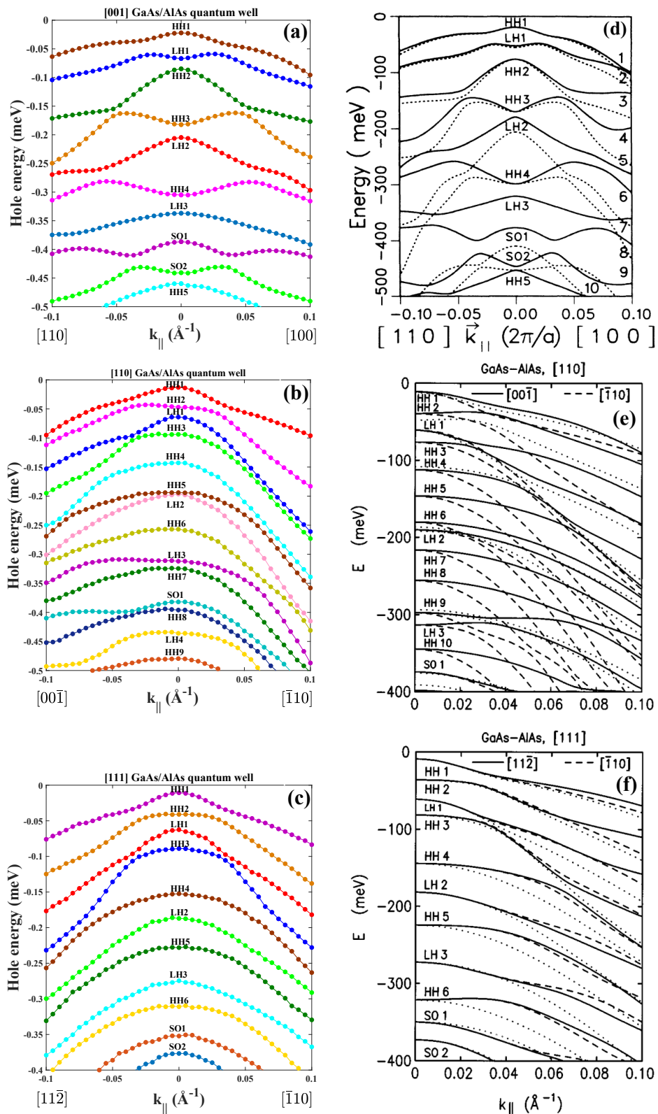
FIGURE 2.13: Hole's dispersion in AlAs/GaAs 6nm quantum well calculated by a 30-band k \cdot p model using ghost-band method for the three respective growth directions [001] [110] and [111], Fig. (a), (b) and (c) respectively, in comparison with the result calculated by Eppenga et al. [202] with 6-band k \cdot p model, Fig. (d), and Winkler et al. [203], Fig. (e) and (f).
