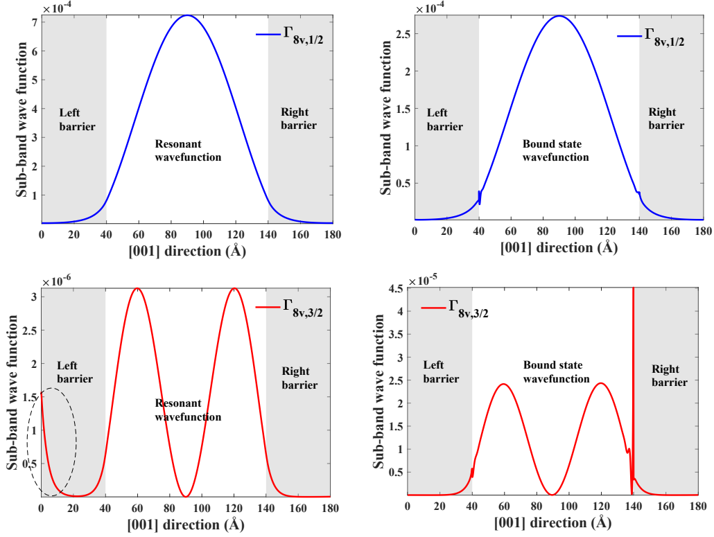
FIGURE 3.13: Scattering wavefunction (left panel) and bound state wavefunction (right panel) correspond to LH1 energy level in (In,Ga)As/GaAs 10 nm quantum well. The blue curves are the \Gamma_{8v,1/2} subband wave function and the red curves are the \Gamma_{8v,3/2} subband wave function.
