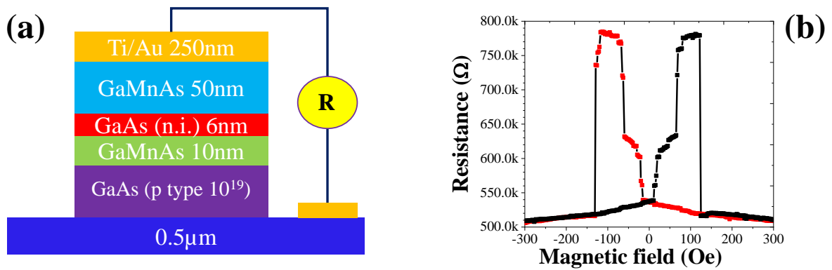
FIGURE 5.8: (a) Structure used for the investigation of the Tunneling Magnetoresistance. (b) Tunneling Magnetoresistance (TMR) obtained on the structure shown in this figure a at temperature of 12 K and at bias of 20 mV. The (Ga,Mn)As layers where made different to promote a different reversal of the two (Ga,Mn)As layers and a clear antiparallel (AP) plateau.
