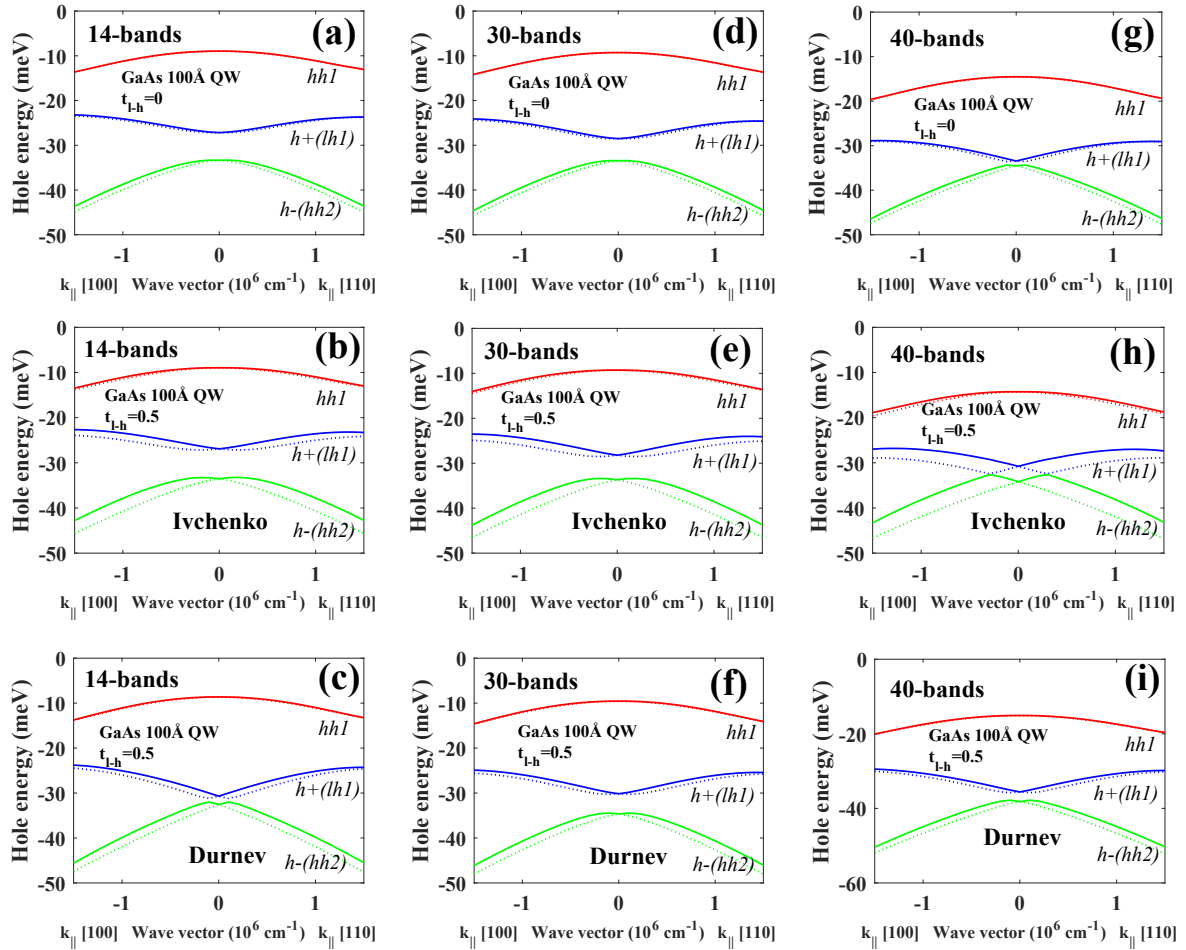
FIGURE 3.24: Valence subbands dispersion in GaAs/AlAs 10nm QW calculated with different k, p platforms (indicated in the figures), for two values of the mixing term t_{l-h} = 0 and t_{l-h} = 0.5 with two sets of boundary conditions proposed by Ivchenko et al. [30] and Durnev et al. [31].
