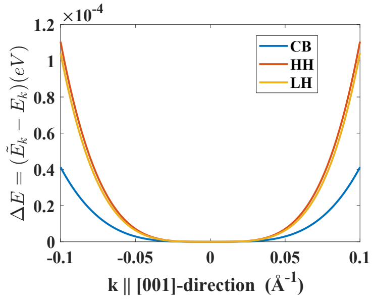
FIGURE B.7: Numerical calculations of errors for CB, HH and LH subband, calculated via 30-band k \cdot p model.
