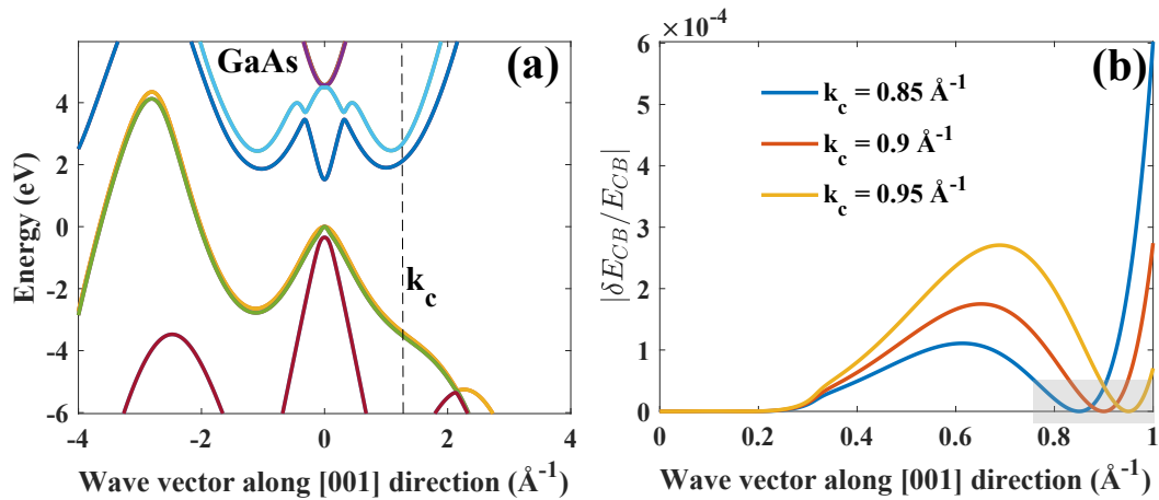
FIGURE 2.11: (a) The band structure of GaAs along typical [001]-direction by using ghost-band method with the couplings at +k_c only. (b) the errors induced by the ghost bands on the dispersion of first conduction band with different coupling points k_c .
