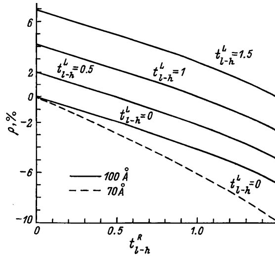
FIGURE 6.18: The anisotropy of optical matrix transitions elements as a function of the mixing term parameter at right interface of quantum well originating from HH and LH with different values of mixing term parameter at left interface, taken from Ref.[409].
