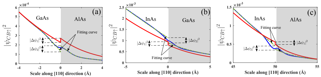
FIGURE 3.4: (a) The zoom in of the wave function in Fig 3.3a close to the interface between GaAs and AlAs showing the jump in both analytical formula \Delta\psi_1 and numerical calculations \Delta\psi_2 with 30 bands \mathbf{k}, \mathbf{p} Hamiltonian. The same calculations have been performed for wave function at InAs/GaAs interface (b) and InAs/AlAs interface (c).
