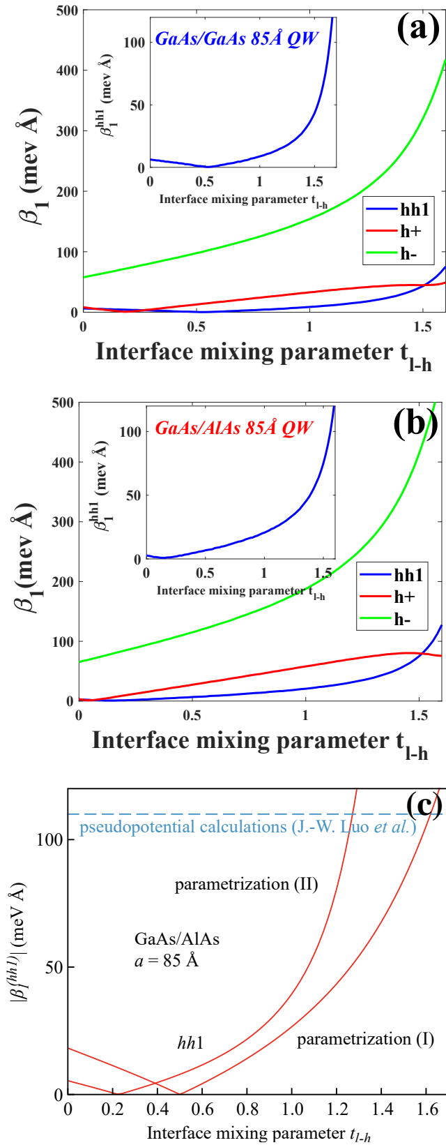
FIGURE 3.26: The results of calculations for valence subbands spin splitting as a function of the interface mixing strength for GaAs/GaAs and GaAs/AlAs 85 Å quantum well (a,b) respectively. The insets in (a,b) present heavy-hole (HH1) spin splitting for comparison with the result from Durnev et al. in figure (c) [31].
