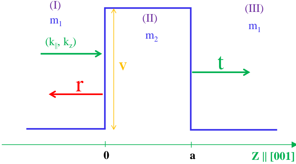
FIGURE 2.20: Sketch of a three-dimensional model of electron tunneling. Transmission of electrons with the wave vector \mathbf{k} = (k_{\parallel}, k_z) through the potential barrier V of width a grown along z . Taken from Ref.[54]
