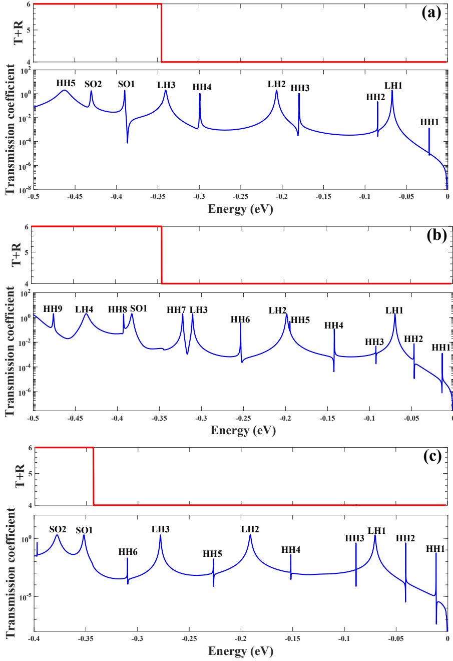
FIGURE 3.9: Calculation of transmission coefficient (blue) and sum of transmission and reflection coefficient (red) for resonant tunneling through GaAs/AlAs quantum wells with growth directions along three characteristic directions: [001], [110] and [111] (figures (a), (b) and (c) respectively) with normal incidence k_{\parallel} = 0 via 30-band k.p method.
