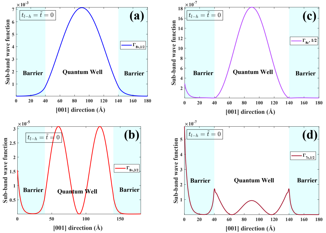
FIGURE 3.21: The envelope functions in a GaAs/AlAs quantum well calculated in the framework of 30-band k, p theory with standard matching condition ( t_{l-h} = \tilde{t} = 0 ) and normal incidence k_{||} = 0 for corresponding LH_1 (h+) energy level. The calculated wavefunctions are the scattered waves propagating from left to right.
