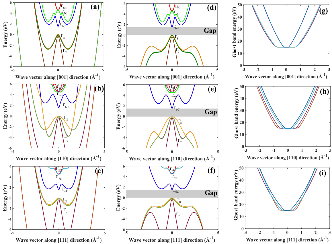
FIGURE 2.12: Electronic band structures of GaAs near the band gap along three characteristic directions with native 30 band k \cdot p method (a,b,c) and 30 bands + 8 ghost bands method (d,e,f). Figure (g,h) and (i) are the 8-ghost bands corresponding to three characteristic directions. The effective mass and band dispersion along the different crystal graphic directions are leaved unchanged.
