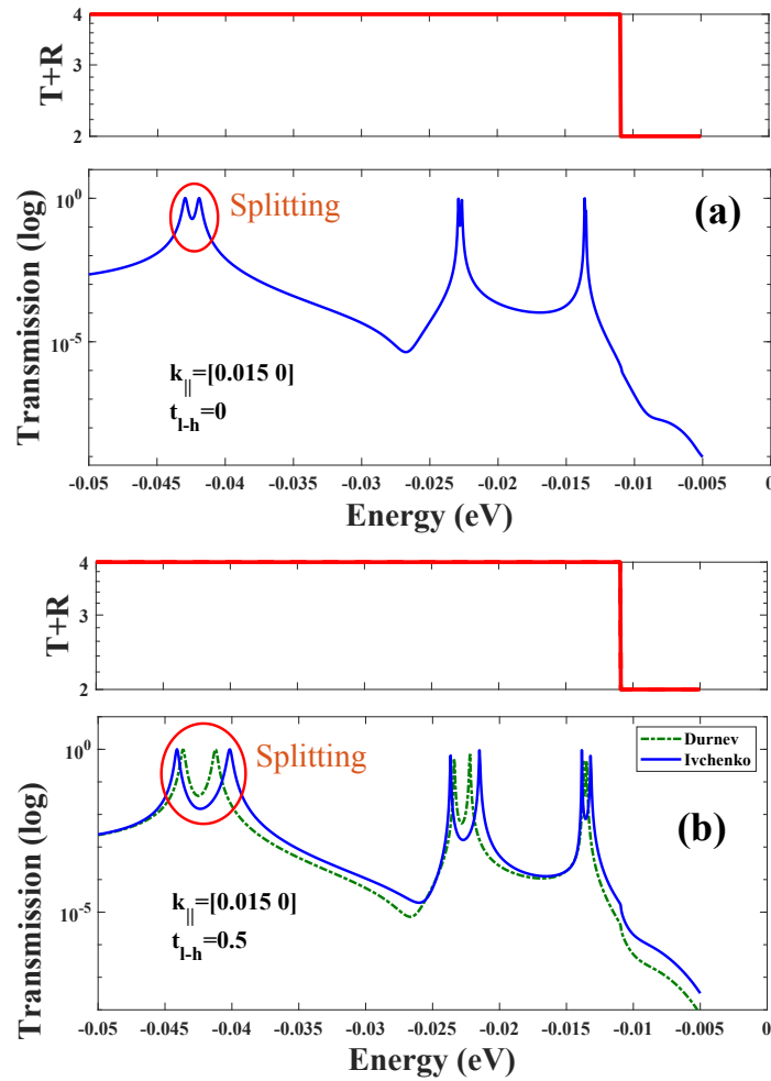
FIGURE 3.17: Spin splitting in resonant tunneling through GaAs/GaAs quantum well structures [31] where the mixing between the heavy hole and light hole in figure (b) ( t_{lh} = 0.5 ) allows splitting to become larger than the splitting caused only by Dresselhaus term in figure (a) ( t_{lh} = 0 ). In figure (b) are the calculations with two boundary conditions proposed by Durnev [31] and Ivchenko [30] which were adapted to 30-band \mathbf{k}, \mathbf{p} model. The sum of transmission and reflection coefficients (red curve) for both two adapting boundary condition in 30-band \mathbf{k}, \mathbf{p} model are almost constantly and are equal to number of bands included in tunneling. This mean that the wave current is conserved.
