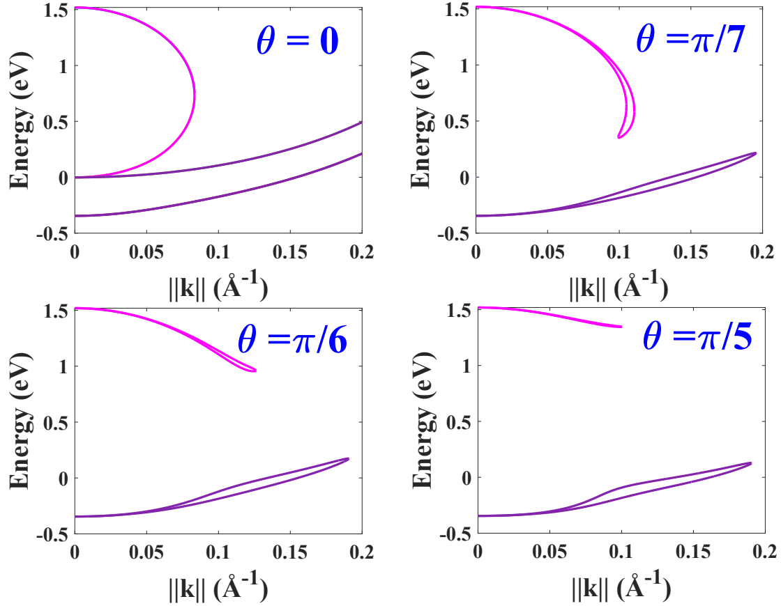
FIGURE 2.16: Plot of the real energy line inside the gap for \mathbf{k} = [\xi, 0, iK] = [\tan\theta, 0, i]k where \xi and K are real and positive and \theta = \frac{\xi}{K} . The calculations were performed using our 30 \times 30 \mathbf{k} \cdot \mathbf{p} model. The presence of the spin-orbit coupling and the lack of an inversion center lead to a splitting in the complex band structure when \theta \neq 0 . These results are in good agreement with results of Richard et al. in Ref.[204].
