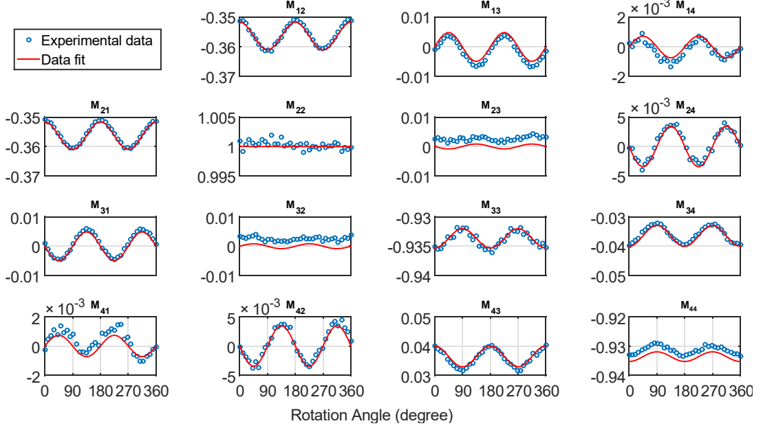
FIGURE 6.6: The measured Mueller matrix elements as a function of the in-plane azimuth rotation angle ranging from 0 to 360 degree for E = 2.2 eV and for the angle of incidence \theta = 40^\circ . Taken from [397].
