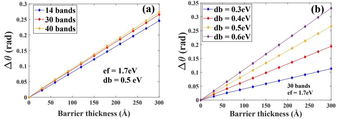
FIGURE 4.7: Spin rotation experienced by the outgoing electron transmitted through the [110] GaAs barrier for different barrier thickness up to 300 Å. (a) Calculated with different \mathbf{k}\cdot\mathbf{p} platforms for db = 0.5\text{ eV} and incident energy ef = 1.7\text{ eV} above top of valence band. (b) Calculated with 30 bands \mathbf{k}\cdot\mathbf{p} method with different values of db . The rotation of the spin is proportional to the barrier thickness.
