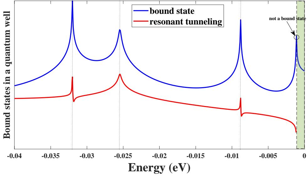
FIGURE 3.12: Resonant tunneling (red curve) and \text{Det}[S(0, N)] (blue curve) in arbitrary units as the functions of energy of an electron in (In,Ga)As/GaAs 10 nm quantum well structure. The positions of the maximum points corresponding to the bound state solutions of blue curve are exactly the same as the resonant peaks of red curve excepts the first maxima (of blue curve) which is not a bound state solution, but a tuning point of current from pure evanescent to propagating states.
