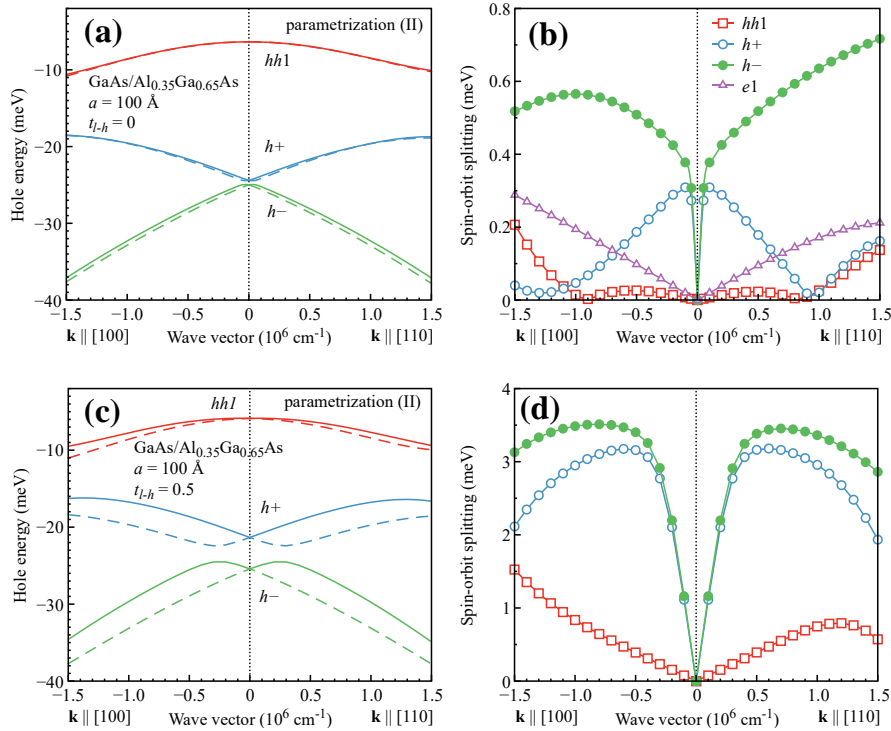
FIGURE 3.23: Dispersion (a, c) and spin splitting (b, d) of valence subbands for GaAs/Al 0.35 Ga 0.65 As 10nm QW. The calculations are done for two cases: mixing parameter t_{l-h} = 0 [panels (a) and (b)] and t_{l-h} = 0.5 [panels (c) and (d)]. The spin splitting of conduction subband e1 is presented in (b) for comparison. Taken from Ref.[31].
