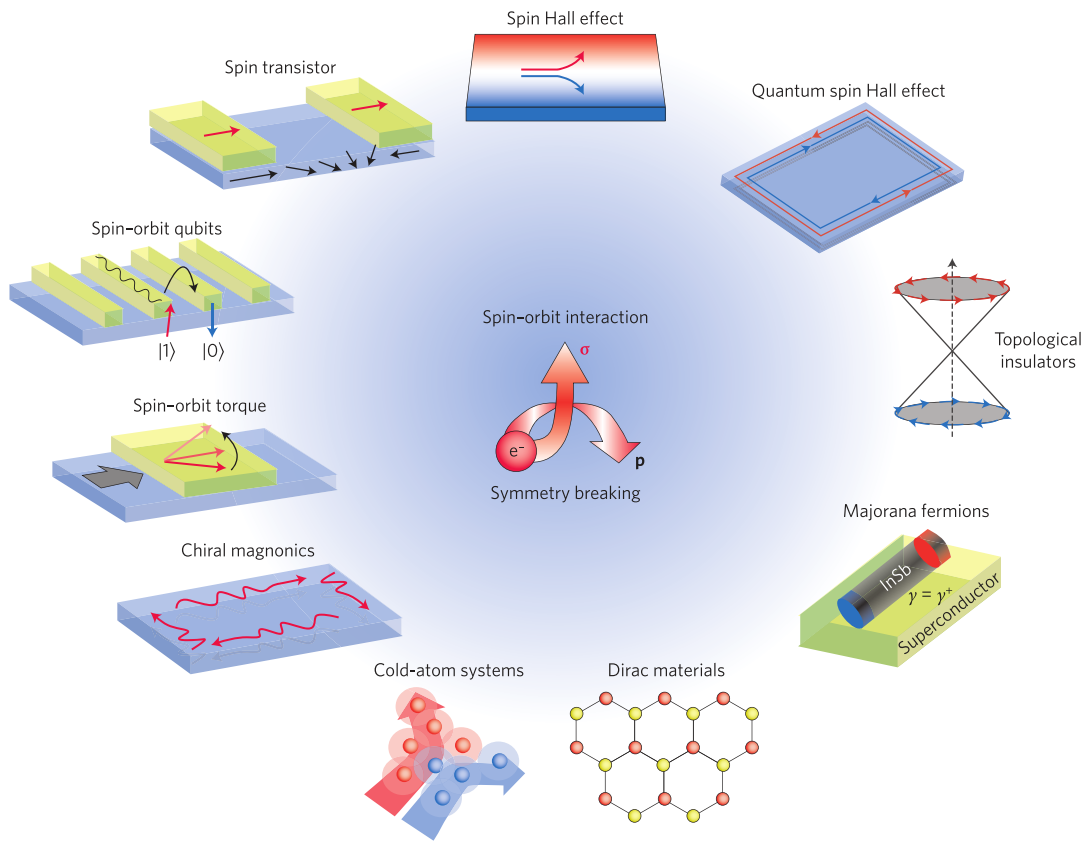
FIGURE 2: The tremendously active field of spinorbitronics: the various sub-fields in which magnetization and spin directions can be manipulated electrically via the spin orbit coupling in systems broken inversion symmetry which reveals novel states of matter. Taken from [10].
