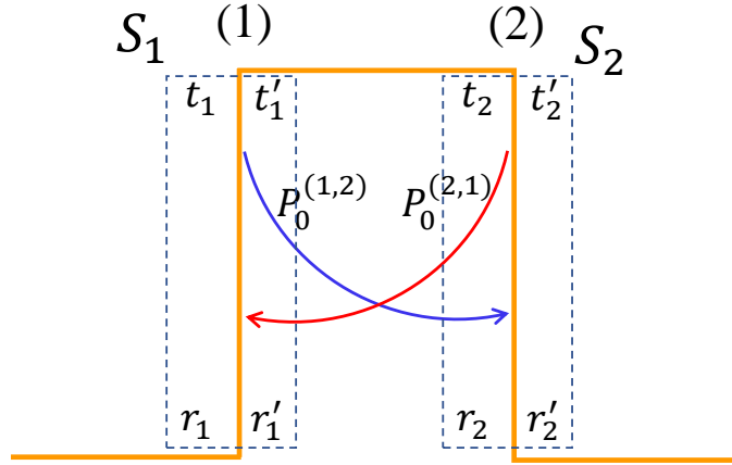
FIGURE C.4: The elements to build up a global scattering matrix S_G for a simple barrier structure.
