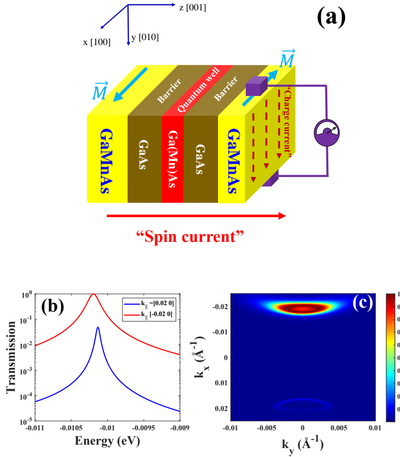
FIGURE 5.24: (a) Schematic of Anomalous Tunnel Hall effect in a GaAs quantum well with 2 nm barrier thickness and 10nm quantum well width, 0.5 eV barrier height and \uparrow\downarrow magnetization configuration; (b): transmission as function of energy for anti-parallel configuration with opposite incident wave vectors k_{||} around the second peak of quantum well dispersion, and (c) two dimensional map of transmission vs. k_{||} calculated for hole's energy which corresponds to the energy position of the peak in (b).
