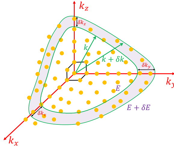
FIGURE 2.24: Scheme of construction in k -space to calculate the density of states in three dimensions. The shells have radii k and k + \delta k corresponding to energies E and E + \delta E .
