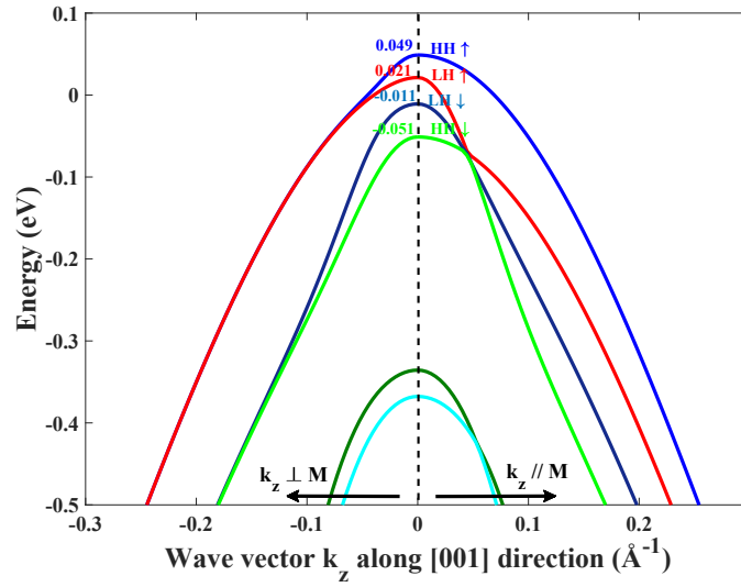
FIGURE 2.23: Valence band structure of (Ga,Mn)As along [001] direction via 30 – band \mathbf{k}\cdot\mathbf{p} model with exchange energy equal 0.05 eV for two cases of magnetization direction: perpendicular and parallel to the growth direction.
