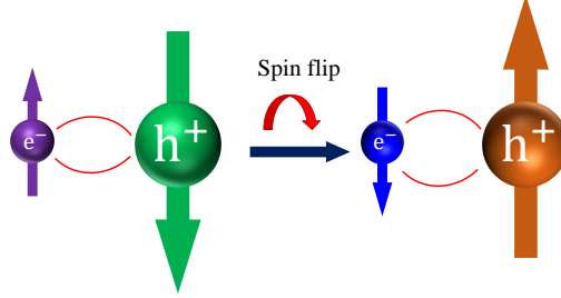
FIGURE 1.21: Schematic of Bir-Aronov-Pikus mechanism: Electron-Hole exchange interaction leading to fast spin relaxation through Elliot-Yafet mechanism
