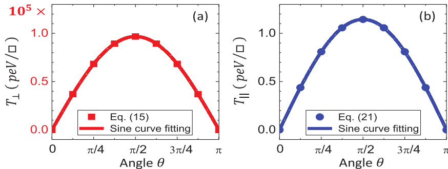
FIGURE 5.12: The angular dependence of (a) T_{\perp} and (b) T_{\parallel} for SFMJ with bias of 0.2 V. The solid points are analytical calculation and the solid lines are the sine curve fit, taken from Ref.[309].
