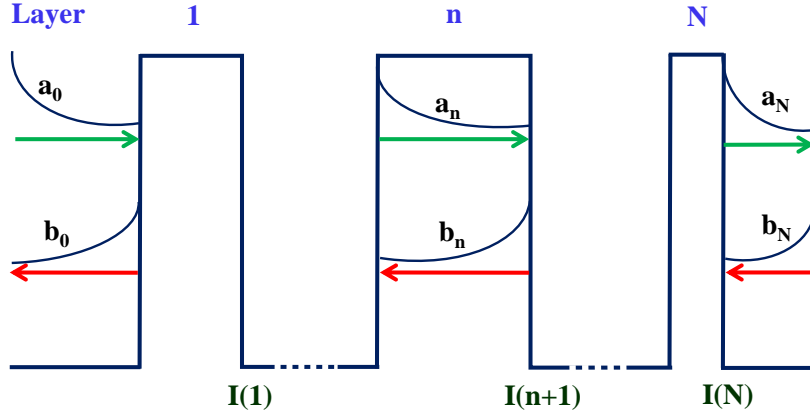
FIGURE C.2: Schematic diagram of electron tunneling through heterostructure.
