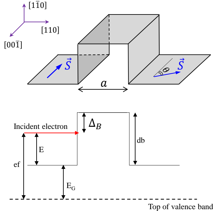
FIGURE 4.4: Schematic of spin rotation through the [110] barrier structure and the potential profile of the structure.
