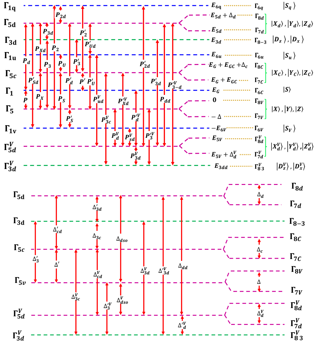
FIGURE A.10: Schematic representation of the 40-band \mathbf{k}\cdot\mathbf{p} model representing involved bands, relevant parameters, momentum matrix elements and spin-orbit couplings.
