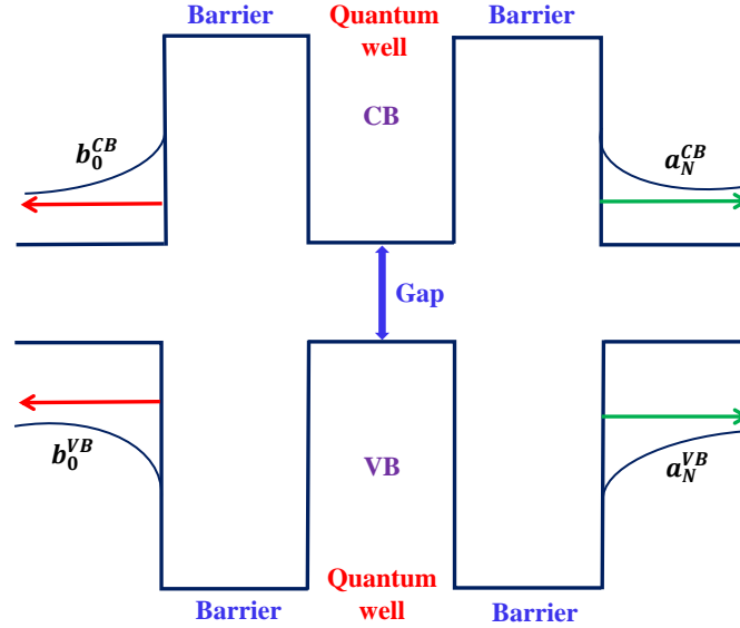
FIGURE 3.11: Scheme of bound state wavefunction in quantum well. Outside of quantum well, the wave function decays exponentially which means that \mathbf{a}_0 = \mathbf{b}_N = [0] .
