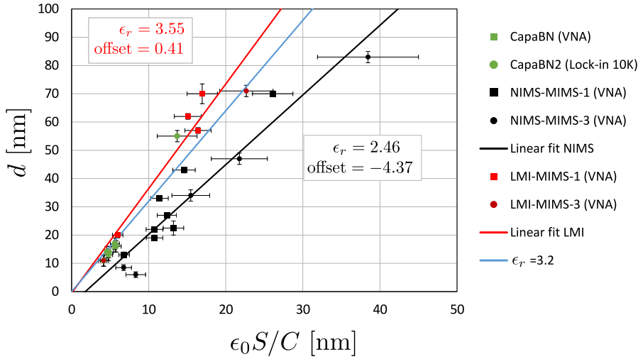
Figure 6.9 – Determining the out-of-plane permittivity of hBN from capacitance measurements.
