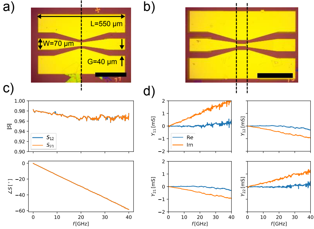
Figure 2.17 – De-embedding . a) Microscope image of a thru-line. b) Microscope image of a dummy structure. In both cases the scale bar corresponds to 200 \mu\text{m} . The black dashed lines indicate the calibration plane after de-embedding the propagation in the thru-line. c) Transmission parameters ( S_{12} and S_{21} , magnitude and phase) of a thru-line. d) Complex admittance matrix of a dummy structure.
