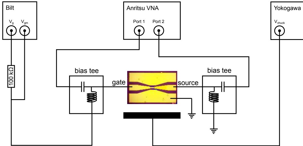
Figure 2.15 – Wiring scheme for the VNA characterization of plasma resonance capacitors.
