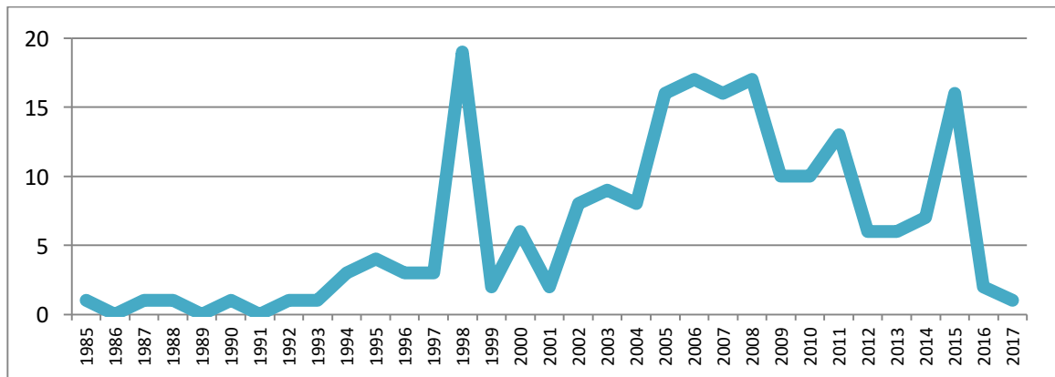
Figure 3.4 A-level publications by year: bibliographic entries with at least 3-keyword proximity to subject.
