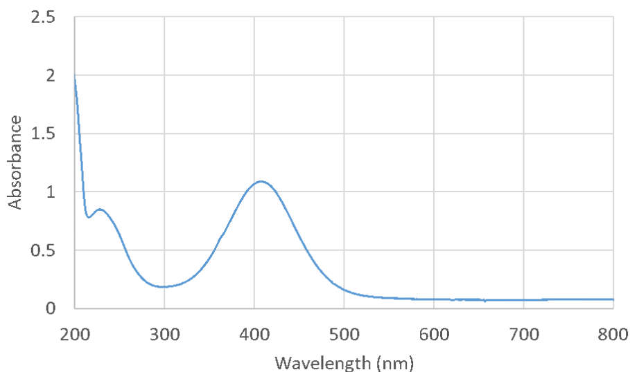
Figure III-1. Absorption spectrum of a 1.64 \times 10^{-4} M pNTP aqueous solution. Optical path: 1 cm
