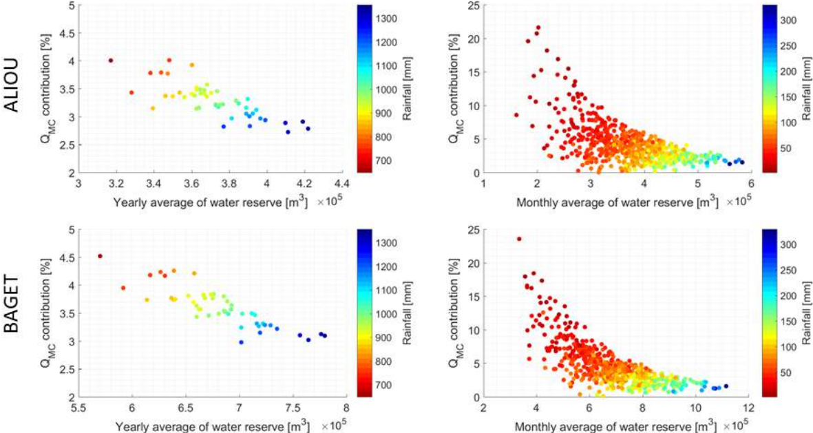
Figure 6 – Contribution of the exchange between reservoir M and reservoir C to the total discharge on the annual scale (left) and the monthly scale (right).
