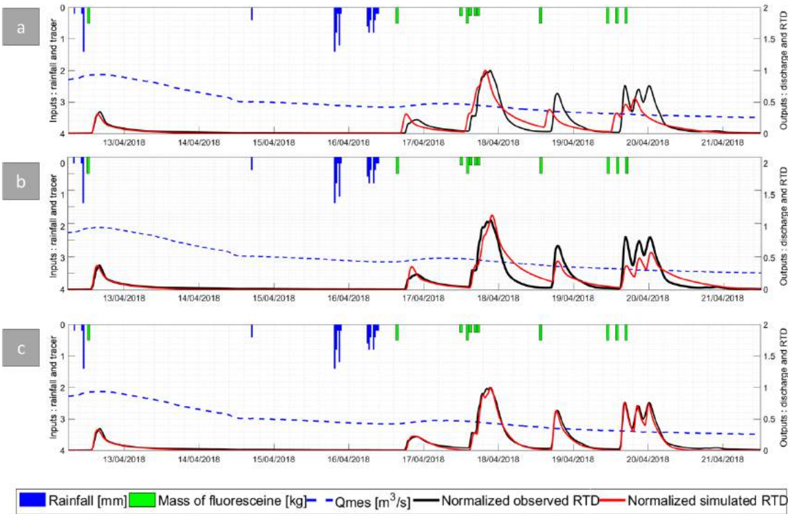
Fig. 5 – Experimental RTD and simulated RTD curves — a hypothesis : the system is linear and transit time is independent of discharge rate, b hypothesis : the system is linear and transit time is dependent on discharge rate and c hypothesis : the system is non-linear, and both transit time and mixing coefficient are dependent on the discharge rate
