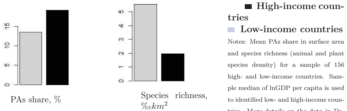
Figure 4.1: Mean PAs share in surface area and species richness
