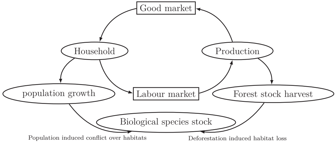
Figure 3.1: Synopsis of the population-forest-biodiversity model
