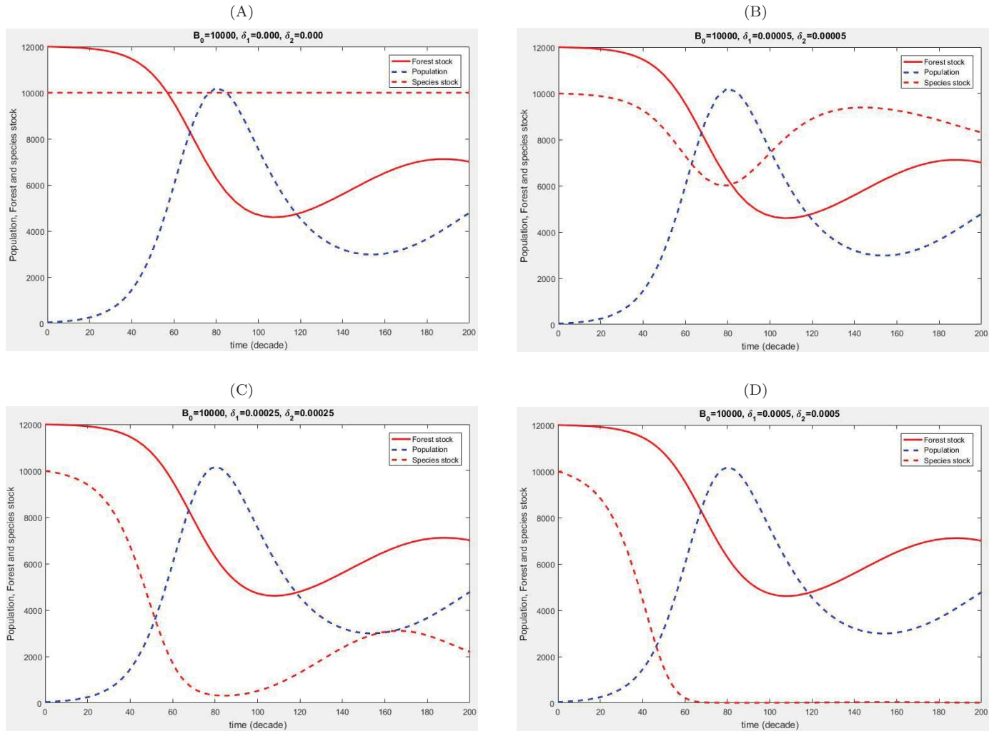
Figure 3.3: Scenario 1: Species loss in the Easter-Island framework
