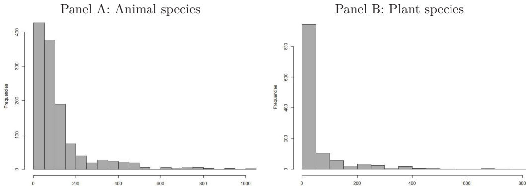
Figure 2.1: Histogram of counts on threatened animal and plant species
