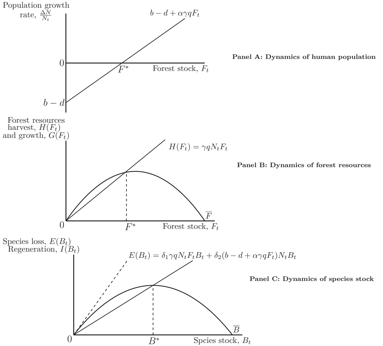
Figure 3.2: Illustration of the dynamics of population-forest-species stock
