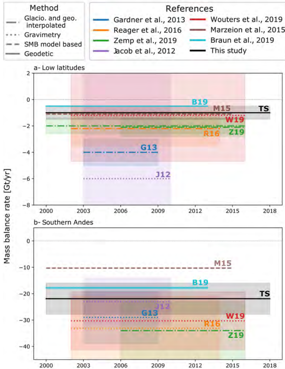
Figure 3.3: Glacier mass change rates estimates for (a) Low Latitude (10°N – 25°S, 99% Andean glaciers) and (b) Southern Andes (25°S – 56°S) regions from multiple methodologies. The results from this study do not account for subaqueous mass loss. In (a) the estimates from 3.8 and This study correspond to Andean Low latitude glaciers only.
