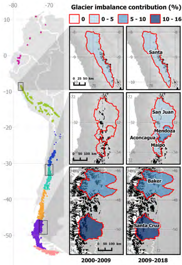
Figure 3.4: Seven main river basins used in the hydrological analyses: Santa basin (Peru); Aconcagua, Maipo and Baker basin (Chile); San Juan, Mendoza and Santa Cruz basins (Argentina). Color scale represents the relative decadal glacier imbalance contribution to river runoff for each decade.
