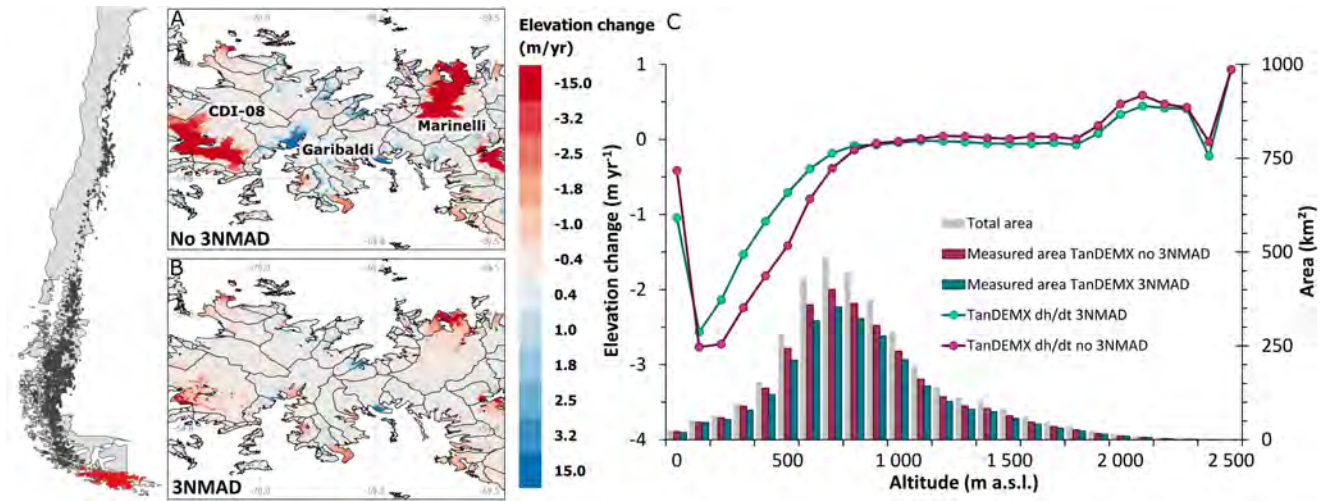
Figure 3.21: Influence of the 3NMAD regional filter on Tierra del Fuego. (A) TanDEM-X dh/dt map for Marinelli, Garibaldi and CDI-08 glaciers in Cordillera Darwin, NO-3NMAD filter. (B) TanDEM-X dh/dt map for Marinelli, Garibaldi and CDI-08 glaciers in Cordillera Darwin, using 3NMAD filter. (C) TanDEM-X hypsometric dh/dt (average of a 100 m elevation band) for the entire Tierra del Fuego region, for NO-3NMAD filter (purple) and 3NMAD filter (blue).
