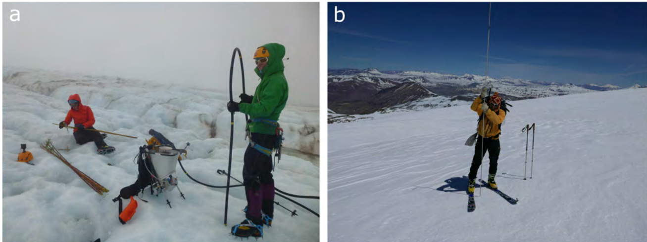
Figure 1.10: Examples of glaciological measurements performed during this PhD work on the Argentinian Andes as a collaboration with the Argentinian glaciology institute (IANIGLA). (a) Installation of 6 m bamboo stakes at the ablation area of Alerce glacier (Monte Tronador, North Patagonia) in spring using a water vapour perforator. (b) Winter snow probing at the accumulation area of Aguas Negras glacier (Desert Andes).
