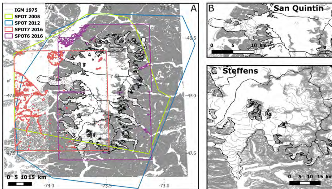
Figure 4.1: Spatial footprints of NPI data sets. (A) IGM 25 m contour lines over the NPI (west of -74^{\circ} W contours are every 50 m). Note that above ice the coverage is not complete with many data missing in the accumulation zones of the biggest glaciers and no data on San Rafael glacier tongue. Coloured polygons correspond to DEM footprints: SPOT5 2005 (green), SPOT5 2012 (blue), SPOT7 2016 (red) and SPOT6 2016 (purple). Selected subsets show the IGM contour lines over (B) San Quintin glacier and (C) Steffens glacier. IGM contour lines are rasterized to fit the 40 m SPOT DEM resolution, valid pixels correspond to the 7 % of the total icefield area.
