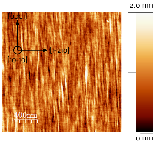
Figure 0.63.: 2 \times 2 \mu\text{m}^2 AFM image of an m-plane ZnO/(Zn, Mg)O MQW. The RMS is 3 Å. The lateral undulation period is around 10 nm.
