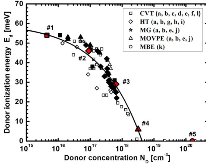
Figure 0.62.: Donor ionisation energy E_d as a function of the donor concentration N_d in ZnO thin films grown by various growth methods (see figure legend). Samples #1, #2 and #3 are non-intentionally doped whereas samples #4 and #5 are doped with Al and Ga respectively. Reprinted from (Brochen et al., 2017), with the permission of AIP Publishing.
