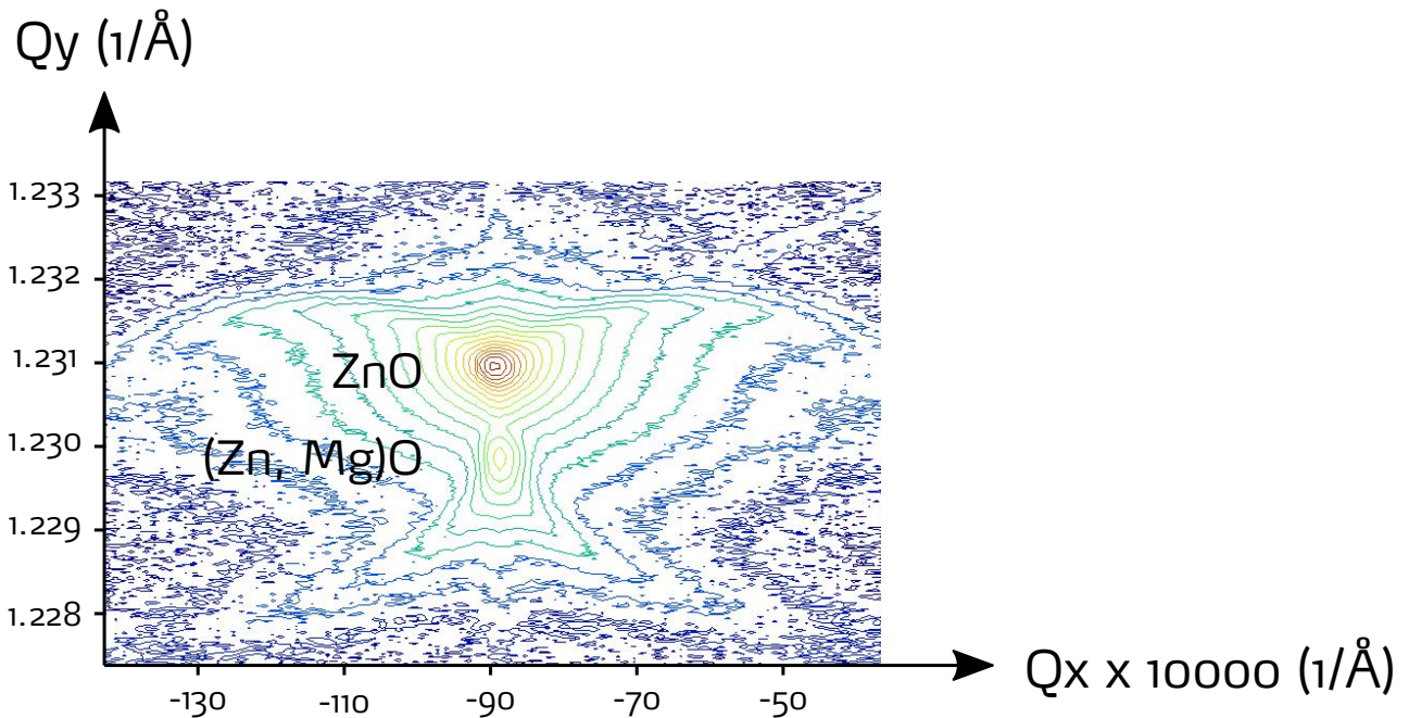
Figure 0.111.: RSM around the node (220), with \varphi = 0^\circ for a sample with cracks in oblique configuration.
