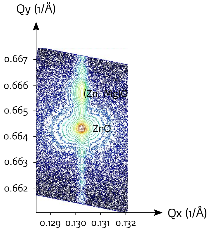
Figure 0.119.: RSM around the (103) node for \varphi = 0^\circ .
