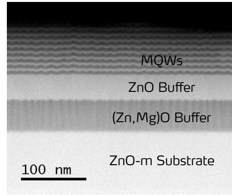
Figure 0.67.: STEM-HAADF image of a MQW sample in the [0001] zone axis (meaning that the c -axis is pointing out of the image).
