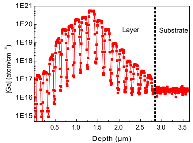
Figure 0.61.: SIMS profile of the Ga concentration.
