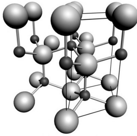
Figure 0.10.: Wurtzite structure of ZnO. Zn atoms are represented by large gray spheres and O atoms by small black ones. Reprinted from (Jagadish & Pearton, 2011), Copyright (2011), with permission from Elsevier.
