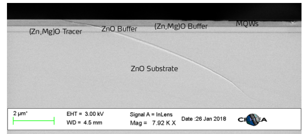
Figure 0.48.: SEM cross-section of a calibration layer.
