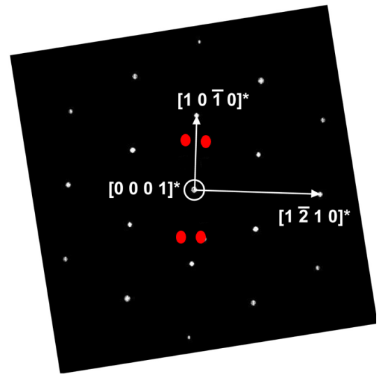
Figure 0.131.: Fourier transform of a TEM image in the [0001] zone axis. The hexagonal pattern comes from the crystal symmetry. Additional diffraction spots are highlighted in red.
