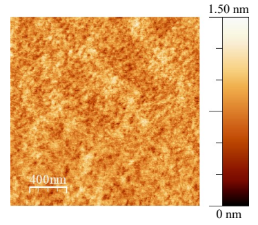
Figure 0.87.: AFM picture of sample C on a 4 \mu\text{m}^2 area. The RMS roughness is 0.15 \text{ nm} .
