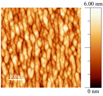
Figure 0.85.: AFM picture of sample A on a 4 \mu\text{m}^2 area. The RMS roughness is 0.88 \text{ nm} .
