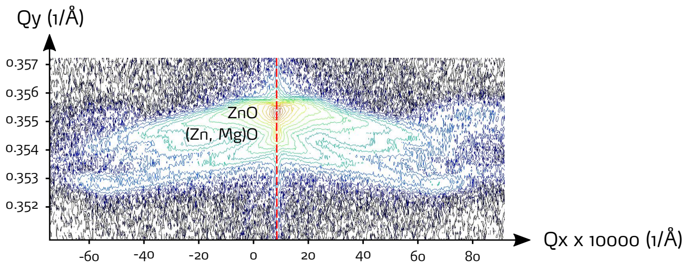
Figure 0.106.: RSM around the node (100), with \varphi = 0^\circ .
