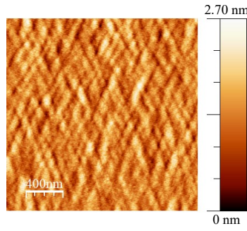
Figure 0.86.: AFM picture of sample B on a 4 \mu\text{m}^2 area. The RMS roughness is 0.35 \text{ nm} .
