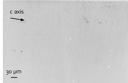
Figure 0.147.: SEM plane-view of a QCD sample with 30 periods. Cracks perpendicular to the c-axis can be seen with a density of 30 \text{ mm}^{-1} .
