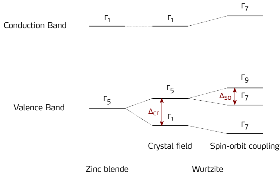
Figure 0.15.: Schematic explaining the valence band splitting in wurtzite ZnO.
