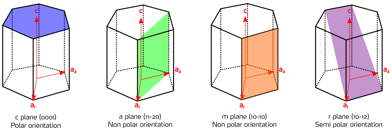
Figure 0.12.: Usual orientations for wurtzite ZnO epitaxial growth.
