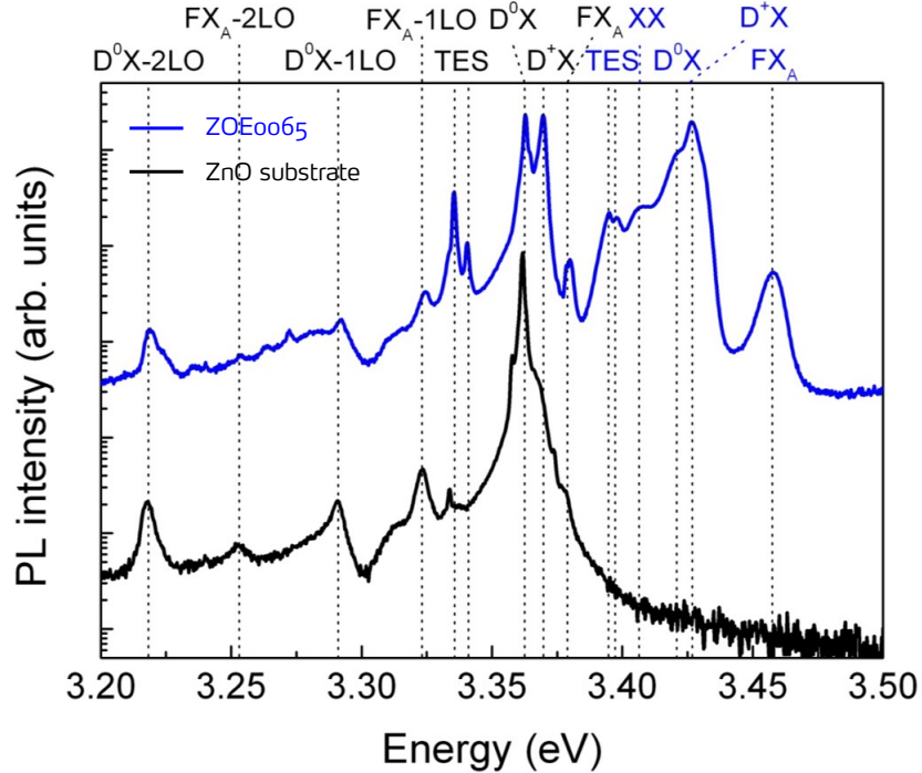
Figure 0.29.: PL spectra of a single QW sample and a m-plane ZnO substrate (respectively in blue and black curves) at 10 K. The QW is 2.9 nm thick, barriers are 80 nm wide and the Mg content is 26 %. The peaks attribution is shown in black for ZnO bulk related transitions and in blue for QW related transitions. The spectra have been shifted vertically in order to be easily compared.
