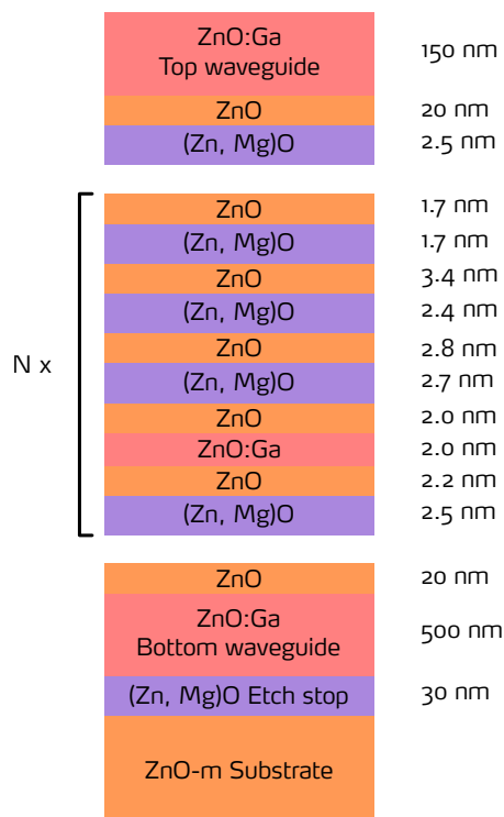
Figure 0.155.: Structure of QCL samples for THz. The number of active region period varies from one sample to another.
