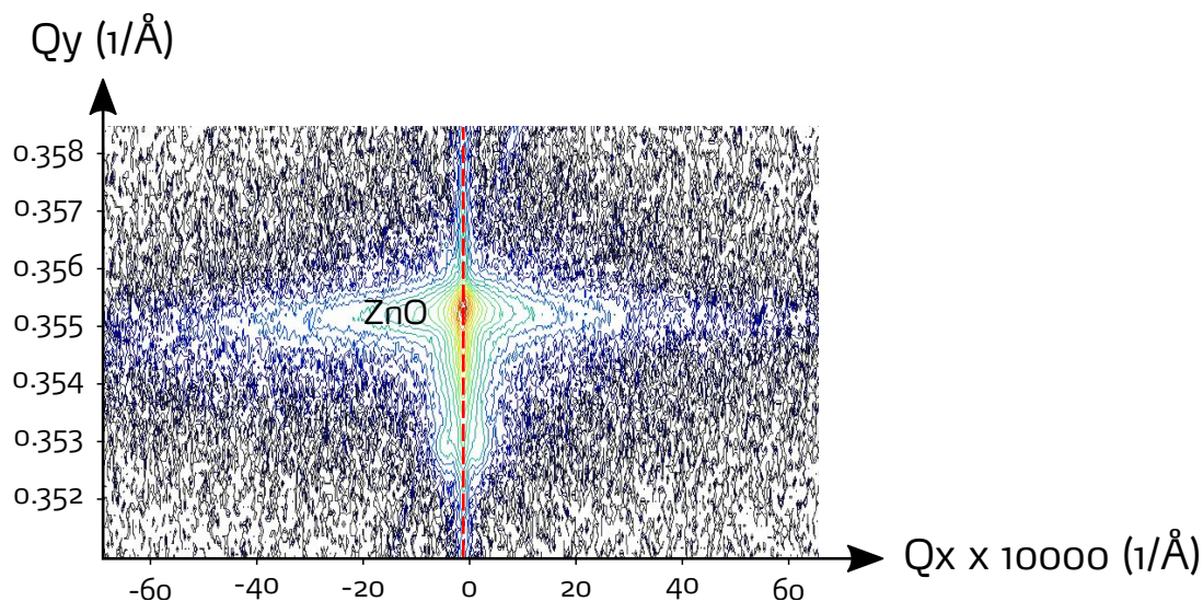
Figure 0.107.: RSM around the node (100), with \varphi = 90^\circ .
