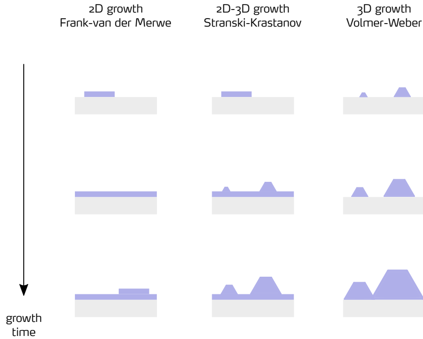
Figure 0.23.: Illustration of growth modes.
