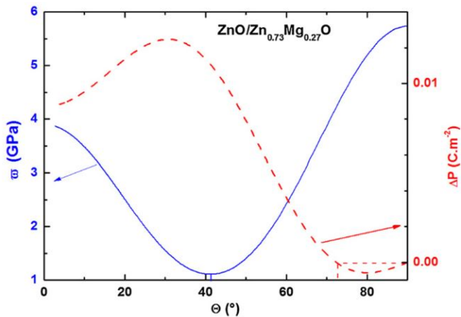
Figure 0.114.: Evolution of the elastic energy density stored as a function of the tilt angle \Theta with respect to the c-axis (blue curve). The red curve represents the evolution of the polarization shift at the interface between ZnO and (Zn, Mg)O. It is assumed that the (Zn, Mg)O is lattice matched on the ZnO. Bigenwald et al. (2012), URL, © IOP Publishing. Reproduced with permission. All rights reserved.
