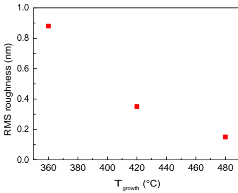
Figure 0.88.: Evolution of the RMS roughness with the growth temperature T_{\text{growth}} taken on 4 \mu\text{m}^2 images.
