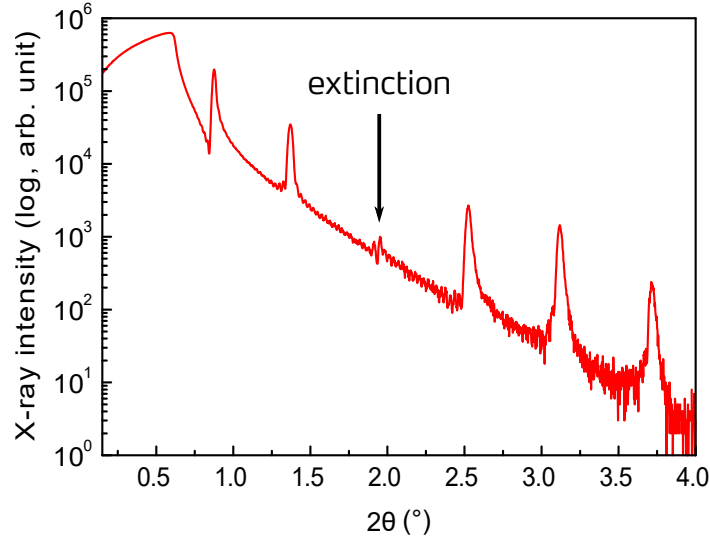
Figure 0.133.: XRR spectra of the asymmetrical QW with the thinner barrier - 0.5 \text{ nm} .
