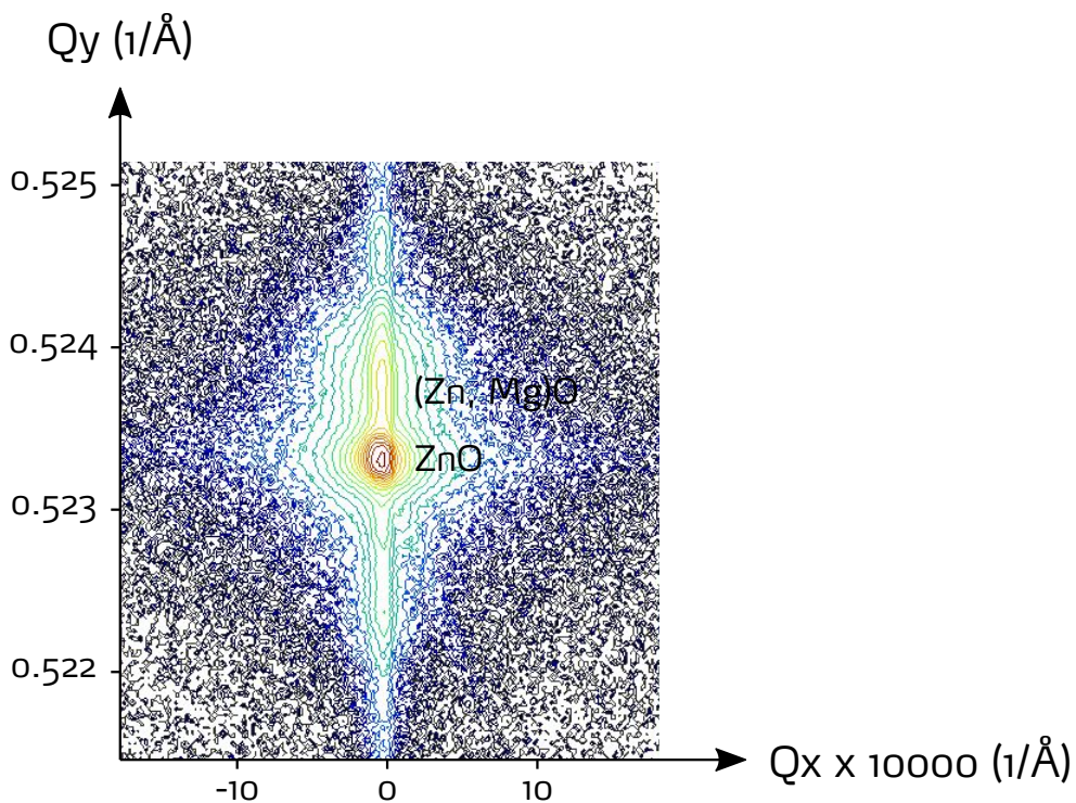
Figure 0.118.: RSM around the (102) node for \varphi = 90^\circ .
