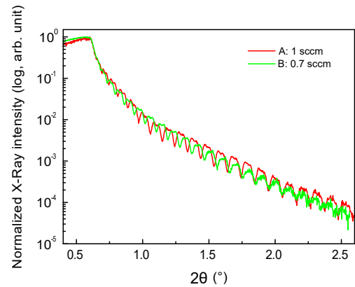
Figure 0.33.: XRR spectra of samples A and B.
