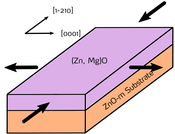
Figure 0.100.: Schematic representation of the stress states of m-plane (Zn, Mg)O grown on ZnO. The alloy is in tension in the [0001] direction, whereas it undergoes compression in the [1\bar{2}10] direction.
