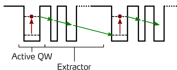
Figure 0.145.: QCD schematic principle.
