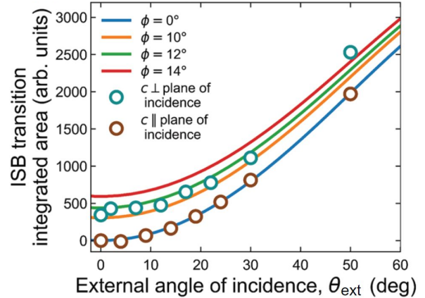
Figure 0.129.: Evolution of the ISBT intergrated area when the angle of incidence varies. Dots represents the experimental data and the lines the geometric model for various tilted angles \phi . (Montes Bajo et al., 2018a), © figure used under the Creative Commons Attribution 4.0 International Licence. To view a copy of this licence, visit: URL
