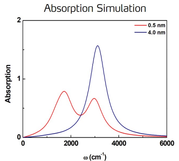
Figure 0.136.: Simulation of the absorption spectra for a 0.5\text{ nm} and 4.0\text{ nm} coupling barrier (red and blue curve respectively). The absorption unit is arbitrary.
