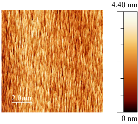
Figure 0.148.: AFM image 10 \times 10 \mu\text{m}^2 of the 20 periods QCD. The RMS roughness is 0.72 \text{ nm} .
