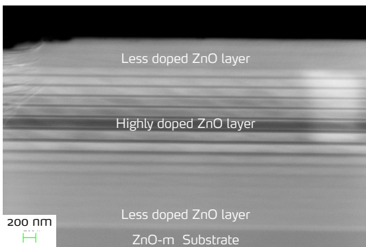
Figure 0.60.: SEM cross-section of the gradually doped sample.
