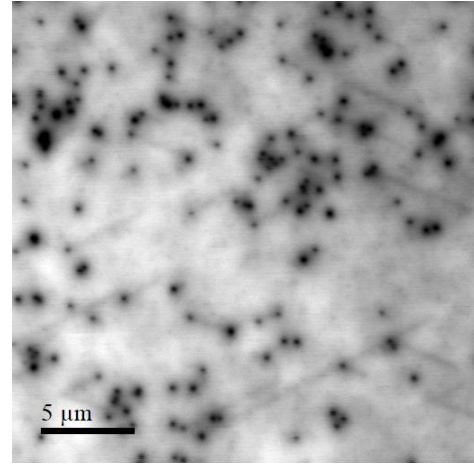
Figure 0.116.: CL image of a r-plane MQW sample with x_{Mg} = 18\% . The applied tension for electrons is 20 kV. This image is rotating by 90^\circ with respect to the AFM picture 0.115.
