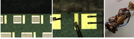
Figure 0.161.: Photos of processed QCLs that have been lapped, cleaved and mounted for spectroscopic measurements. Squares are top contacts whereas rectangles are the bottom ones.
