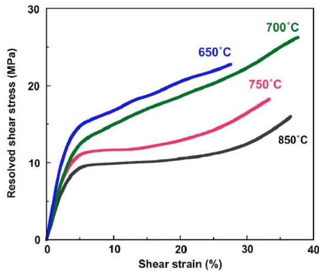
Figure 0.98.: Resolved shear stress as a function of the shear strain for ZnO at different temperatures during a compression test at a strain rate of 4.2 \times 10^{-4} \text{ s}^{-1} . Damaging is not reached during this test. Reprinted from Yonenaga et al. (2008), with the permission of AIP Publishing.
