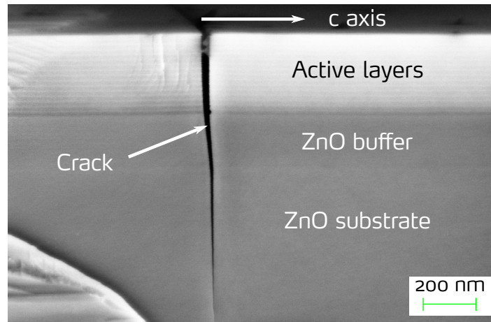
Figure 0.101.: SEM image in cross-section of a MQW with x_{Mg} = 40\% . The total (Zn, Mg)O thickness is 160 \text{ nm} . A crack is starting from the surface and end in the substrate.
