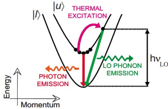
Figure 0.8.: Schematic showing the LO-phonon mechanism responsible for the lowering of the population inversion for RT QCLs. Reprinted from (Bellotti et al. , 2009), with the permission of AIP Publishing.
