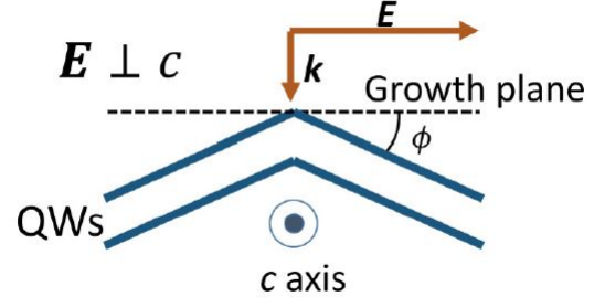
Figure 0.127.: Schematic of the incident case for undulated interfaces when the electric field is perpendicular to the c-axis. (Montes Bajo et al., 2018a), © figure used under the Creative Commons Attribution 4.0 International Licence. To view a copy of this licence, visit: URL
