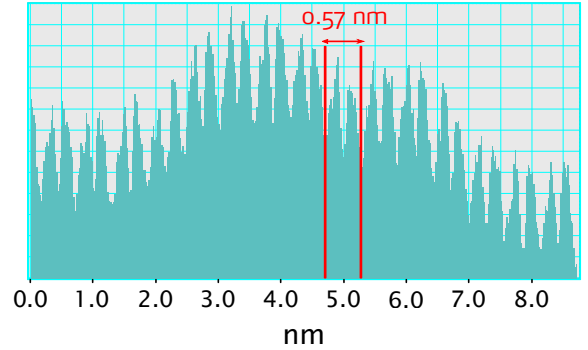
Figure 0.143.: Intensity profile of the area shown in figure 0.142. The thin barrier thickness on this image is 0.57 nm.
