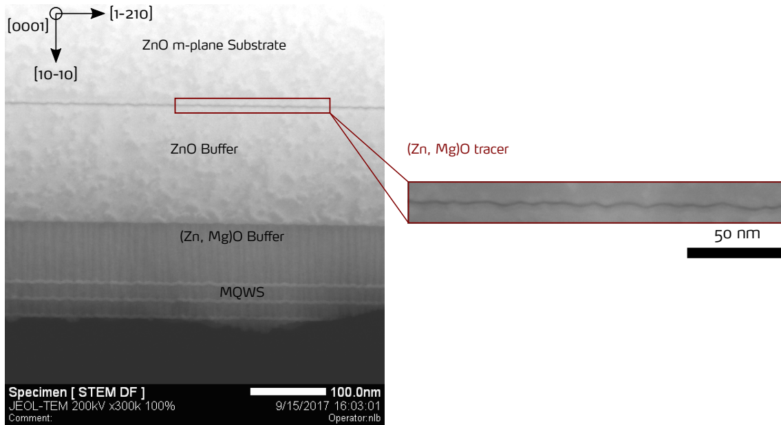
Figure 0.68.: STEM-HAADF image of a MQW sample in the [0001] zone axis. The zoomed part shows the (\text{Zn}, \text{Mg})\text{O} tracer grown between the ZnO substrate and the ZnO buffer.
