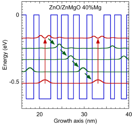
Figure 0.146.: MIR QCD design of a single period. The targeted wavelength is 3.7\ \mu\text{m} . The thicknesses are 2.6/1.5/0.9/1.5/1.2/1.3/1.7/1.2\ \text{nm} starting from the active QW. Bold values correspond to (Zn, Mg)O layers. The nominal Mg content is 40%. The only layer doped is the active QW with a nominal value of 2 \times 10^{19}\ \text{cm}^{-3} . Reprinted from (Jollivet et al., 2018), with the permission of AIP Publishing.
