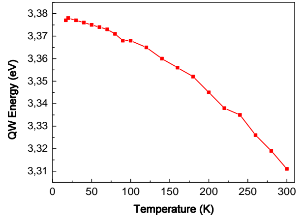
Figure 0.73.: Evolution of the exciton energy in the QW with the temperature. The Mg content in barriers is 25 %.
