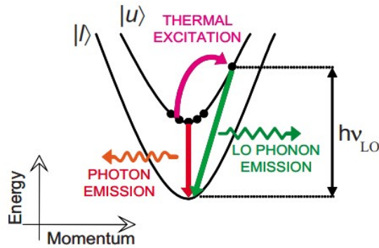
Figure 0.8.: Schematic showing the LO-phonon mechanism responsible for the lowering of the population inversion for RT QCLs. Reprinted from (Bellotti et al. , 2009), with the permission of AIP Publishing.
