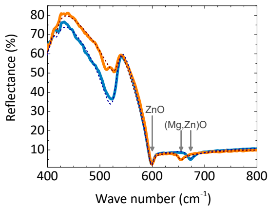
Figure 0.52.: Reflectance spectra taken in p -polarization at 30° of incidence of 2 MQWs based samples. The nominal Mg content for the sample described by the orange curve is 30 % and 34 % for the blue one. The thick lines are experimental curves and the dotted curves the fitted ones.
