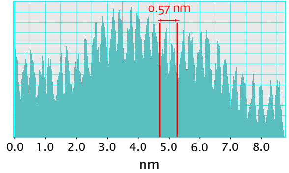
Figure 0.143.: Intensity profile of the area shown in figure 0.142. The thin barrier thickness on this image is 0.57 \text{ nm} .
