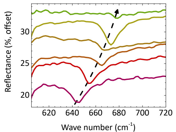
Figure 0.53.: Zoomed reflectance spectra taken in p -polarization at 30° of incidence of various MQWs with nominal Mg content ranging from 22 to 41 % according to the black arrow.
