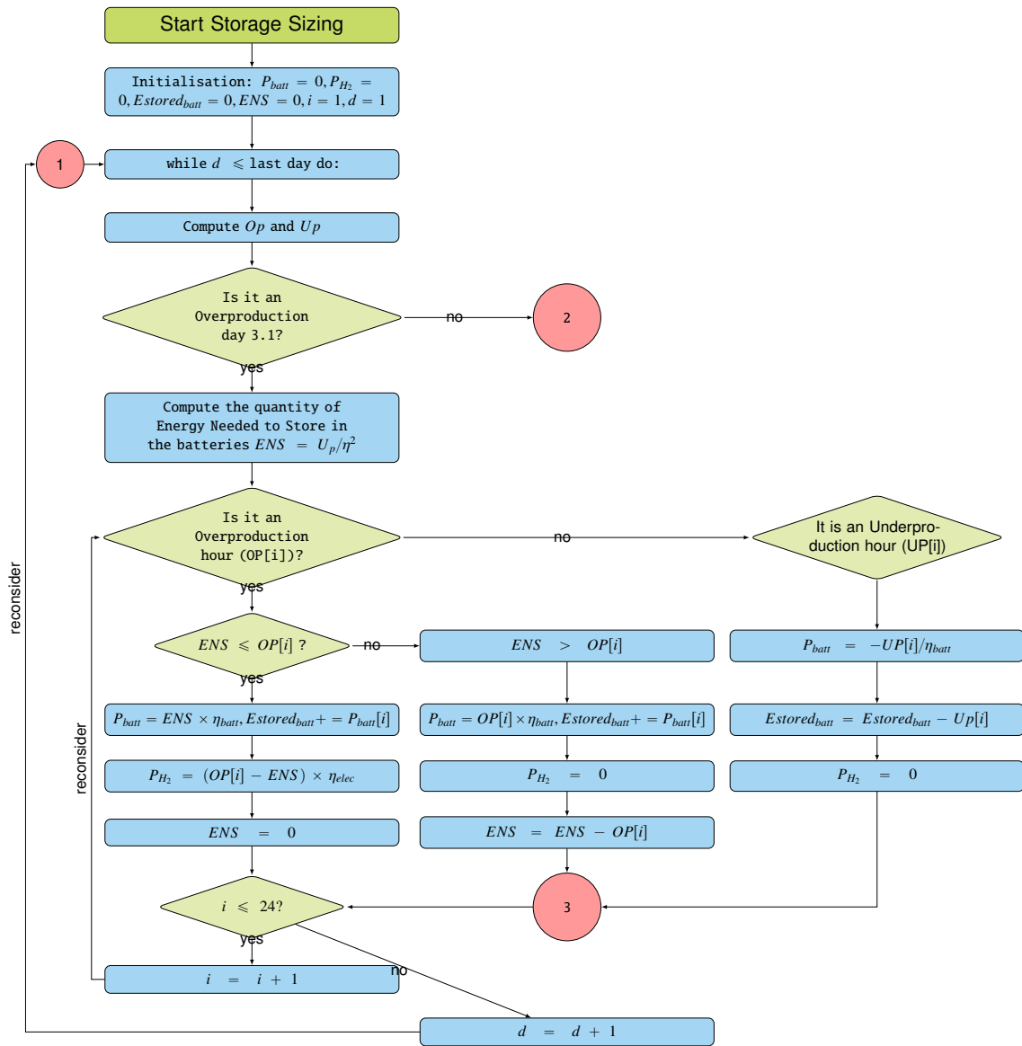
Figure 3.10: Overproduction day sizing
