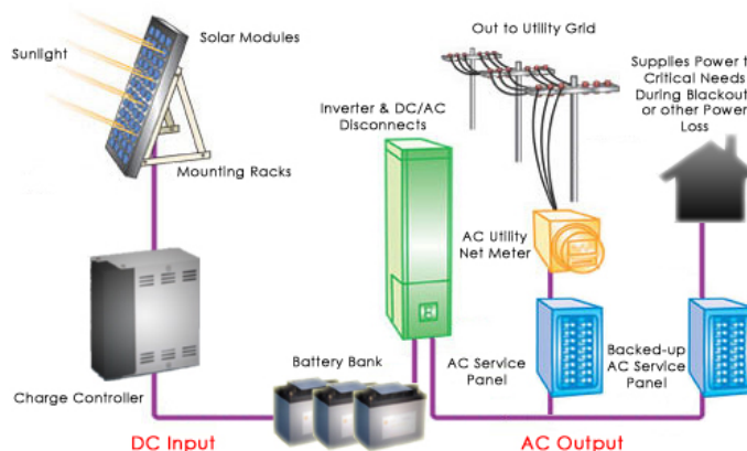
Figure 1.10: Grid Tied System [141]
