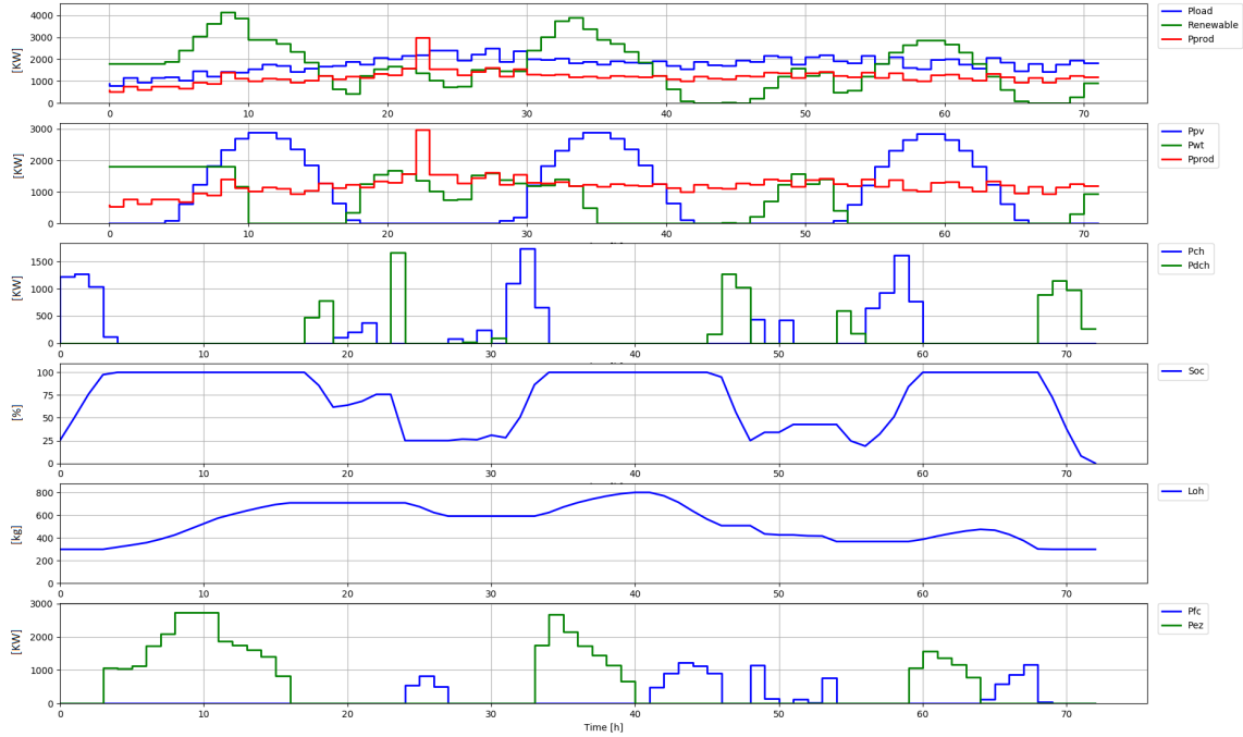
Figure 4.8: Management of the resources to match with a requested profile with r_f = 0.3
