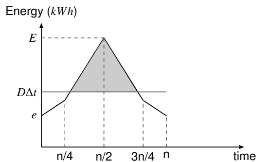
Figure 3.2: Primary energy produced by PV respectively for the best and the worst day (Integral of the power during both days)
