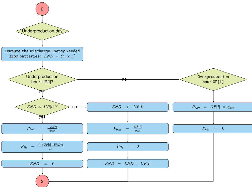
Figure 3.12: Underproduction day sizing
