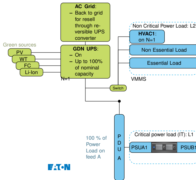
Figure 2.1: Classical N architecture.
