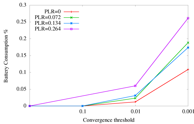
Fig. 4.6: Battery consumption with lossy transmission channel
