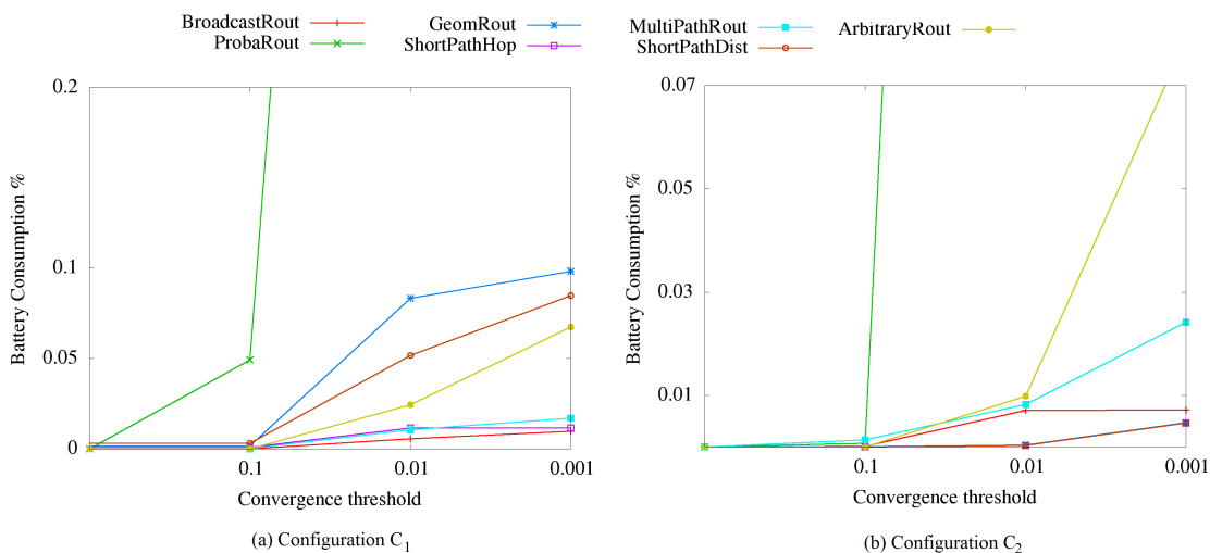
Fig. 5.2: Battery Consumption of optimization step
