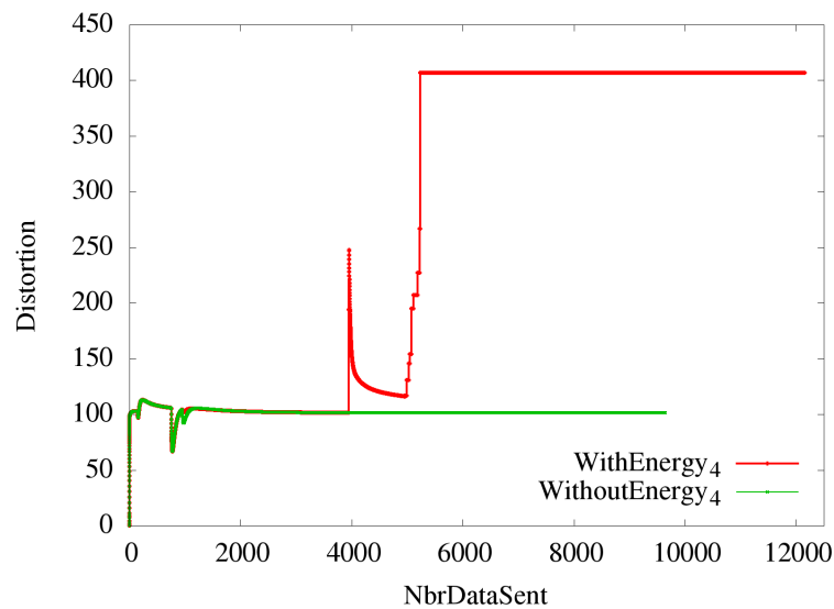
Fig. 7.14: Distortion comparison
