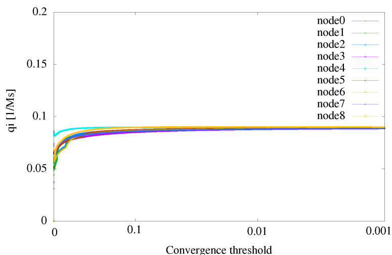
Fig. 4.1: Auxiliary variables convergence
