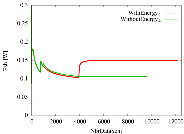
Fig. 7.16: Encoding power comparison
