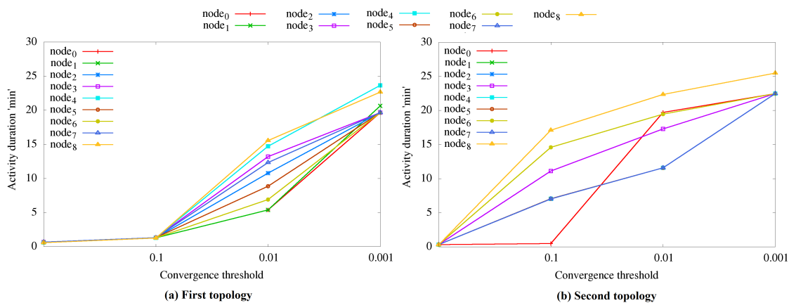
Fig. 6.10: Optimization duration for the first topology
