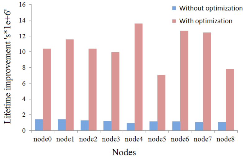
Fig. 3.8: Remaining lifetime comparison
