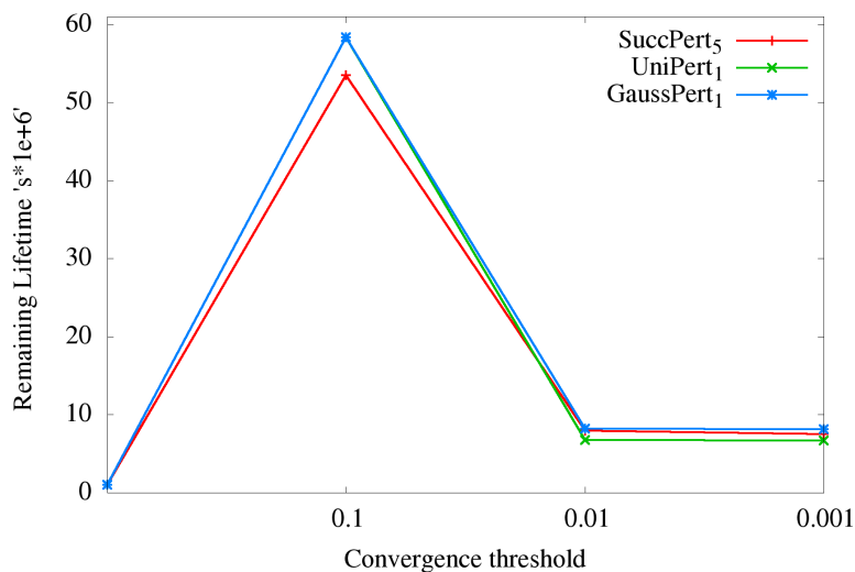
Fig. 7.7: Remaining lifetime after each convergence threshold
