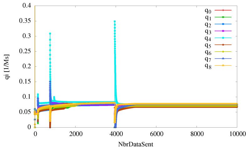
Fig. 7.12: Convergence of the system
