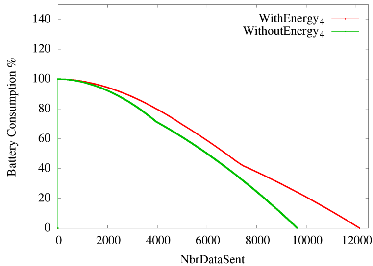
Fig. 7.13: Energy consumption comparison
