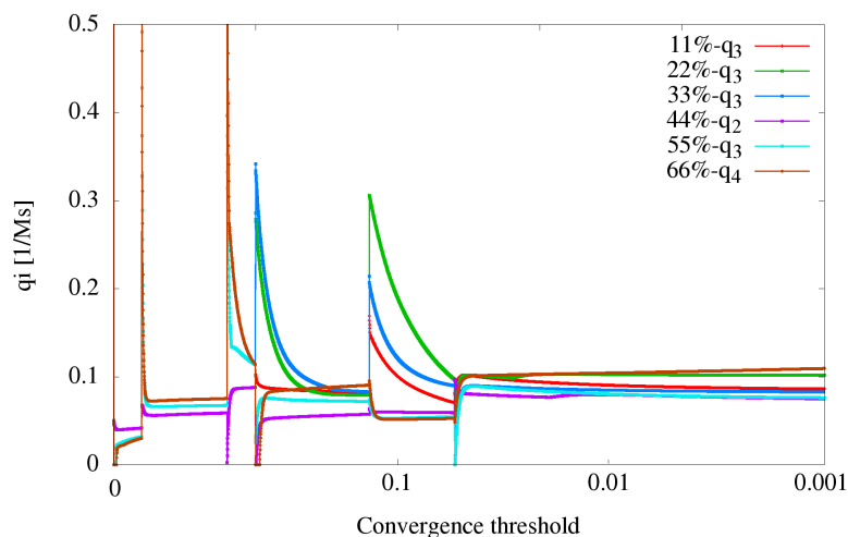
Fig. 7.8: System convergence
