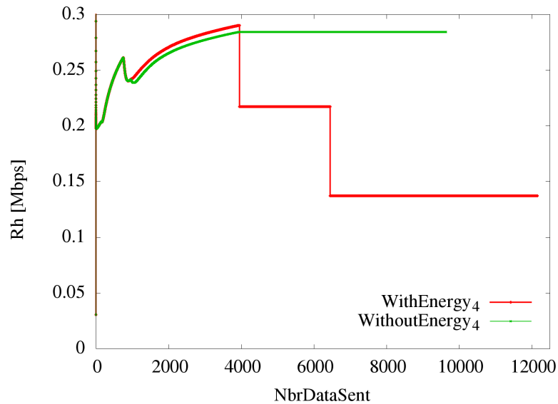
Fig. 7.17: Data rate comparison
