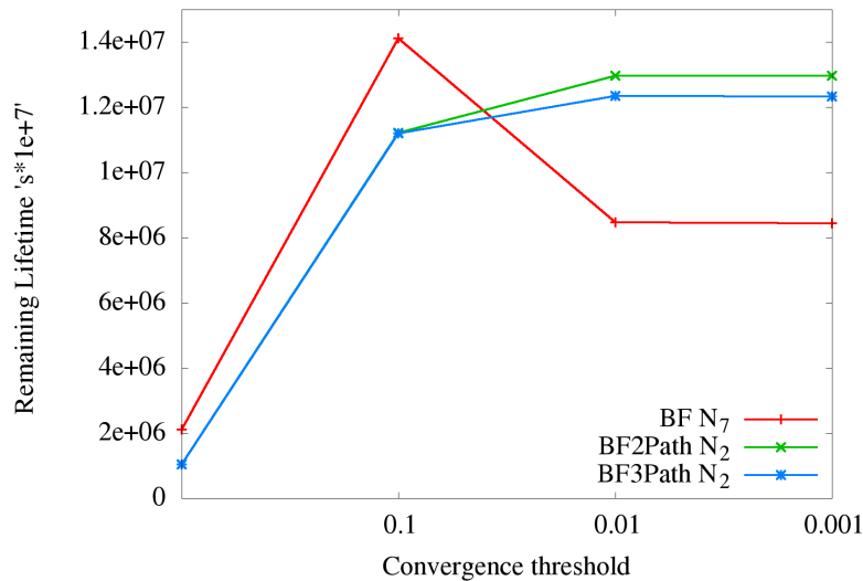
Fig. 6.6: Remaining lifetime after each convergence threshold
