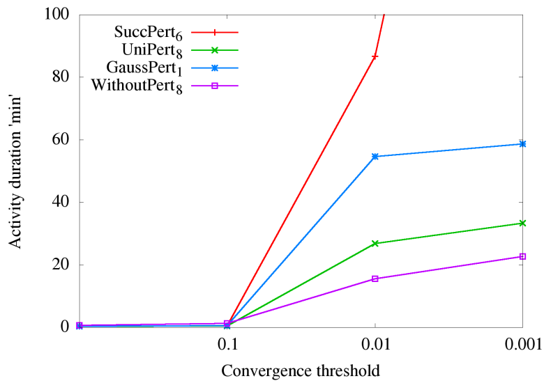
Fig. 7.6: Activity duration of optimization steps
