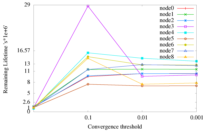
Fig. 3.7: Remaining lifetime after each convergence threshold
