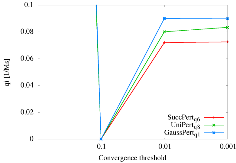
Fig. 7.3: Convergence to a common value q
