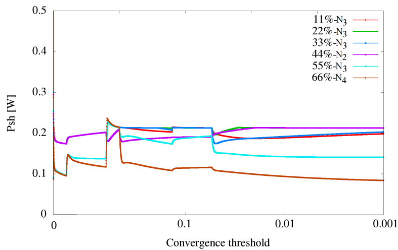
Fig. 7.9: Encoding power variation
