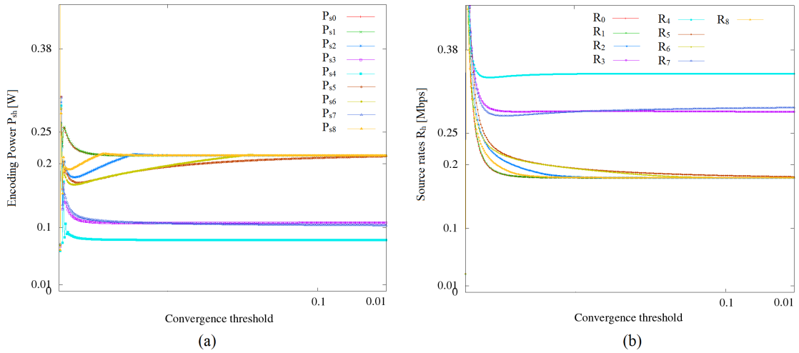
Fig. 3.3: (a)Encoding powers, (b)Source rates versus the convergence threshold
