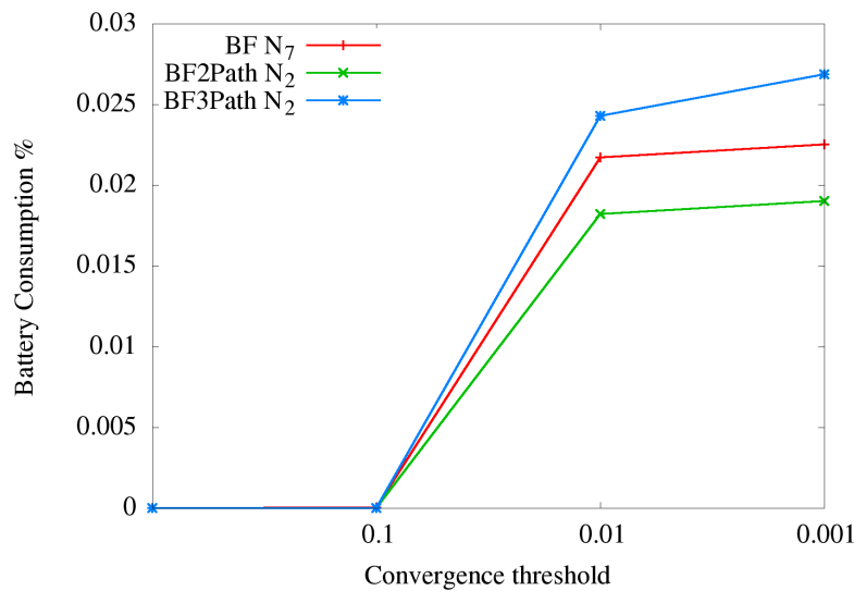
Fig. 6.4: battery consumption of optimization steps
