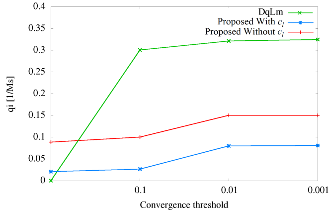
Fig. 4.5: Network lifetime inverse comparison
