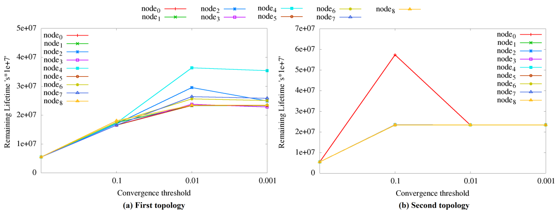
Fig. 6.11: Remaining lifetime after each convergence threshold for the first topology
