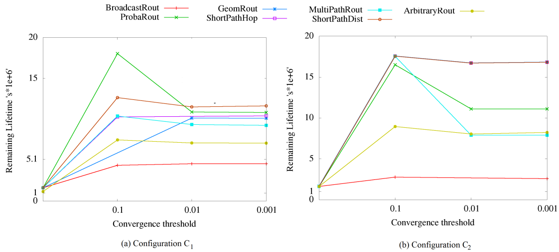
Fig. 5.4: Remaining Lifetime
