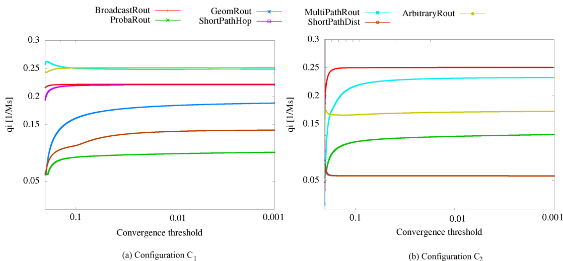
Fig. 5.5: Lifetime inverse q = 1/T_{net}
