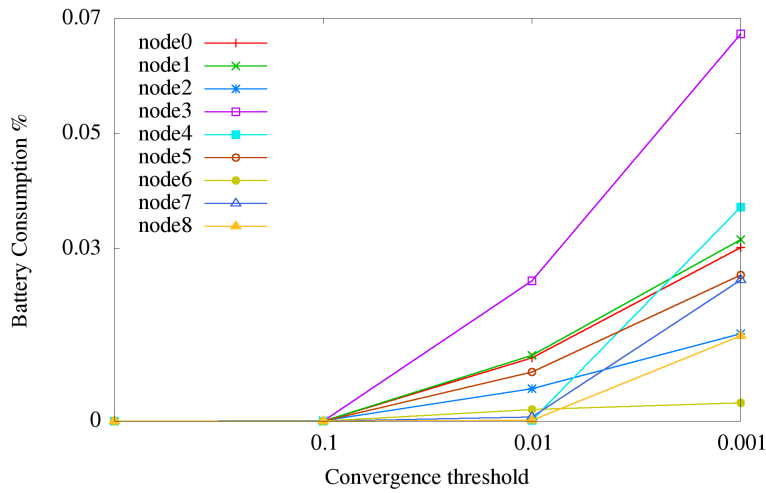
Fig. 3.5: battery consumption of optimization steps
