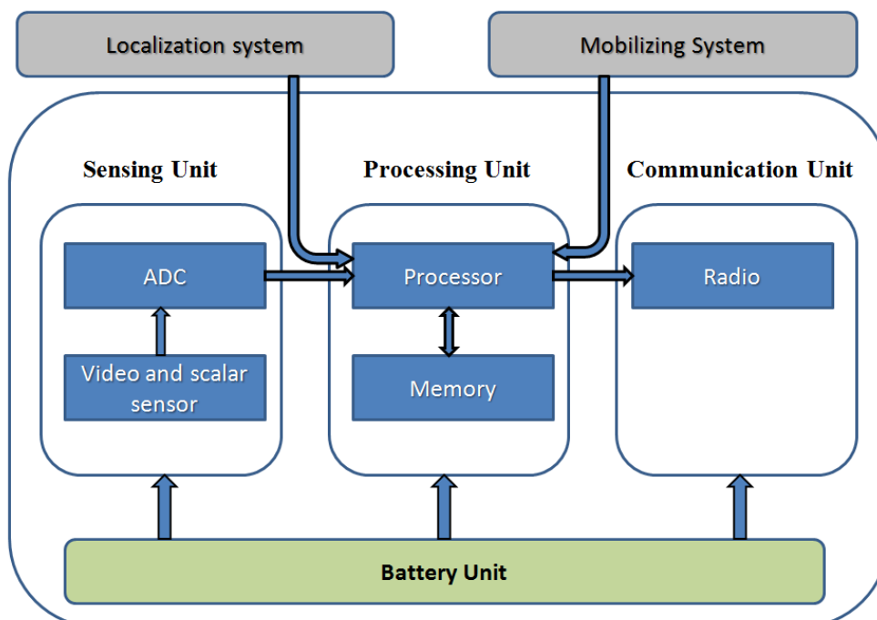
Fig. 1.3: Video sensor node architecture.
