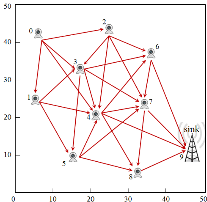
Fig. 6.1: Example of a WMSN.
