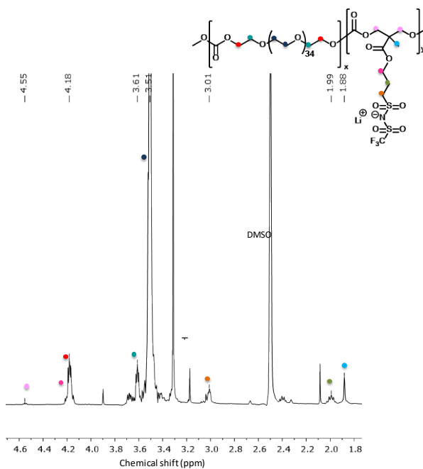
Figure A11. 1 H NMR spectra of SIPC-2 in DMSO-d 6 .
