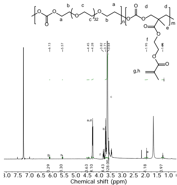
Figure A10. 1 H NMR spectra of PEO 34 -PC 10 wt% MA in CDCl 3 .
