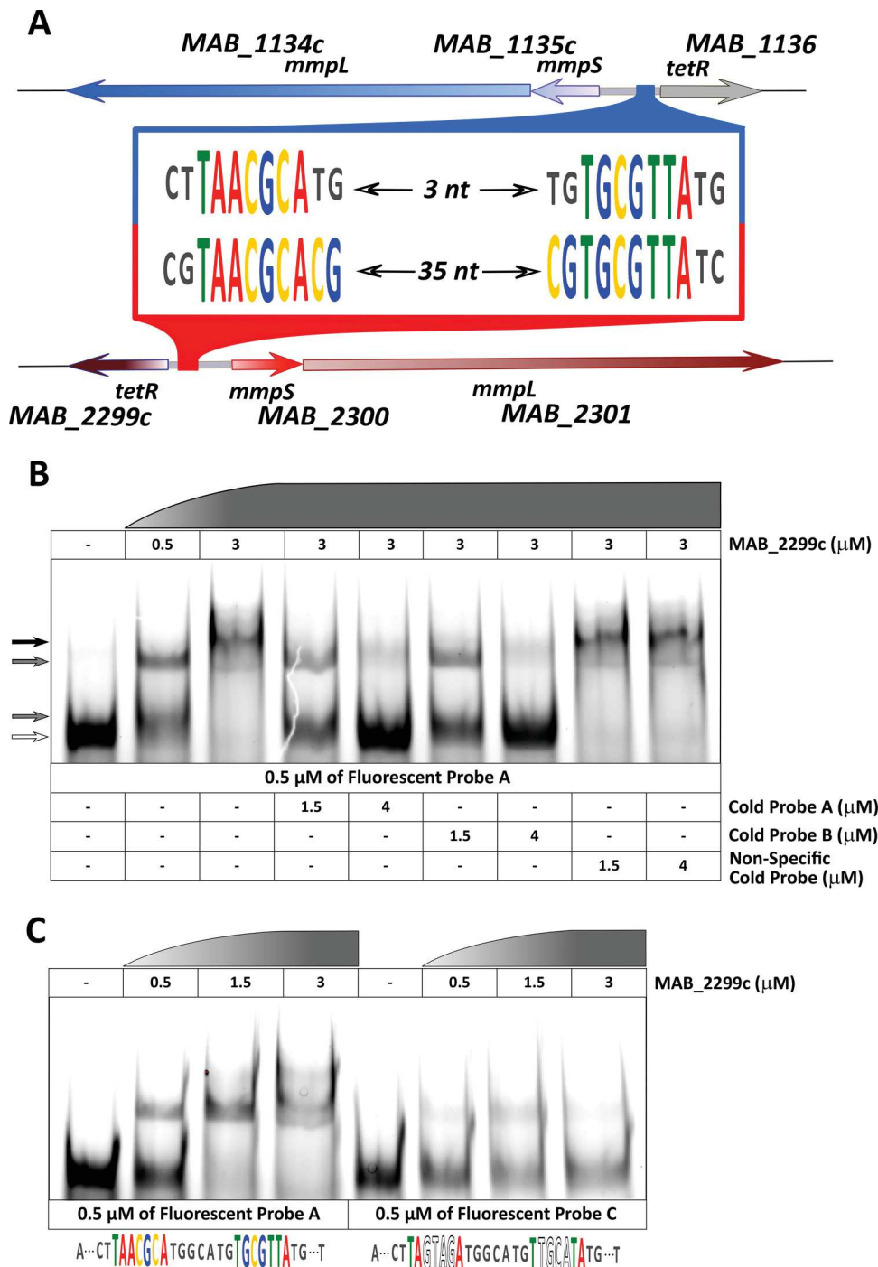
FIG 4 TetR regulator MAB_2299c binds to the intergenic region upstream of MAB_1135c-1134c. (A) Schematic representation of the DNA operators located upstream of MAB_1135c-1134c (comprising probe A) and MAB_2300-2301 (comprising probe B). The palindromic sequences of 7 nucleotides in probe A are separated by a spacer and are identical to those found in probe B, in which they are separated by 35 nucleotides. (B) EMSA and competition assays using purified MAB_2299c and incubated with 5' fluorescein-labeled probe A in the absence or presence of an excess of unlabeled probe A or probe B. A nonrelated probe was also included as a control of specificity of the TetR/DNA complex formed. Detection of the unbound or the complexed probe A was revealed by fluorescence emission. The white arrow indicates the DNA alone, gray arrows the formation of intermediate TetR/DNA complexes, and the black arrow the formation of a complete TetR/DNA complex. (C) Comparison of the EMSA pattern of MAB_2299c incubated with 5' fluorescein-labeled probe A and probe C in which 4 of the central nucleotides forming the palindromic sequences of probe A were replaced by a random sequence, resulting in a clear defect in the formation of the TetR/DNA complex. The corresponding unbound and complexed probes were revealed by fluorescence emission.
