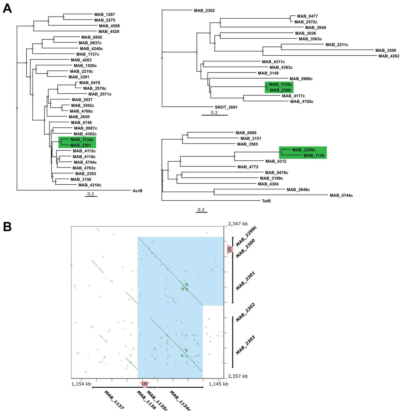
FIG 1 Closest paralogs of the MmpS - MmpL couple MAB_2300-2301 , MAB_1135c-1134c , arose as a result of a gene duplication event. (A) Homology trees of all M. abscessus MmpL (left), all M. abscessus MmpS (top right), and several M. abscessus TetR / MarR family transcriptional regulators in close proximity to MmpS - MmpL couples (bottom right). The scale bar below each tree indicates 0.2 amino acid substitutions per site. The trees were rooted to Escherichia coli AcrB ( MmpL ) and TetR (transcriptional regulator) and Segniliparus rotundus MmpS ortholog SROT_2691 ( MmpS ). (B) Dot plot generated using the YASS genomic similarity tool ( http://bioinfo.lifl.fr/yass/yass.php ), showing nucleotide similarity between the MAB_2299c-2300-2301 and the MAB_1136-1135c-1134c loci (highlighted by a light blue inverted-L-shaped box). Green lines indicate forward matches, and red lines indicate reverse matches. The intergenic regions (IR) between the tetR genes ( MAB_2299c and MAB_1136 ) and the mmpS genes ( MAB_2300 and MAB_1135c ) are highlighted by light gray trapezoidal boxes.
