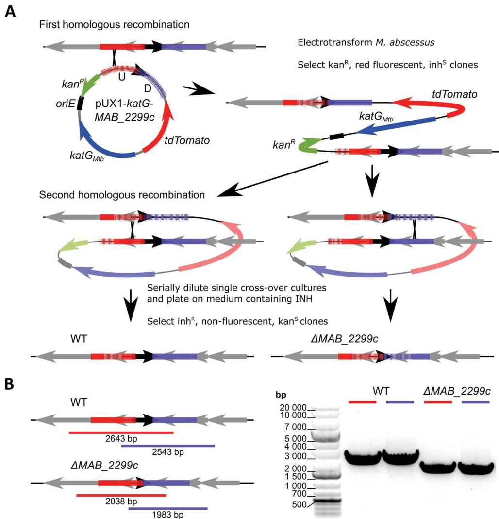
FIG 3 Generation of an unmarked MAB_2299c deletion mutant in M. abscessus . (A) Line drawing illustrating the general protocol followed to ascertain the \Delta MAB_{2299c} mutant. katG_{Mtb} , M. tuberculosis katG . (B) (Left) Line drawing of the genomic context in the M. abscessus WT and \Delta MAB_{2299c} mutant that also illustrates the PCR strategy followed to confirm the deletion of MAB_2299c . Red and blue bars, the PCR products obtained during the screening of potential mutant clones; black arrow, MAB_2299c . (Right) A gel confirming the \Delta MAB_{2299c} genotype. The red and blue bars correspond to the amplicons obtained in the left panel. These amplicons were subjected to sequencing analysis to confirm the correct deletion of the MAB_2299c gene.
