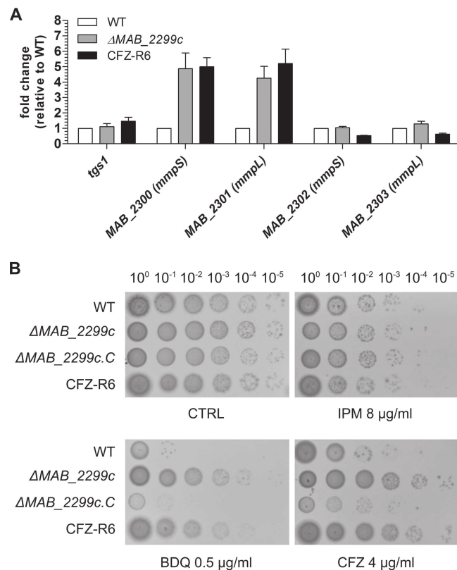
FIG 4 Deletion of MAB_2299c confers resistance to both CFZ and BDQ. (A) Results of a qRT-PCR experiment showing the induction levels of the mmpS-mmpL ( MAB_2300-MAB_2301 ) pair but not MAB_2302-MAB_2303 when MAB_2299c is deleted from the M. abscessus genome. (B) Profile of the susceptibility or resistance of M. abscessus WT, M. abscessus \Delta MAB_{2299c} , and the complemented derivative of \Delta MAB_{2299c} ( \Delta MAB_{2299c.C} ) to BDQ, CFZ, or IPM. Five microliters of 10-fold serially diluted bacterial suspensions of exponentially growing cultures was spotted on Middlebrook 7H10 plates in the absence (control [CTRL]) or presence of drugs at the indicated concentrations. The plates were incubated at 37°C for 4 days.
