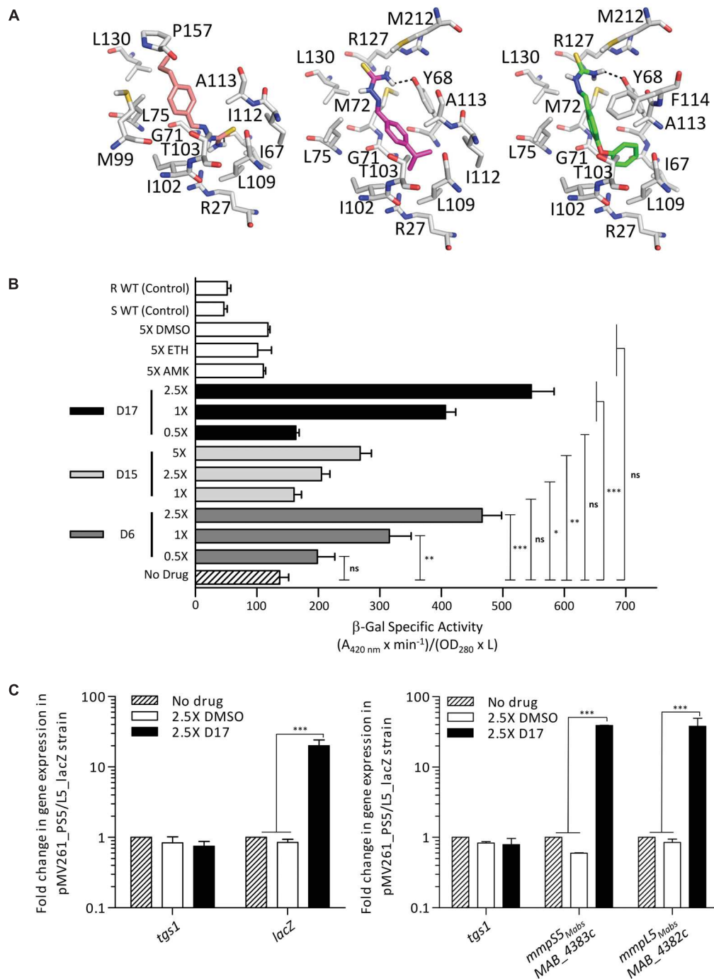
FIGURE 7 | IR S5/L5 can be induced by structural analogs of thiactazone. (A) Docking of TAC derivatives in the ligand binding site of MAB_4384. All the residues involved in van der Waals, hydrophobic bonds or hydrogen bonds (in black dashes) are displayed as sticks. D15 in salmon has a binding energy of \Delta G = -6.6 kcal/mol, D6 in magenta has a \Delta G = -7.3 kcal/mol, and D17 seems to bind slightly stronger with a \Delta G = -8.3 kcal/mol. (B) Conditional induction of lacZ by structural analogs of TAC in M. abscessus . Induction of \beta -Gal activity in wild-type M. abscessus S carrying pMV261_P S5/L5 - lacZ was assayed using mid-log phase cultures incubated with increasing drug concentrations varying from 1X to 5X the MIC for D15 and varying from 0.5X to 2.5X the MIC for D6 and D17. Inductions were performed for 96 h at 37°C. The \beta -galactosidase specific activity ( SA_{\beta-Gal} ) was quantified in liquid cultures using ONPG as a substrate. Amikacin (AMK) and ethionamide (ETH) were included as unrelated drug controls. (C) Transcriptional profile of lacZ in the M. abscessus pMV261_P S5/L5 - lacZ reporter strain exposed to 2.5X the MIC of D17 for 8 h (left). tgs1 was included as a non-relevant control. Replacing D17 by an equal volume of DMSO had no effect on lacZ transcription. Transcriptional induction of mmpS5 Mabs and mmpL5 Mabs following exposure to 2.5X the MIC of D17 for 8 h (right). Results were obtained from three independent experiments and the error bars represent standard deviation. For statistical analysis the Student's t -test was applied with ns, *, **, ***, **** indicating non-significant, p < 0.05 , p < 0.01 , p < 0.001 , and p < 0.0001 , respectively.
