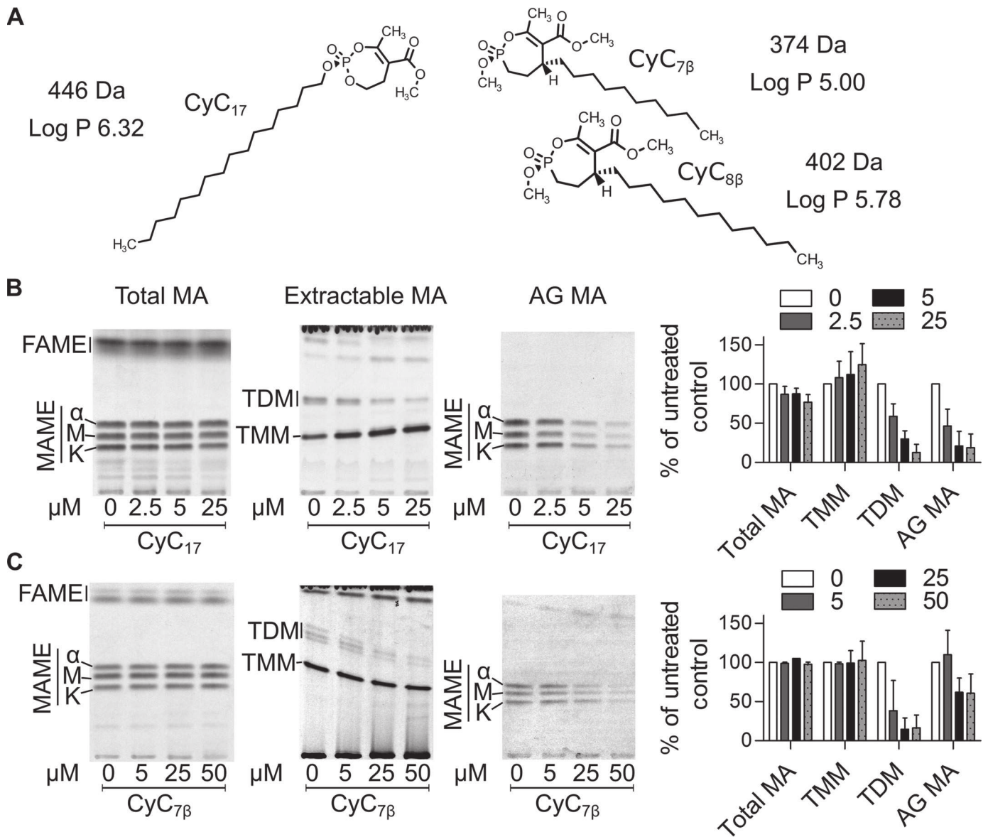
Figure 1. Ag85 complex mycolyltransferase activity is inhibited by CyC analogs in vivo . Exponentially growing M. tuberculosis mc 2 6230 was incubated with increasing concentrations of CyC 17 or CyC 7β in 7H9 OADC /Tween 80 at 37 °C with agitation for 1 h. Subsequently, bacteria were labeled with sodium [2- 14 C]acetate for 6 h at 37 °C with agitation. The cultures were split, and from the first volume were extracted the total methyl esters of mycolates (MAME) and fatty acids (FAME). From the second volume, apolar and polar lipid fractions were obtained before derivatization of arabinogalactan MAME. A , chemical structures of the CyC analogs used in this study. B and C , effect of CyC 17 ( B ) or CyC 7β ( C ) treatment on the mycolic acid profiles of M. tuberculosis mc 2 6230. Equal counts (50,000 cpm) of MAME + FAME fraction were loaded on a TLC plate and resolved once using the solvent system hexane/ethyl acetate (95:5, v/v) run twice ( far left ). The apolar fraction was loaded (50,000 cpm), and TMM and TDM were visualized on a 1D TLC plate using the solvent system chloroform/methanol/water (40:8:1, v/v/v) ( middle left ). Equal volumes of arabinogalactan MAME fraction were loaded, and α, methoxy, and keto mycolic acids were visualized on a 1D TLC plate using the solvent system hexane/ethyl acetate (95:5, v/v) run twice ( middle right ). Densitometric analysis ( far right ) was performed on the TLCs shown in the left panels. Histograms and error bars , means and S.D. values calculated from at least two independent experiments.
