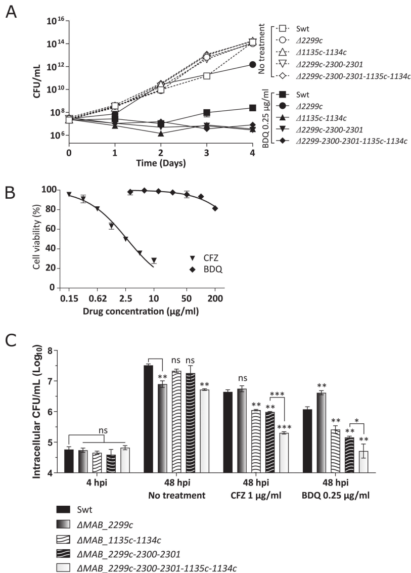
FIG 5 Activity of BDQ in vitro and in infected macrophages. (A) M. abscessus CIP104536 T WT and its mutant derivatives were either left untreated or exposed to 0.25 µg/ml BDQ in 7H9 ODC at 30°C. Bacterial suspensions were collected on a daily basis, diluted, plated on LB agar, and further incubated at 37°C for 4 days prior to CFU determination. Results are expressed as the means ± standard errors of the means from triplicates and are representative of two independent experiments. Ctrl, untreated cultures; Swt, smooth wild type. (B) Cytotoxicity assay of CFZ and BDQ toward THP-1 macrophages. Cells were treated for 48 h with increasing concentrations of CFZ or BDQ, and viability was determined using the CellTiter-Blue reagent. The percentage of cell survival was determined based on control cells incubated in DMSO-containing medium. (C) M. abscessus -infected THP-1 macrophages were exposed to either 1 µg/ml CFZ or 0.25 µg/ml BDQ for 2 days before they were lysed and plated for subsequent CFU enumeration. Histograms and error bars represent means and standard errors of the means calculated from three independent experiments. CFU numbers at 4 h postinfection reflect the sizes of the different inocula. For statistical analysis, Student's t test was applied. ns, *, **, and *** stand for nonsignificant, P < 0.01 , P < 0.001 , and P < 0.0001 , respectively.
