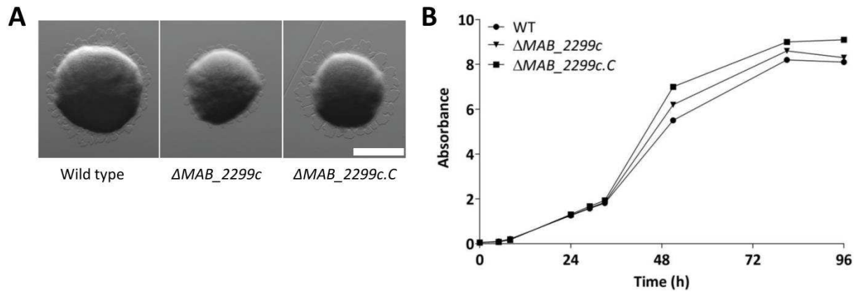
Fig. S3. Colony morphology ( A ) and in vitro growth ( B ) of parental M. abscessus WT CIP104536 T , \Delta MAB_{2299c} and its complemented derivative \Delta MAB_{2299c.C} . Bacteria were grown in 7H9 broth supplemented with OADC and 0.05% Tween 80. Growth was monitored by determining the OD 600 at different time points. Scale bar corresponds to 150 \mu m.
