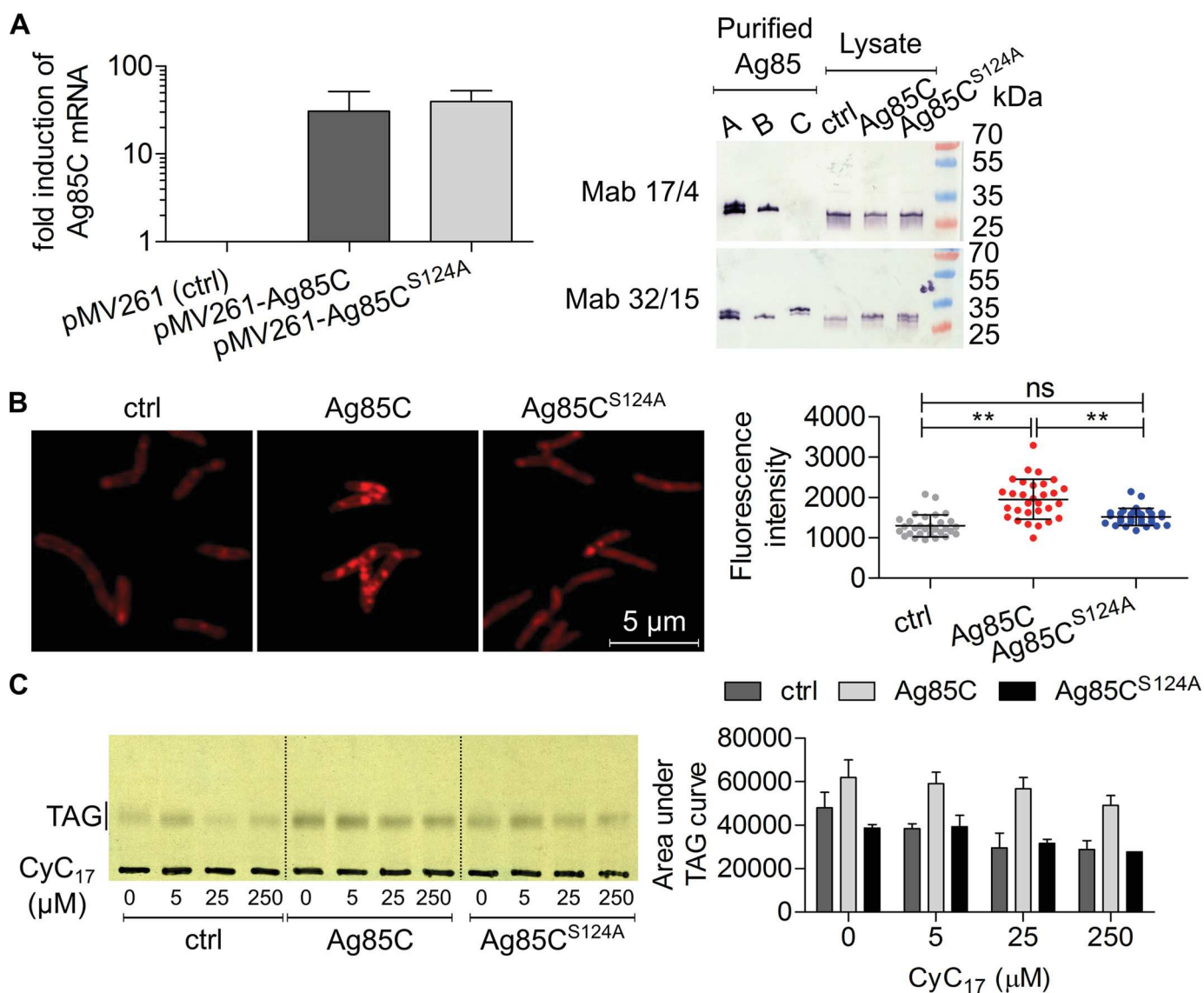
Figure 4. Biosynthesis of TAG in M. tuberculosis is inhibited by CyC 17 and is dependent upon Ag85C expression. A , quantitative real-time PCR analysis showing the -fold increase in the Ag85C transcripts in M. tuberculosis mc 2 6230 containing either pMV261 (ctrl), pMV261-Ag85C, or pMV261-Ag85C S124A (left). Western blotting using the 32/15 and 17/4 monoclonal antibodies probed against purified Ag85A/B/C and crude lysates of M. tuberculosis mc 2 6230 containing either pMV261, pMV261-Ag85C, or pMV261-Ag85C S124A (right). B , Nile Red staining of M. tuberculosis strains growing exponentially (left) with the corresponding fluorescence quantification (right). Fluorescence quantification was performed on 30 bacilli of each group. Shown are the mean fluorescence and S.D. values. Means were compared by the two-tailed Mann-Whitney test. ns, non-significant; **, p < 0.01 . Results shown are representative of two independent experiments. C , cultures were exposed to increasing concentrations of CyC 17 in 7H9 OADC/Tween 80 and labeled with sodium [2- 14 C]acetate for 4 h at 37 °C with agitation. The apolar fraction was extracted to analyze de novo synthesis of TAG. Equal counts (50,000 cpm) of apolar fraction were loaded, and TAG was visualized on a 1D TLC plate using the solvent system petroleum ether/diethyl ether (90:10, v/v) (left). Right, densitometric analysis of TLCs. Histograms and error bars, means and S.D. values calculated from four independent experiments.
