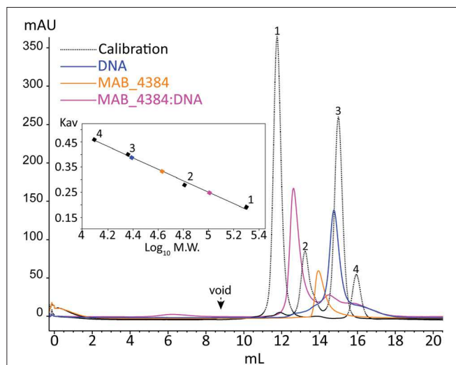
FIGURE 5 | Oligomerization of MAB_4384 and the MAB_4384:DNA complex in solution. The oligomeric states of MAB_4384 alone or complexed to its DNA target were determined by size exclusion chromatography. The elution profile of the proteins, used for the calibration is displayed as a dashed black line. Calibration was established using \beta -amylase (200 kDa) (1), bovine serum albumin (66 kDa) (2), carbonic anhydrase (29 kDa) (3), and cytochrome C (12.4 kDa) (4), eluting with estimated volumes of 11.7, 13.2, 14.9, 15.9 mL, respectively. The void volume was determined with the elution volume (8.8 mL) of dextran blue. MAB_4384 (dimer) was at a concentration of 3.9 mg/mL. The elution profiles of MAB_4384 dimer, DNA target and MAB_4384 bound to the DNA target are shown in orange, blue, and pink and their respective elution peaks were at 13.9, 14.7, and 12.6 mL. K_{av} indicates the partition coefficient.
