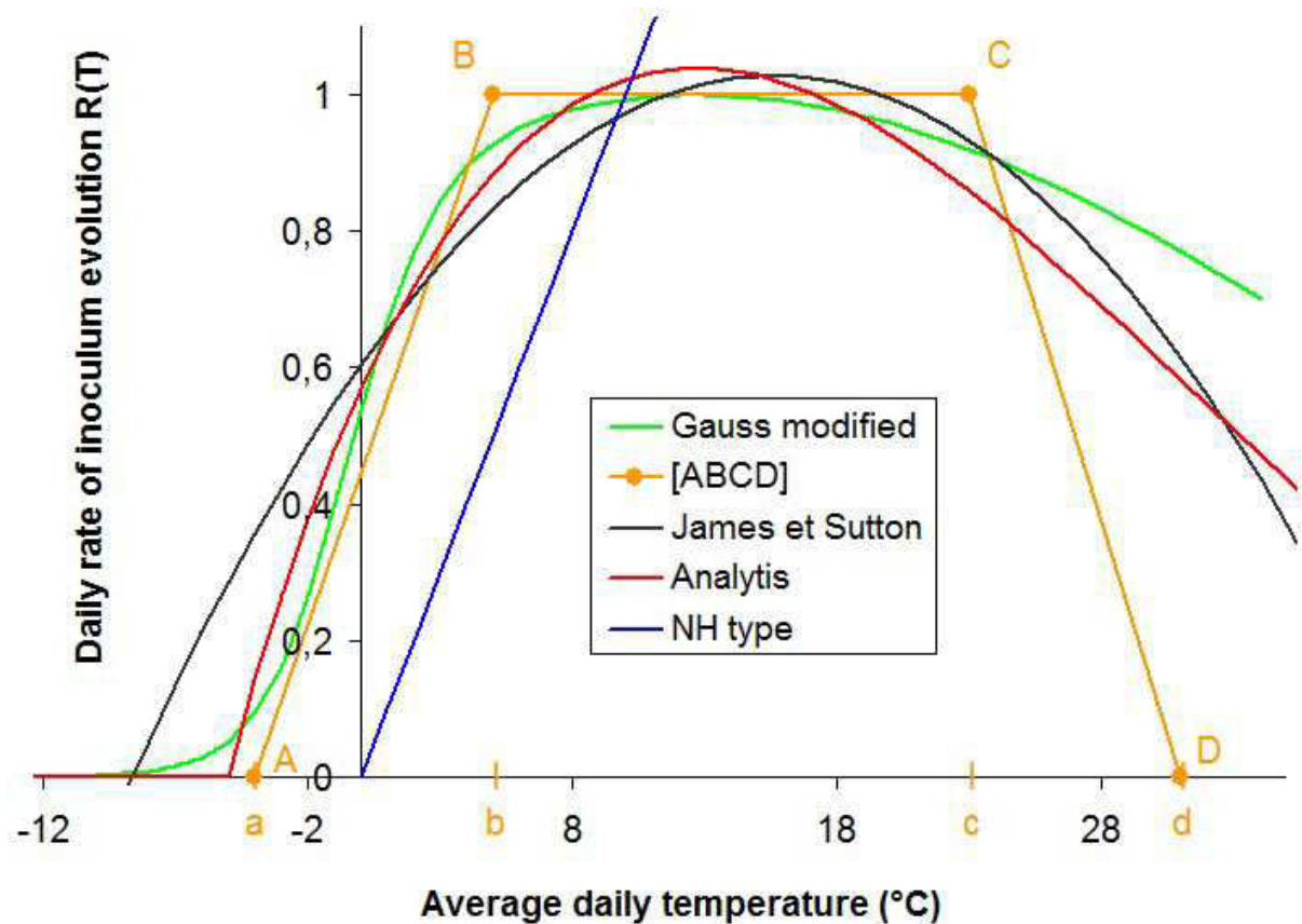
Figure 1. Temperature response functions used for describing the relationship between the daily rate of pseudothecial maturation R and the average daily temperature T for ascospore release models. The definitions of the functions are provided in Table 1.
