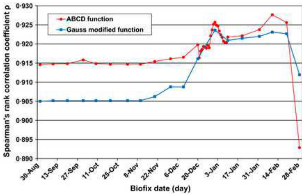
Figure 5. Comparison of the effect of the biofix on the level of statistical dependence between observed data and the calculated sum of daily rates of pseudotheical maturation (evaluated with Spearman's rank correlation \rho ) for the ABCD and the Gauss modified thermal time scale functions.
