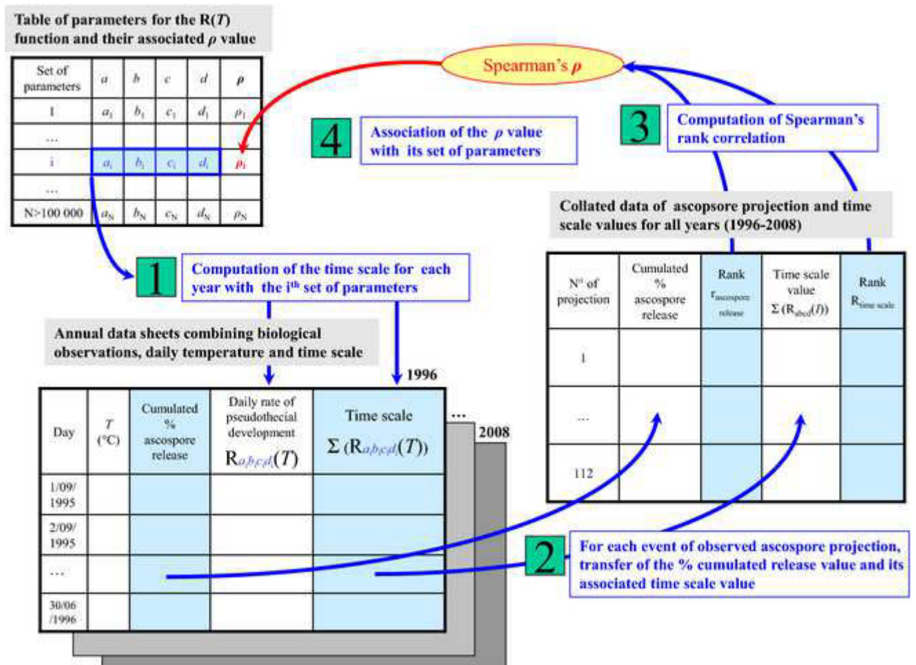
Figure 2. Algorithm showing the four steps used for the computation of Spearman's \rho for each set of parameters tested for the R(T) function describing the daily rate of pseudothecial maturation.
