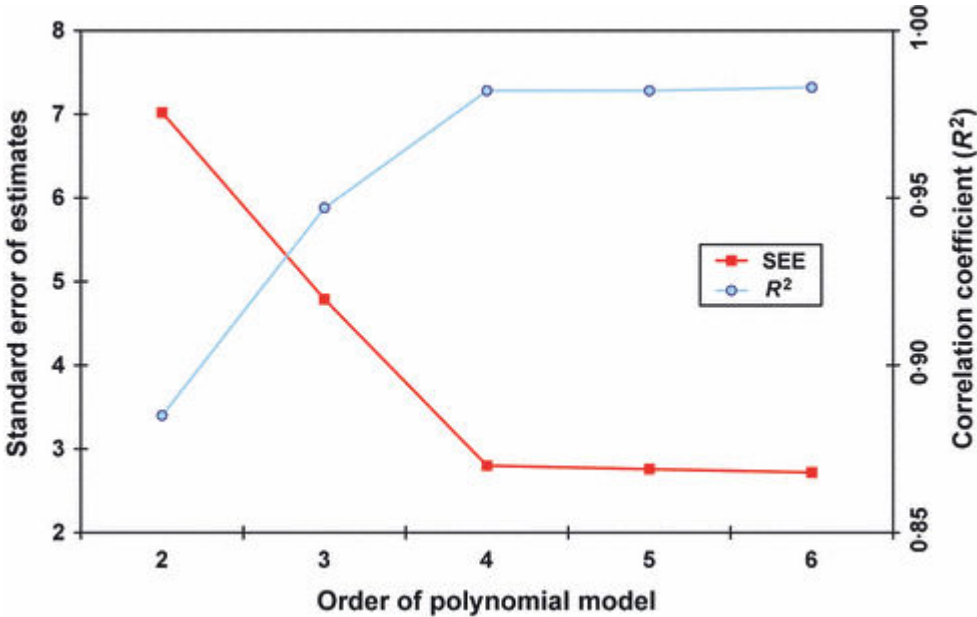
Figure 4. Relationship between goodness-of-fit indicators and the order of polynomial models relating the duration of olive peacock leaf spot ( Fusicladium oleagineum ) latent period as a function of air temperature.
