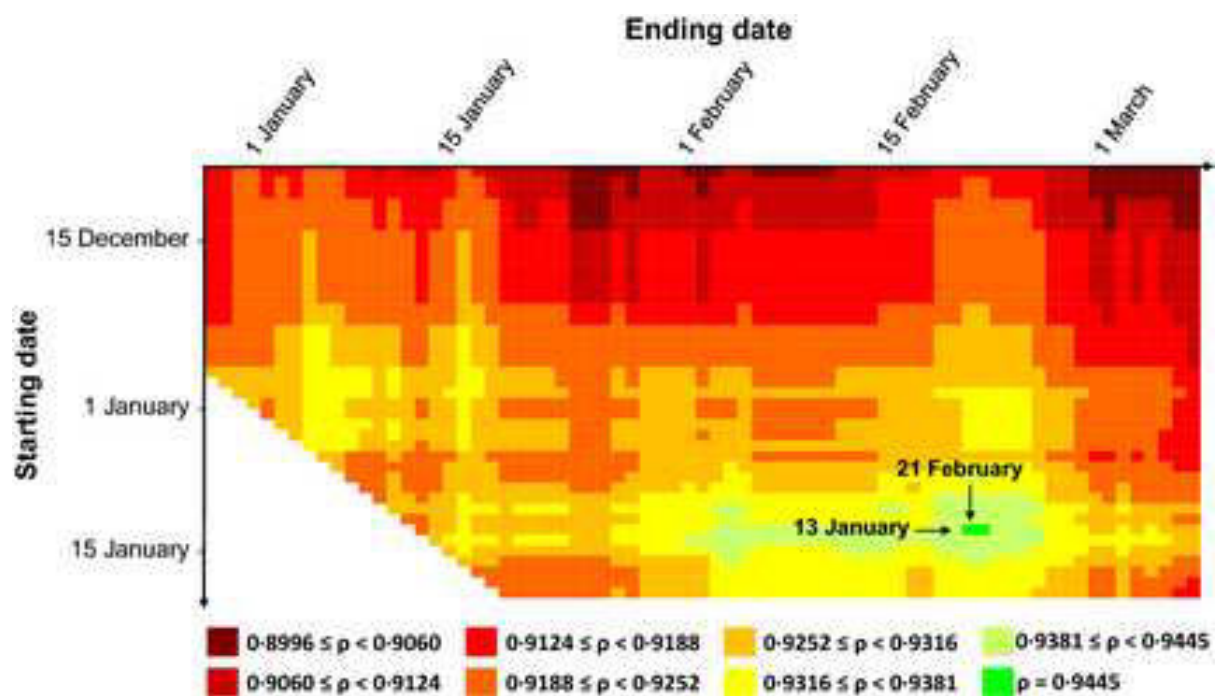
Figure 8. Optimization of the starting and ending dates for the rain-recording period in the rABCD thermal time scale. For each pair of dates, the p value is shown, evaluating the relationship between the time scale and the cumulated percentage of released ascospores in Avignon, France between 1996 and 2008.
