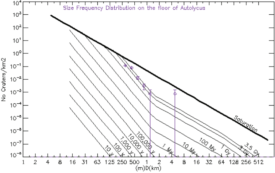
Figure 5.13: Size frequency distribution of Autolycus.
