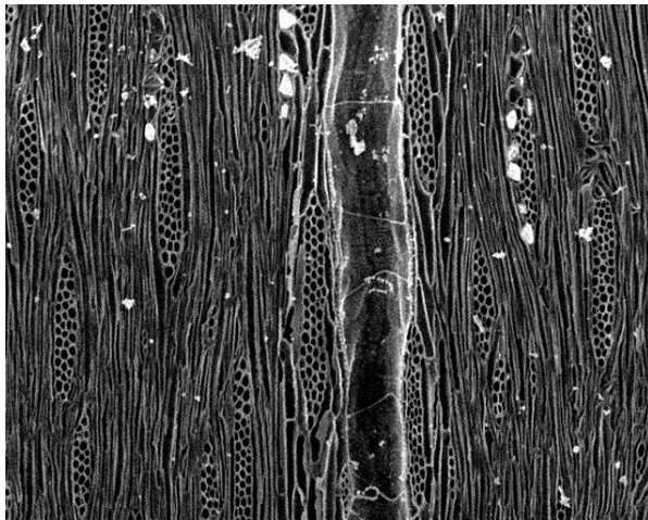
Vac-High PC-Std. 10 kV x 200 100 \mu m
