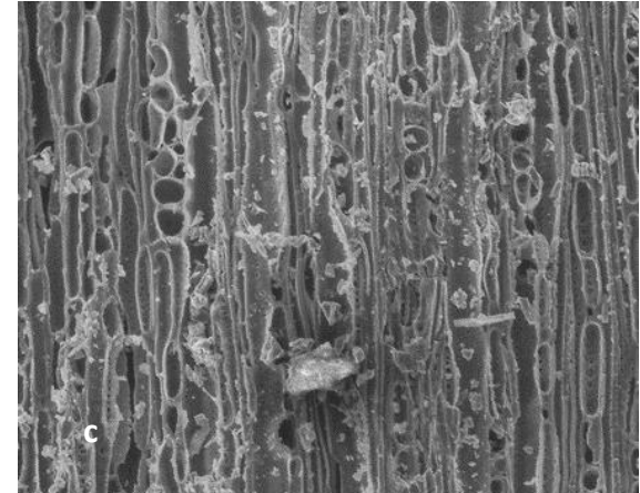
Vac-High PC-Std. 10 kV x 400 50 μm
