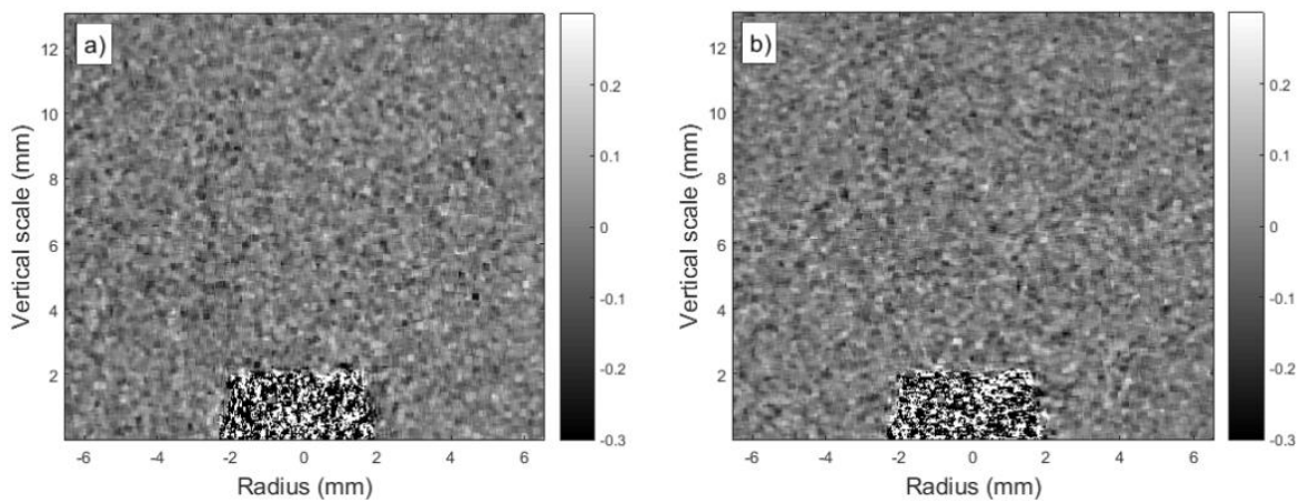
Figure 4-21: Mean horizontal displacement (a) and RMS displacement (b) in pixels for ten reference images [103].
