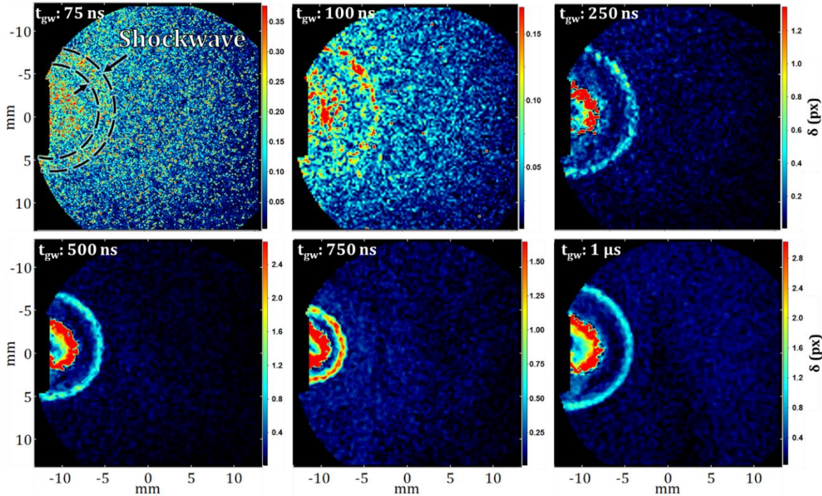
Figure 5-38: Displacement fields with initial hot kernel and shockwave, for different acquisition gate widths.
