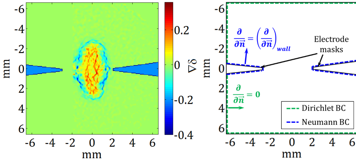
Figure 4-10: Displacement divergence field (left), with masked electrodes in blue, and boundary conditions applied to the displacement divergence field (right).
