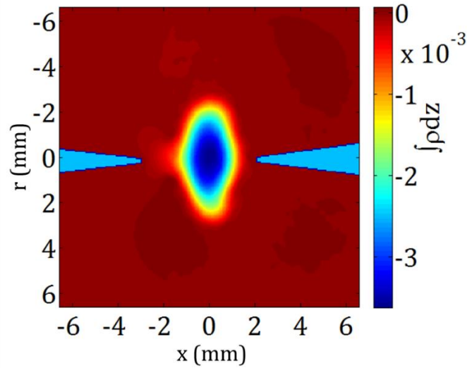
Figure 4-11: Integrated density field by integration of the Poisson equation.
