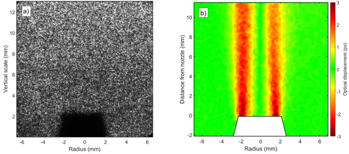
Figure 4-19: CO 2 jet SBOS images. Example of reference image under no-flow conditions (a) and mean displacement magnitude field in pixel (b), in each case the radius is the distance from the center of the nozzle [103]
