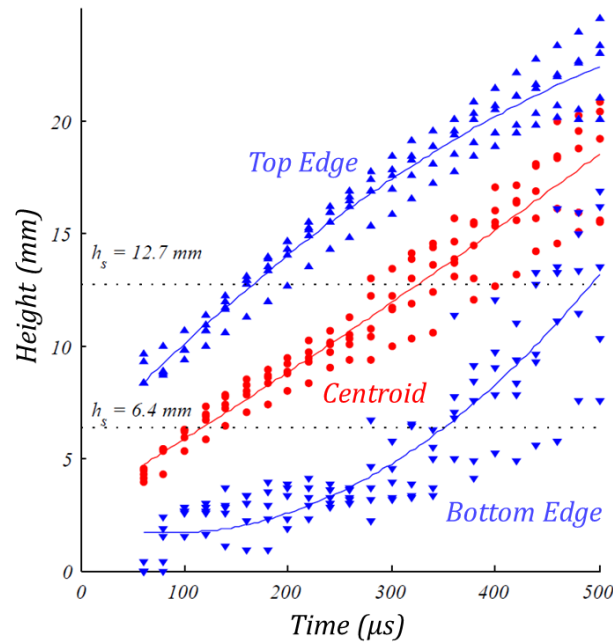
Figure 5-26: Kernel location heights from wall at different times for five kernel events [124].
