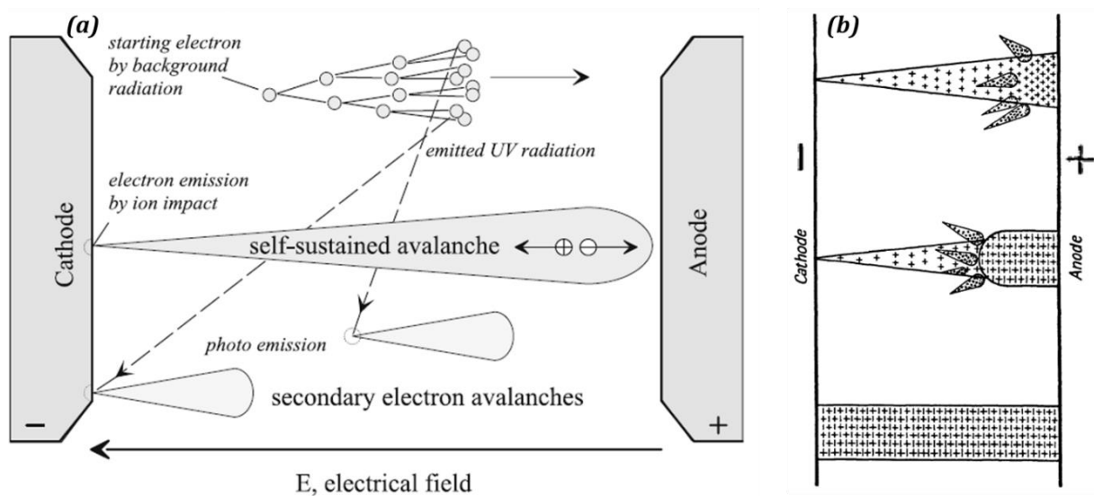
Figure 1-2: Formation of a primary electron avalanche (a) and transition electronic avalanche - positive streamer - conductive channel (b) [5] [8].
