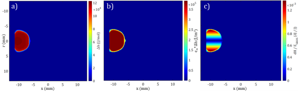
Figure 5-30: SBOS energy calculation: a) molar enthalpy, b) enthalpy per unit of volume, c) total enthalpy planar distribution.
