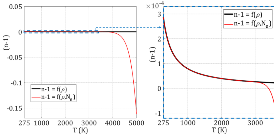
Figure 4-8: Influence of electronic density on the refractive index-temperature relation in air.
