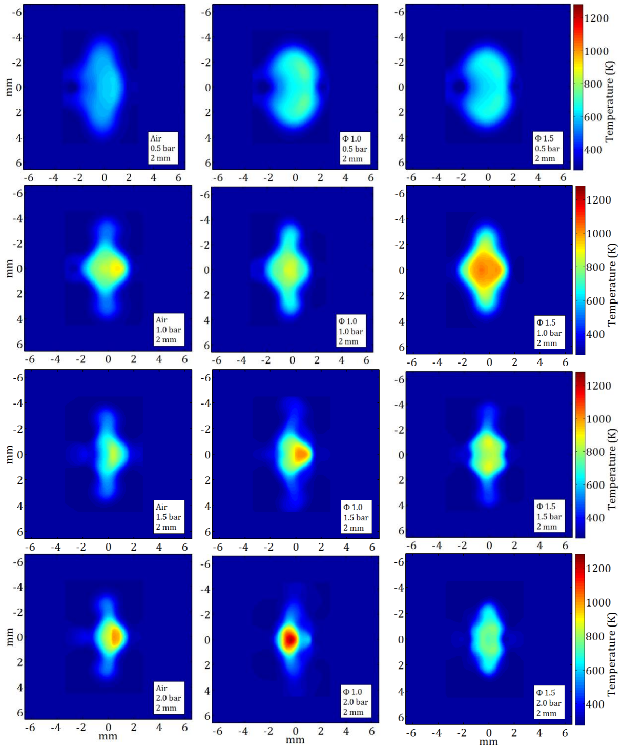
Figure 4-40: Temperature fields for different gases and pressures, 2 mm gap. From left to right: air, C_3H_8-N_2 at \Phi_{eq}=1.0 and C_3H_8-N_2 at \Phi_{eq}=1.5 . From top to bottom, pressure from 0.5 to 2 bar.
