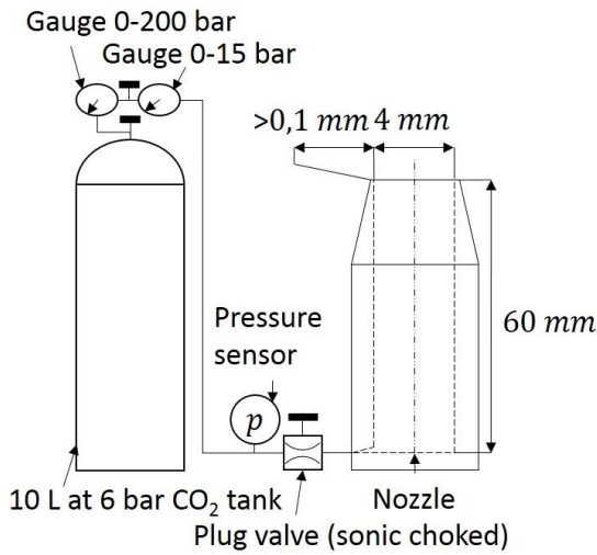
Figure 4-18: CO 2 jet setup scheme (left) [103] and picture of the exit nozzle (right).
