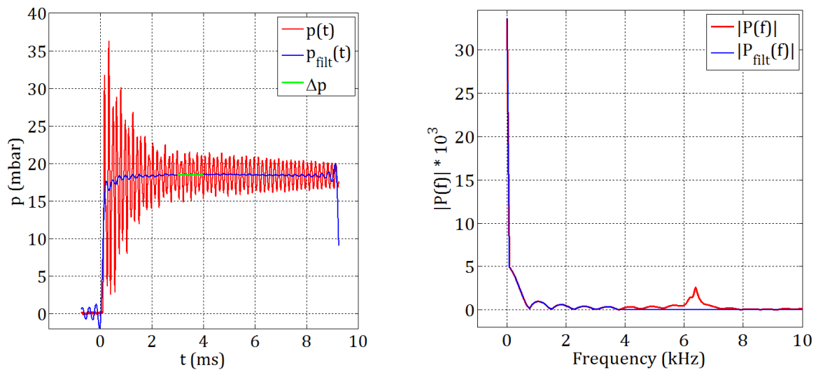
Figure 5-7: Pressure signal, pressure filtered by Fourier low pass at 4 kHz, and the averaged final pressure (left). Amplitude spectrum of the signal and filtered spectrum (right).
