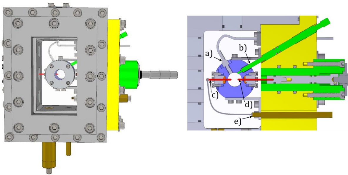
Figure 2-5: Pressurized ensemble 3D view (left), and transversal cut (right). (blue) 6 ml inner volume chamber, a) differential pressure transducer, b) by-pass valve, c) ground electrode (red), d) high V electrode attached to millimetric positioner, e) electric ground.
