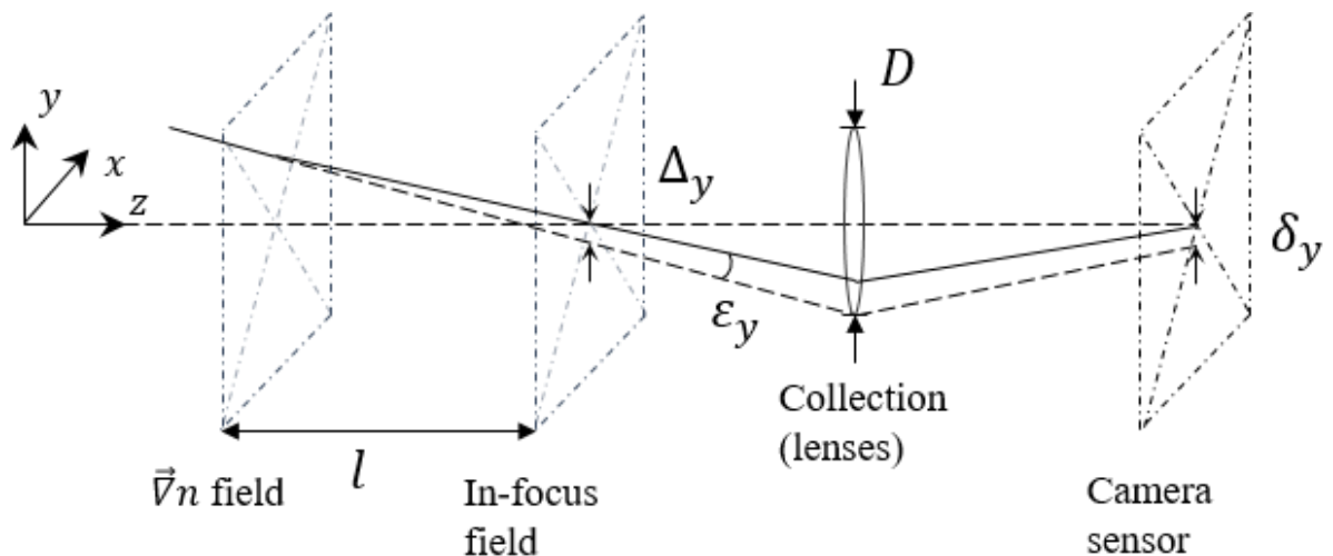
Figure 4-2: Geometry of SBOS configuration with negative focus to subject field distance [103]
