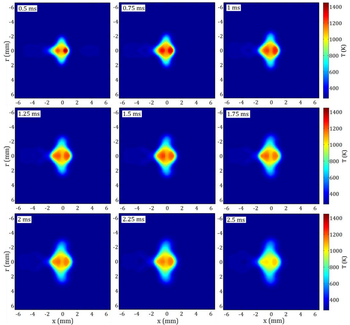
Figure 4-28: Temperature fields averaged for 10 tests, 0.5 to 2.5 ms after discharge onset, 2 mm gap.
