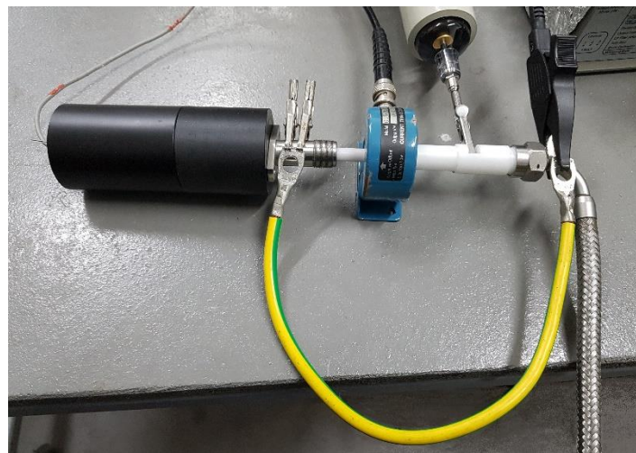
Figure 5-14: Atmospheric test with aeronautical igniter in a 60 ml chamber.
