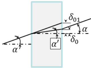
Figure B-1: Window influence on optical path (refraction)
