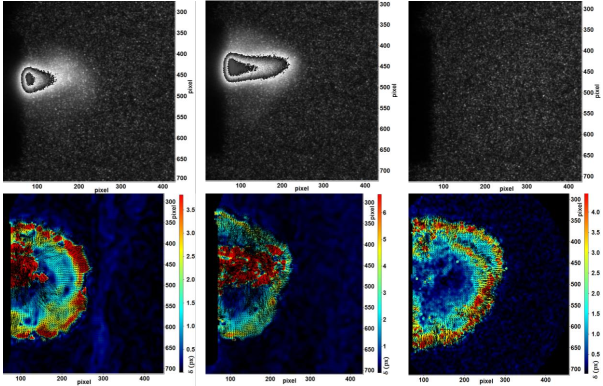
Figure 5-21: SBOS tests images without filter (left), with the low-pass filter (middle) and the interferometric filter (right). On the bottom row, the corresponding displacement fields from cross-correlation processing.
