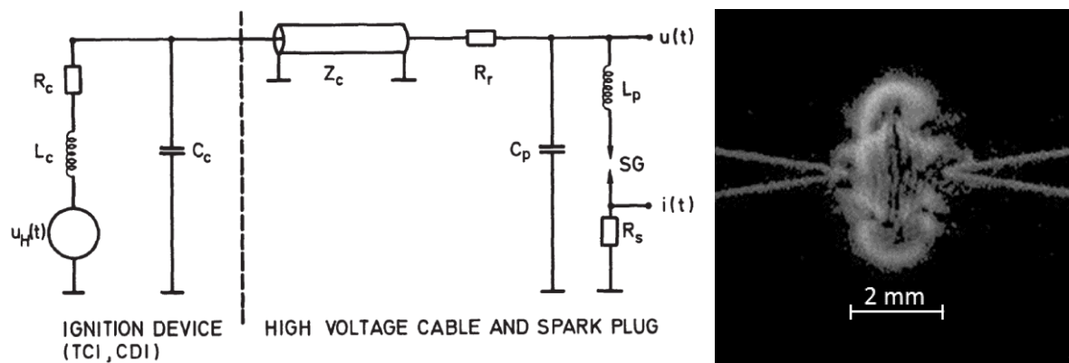
Figure 2-1: Schematic equivalent circuit of technical ignition systems[2] and schlieren image of a pin-to-pin electrodes discharge with TCI circuit and a 2 mm inter-electrode gap.
