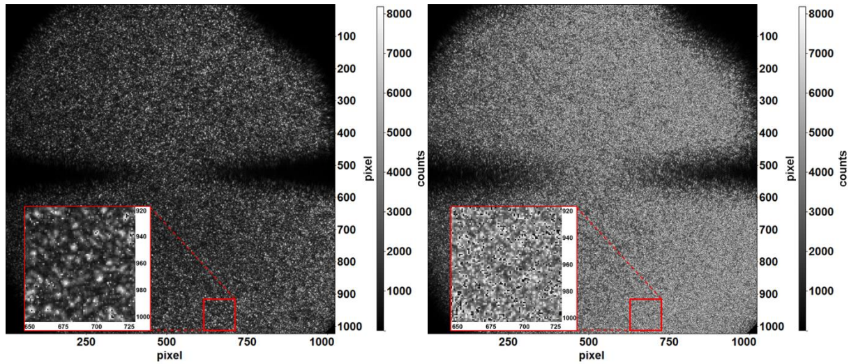
Figure 4-4: Different speckle backgrounds for different diaphragm opening diameters: 6 mm (left) and 10 mm (right). Pin-to-pin electrodes with 1 mm gap, at 2 bar with defocus distance l = -80 \text{ mm} .
