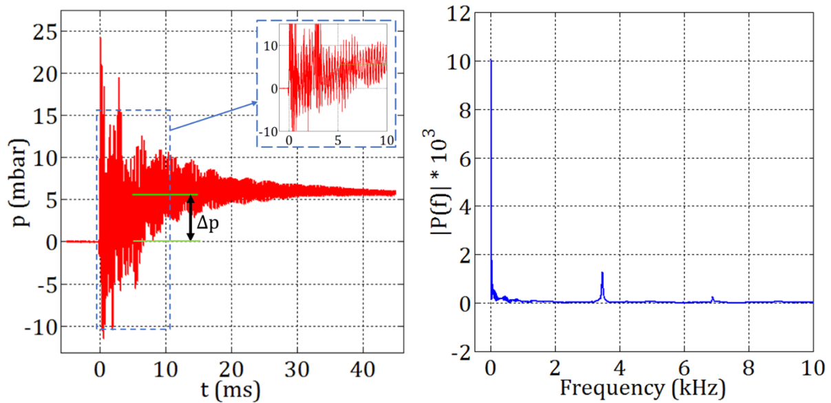
Figure 5-4: Differential pressure signal from an aeronautic igniter discharge in a 63 ml chamber (left) and its single-sided amplitude spectrum from the Fourier transform (right).
