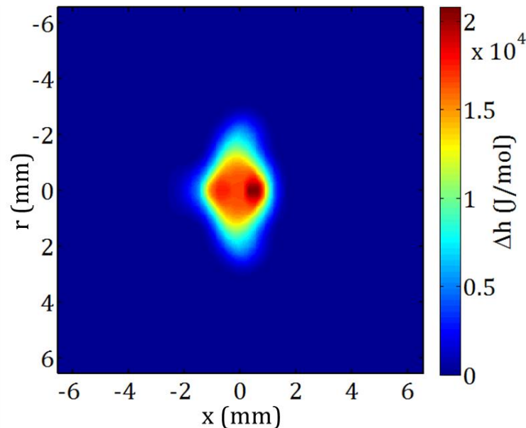
Figure 4-15: Local enthalpy, \Delta h(T) , in J/mol
