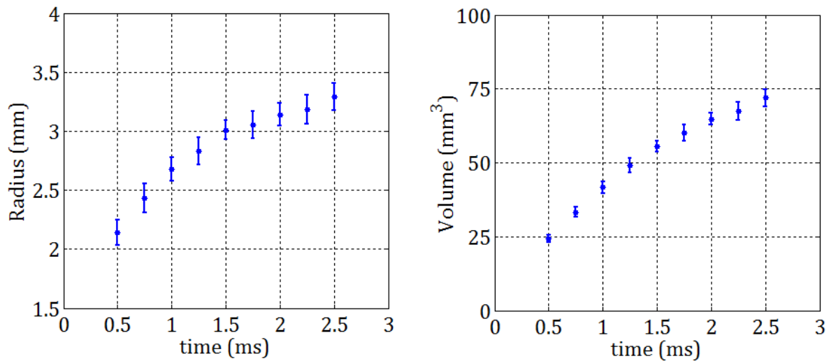
Figure 4-30: Kernel maximum radius (left) and kernel volume (right) from 0.5 to 2.5 ms after the discharge onset for a 2 mm gap.
