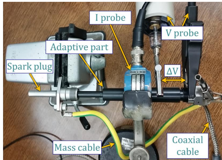
Figure 5-2: Ardiden 3 spark plug and connector adaptive part.
