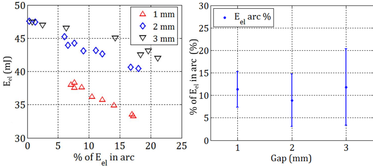
Figure 3-15: Arc phase energetic contribution (fraction of the electrical energy supplied in arc phase). On the left, E_{el} versus E_{el} % in arc mode; on the right, E_{el} % in arc mode for different gaps.
