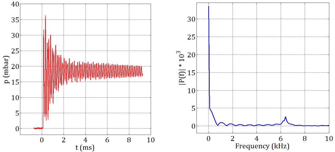
Figure 5-6: Differential pressure signal (left) and single-sided amplitude spectrum of p(t) .
