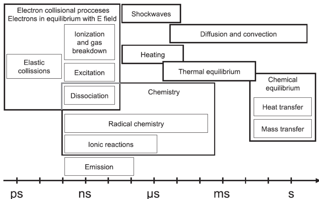
Figure 1-4: Timescales of relevant collisional and transport processes in atmospheric pressure plasmas for a pulsed breakdown discharge [14].
