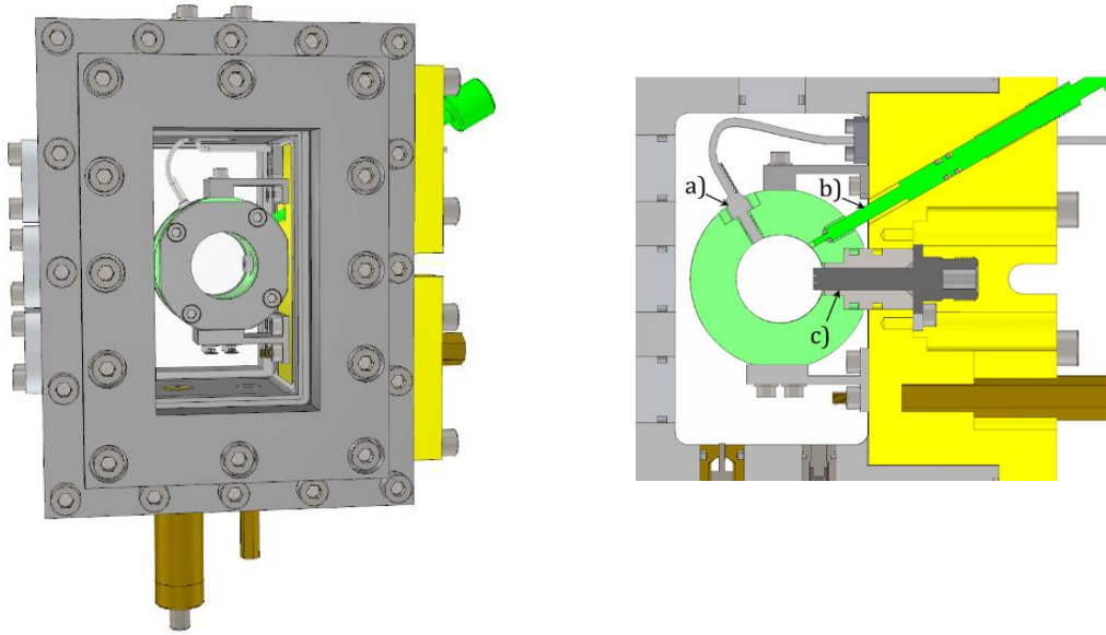
Figure 2-6: Pressurized ensemble 3D view (left), and transversal cut (right). (light green) 20 ml inner volume chamber wall, a) pressure transducer, b) by-pass valve, c) helicopter spark plug.
