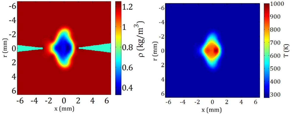
Figure 4-13: Density field obtained by backprojection and masked electrodes (left). Corresponding temperature field (right).
