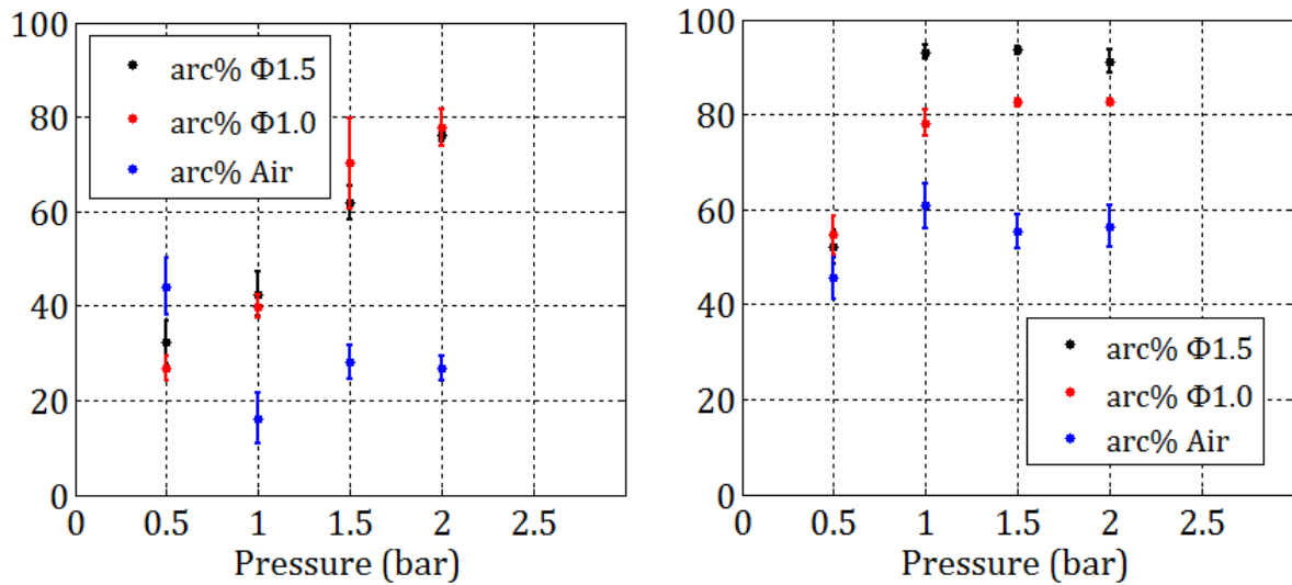
Figure 3-26: Arc phase fraction of total E_{el} vs pressure for different mixtures, at 1 mm (left) and 2 mm (right) gap.
