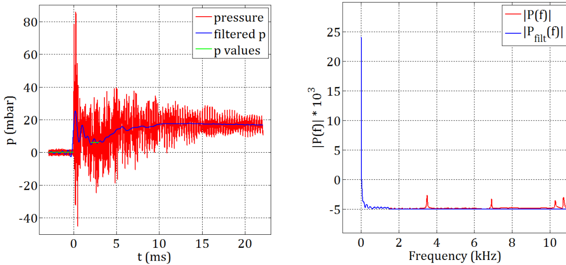
Figure 5-16: Pressure rise for a Eyquem igniter discharge in red (left); filtered using a low-pass Fourier transform, in blue; and final pressure rise (green). On the right, single-sided amplitude spectrum in red and filtered spectrum in blue.
