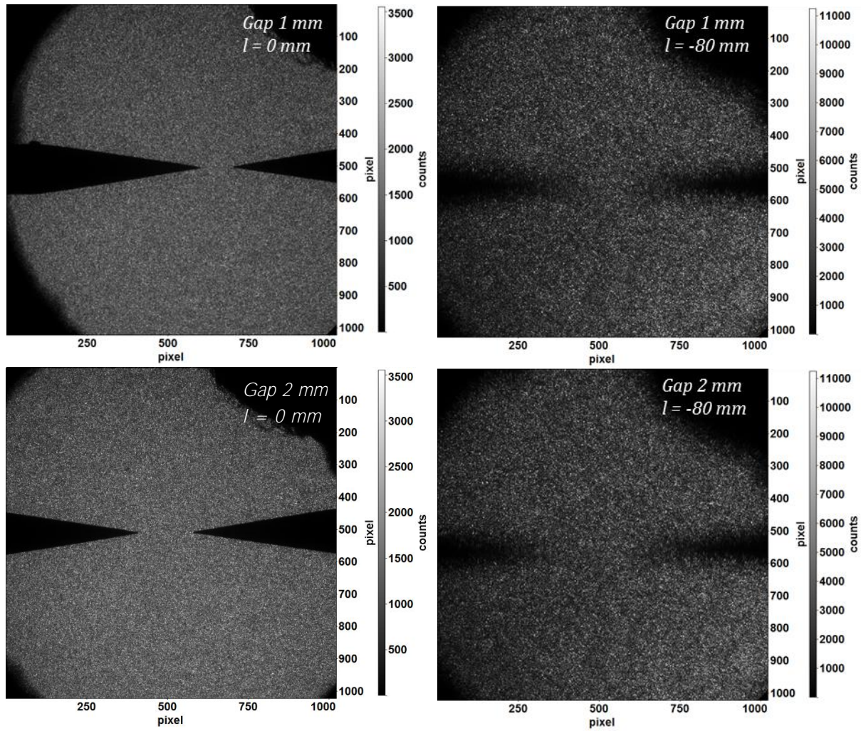
Figure 4-5: Effect of defocus distance on speckle and background elements. Top, 1 mm gap, bottom, 2 mm gap. Left, electrodes in the focal plane ( l = 0 mm), Right: defocus l = -80 mm (further from the camera). Focused image: calibration, gate width 1 ms, low laser power ( \sim 0.5 W). Defocused: test conditions, maximum laser power (3 W), gate width 1 \mu s.
