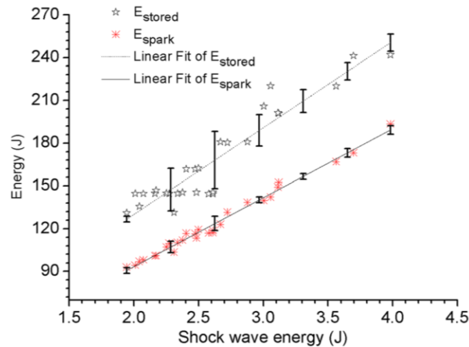
Figure 1-11: Variations in E_C and E_{el} with Shock wave energy E_{sw} (for a capacitance C_{100J}=3.998 \mu F ) [73]
