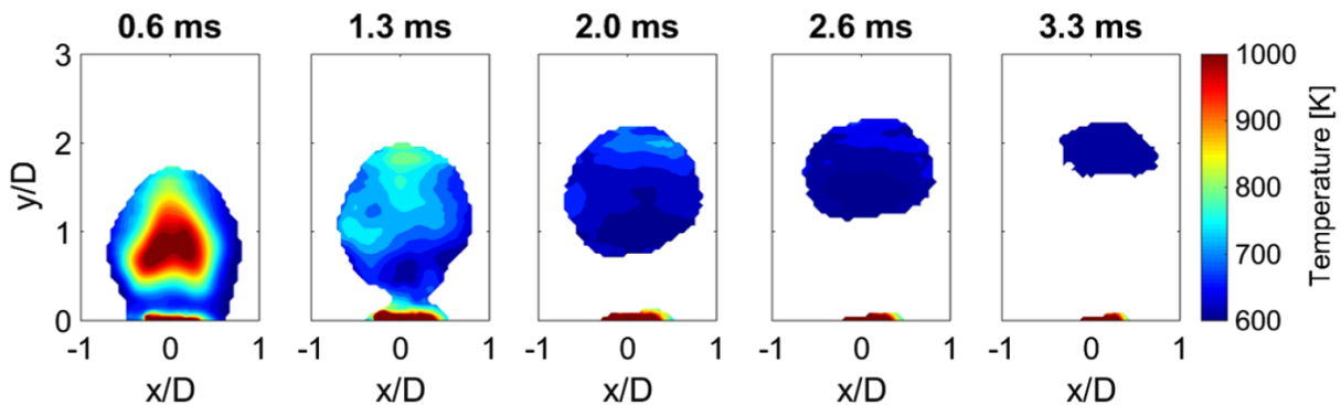
Figure 1-16: Phase averaged temperatures for the sunken igniter discharge kernel in air[19]
