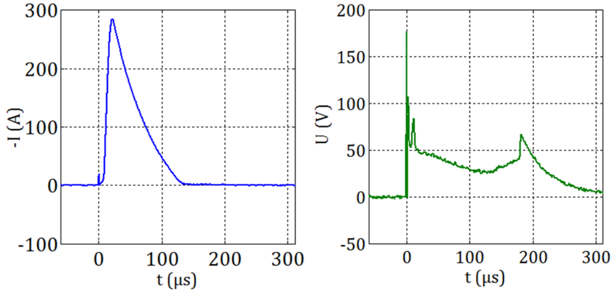
Figure 5-9: Electrical signals: Intensity (inversed, left) and Voltage (right).
