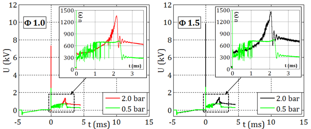
Figure 3-25: Voltage at 0.5 and 2 bar for a 2 mm gap in C_3H_8-N_2 at \Phi = 1.0 (left) and \Phi = 1.5 (right).
