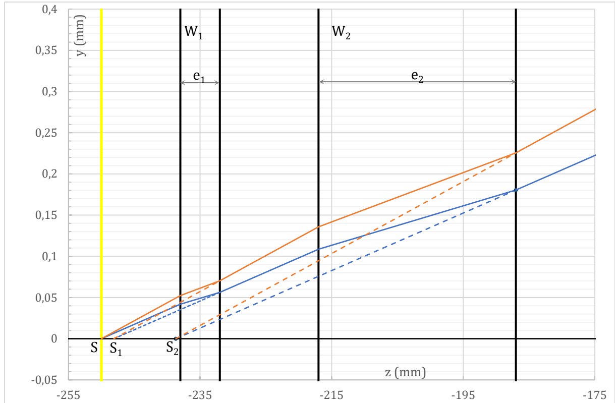
Figure B-5: Detail of window influence on light beams, zoomed at the window passage. Dashed lines represent virtual projections.
