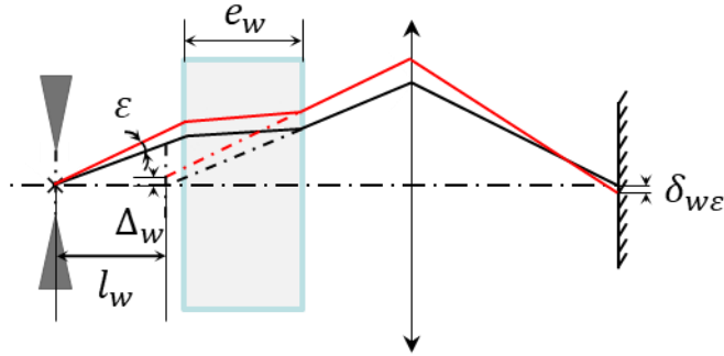
Figure B-3: Window effect on optical path after angle deviation
