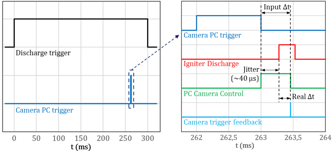
Figure 5-19: Camera and discharge control synchronization. Signals generated by the delay generator (left) and camera-discharge events synchronization (right).
