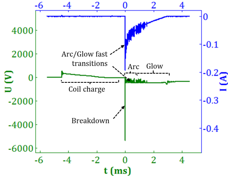
Figure 3-2: Electrical signals for a 1 mm gap and E_{el} = 39 mJ.
