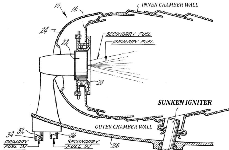
Figure 1-15: Gas Engine combustion chamber and sunken igniter [97]
