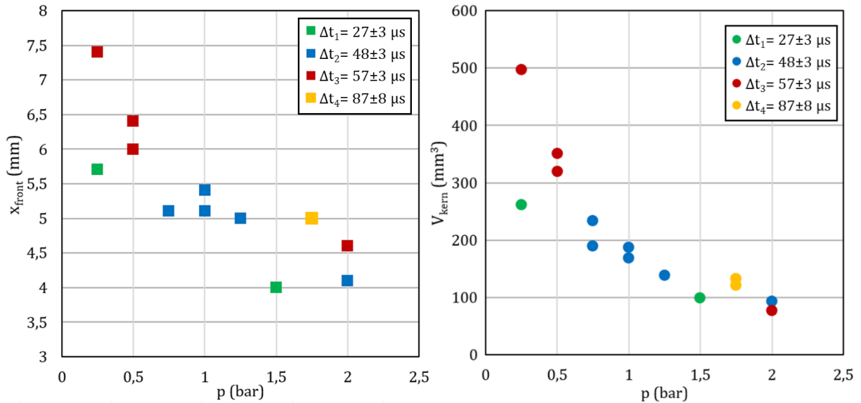
Figure 5-37: Kernel front penetration length and kernel volume versus pressure, at iso- \Delta t .
