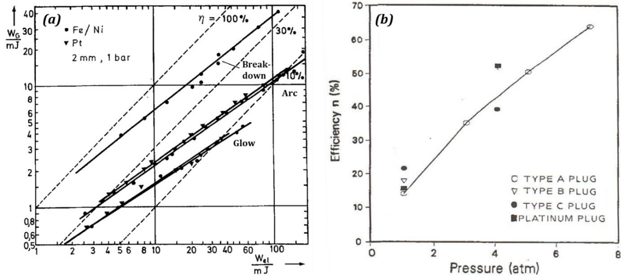
Figure 1-10: Electrical discharge efficiency for the three discharge modes (a)[12] and for different pressures (b)[62].
