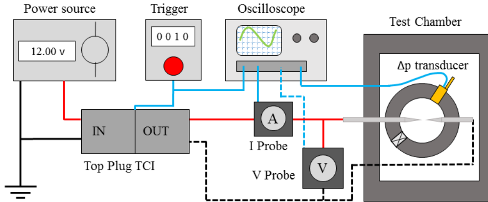
Figure 2-7: Pressure-rise calorimetry experimental setup.
