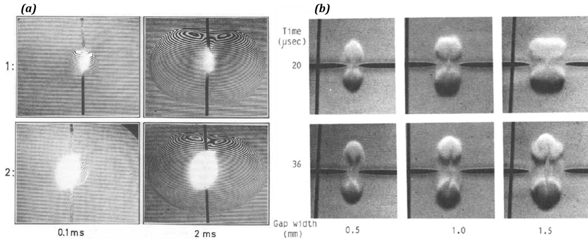
Figure 1-12: Interferograms of differently activated volumes in CH 4 -air mixture at 4 bar, where 1: 3 mJ CDI and 2: 3 mJ CDI + 30 mJ arc (a)[5]; and Schlieren photographs of spark kernels in air for different gaps and a 4.6 mJ discharge (b)[78].
