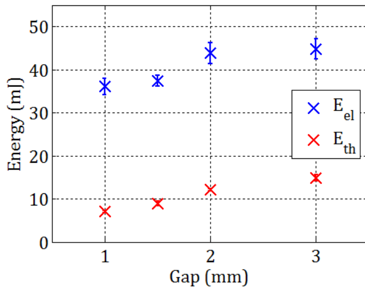
Figure 3-9: Thermal energy and electrical energy for different gap distances. E_{th} increases with gap distance.
