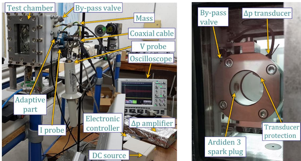
Figure 5-5: Calorimetry setup adapted to the Ardiden 3 engine igniter (left) and detail on the 20 ml chamber (right).
