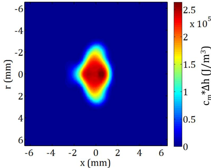
Figure 4-16: Enthalpy variation per unit of volume, c_m(T) \cdot \Delta h(T)
