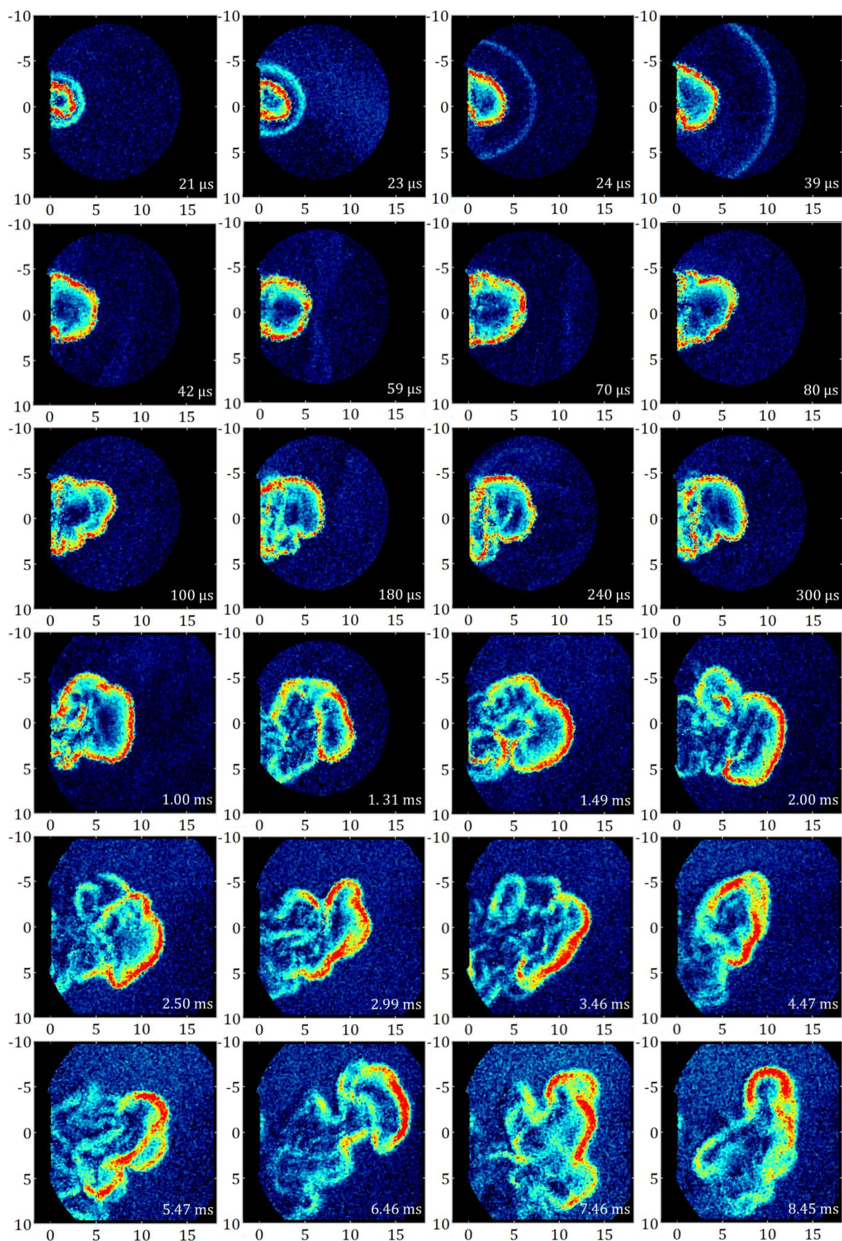
Figure 5-25: Helicopter igniter discharge kernel evolution, as SBOS \delta fields with \Delta t from 21 \mu\text{s} to 8.45 ms. Each image correspond to a different test.
