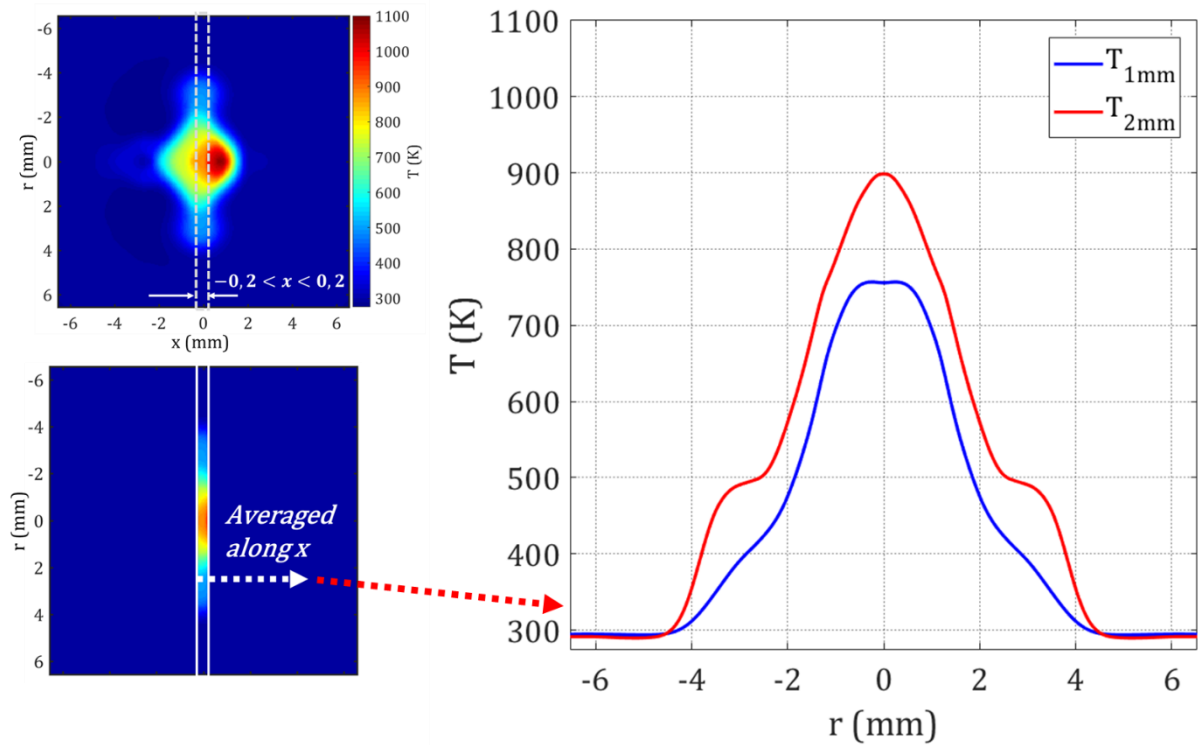
Figure 4-25: Temperature profiles along kernel diameter for 1 mm and 2 mm gap and at \Delta t of 3.0 and 2.9 ms respectively, averaged over a 0.4 mm band.
