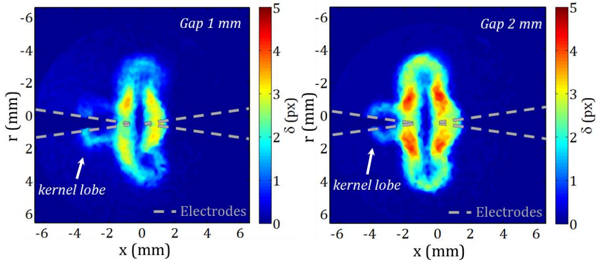
Figure 4-23: Displacement fields for 1 and 2 mm gap (left and right, respectively) at the end of the discharge averaged for each set of tests. In air at 1 bar. \Delta t = 3.0 \text{ ms} (1mm), 2.9 \text{ ms} (2 mm).
