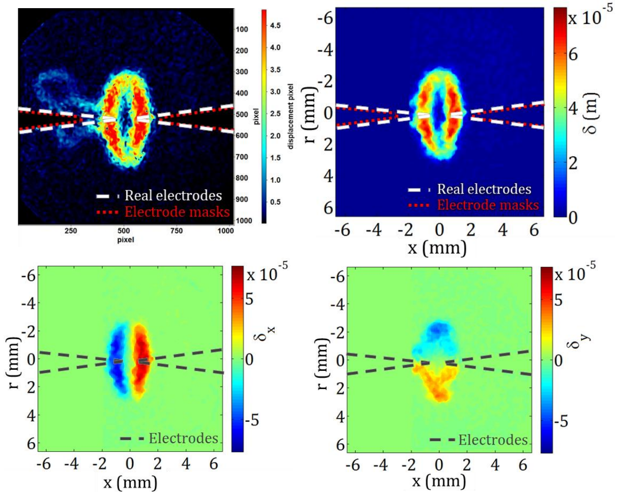
Figure 4-7: Displacement fields: (a) Original scalar \delta field, (b) \delta filtered and re-scaled, (c) \delta_x , (d) \delta_y
