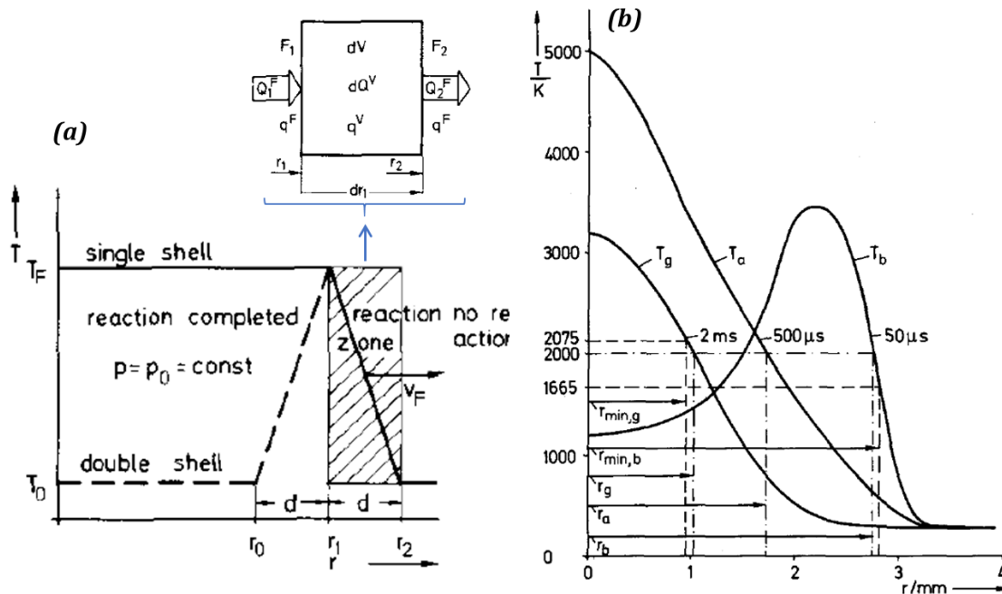
Figure 1-8: Thermal model of the plasma outer shell-reaction zone (a) and radial temperature profiles for three ignition devices at the indicated points of time after spark onset in methane-air (b)[48]. In (b), T_b = 30 mJ breakdown in 60 ns; T_a = CDI with 3 mJ for 100 \mu s + 30 mJ in arc for 230 \mu s, and T_g = 3 mJ for 100 \mu s + 30 mJ glow for 770 \mu s.
