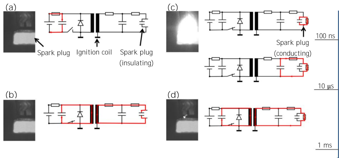
Figure 1-5: Events during spark discharge for a CDI. Timeline applies to breakdown and arc-glow phases (c and d). [15]
