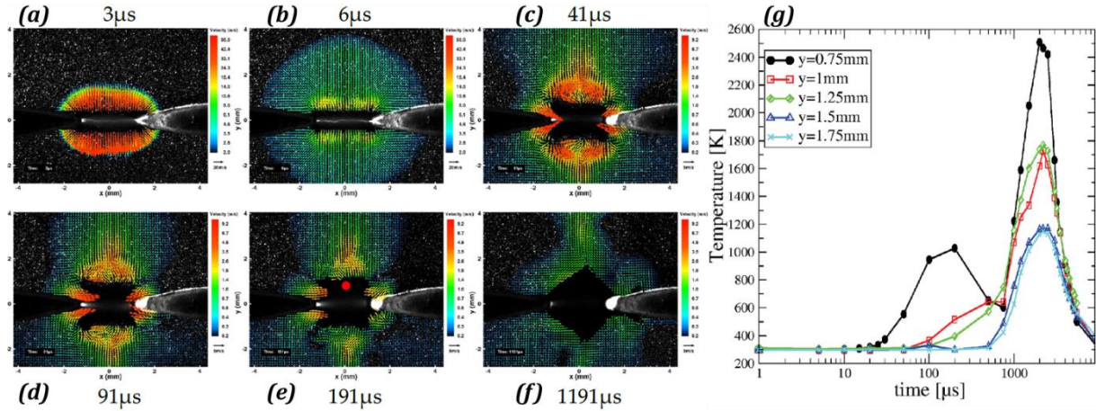
Figure 1-14: Gas velocity fields surrounding the spark after breakdown in quiescent air measured by PIV (a-f) and temperature evolution with time along a vertical profile in the center plane measured by SRS (g); all from [87].
