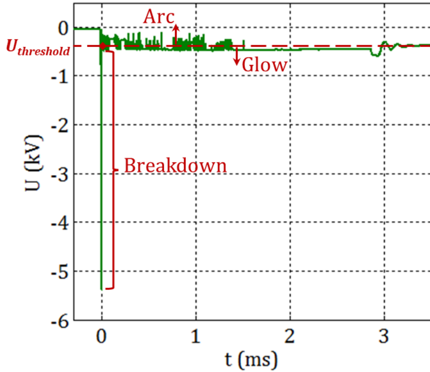
Figure 3-13: Voltage signal with voltage threshold and discharge phase detection.
