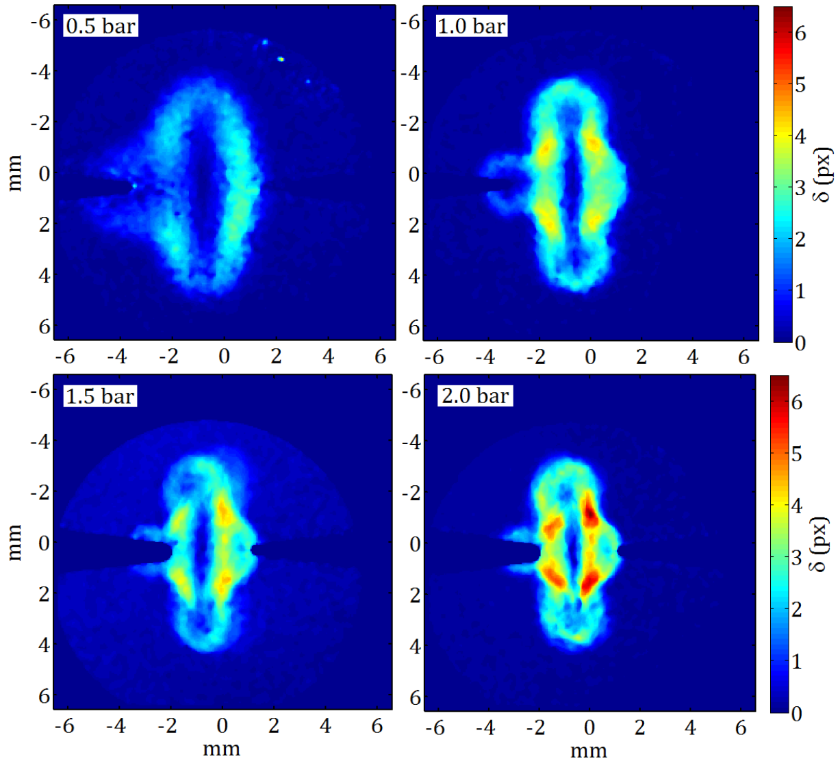
Figure 4-33: Averaged displacement field for 0.5, 1.0, 1.5 and 2 bar in air and a 2 mm gap.
