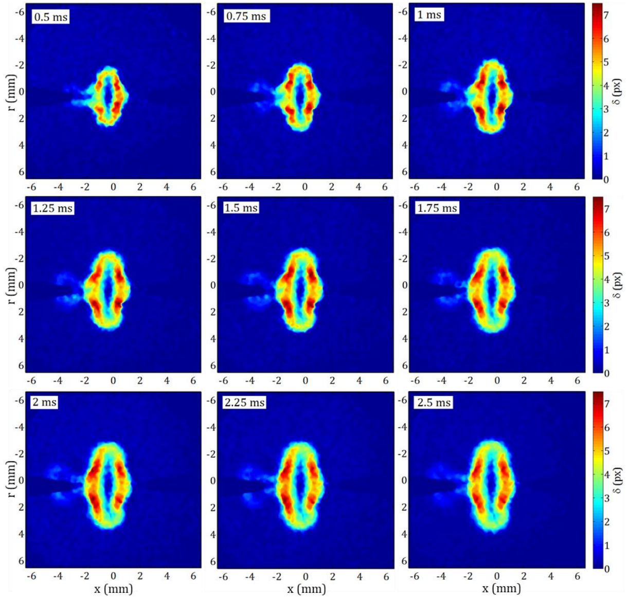
Figure 4-27: Displacement fields averaged from 10 tests, for \Delta t = 0.5 to 2.5 ms from left to right and top to bottom, 2 mm gap.
