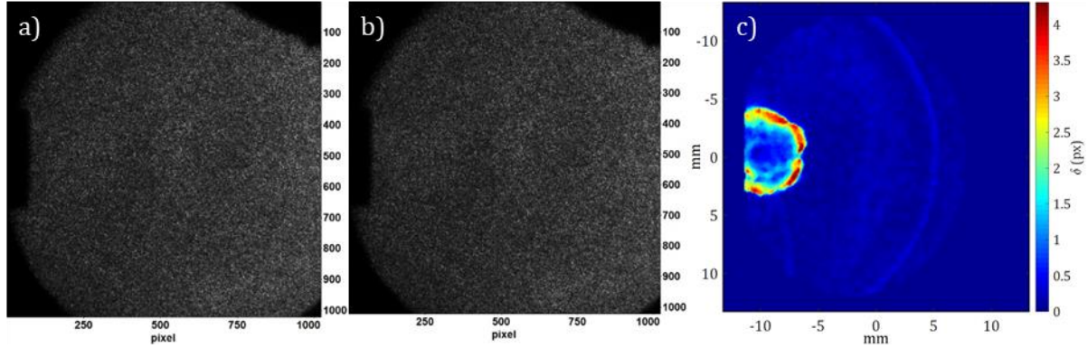
Figure 5-27: SBOS test in atmospheric conditions: a) reference image, b) test image, c) displacement field.
