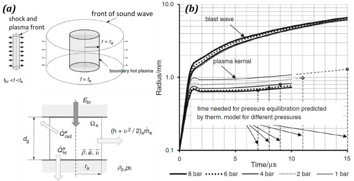
Figure 1-9: Thermodynamic model used by Meyer [15](a) and temporal evolution of plasma and blast wave radii at different pressures together with time needed for pressure equilibration [15], [61](b)
