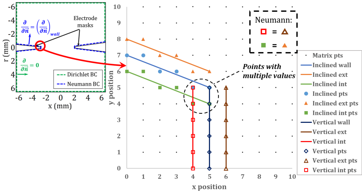
Figure C-3: Neumann BC applied to a corner
