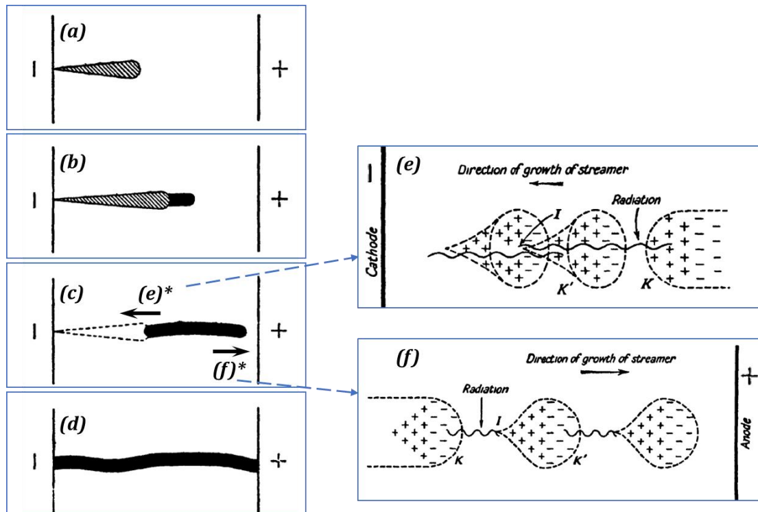
Figure 1-6: Formation of a conductive channel voltage in excess of the minimum for breakdown: the electronic avalanche (a) produces a mid-gap streamer (b) which propagates towards the electrodes (c) forming the conductive channel (d). The streamer propagates towards the cathode as a positive streamer (e) and towards the anode as a negative streamer (f)[8].
