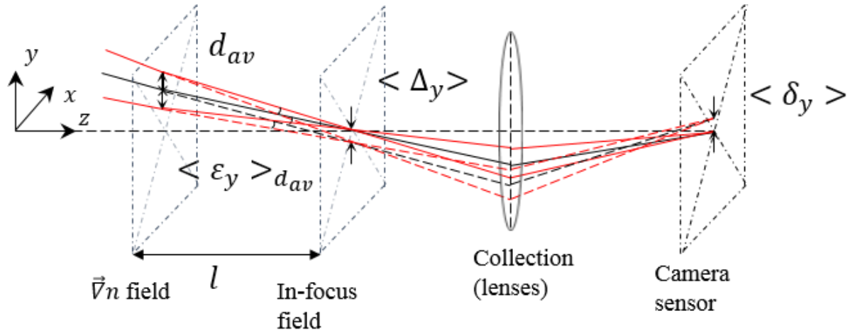
Figure 4-3: Scheme similar to Figure 4-2, where defocusing blur affected by ray tracing is added (in red). For simplicity of representation, \epsilon_y(x,y) for each ray is taken as an average ( \langle \rangle operator) \epsilon_y(x,y) over d_{av} resulting in an averaged \Delta y and averaged \delta y [103]
