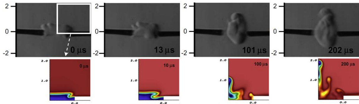
Figure 1-13: Images from high-speed schlieren visualization (upper row) and simulation (lower row) for a 2 mJ spark discharge in air with cylindrical electrodes [84].
