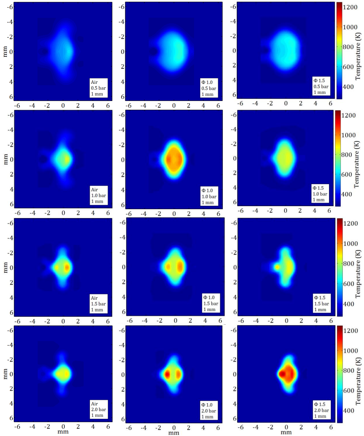
Figure 4-39: Temperature fields for different gases and pressures, 1 mm gap. From left to right: air, C_3H_8-N_2 at \Phi_{eq}=1.0 and C_3H_8-N_2 at \Phi_{eq}=1.5 . From top to bottom, pressure from 0.5 to 2.0 bar.
