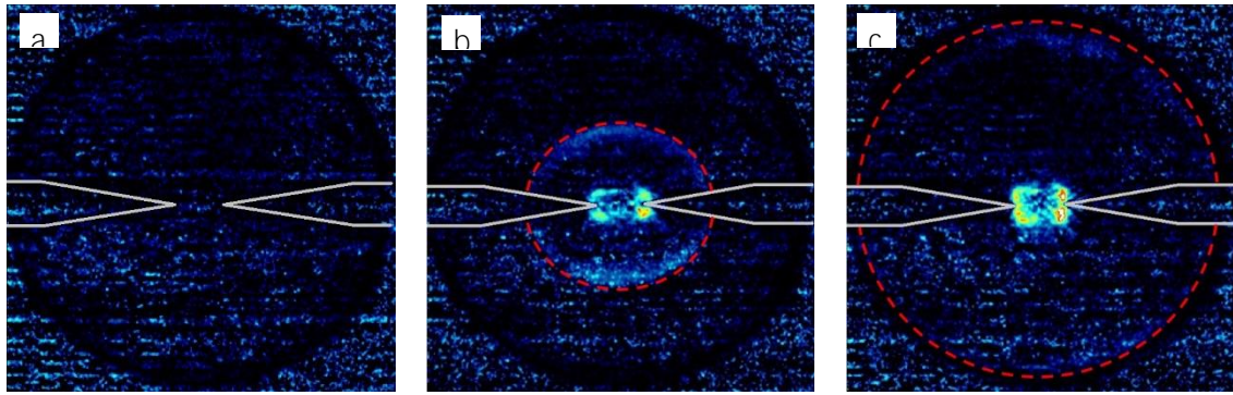
Figure 3-5: Schlieren images of the beginning of the discharge, filtered and after background subtraction, with dt = 11 \mu s . Electrodes position pointed out in grey, shockwave front in red. At (a.) discharge starts, shockwave is observed 11 \mu s later at (b.) and it has already bounced at the wall 11 \mu s later at (c).
