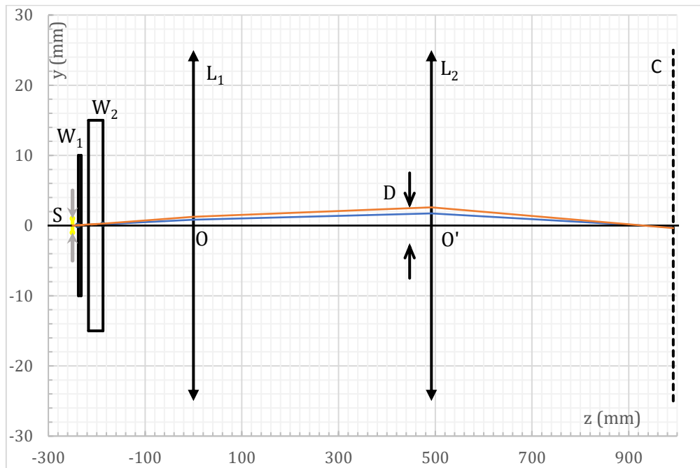
Figure B-4: Optical setup scheme for magnification M = -1 . Y and Z axis in mm, in different scales for a better visualization. In blue the reference light path and in orange the light path deflected an angle \varepsilon by the spark.
