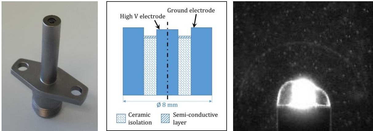
Figure 2-2: Ardiden 3 helicopter engine igniter spark plug (left), spark plug cutaway view (middle) and schlieren acquisition of an electrical discharge (right).
