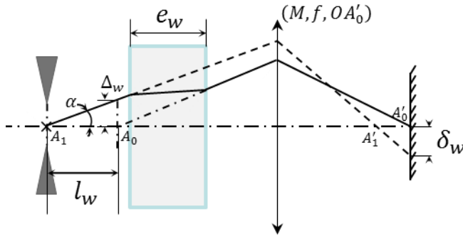
Figure B-2: Window influence on optical path and focal point
