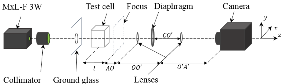
Figure 2-8: SBOS optical configuration.
