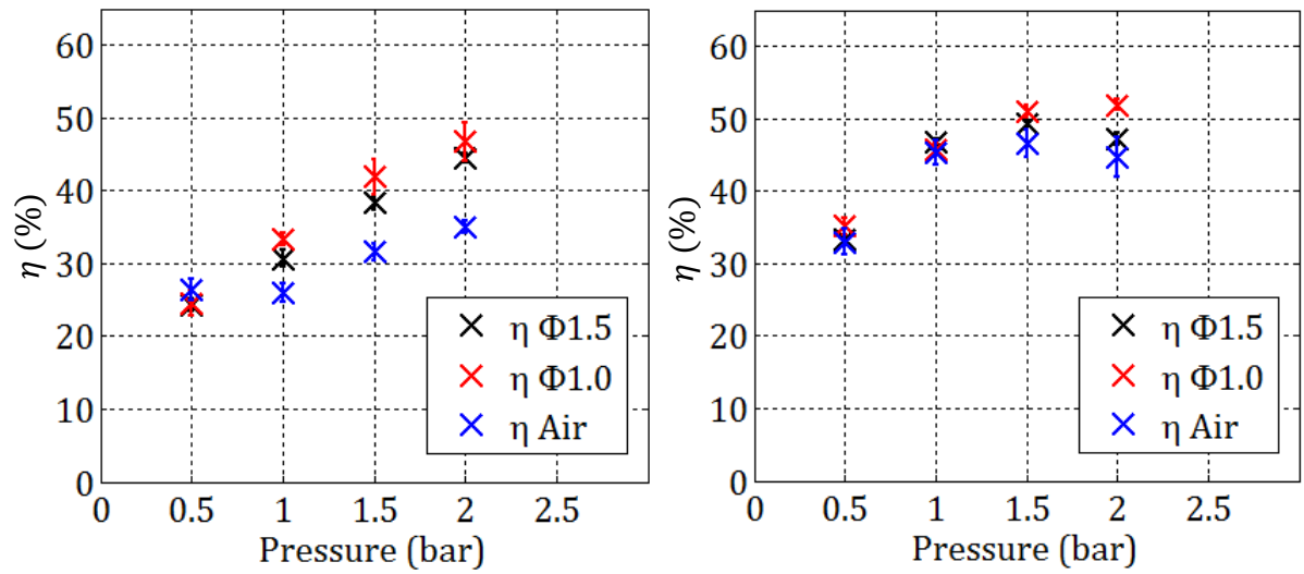
Figure 3-23: Efficiency vs pressure for different mixtures, at 1 mm (left) and 2 mm (right) gap.
