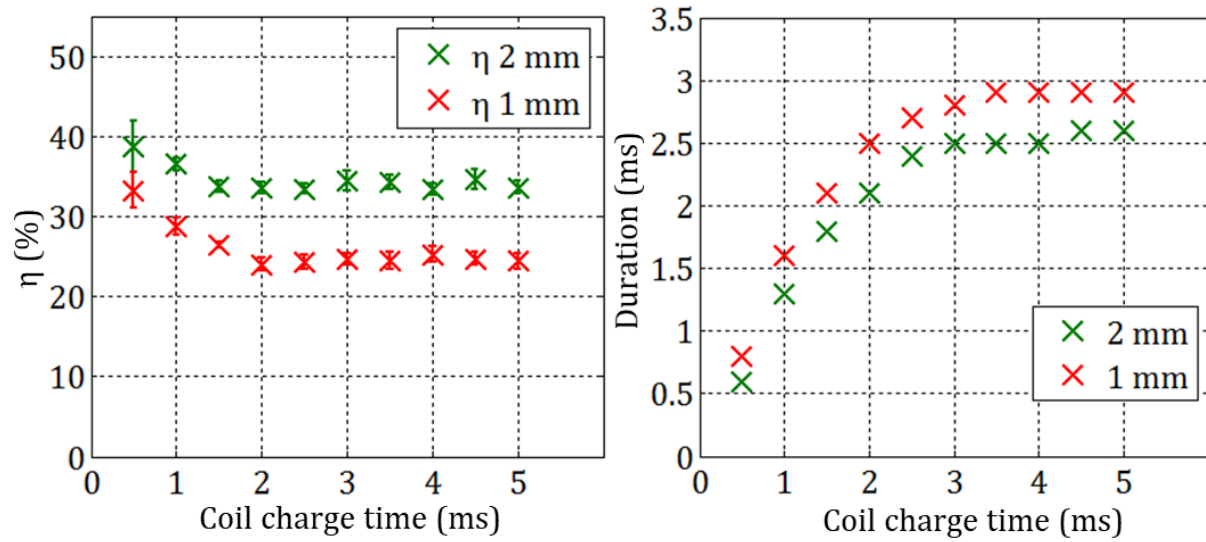
Figure 3-8: Efficiency \eta (left) and Discharge duration (right) versus coil charge time, for 1 and 2 mm gap.
