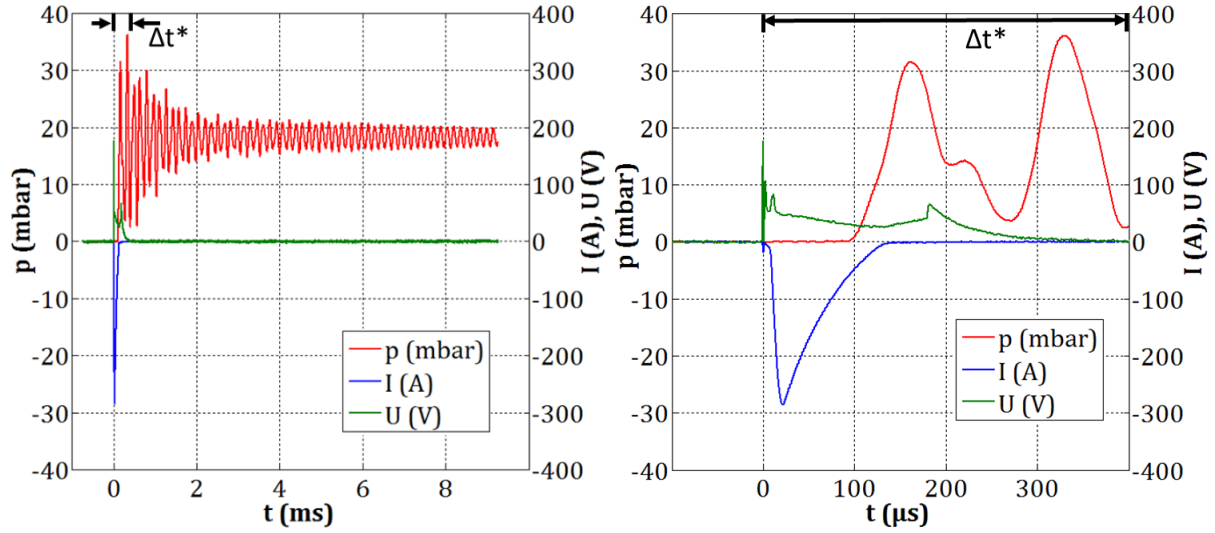
Figure 5-8: Pressure, intensity and current signals for the aeronautic igniter. Left: timescale of pressure registering. Right: timescale of the discharge duration.
