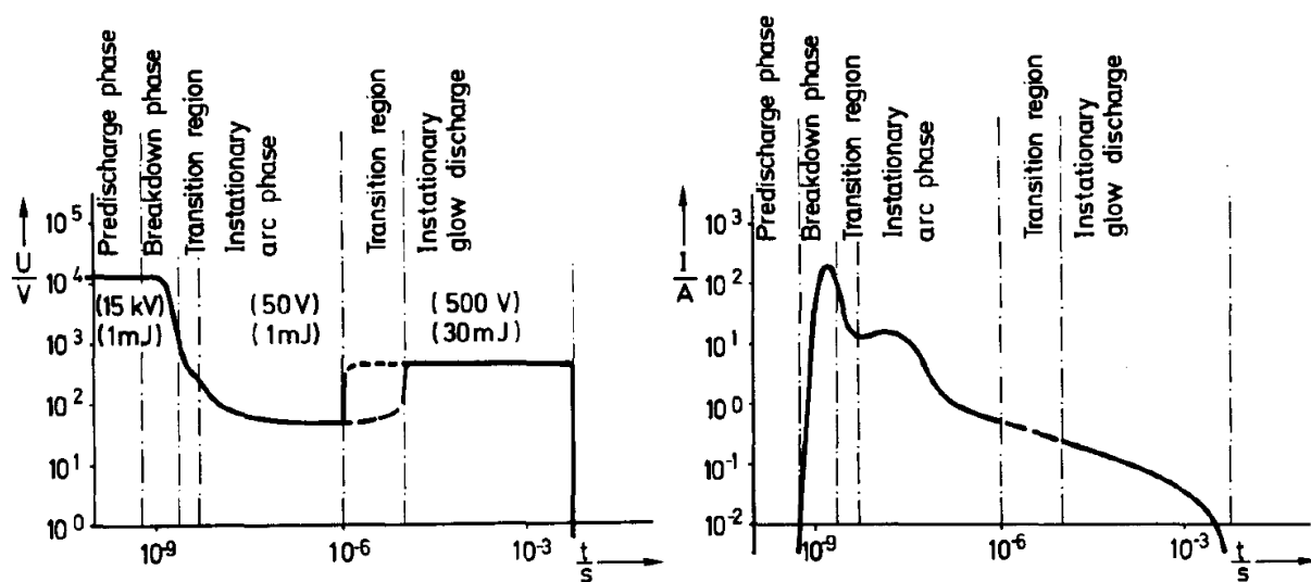
Figure 1-1: Voltage ( U ) and current ( I ) of technical ignition systems versus discharge time. Typical values are given in parentheses [5]
