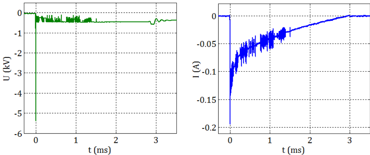
Figure 3-3: Voltage (left) and Intensity (right) during spark duration (from 0 to 3 \mu s in the precedent figure).
