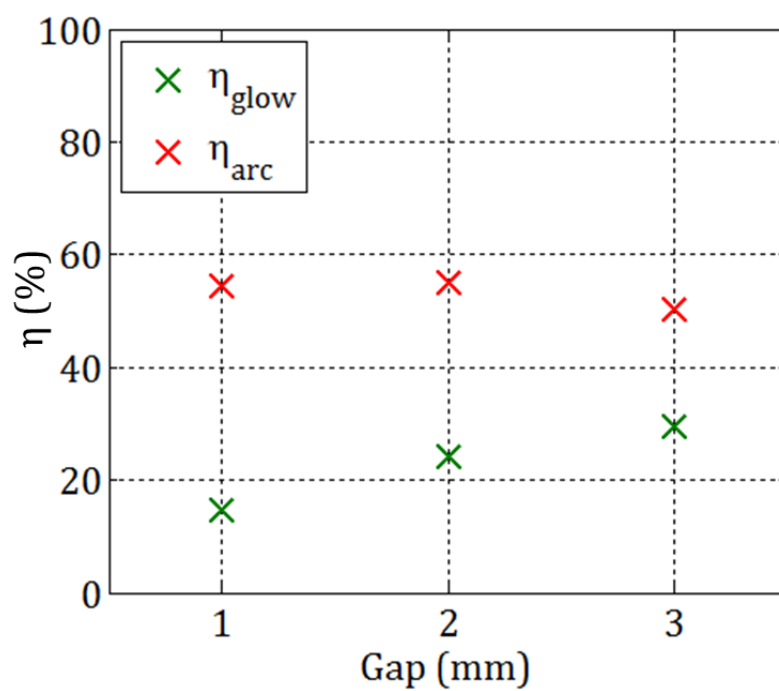
Figure 3-17: Arc and glow efficiencies versus gap.
