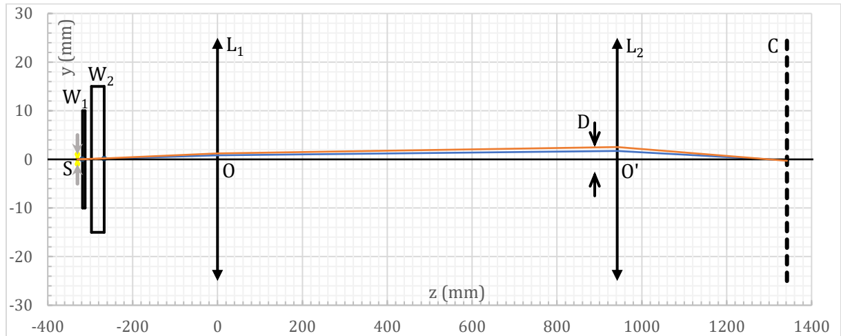
Figure B-6: Optical setup for magnification M = -0.5
