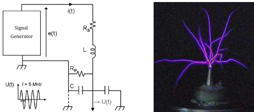
Figure 2-3: Radio-frequency igniter equivalent electric circuit (left) and picture of a radio-frequency discharge in air and atmospheric conditions (right) [24].
