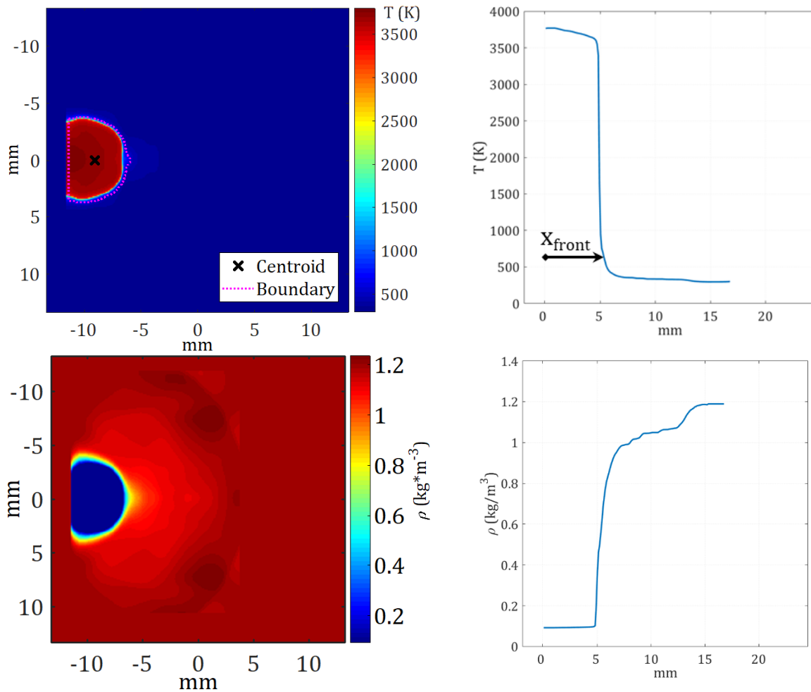
Figure 5-29: Temperature and density fields (left) , and T and \rho along the symmetry axis (right); in air, at 1 bar, \Delta t = 48.6 \mu\text{s} .
