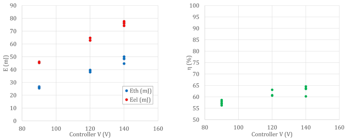
Figure 5-43: Experiments in air for the RF igniter, E_{el} and E_{th} (left) and \eta (right) versus controller voltage.
