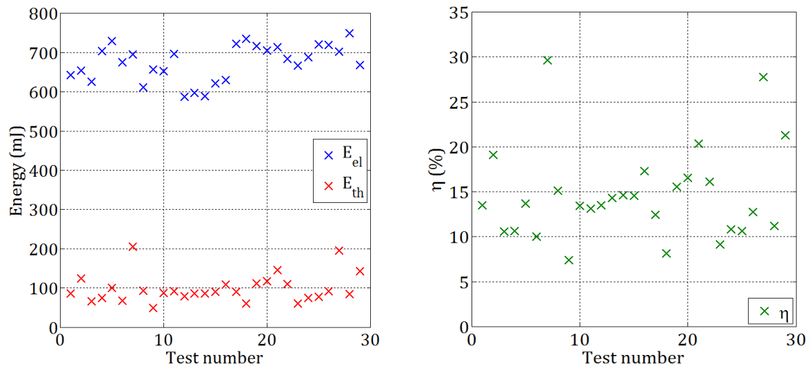
Figure 5-17: Set of tests for the Eyquem helicopter igniter. Results for E_{el} and E_{th} (left) and corresponding \eta (right).
