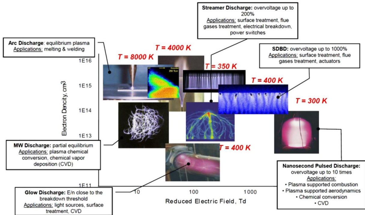
Figure 1-7: Discharge development and plasma generation for different applied overvoltages and their applications [21]
