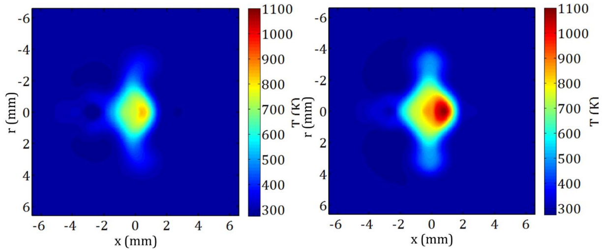
Figure 4-24: Temperature field for 1 and 2 mm gap for 3.0 and 2.9 ms, averaged for 10 tests.
