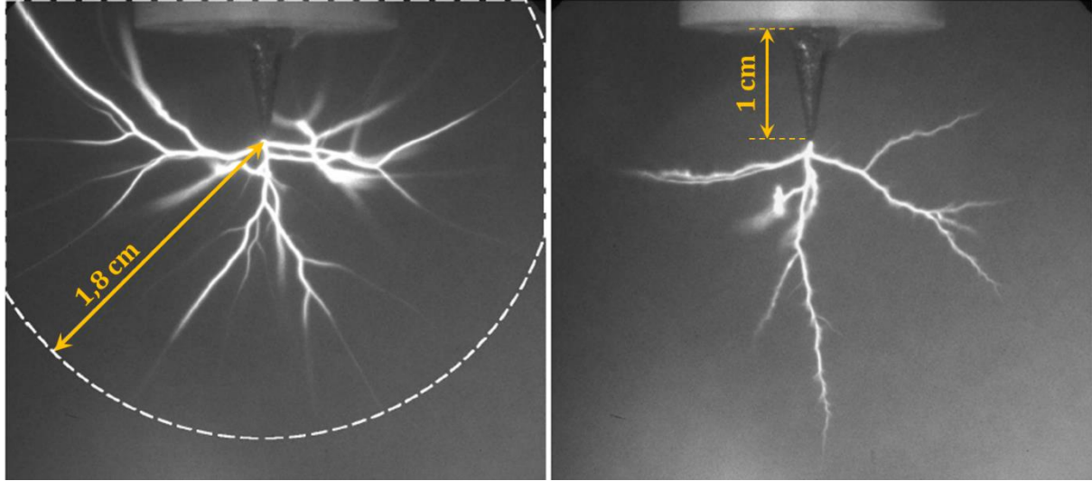
Figure 5-42: Radio-frequency discharge at 1 bar (left) and at 5 bar (right) [24].
