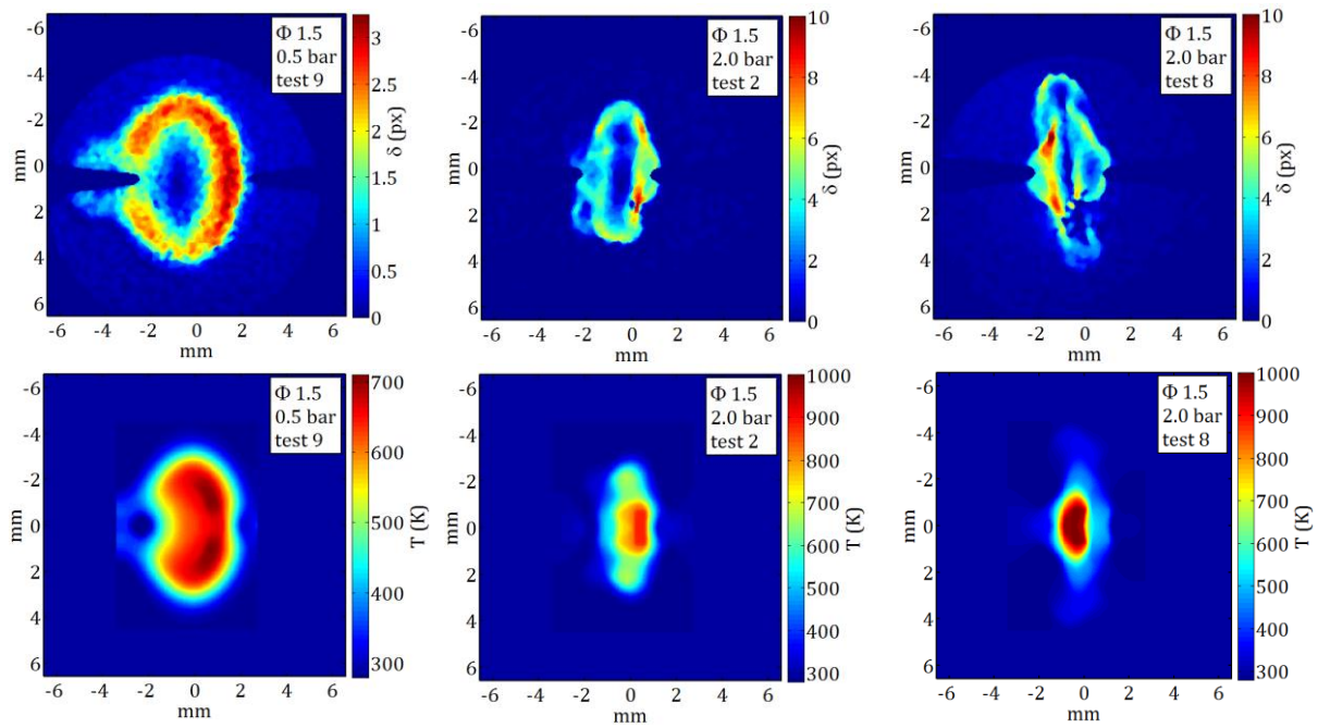
Figure 4-38: Instantaneous displacement and corresponding temperature fields for discharges with a 2 mm gap in the mixture \Phi_{eq} 1.5 and different pressures. In 0.5 bar (left), high repeatability with symmetric kernel shape. At 2.0 bar, higher variability with symmetric kernels (central image) as well as asymmetric structures (right).
