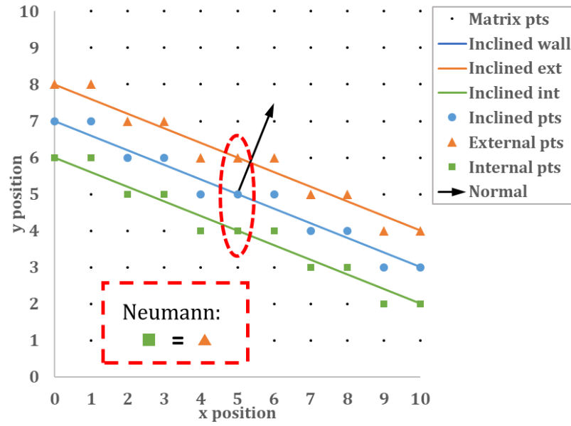
Figure C-2: Neumann BC on an inclined wall
