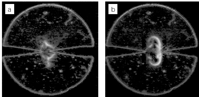
Figure 3-11 : Schlieren images 0.633 ms after discharge. Hot kernel is in contact with electrode tips for 1 mm gap (a) but mostly between electrode tips for a 3 mm gap (b).
