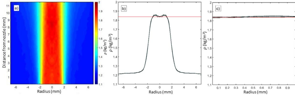
Figure 4-20: Jet CO 2 – noise. Density field in cylindrical coordinates (a), density radial distribution average and deviation profiles obtained 1 mm above nozzle exit (b) and density axial distribution, average and deviation profiles in the jet core ( r=0 ) (c) with CO 2 theoretical density for reference (in red) [103].
