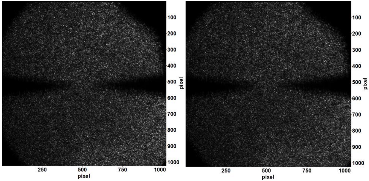
Figure 4-6: SBOS images of an electrical discharge in air and atmospheric conditions, with l = -80 mm and 1 mm gap. Left: Reference speckle pattern image, before the discharge event. Right: Caption 3.0 ms after discharge onset, with speckle pattern influenced by the hot discharge kernel.
