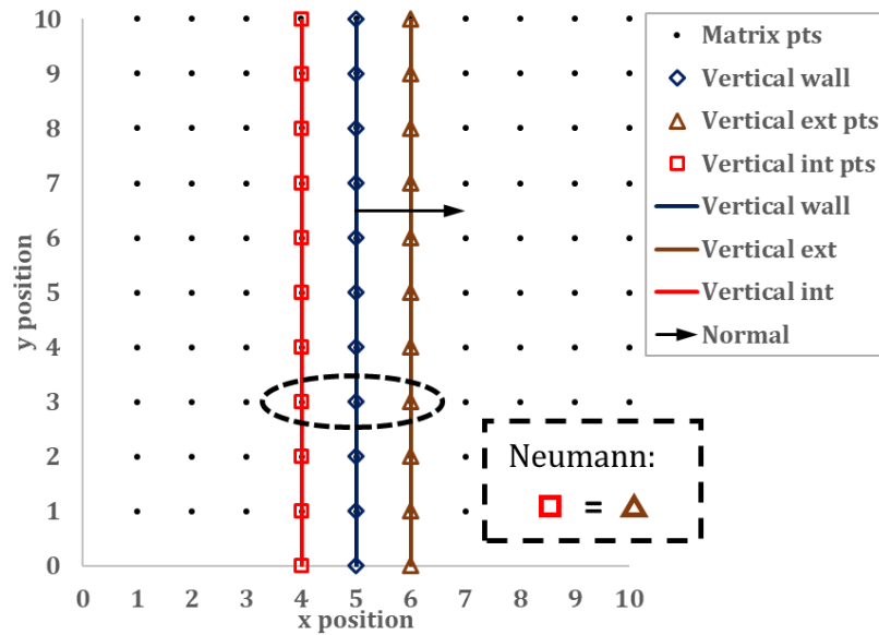
Figure C-1: Neumann Boundary Condition on a vertical wall
