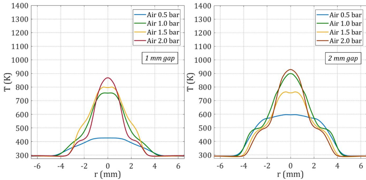
Figure 4-35: Temperature profiles along a vertical band for different pressures. From temperature fields averaged for 10 tests in each condition. Gap of 1 mm (left) and 2 mm (right).
