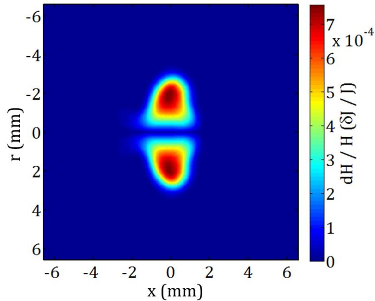
Figure 4-17: Enthalpy differential surface.
