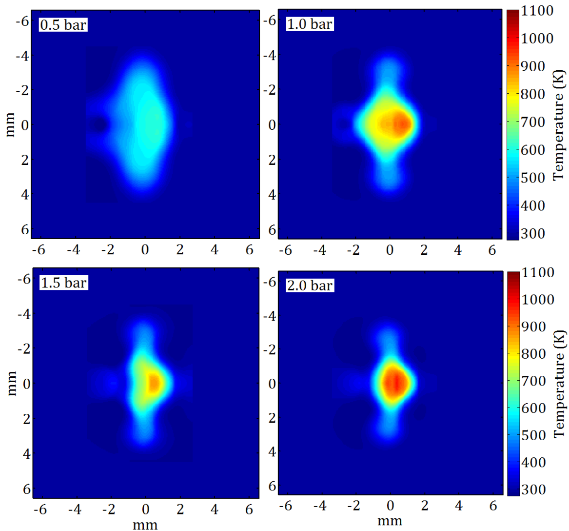
Figure 4-34: Temperature fields averaged for 10 tests, for 0.5, 1.0, 1.5 and 2 bar in air and a 2 mm gap.
