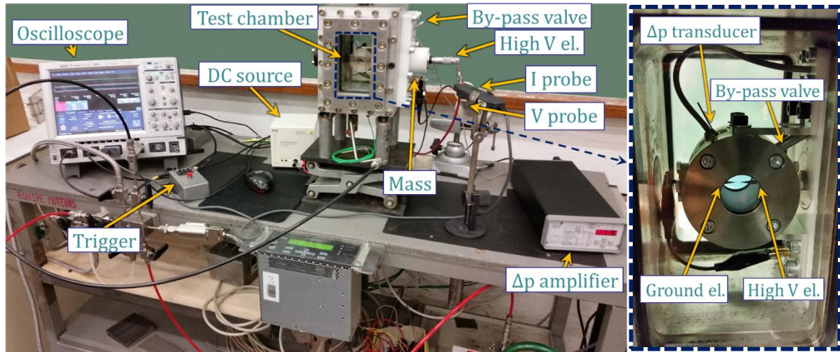
Figure 3-1: Pin-to-pin electrodes calorimetry experimental setup and detail on the inner chamber.
