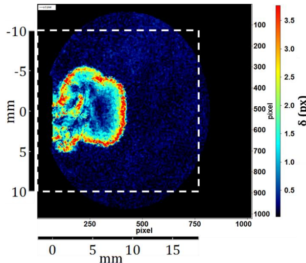
Figure 5-24: Displacement field 1 ms after the discharge start. White: investigation zone for kernel evolution
