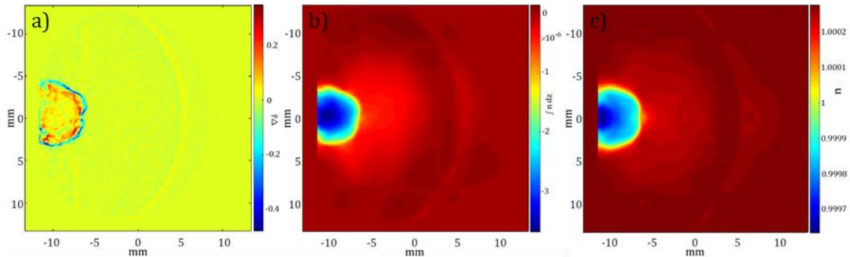
Figure 5-28: SBOS image processing: a) divergence, b) integration, c) filtered back-projection.
