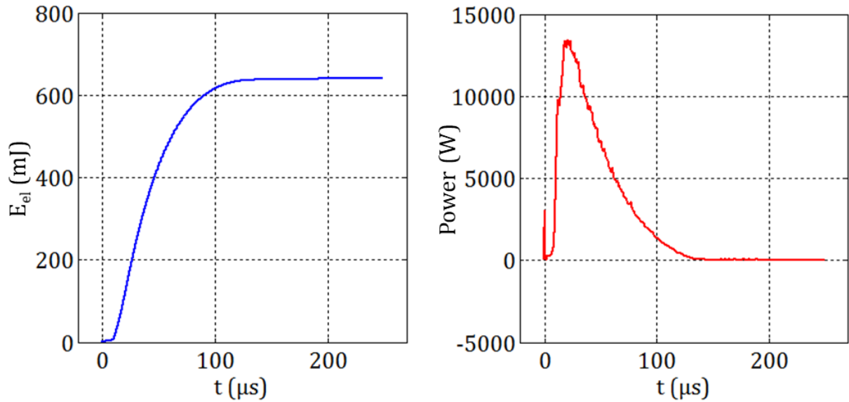
Figure 5-10: Electric energy E_{el} (left) and electric power (right).
