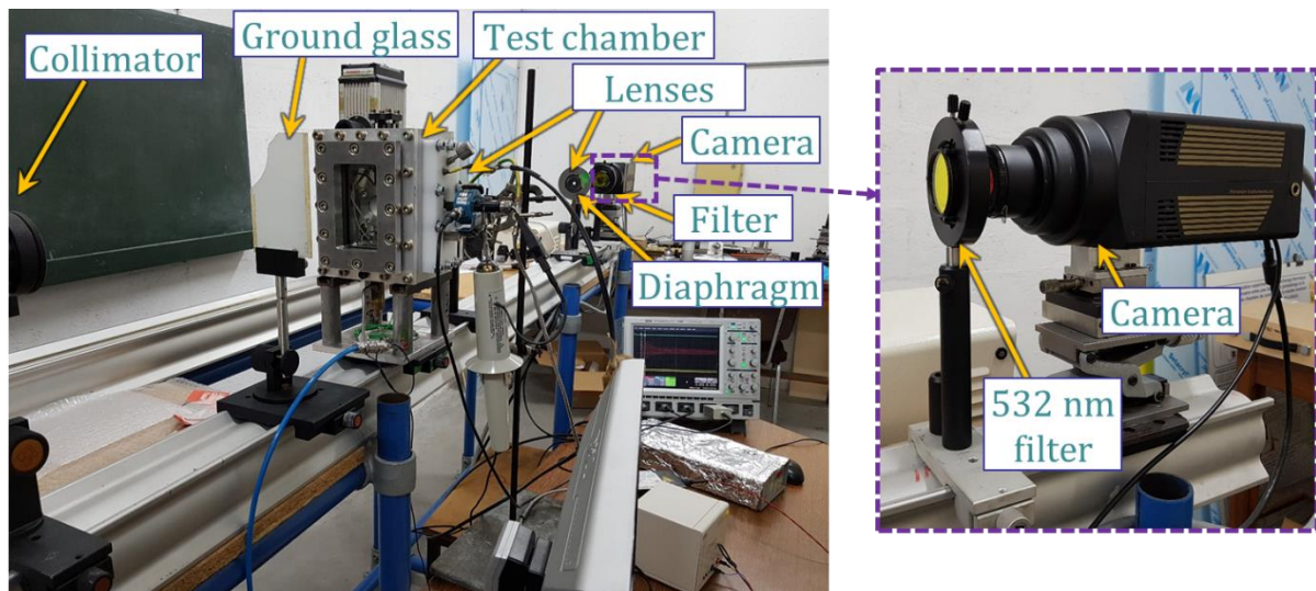
Figure 5-23: SBOS experimental setup.
