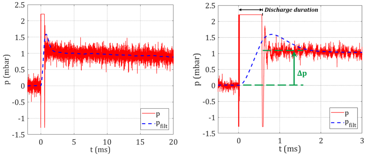
Figure 5-41: Pressure signal during a radiofrequency discharge of E_{th} = 26.6 mJ at 1 bar.
