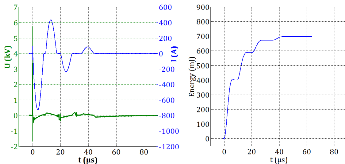
Figure 5-15: Electrical signals and E_{el} for the Eyquem helicopter igniter, in air and atmospheric conditions.
