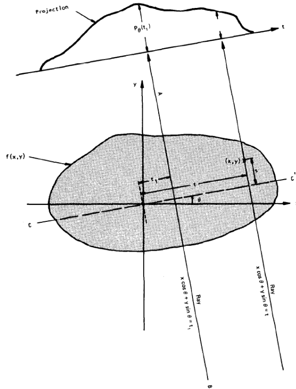
Figure 4-12: An object and its projection [116].
