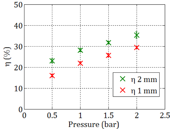
Figure 3-19: Energy transfer efficiency versus pressure for 1 and 2 mm gap
