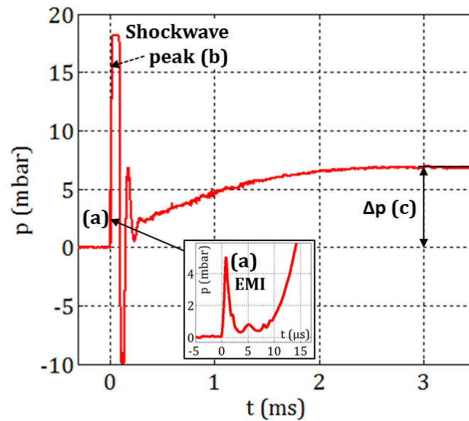
Figure 3-4: Differential pressure evolution measured for a 1.0 mm gap and 39 mJ of electrical energy. (a) Antenna effect and high electromagnetic field. (b) Shockwave peak arrival to the pressure transducer. (c) Maximum mean pressure.
