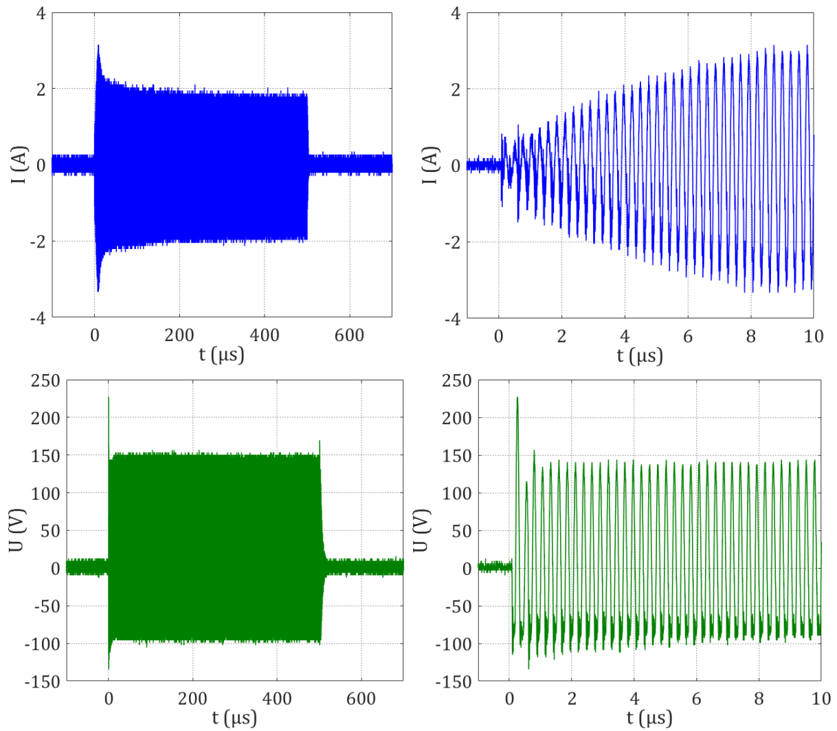
Figure 5-39: Electrical signals during RF discharge
