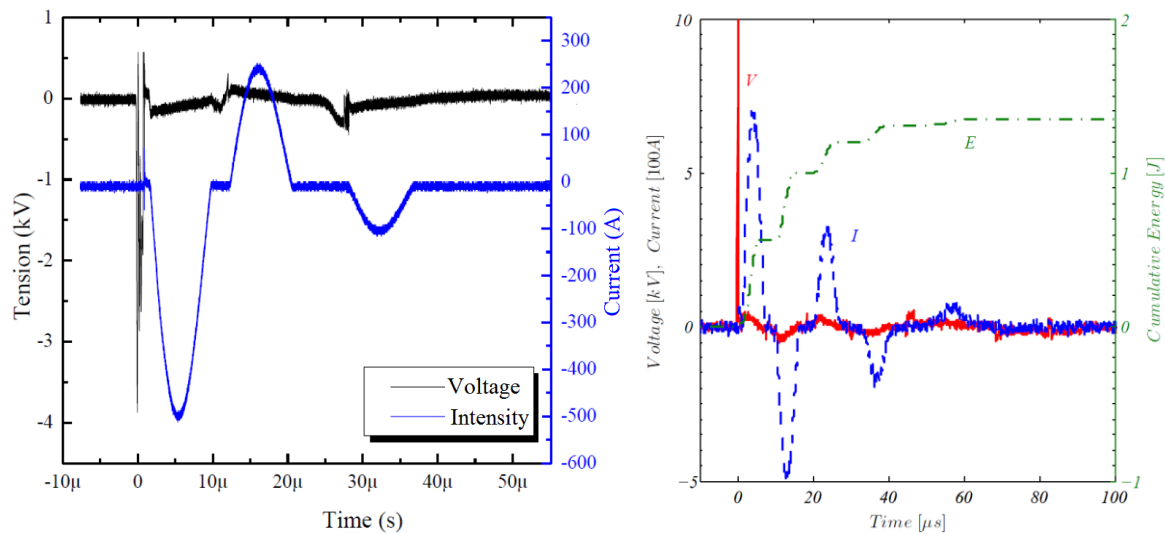
Figure 5-1: Characteristic electric signals for an aircraft igniter, George [36](left), Sforzo [18](right).
