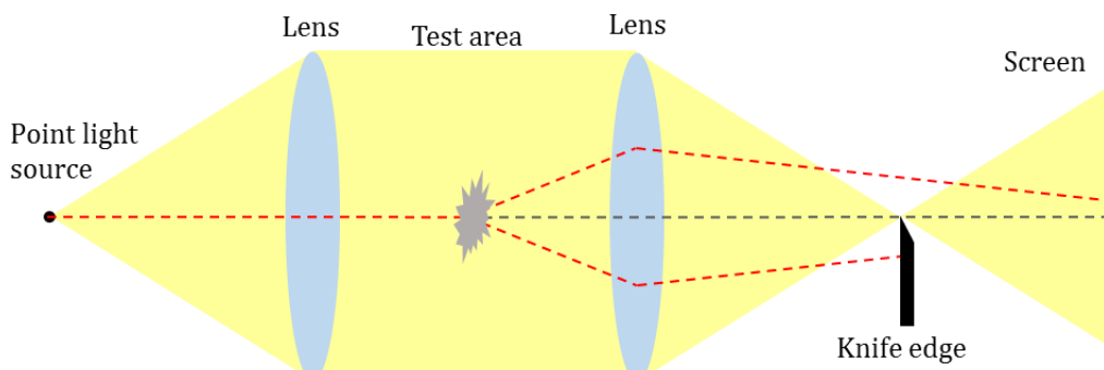
Figure 4-1: Diagram of a schlieren system [105]
