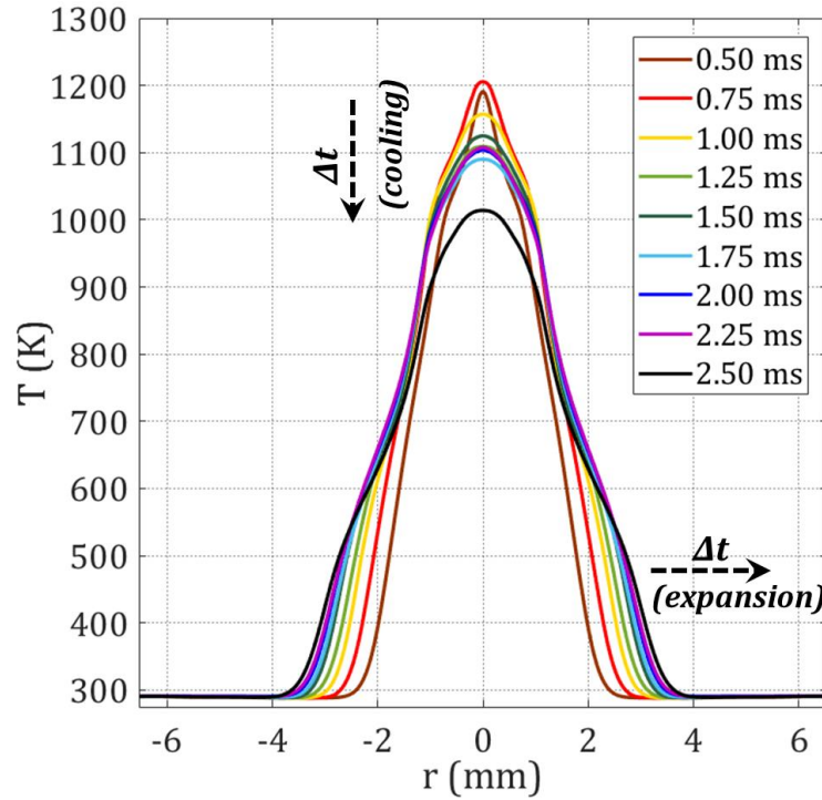
Figure 4-29: Temperature profiles along a central band of the discharge kernel for different \Delta t . Profiles from temperature fields averaged for 10 tests at each \Delta t , at 1 bar for a 2 mm gap.
