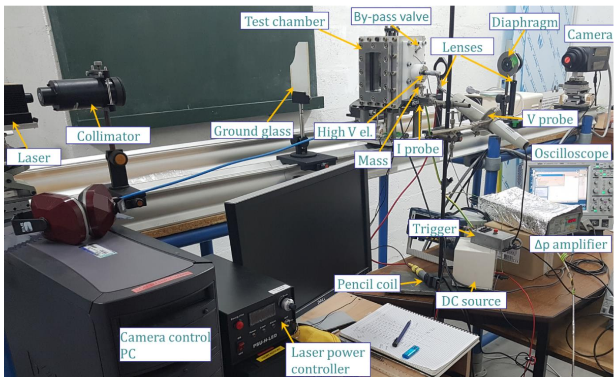
Figure 4-22: Picture of the SBOS and calorimetry experimental setup
