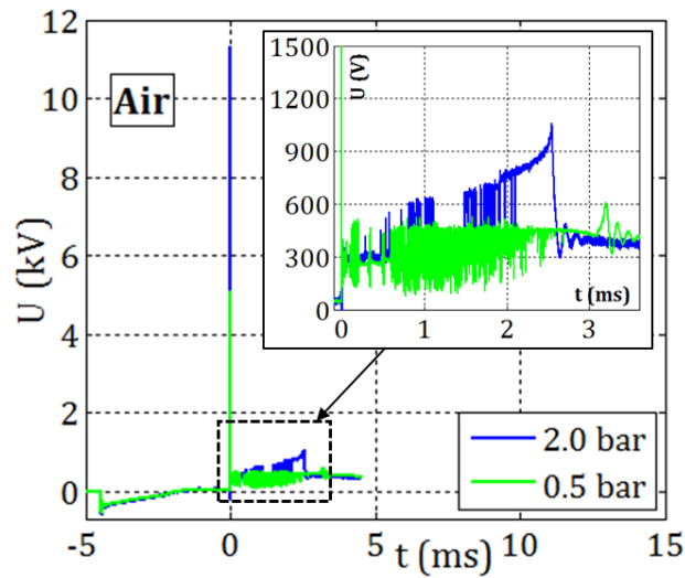
Figure 3-24: Voltage at 0.5 and 2 bar for a 2 mm gap in air.
