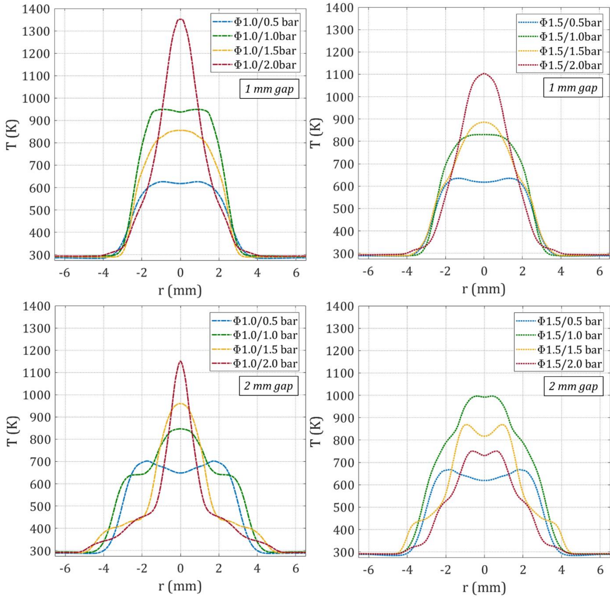
Figure 4-41: Temperature profiles of a vertical band of the central plane at the end of the discharge for different inert mixtures and pressures, for 1 and 2 mm gap.
