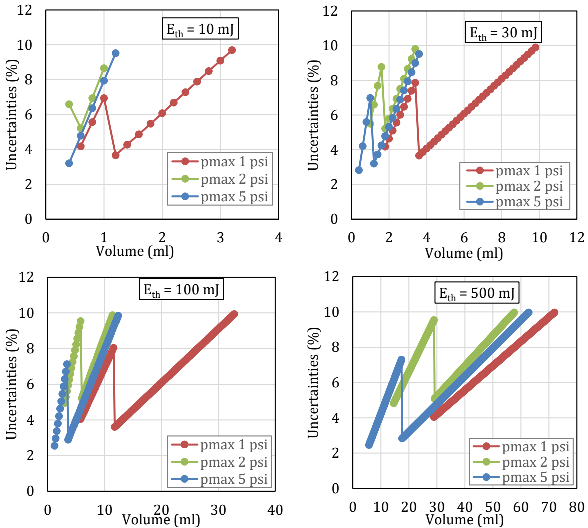
Figure 2-4: Uncertainties versus chamber volume for different pressure transducers. Energy deposits are, from left to right and top to bottom, 10, 30, 100, and 500 mJ.
