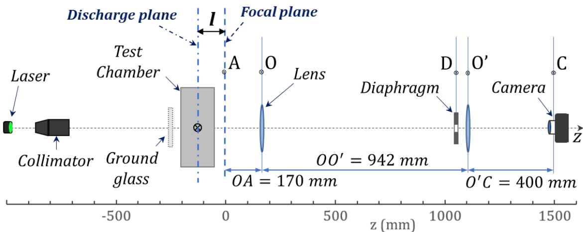
Figure 5-18: Optical setup for a magnification of M = -0.5
