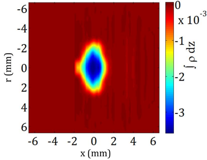
Figure 4-9: Integrated density field by line integration.
