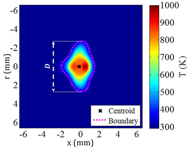
Figure 4-14: Hot kernel boundary superimposed on the temperature field.
