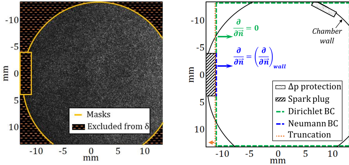
Figure 5-22: Displacement field masks for cross-correlation (left) and schema of the boundary conditions for Poisson equation integration (right).
