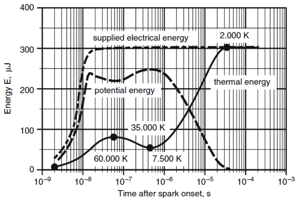
Figure 1-3: Temporal redistribution of the electrically supplied energy in a breakdown phase from initially potential energy (dissociation, ionization) into thermal energy
