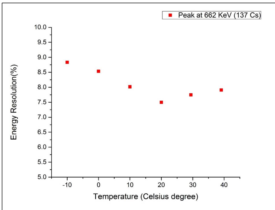
Figure 4.17 The energy resolution of the system CLYC+ArrayJ-30035-64P-PCB as a function of temperature from -10 °C to +40 °C. Data refer to the 662 keV photopeak.
