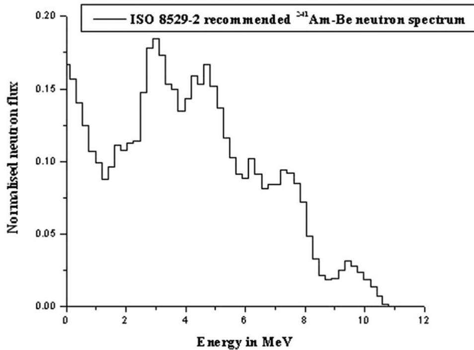
Figure 5.32 ISO 8529-2 recommended ^{241}\text{Am} -Be neutron spectrum [14].
