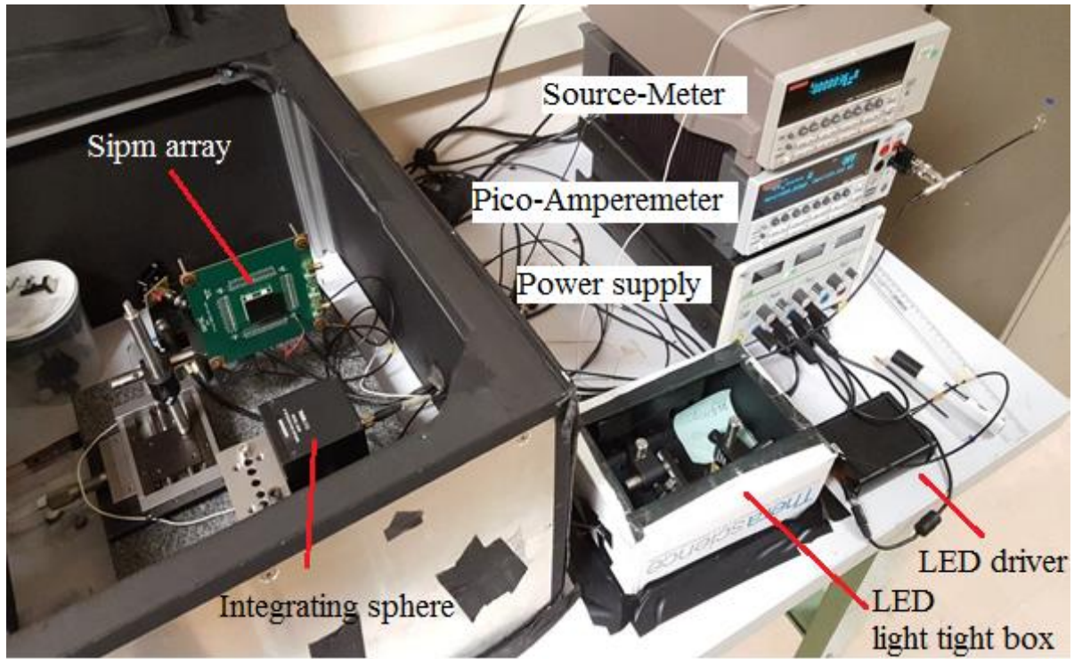
Figure 4.20 Picture of the experimental set-up.
