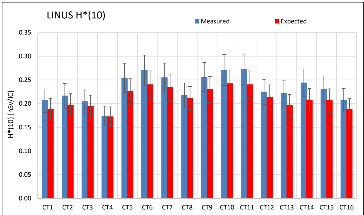
Figure 3.23 H^*(10) in nSv per IC count measured and expected with LINUS on CT positions.
