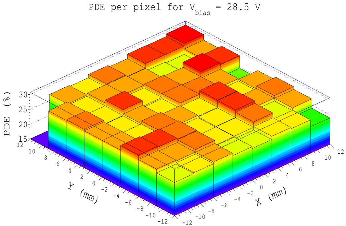
Figure 4.30 Photodetection efficiency (PDE) distribution per pixel at 28.5 V.
