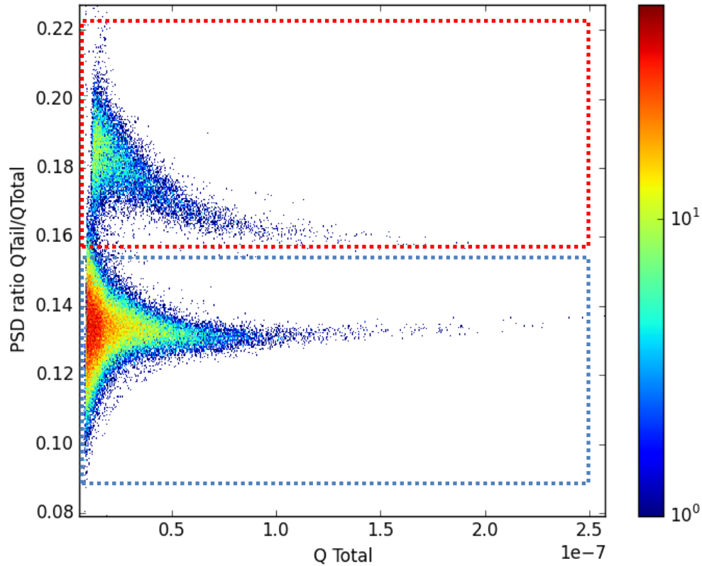
Figure 6.5 Two dimensional PSD plot for the best configuration (prompt window = 1.5 \mu\text{s} , delayed window = 4 \mu\text{s} ). The blue box are gamma events while the red box corresponds to neutron events.
