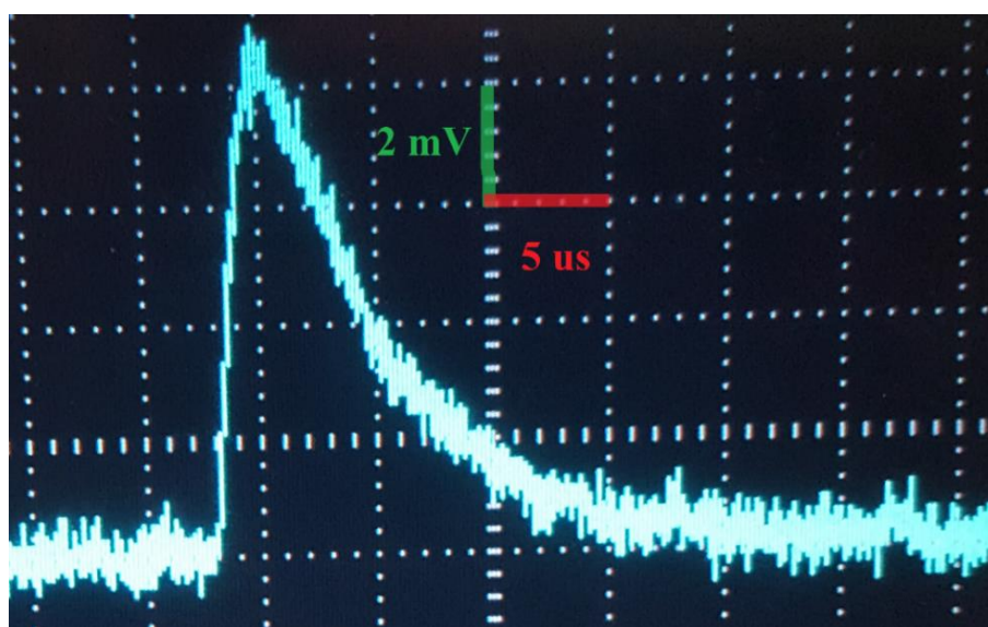
Figure 4.49 Shaper output.
