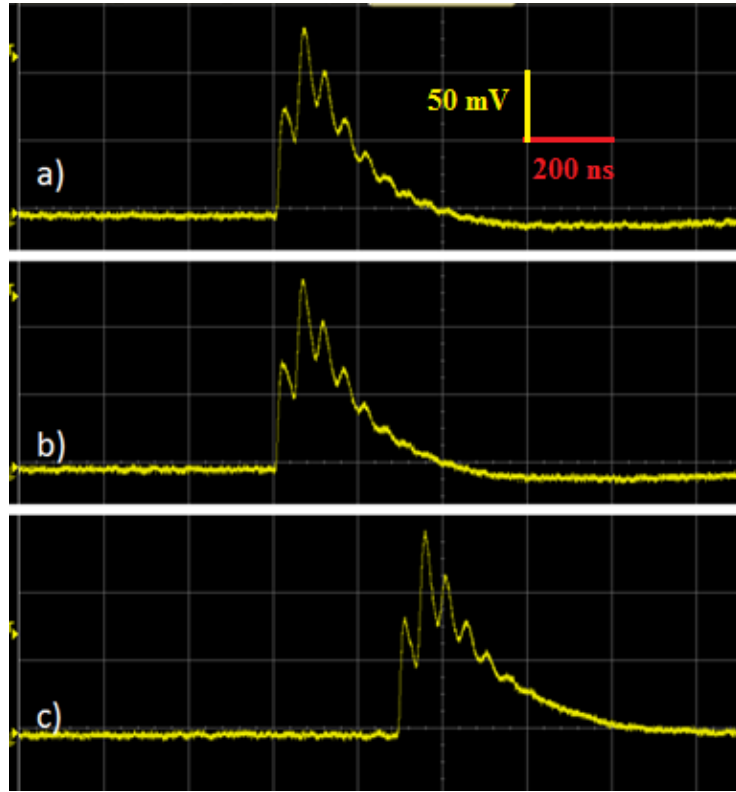
Figure 4.39 ^{137}\text{Cs} signal from \text{LaBr}_3 coupled with the SiPM array with R_{\text{load}}=3.6\ \Omega and Gain = 9.9, with pole-zero compensation with \text{RC}=1\ \mu\text{s} (a), 930 ns (b) and 500 ns (c).
