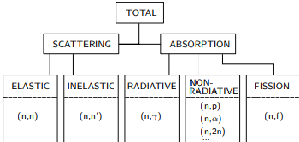
Figure 1.2 Summary of neutron interaction with matter [2].
