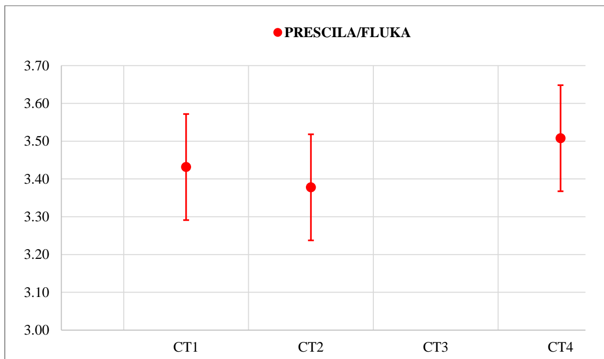
Figure 3.14. H^*(10) ratios between PRESCILA and FLUKA on the CT.
