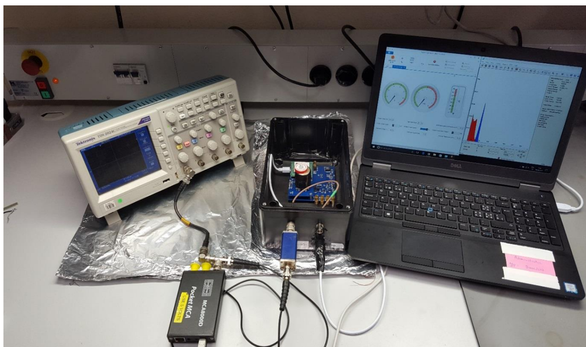
Figure 4.43 Measurement setup.
