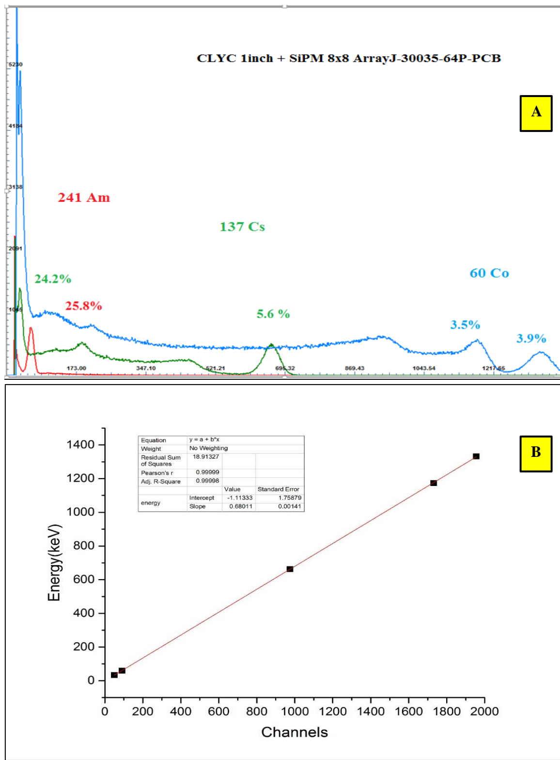
Figure 4.15 ^{241}\text{Am} , ^{137}\text{Cs} and ^{60}\text{Co} spectra, and energy resolutions obtained with the CLYC coupled with the 8x8 ArrayJ-30035-64P-PCB (A) and the energy-channel calibration (B).
