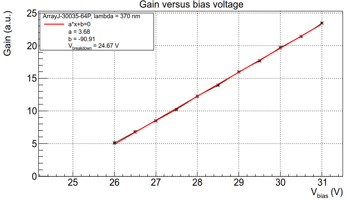
Figure 4.26 Gain versus bias voltage for one pixel.
