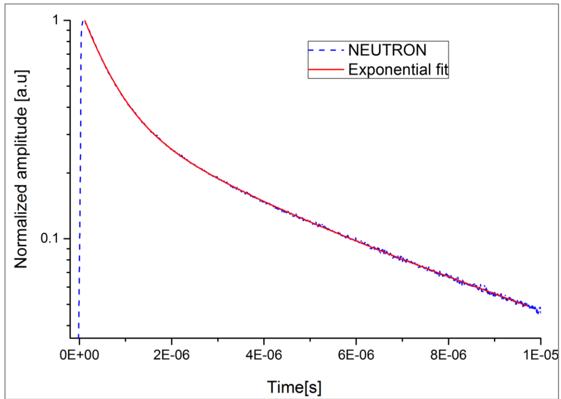
Figure 5.22 Neutron standard pulse.
