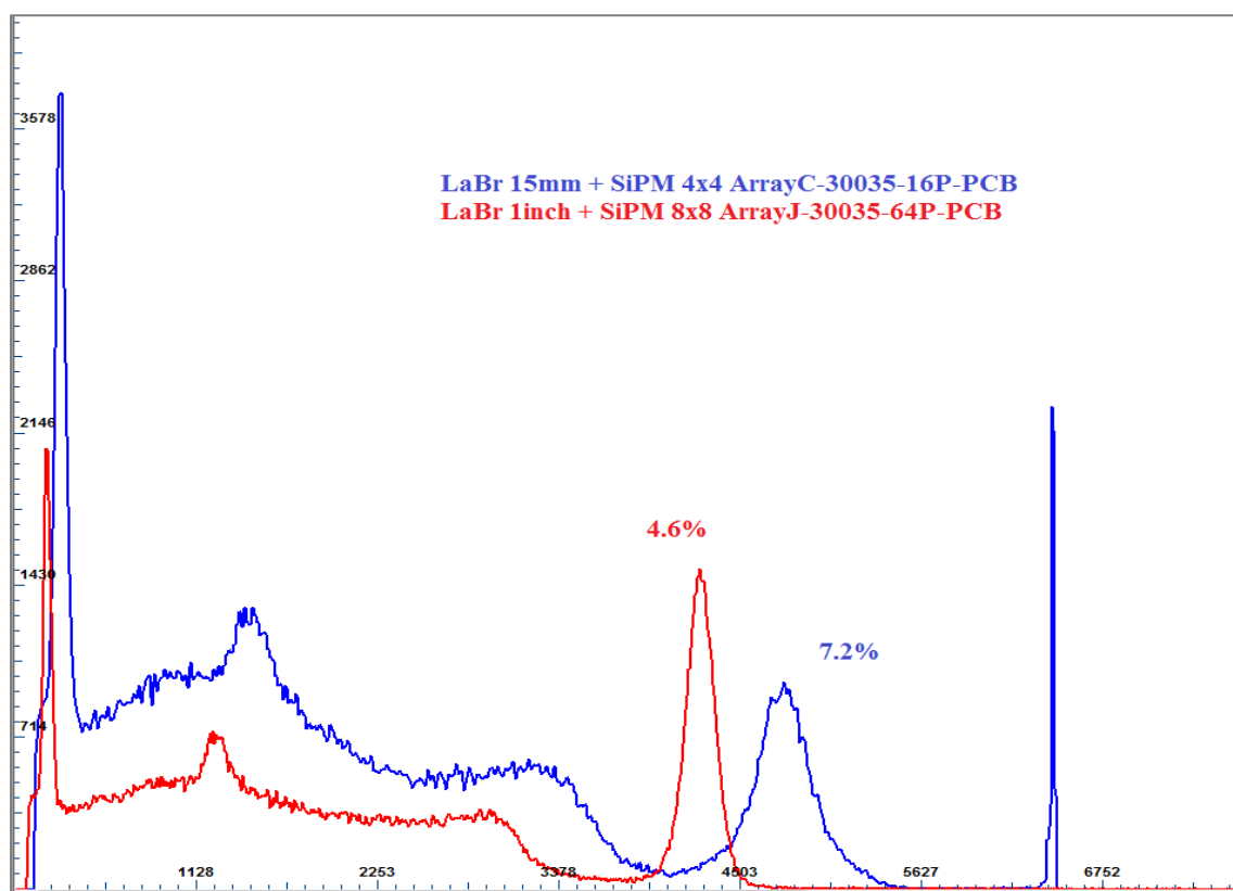
Figure 4.13 137 Cs spectra and energy resolution at 662 keV. The blue spectrum represents the system LaBr 3 (15mm) + 4x4 ArrayC-30035-16P. The energy resolution of the 662 keV peak is 7.2%. The red curve represents the system LaBr 3 (1 inch) + 8x8 ArrayJ-30035-64P-PCB. An energy resolution of 4.6% was obtained for the 662 keV peak.
