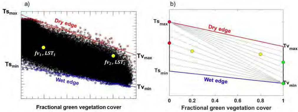
Fig. 3. In a), example of LST-fv feature space constrained by the polygon Ts_{min}-Tv_{min}-Tv_{max}-Ts_{max} from the linear regression of the minimum and maximum LST by fv classes. In b), a conceptual diagram of the LST-fv polygon for partitioning LST for two pixels ( f_v, LST ) (yellow points) showing its Ts (red points) and Tv (green points) values corresponding to the TSEB assumptions. (For interpretation of the references to colour in this figure legend, the reader is referred to the web version of this article.)
