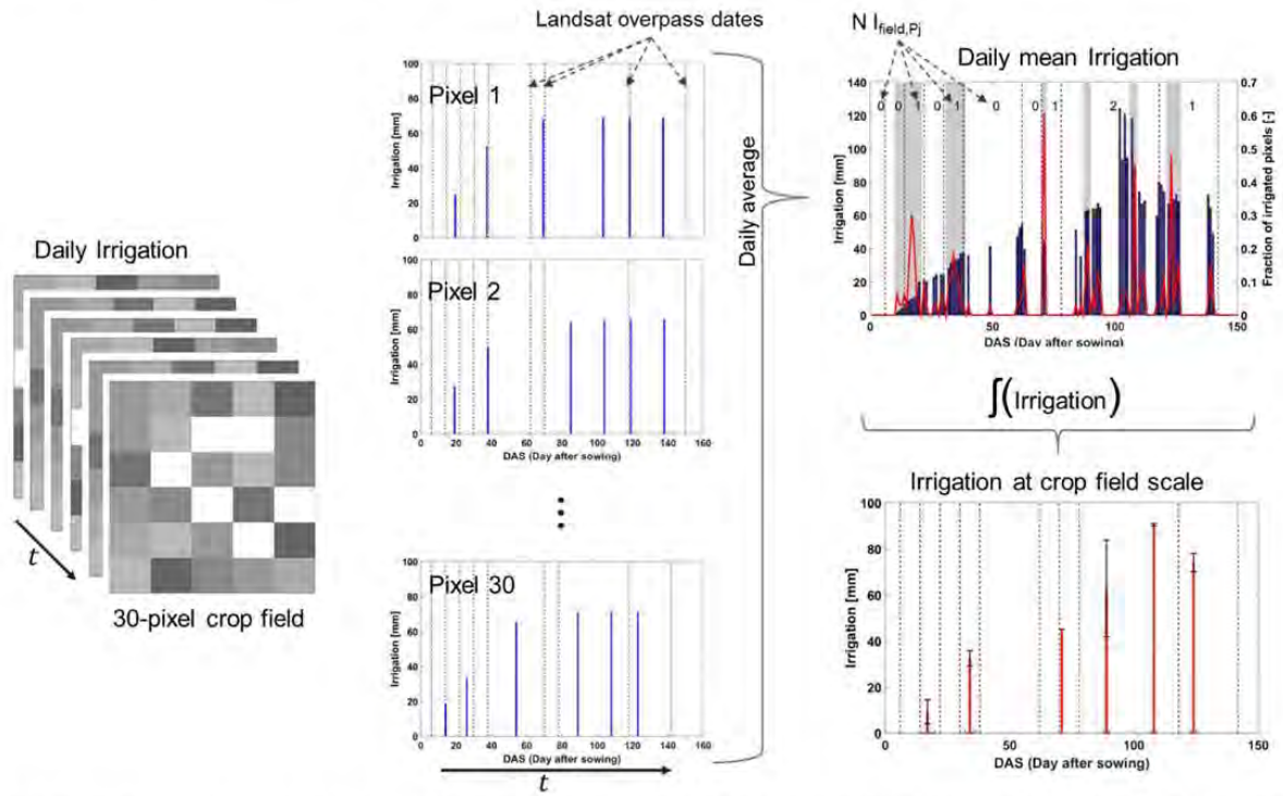
Fig. 4. Schematic diagram presenting the crop field scale irrigation retrieval from pixel-scale irrigation estimates for an example of a 30-pixel crop field. The daily pixel-scale irrigation is represented for every pixel (middle plots), from which are estimated the daily averaged irrigation (blue bar in top right plot) and the fraction of irrigated pixels (red line) according to its fractional irrigated pixels. The crop field scale irrigation (red bar in bottom right plot) is obtained by deriving the most probable irrigation date and is provided with its standard deviation for amount (black error bar) and date (red error bar). (For interpretation of the references to colour in this figure legend, the reader is referred to the web version of this article.)
