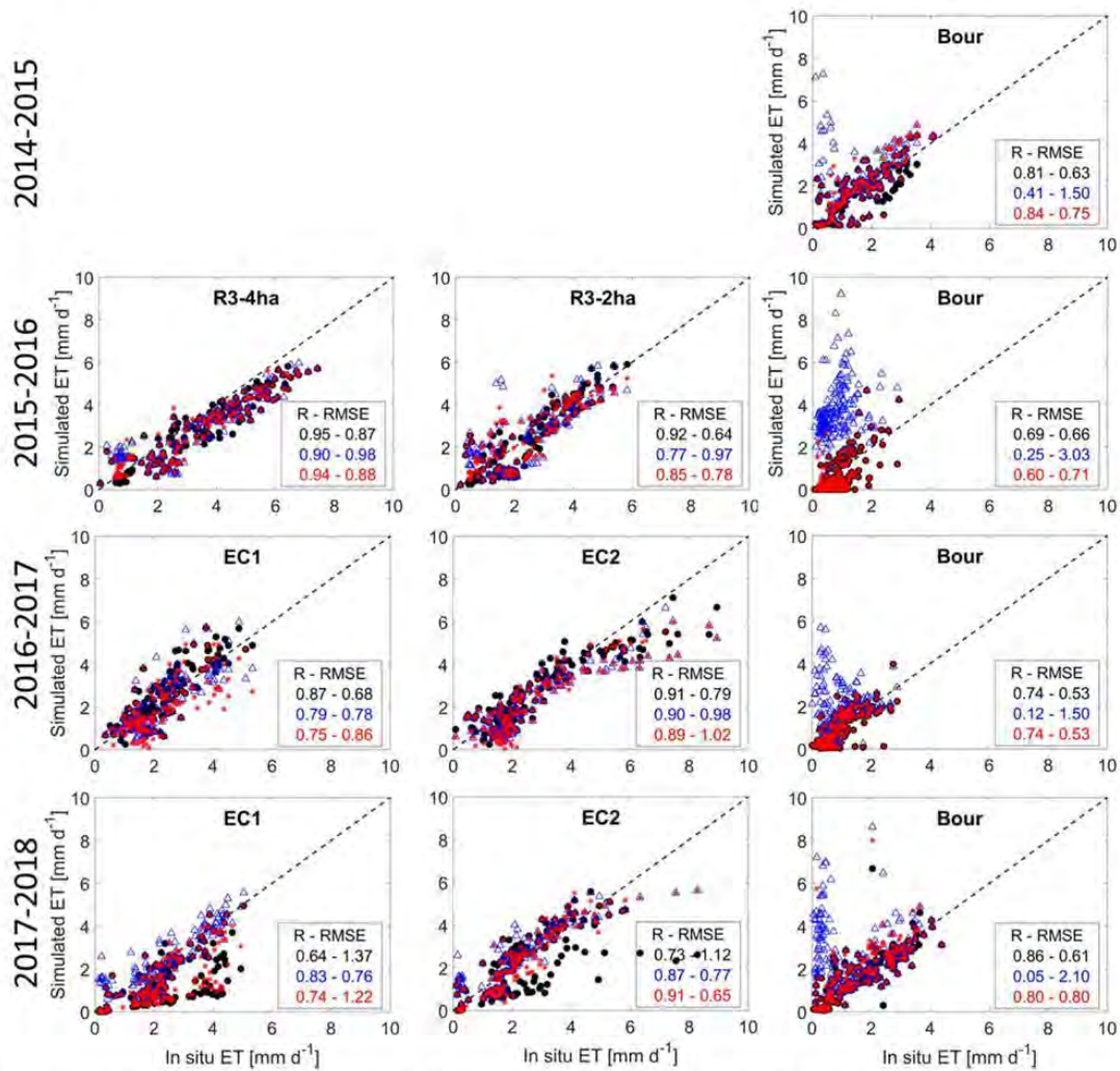
Fig. 9. Ground-based ET is plotted versus the ET simulated by from FAO-2Kc forced by observed irrigation (black, ET_{FAO-2Kc_{1obs}} ), irrigation triggered by avoiding stress (blue, ET_{FAO-2Kc_{Ks=1}} ) and irrigation retrieved from the proposed methodology (red, ET_{FAO-2Kc_{Landsat}} ). The correlation coefficient (R), bias and root mean square error (RMSE) are shown for ET_{FAO-2Kc_{1obs}} , ET_{FAO-2Kc_{Ks=1}} and ET_{FAO-2Kc_{Landsat}} . (For interpretation of the references to colour in this figure legend, the reader is referred to the web version of this article.)
