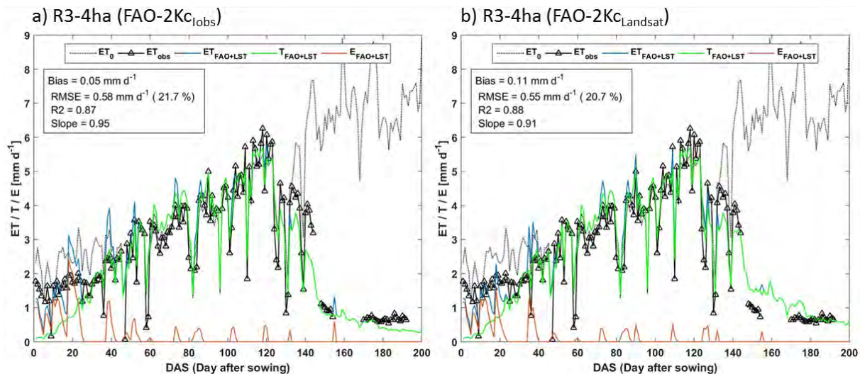
Fig. 4.7. Comparison of ET forced by the actual irrigations (FAO-2Kc lob ) and retrieved irrigations (FAO-2Kc Landsat ) against the observed ET without applying the Bowen correction (ET obs ) over the R3-4ha site along the 2016 growing season.
