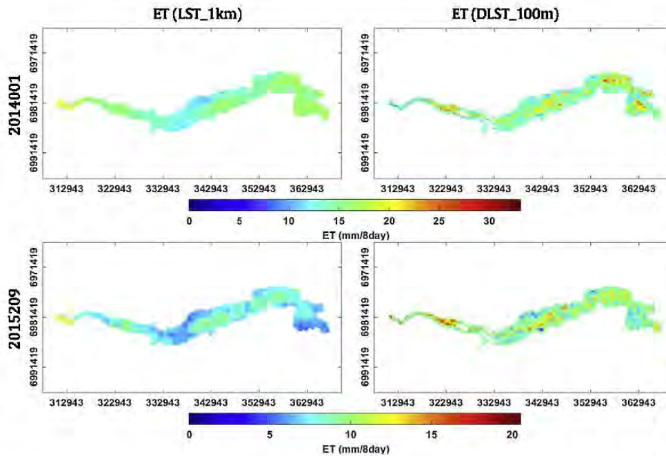
Fig. 6. Comparison between the composite 8-day E_t at 1 km and the disaggregated product at 100 m from MODIS LST at 1 km and the disaggregated LST product at 100 m, respectively.
