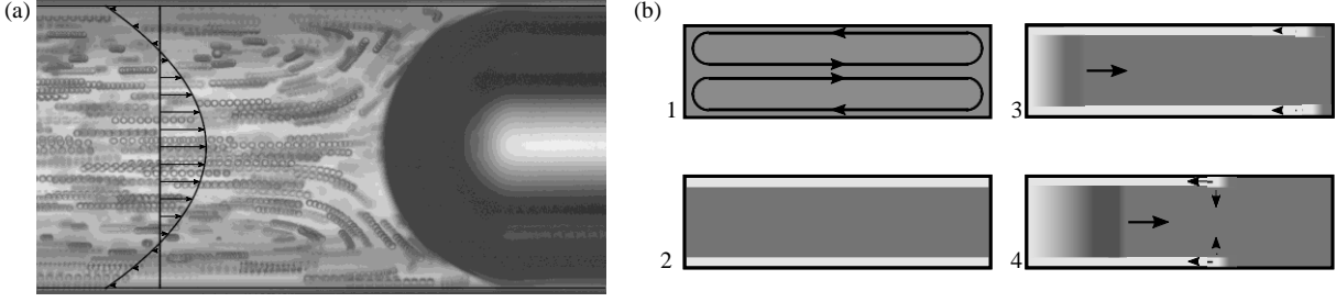
Figure 5: (a) Trajectories of beads at the rear of the leading bubble in the reference frame of the latter ( \varphi_0 = 0.5\% ). The image is a superposition of 10 snapshots with a time interval of 0.5 ms. The velocity field is also shown. (b) Mechanism for the development of longitudinal variation of particle concentration; 1 : recirculation of a homogeneous suspension contained in a closed vessel ; 2 : addition of a depletion layer near the wall ; 3 : propagation of a low volume fraction into the core from the left side and an high volume fraction from the right through the layer near the wall. 4 : coupling with a migration of particles from the wall to the core. Volume fraction is shown in grayscale.
