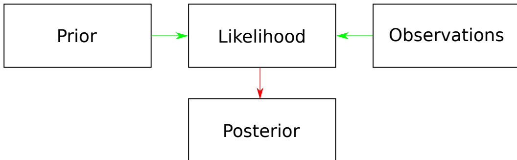
Figure 4.3: Bayesian inverse problem.
