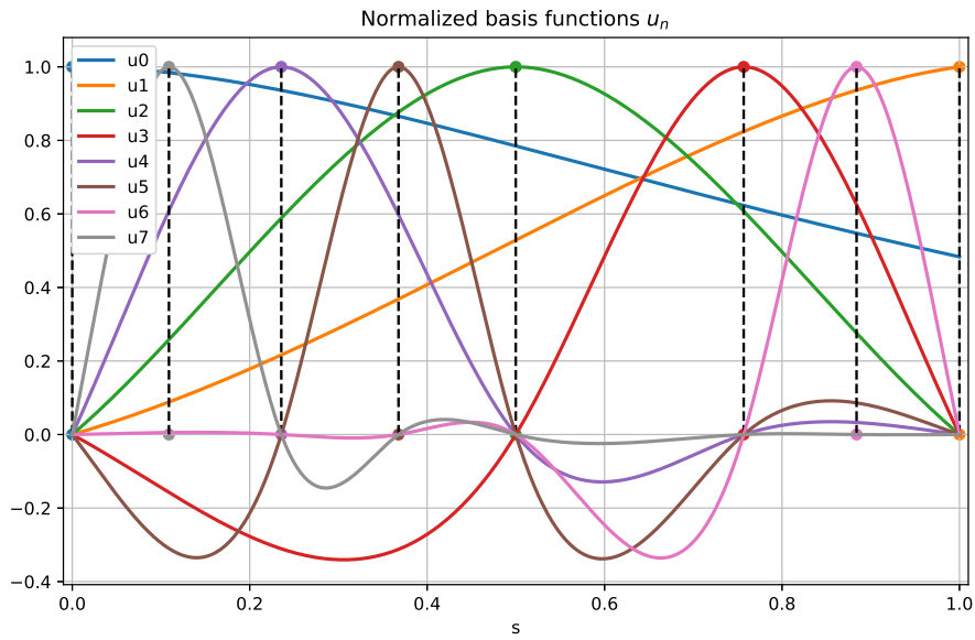
Figure 2.3: 8 first normalized basis functions ( u_0, \dots, u_7 ) (Matérn \nu = \frac{3}{2} kernel). The dots represent positions ( s_0, \dots, s_7 ) of associated Dirac functionals of maximum variance.
