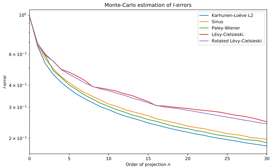
Figure 2.9: Numerical comparison of l -errors of admissible sequences for the standard Wiener process.
