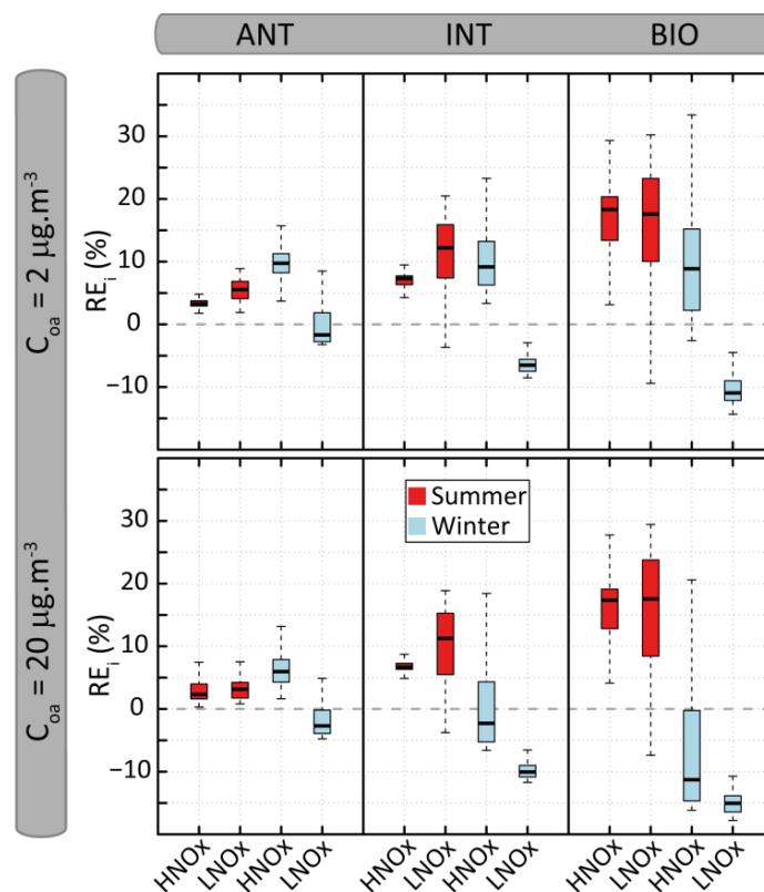
Figure 4.9 - Distribution of the relative errors (RE i ) on organic aerosol mass concentration calculated between VBS-GECKO and GECKO-A for the 24 evaluation scenarios. The bottom and top of the boxes are the first and third quartiles, the bands inside the boxes represent the medians. The ends of the whiskers represent the lowest and the highest RE i . The number of data is of 361 time steps for each evaluation scenario.
