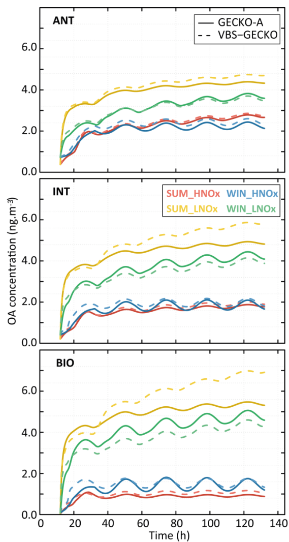
Figure 4.8 – Simulated organic aerosol (OA) mass with GECKO-A (continuous lines) and VBS-GECKO (dashed lines), for the different evaluation scenarios using C_{oa} = 2 \mu\text{g}\cdot\text{m}^{-3} . Top panel presents results for the ANT cases, middle panel for the INT cases and bottom panel for the BIO cases. The different colours represent the different scenarios (see text).
