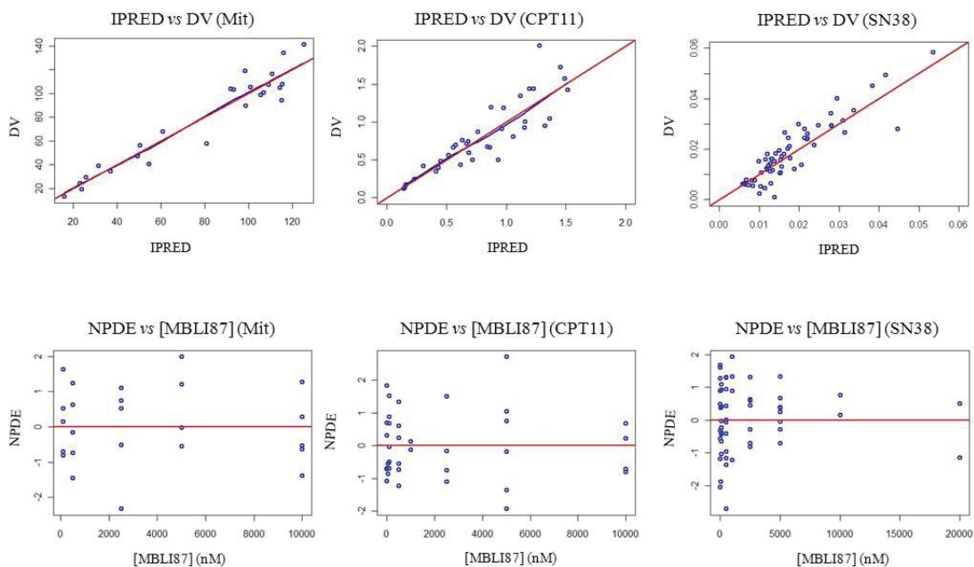
Figure 3: Goodness-of-Fit Plots
