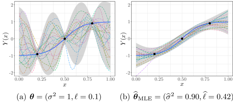
Figure 2.5: Conditional GP from Figure 2.4. Figure 2.5(b) shows the conditional process when the covariance parameters \theta are estimated via ML. On both models, an additive Gaussian white noise was added with a fixed noise variance \tau^2 = 0.03 .
