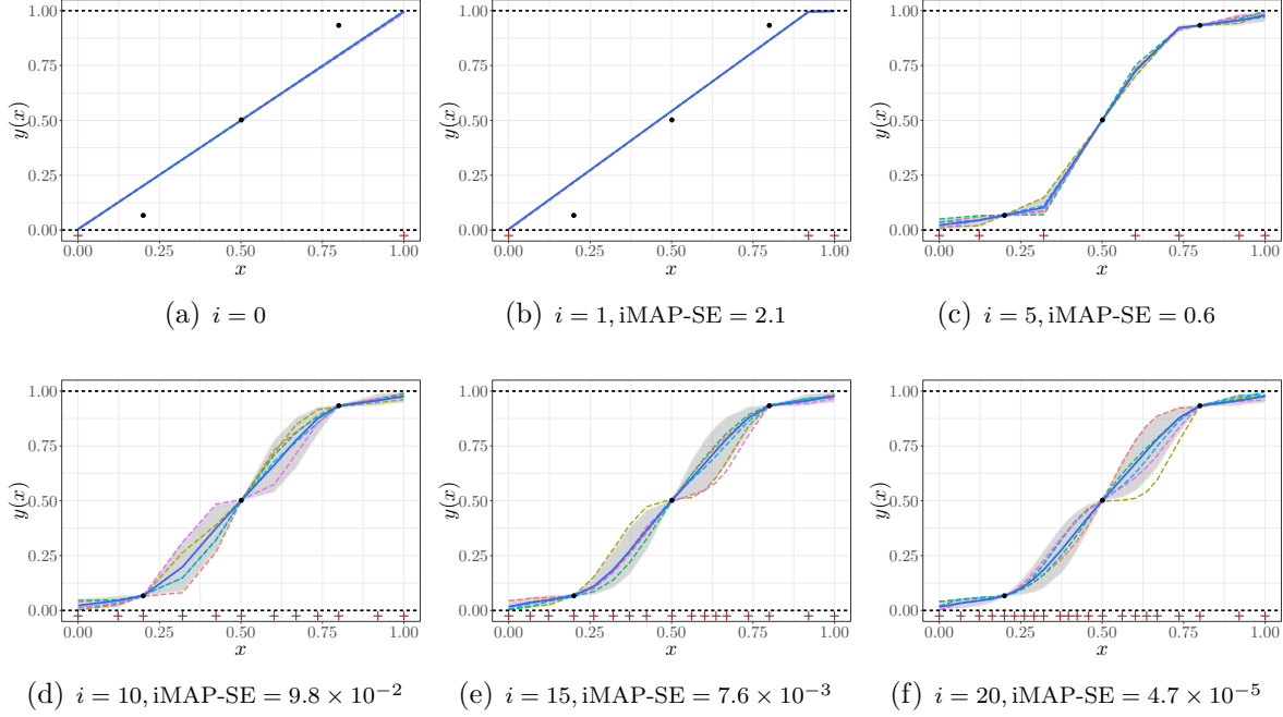
Figure 5.3: Conditional sample-path evolution of the example in Figure 5.2 . Each panel shows: training points and knot locations (black dots and red crosses), the conditional mean function (blue solid line), the 90% confidence intervals (grey region), and conditional realisations (dashed lines). Horizontal black dashed lines denote the bounds.
