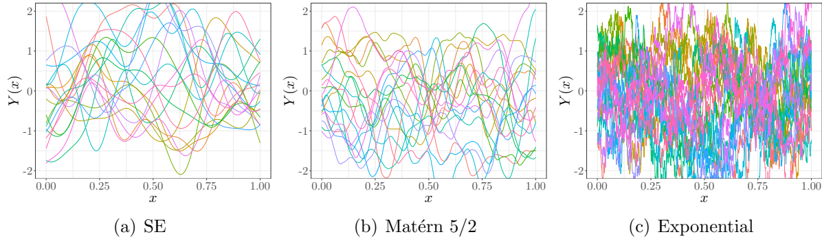
Figure 2.1: Effect of different kernels from Table 2.1 on unconditional GP samples with fixed covariance parameters \theta = (\sigma^2 = 1, \ell = 0.1) .
