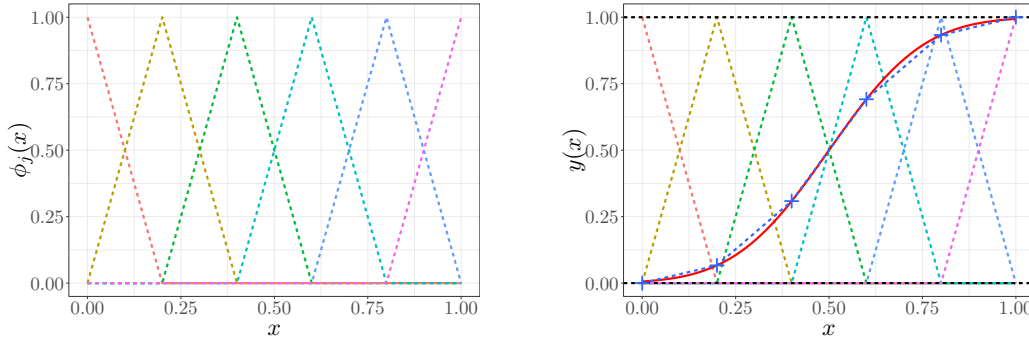
Figure 3.1: Illustration of the finite-dimensional approximation in (3.1). (Left) Hat functions \phi_j for j = 1, \dots, 6 . (Right) Approximation of the function y(x) = \Phi(\frac{x-0.5}{0.2}) , where \Phi is the standard normal cumulative distribution function. Red solid and blue dashed lines are the function y , and its finite approximation with six knots given by blue crosses, respectively. Horizontal black dashed lines denote the bounds.
