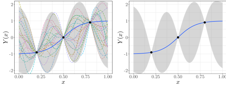
Figure 2.4: Conditional GP of Figure 2.3(a). The panel shows: the conditional mean function (blue solid line), two standard deviation conditional intervals (grey region), and conditional GP realisations (dashed lines).
