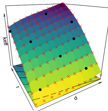
GP with boundedness and monotonicity constraints
