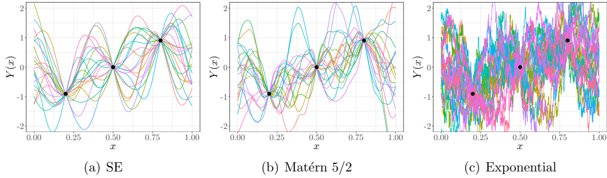
Figure 2.3: Samples of conditional GPs using various types of kernels. Conditioning observations at x_1 = 0.2 , x_2 = 0.5 , and x_3 = 0.8 are shown in black dots. The covariance parameters are fixed to \boldsymbol{\theta} = (\sigma^2 = 1, \ell = 0.1) .
