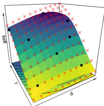
unconstrained GP
