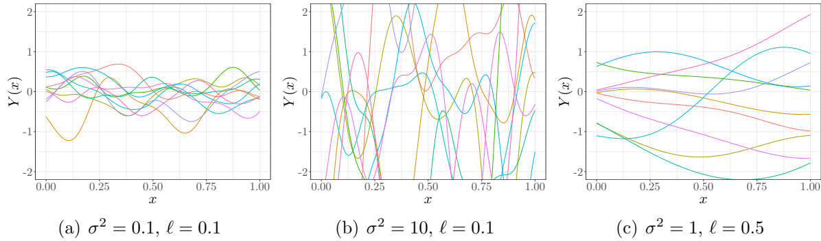
Figure 2.2: Effect of different covariance parameters \theta = (\sigma^2, \ell) on unconditional GP samples with SE kernel functions.
