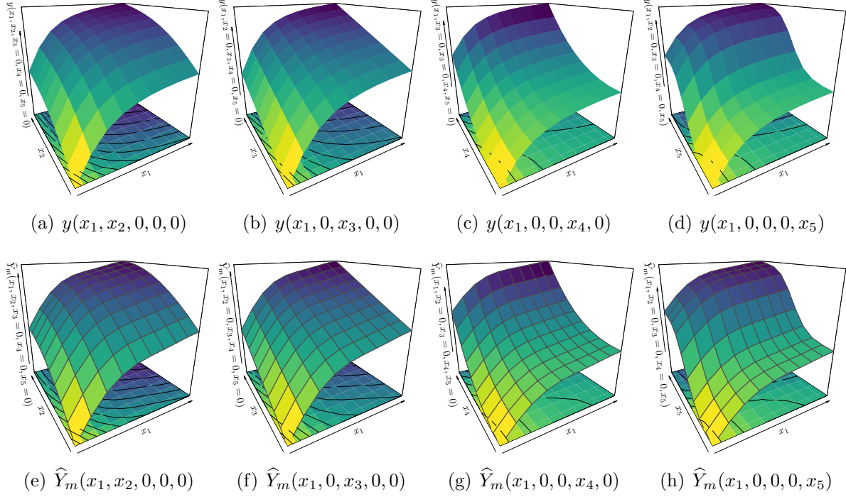
Figure 6.2: Additive GP model under monotonicity constraints in 5D. True and predictive mean profiles are shown in the first and second row, respectively.
