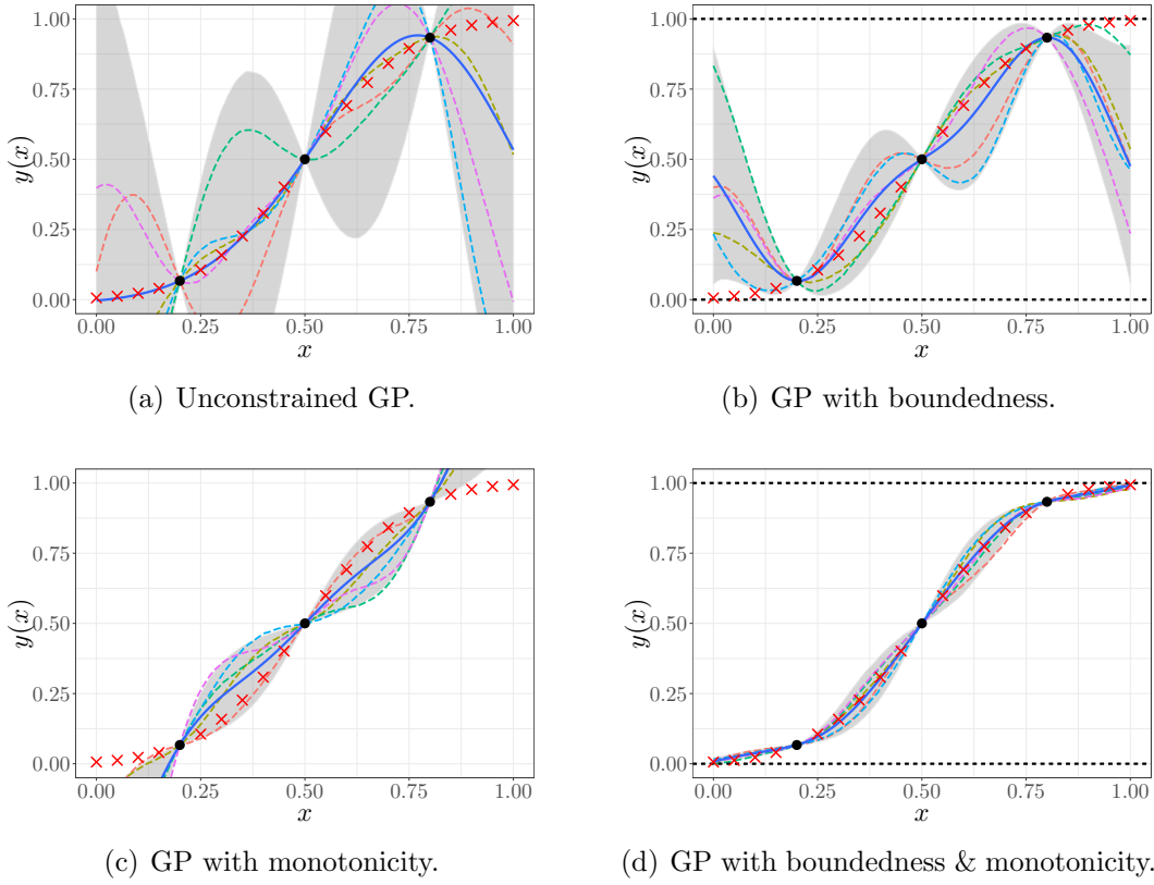
Figure 3.2: Example of Gaussian models satisfying different types of inequality constraints for interpolating the function x \mapsto \Phi(\frac{x-0.5}{0.2}) . Each panel shows: both training and test points (black dots and red crosses, respectively), the conditional mean function (blue solid line), the 90% confidence interval (grey region), and conditional realisations (dashed lines). For boundedness constraints, horizontal dashed lines denote the bounds.
