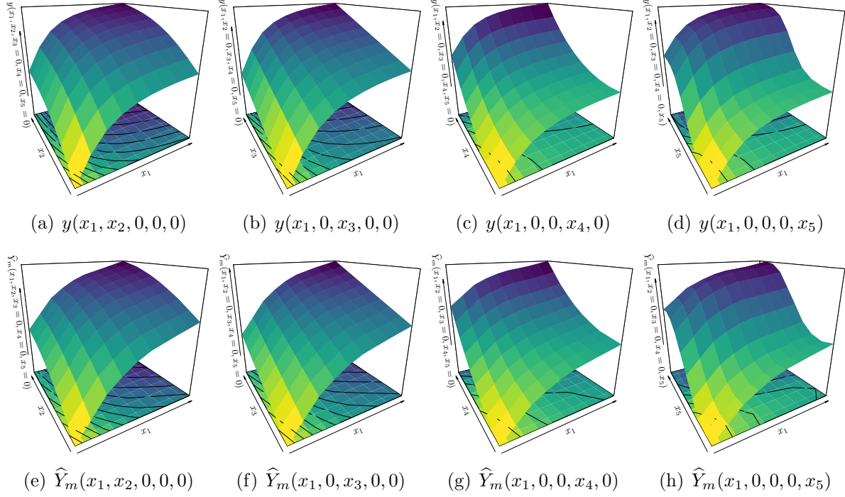
Figure 4.5: GP emulators under monotonicity constraints in 5D. True and predictive mean profiles are shown in the first and second row, respectively.
