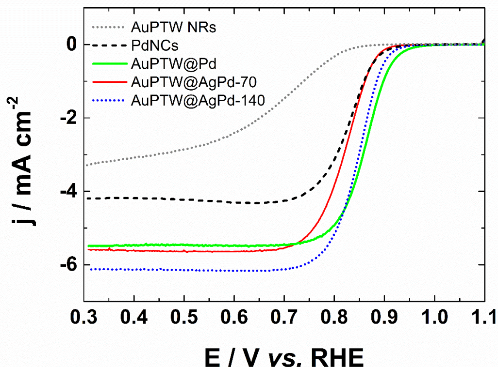
Figure VI.8: Linear polarization curves of the different NPs in 0.1 \text{ mol L}^{-1} KOH recorded at 5 \text{ mV s}^{-1} , at a temperature of 20^\circ\text{C} and at 1600 rpm.
