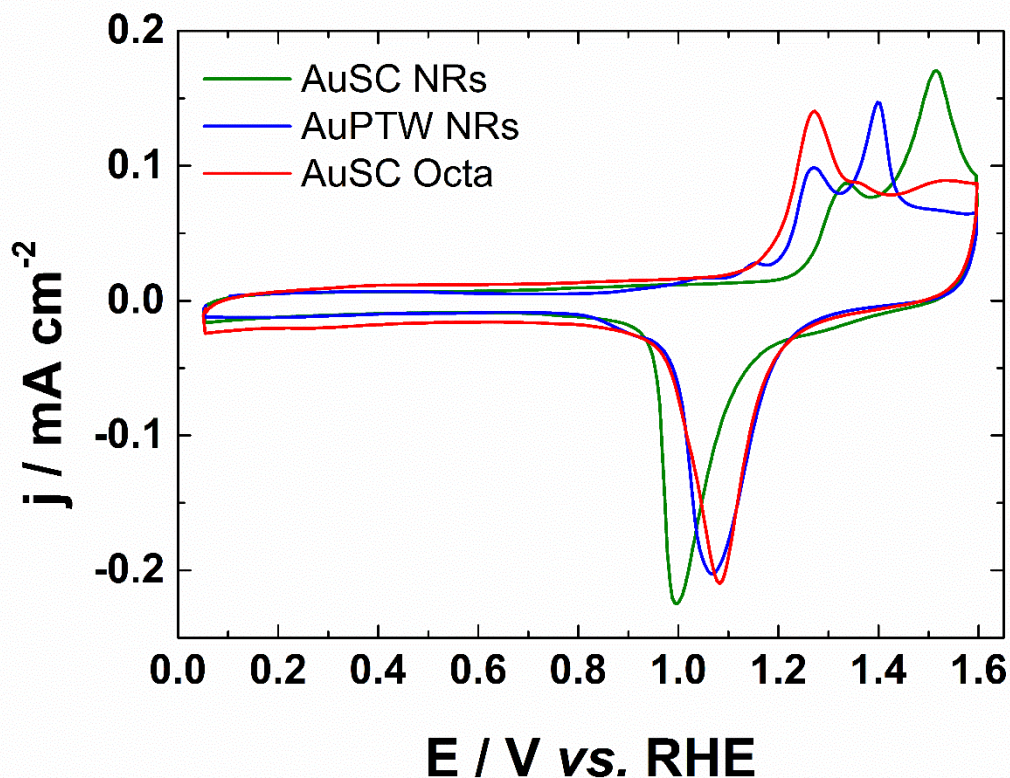
Figure V.3: Voltammograms of Au octahedrons (AuSC Octa), single crystal Au nanorods (AuSC NRs) and pentatwinned Au nanorods (AuPTW NRs) in 0.1 \text{ mol L}^{-1} \text{ NaOH} , recorded at 50 \text{ mV s}^{-1} and at a temperature of 25^\circ\text{C} .
