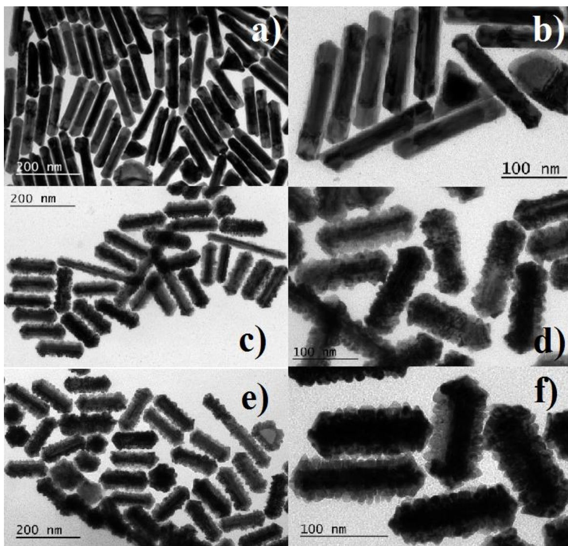
Figure VI.1: TEM images of the NPs. From up to down: a) and b) AuPTW@Pd, c) and d) AuPTW@AgPd-70, e) and f) AuPTW@AgPd-140.
