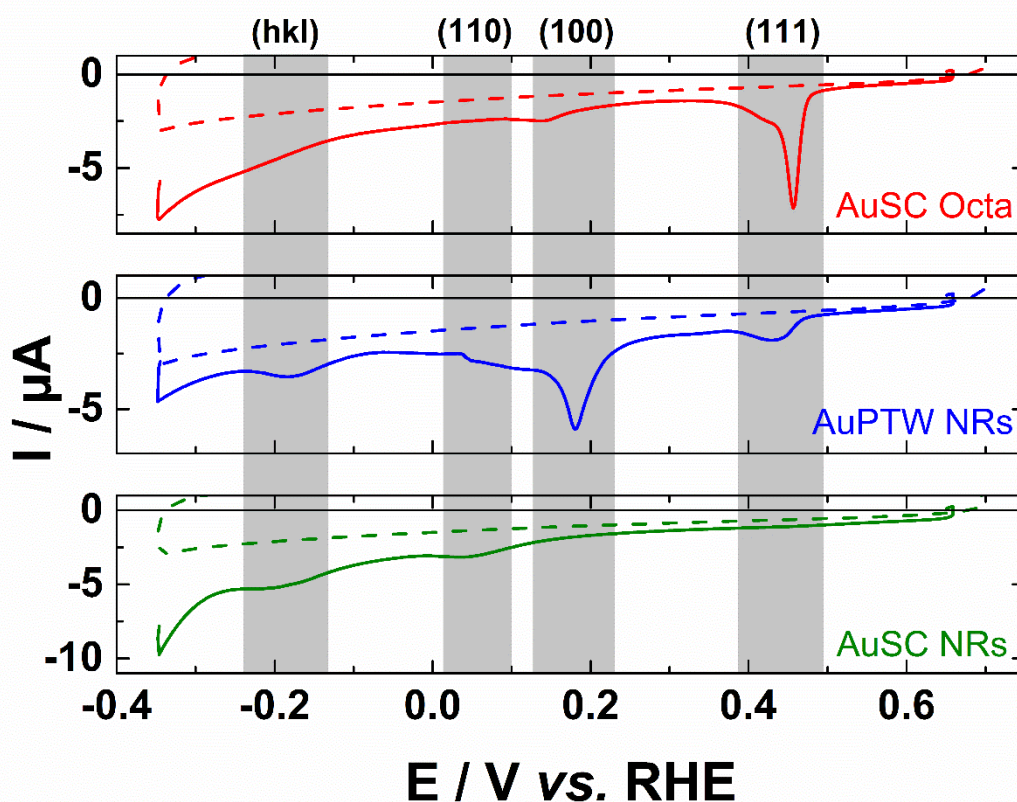
Figure V.7: Voltammograms of Au octahedrons (AuSC Octa), pentatwinned Au nanorods (AuPTW NRs) and single crystalline Au nanorods (AuSC NRs) in 0.5 \text{ mol L}^{-1} KOH recorded at 20 \text{ mV s}^{-1} at a temperature of 25^\circ\text{C} during the reductive desorption of a 4-MBA monolayer self-assembled onto the AuNPs' surface.
