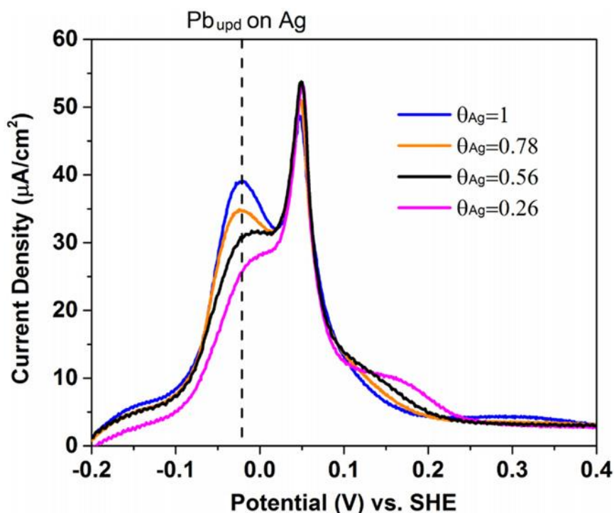
Figure III.10: Lead stripping voltammetric curves of Ag_{upd} -modified Au with different coverages ( \theta_{Ag} ) in 10 \text{ mmol L}^{-1} \text{ HClO}_4 + 0.2 \text{ mmol L}^{-1} \text{ Pb}(\text{ClO}_4)_2 at 20 \text{ mV s}^{-1} . Reprinted from reference [210]. Copyright (2017) with permission from Elsevier.
