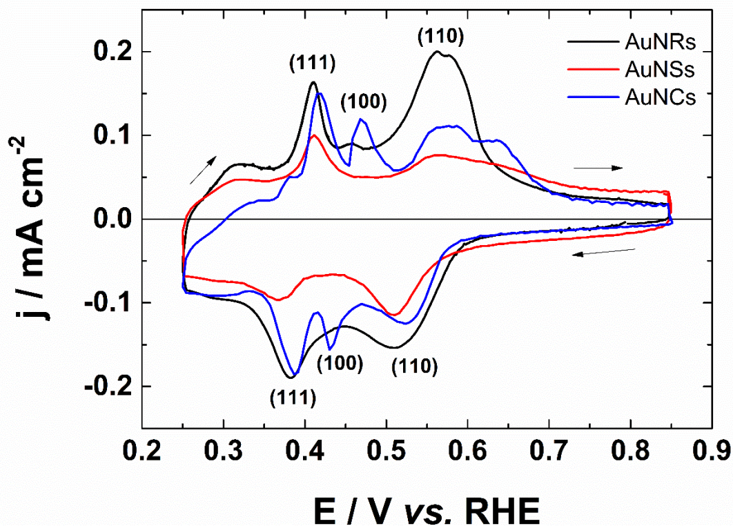
Figure III.11: Cyclic voltammograms of different AuNPs (nanospheres AuNSs, nanorods AuNRs and nanocubes AuNCs) in 0.1 \text{ mol L}^{-1} \text{ NaOH} + 1 \text{ mmol L}^{-1} \text{ Pb}(\text{NO}_3)_2 recorded at 20 \text{ mV s}^{-1} and at a temperature of 20^\circ\text{C} .
