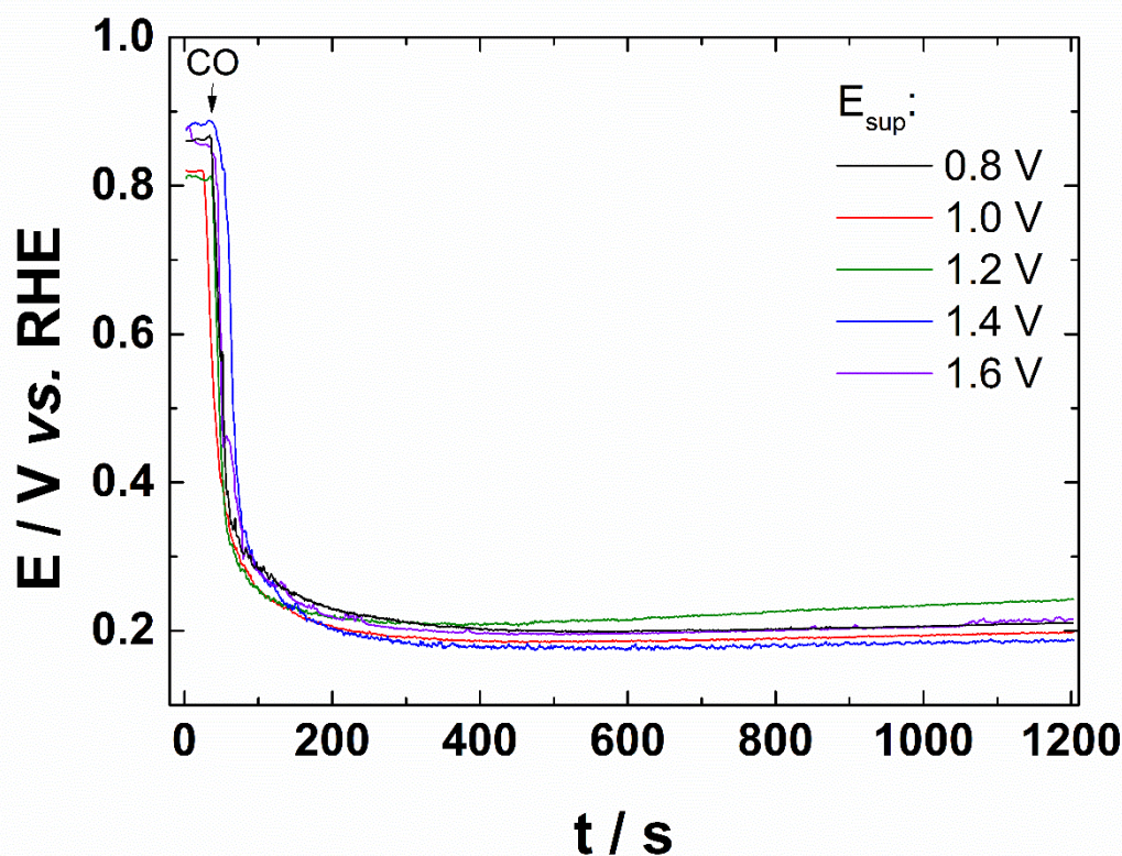
Figure IV.9: Potentiometric curves in 0.1 \text{ mol L}^{-1} NaOH recorded before and after the introduction of CO in the cell, corresponding to the evolution of the open-circuit potential.
