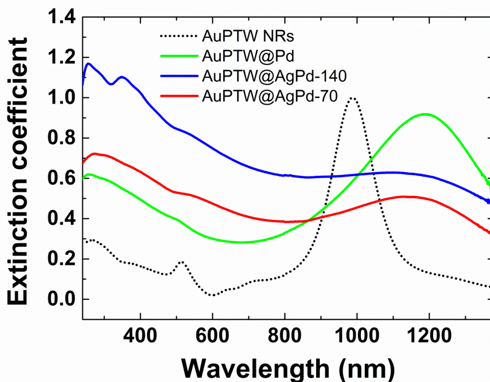
Figure VI.3: UV-vis NIR spectra of AuPTW NRs, AuPTW@Pd, AuPTW@AgPd-70 and AuPTW@AgPd-140.
