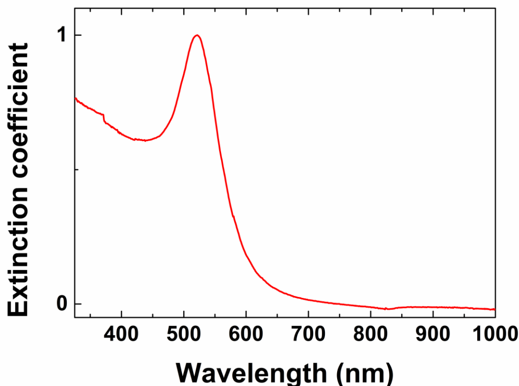
Figure IV.3: UV–visible spectrum of the colloidal solution containing gold nanoparticles.
