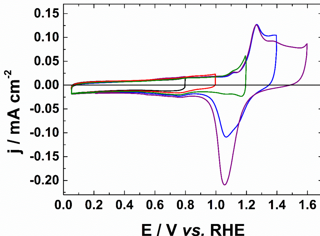
Figure IV.5: Cyclic voltammograms of AuNPs in 0.1 \text{ mol L}^{-1} NaOH recorded at 50 \text{ mV s}^{-1} at a temperature of 20^\circ\text{C} , for different upper potential limits (0.8 V, 1.0 V, 1.2 V, 1.4 V and 1.6 V vs. RHE).
