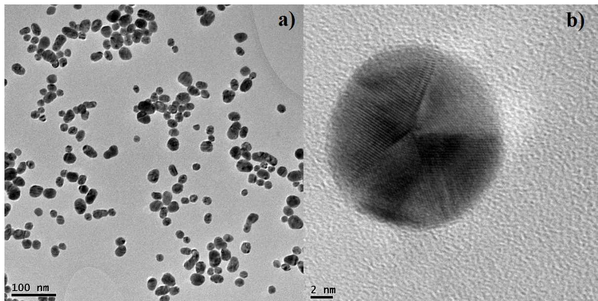
Figure IV.1: a) TEM image of the gold nanoparticles, b) HR-TEM of an isolated nanoparticle.
