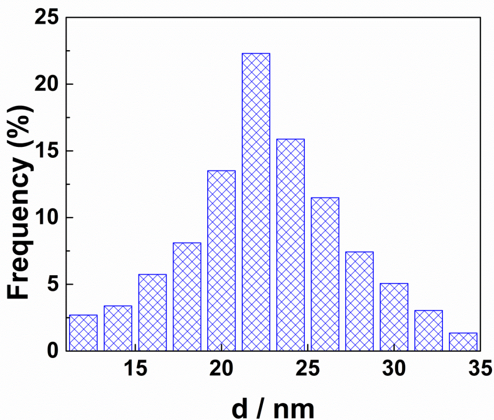
Figure IV.2: Distribution of the nanoparticles diameters (for about 300 nanoparticles).
