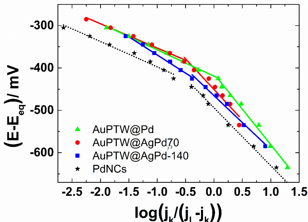
Figure VI.11: Tafel plots obtained for each material.
