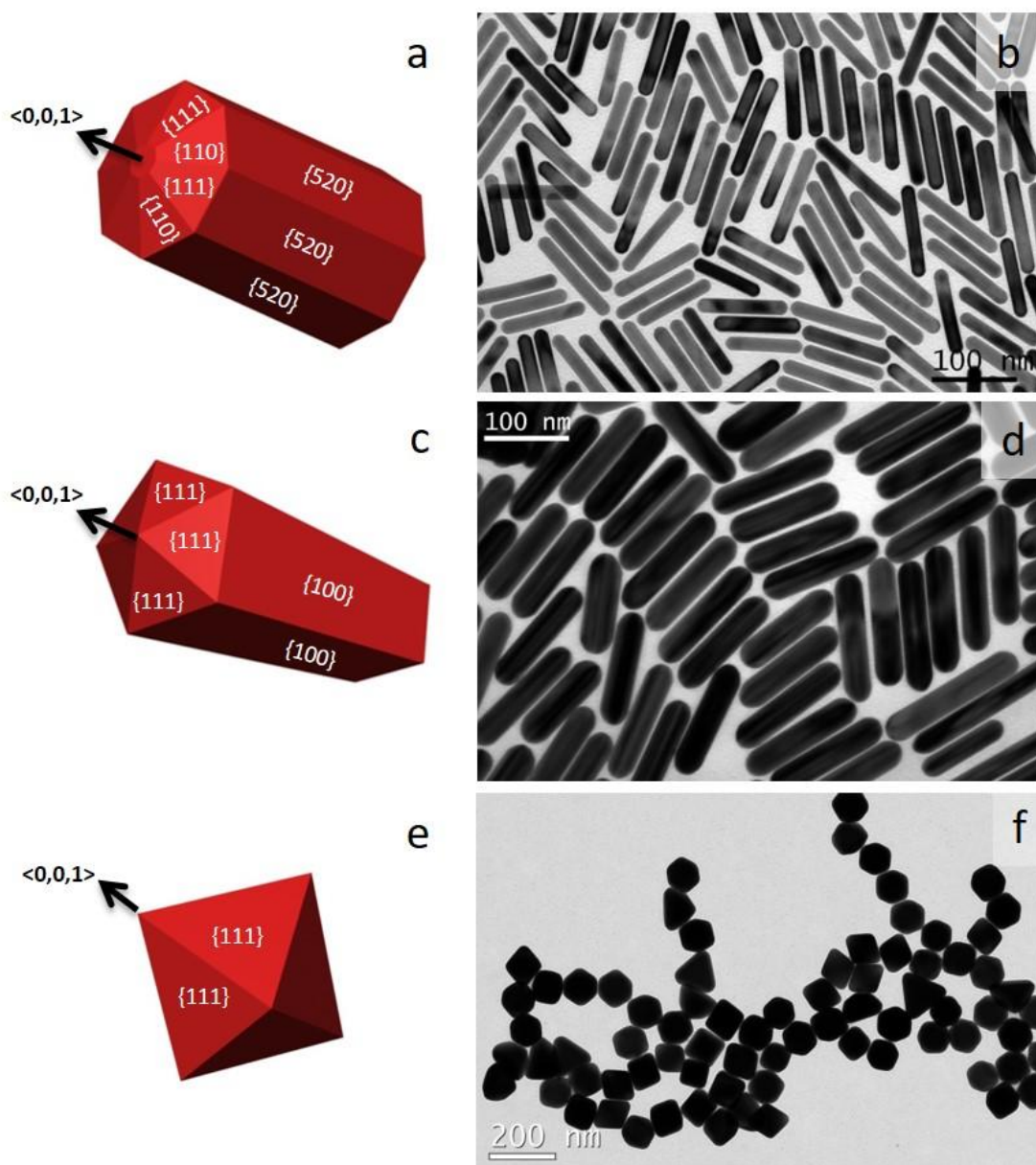
Figure V.2: Models and TEM images of: a), b) single crystalline Au nanorods (AuSC NRs), c), d) pentatwinned Au nanorods (AuPTW NRs) and e) ,f) single crystalline Au octahedrons (AuSC Octa).
