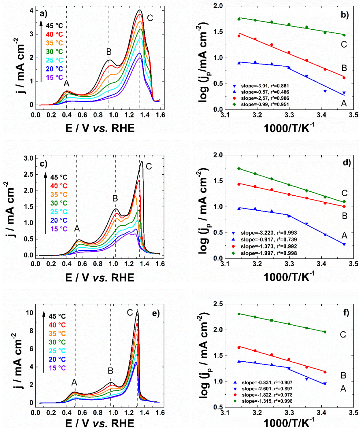
Figure V.9: a), c), e) Voltammograms of AuSC NRs, AuPTW NRs and AuSC Octa, respectively, in 0.1 mol L -1 NaOH + 10 mmol L -1 glucose (positive scan) recorded at 20 mV s -1 and at controlled temperatures ; b), d), f) Plots of log(j peak ) as a function of 1/T for AuSC NRs, AuPTW NRs and AuSC Octa, respectively.
