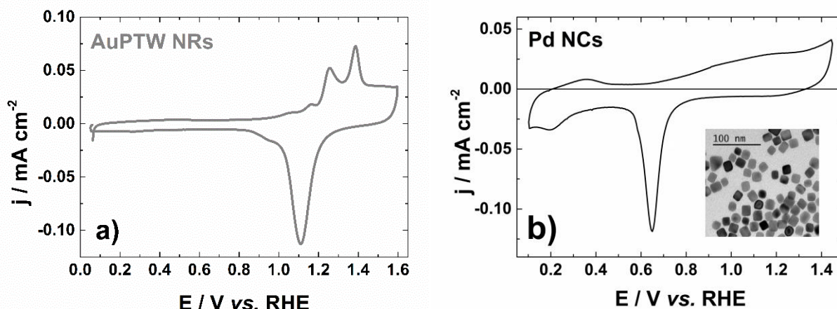
Figure VI.4: Cyclic voltammograms of: a) AuPTW NRs and b) PdNCs in 0.1 \text{ mol L}^{-1} KOH recorded at 20 \text{ mV s}^{-1} at a temperature of 20^\circ\text{C} .
