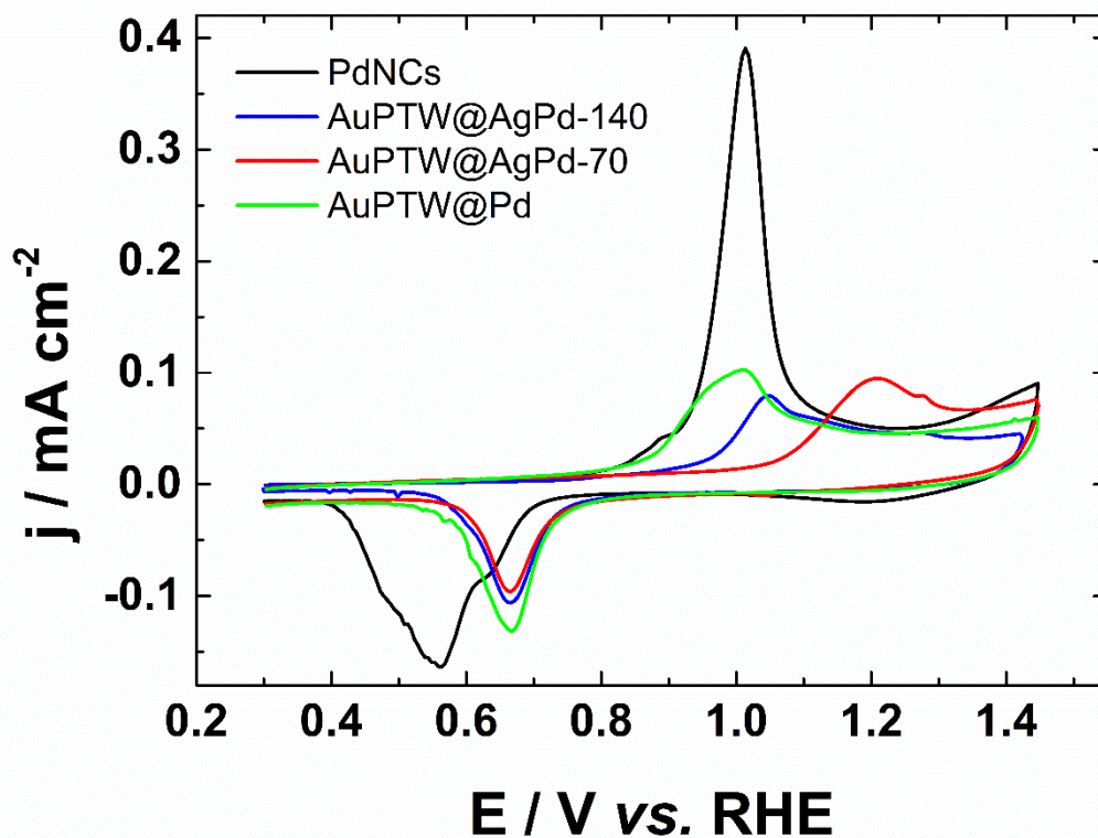
Figure VI.7: First cyclic voltammograms of each material towards CO-stripping in 0.1 \text{ mol L}^{-1} KOH recorded at 20 \text{ mV s}^{-1} and at a temperature of 20^\circ\text{C} .
