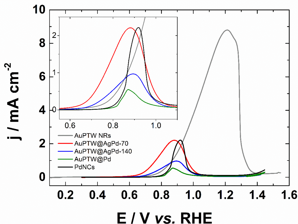
Figure VI.14: Cyclic voltammograms (forward scan) of the different nanoparticles in 0.1 \text{ mol L}^{-1} \text{ NaOH} + 0.1 \text{ mol L}^{-1} \text{ glycerol} recorded at 20 \text{ mV s}^{-1} at a temperature of 25^\circ\text{C} .
