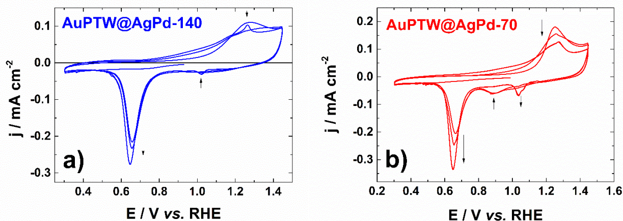
Figure VI.6: Cyclic Voltammograms of: a) AuPTW@AgPd–140 and b) AuPTW@AgPd–70 in 0.1 mol L -1 KOH recorded at 50 mV s -1 and at a temperature of 20°C. First, second and 10 th cycles are displayed.
