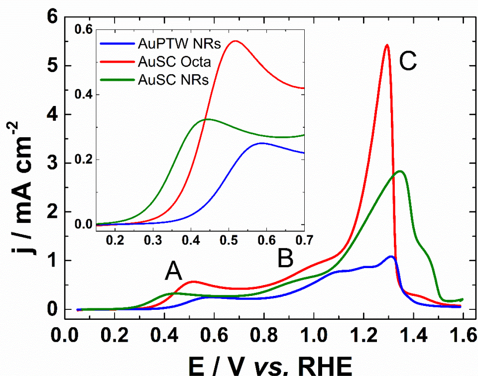
Figure V.8: Voltammograms of Au octahedrons (AuSC Octa), pentatwinned Au nanorods (AuPTW NRs) and single crystalline Au nanorods (AuSC NRs) in 0.1 mol L -1 NaOH + 10 mmol L -1 glucose (positive scan) recorded at 20 mV s -1 and at a temperature of 25°C.
