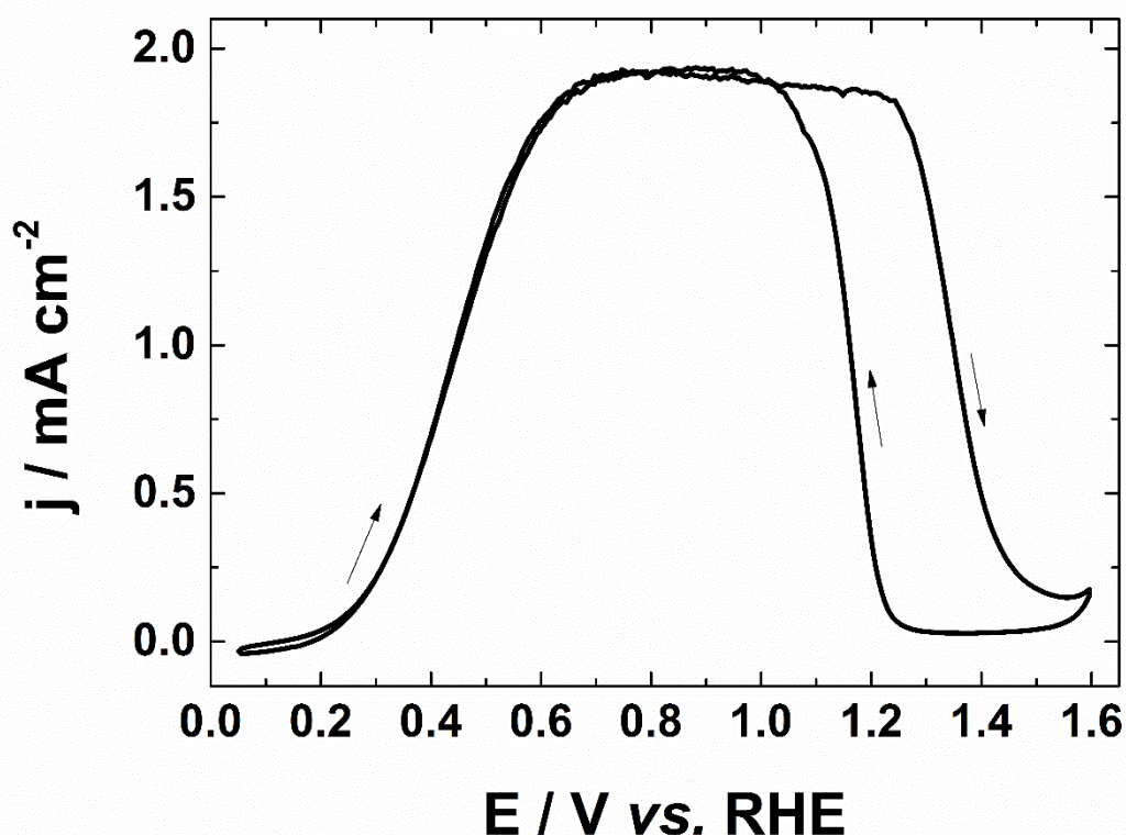
Figure IV.10: Cyclic voltammogram of AuNPs in CO-saturated 0.1 mol L -1 NaOH recorded at 50 mV s -1 at a temperature of 20°C and at 1600 rpm.
