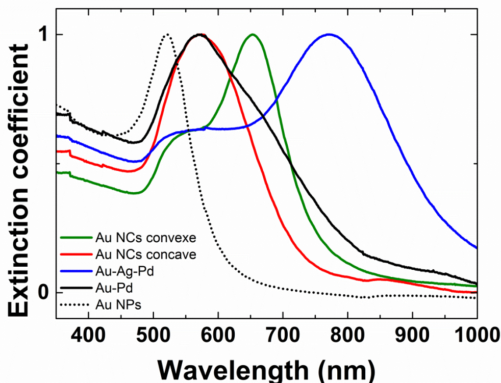
Figure VII.3: UV–visible spectra of the gold-based nanoparticles, dispersed in water.
