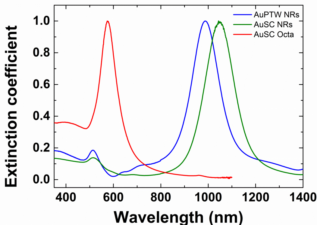
Figure V.1: NIR-Visible absorption spectra of AuNPs in aqueous solution.
