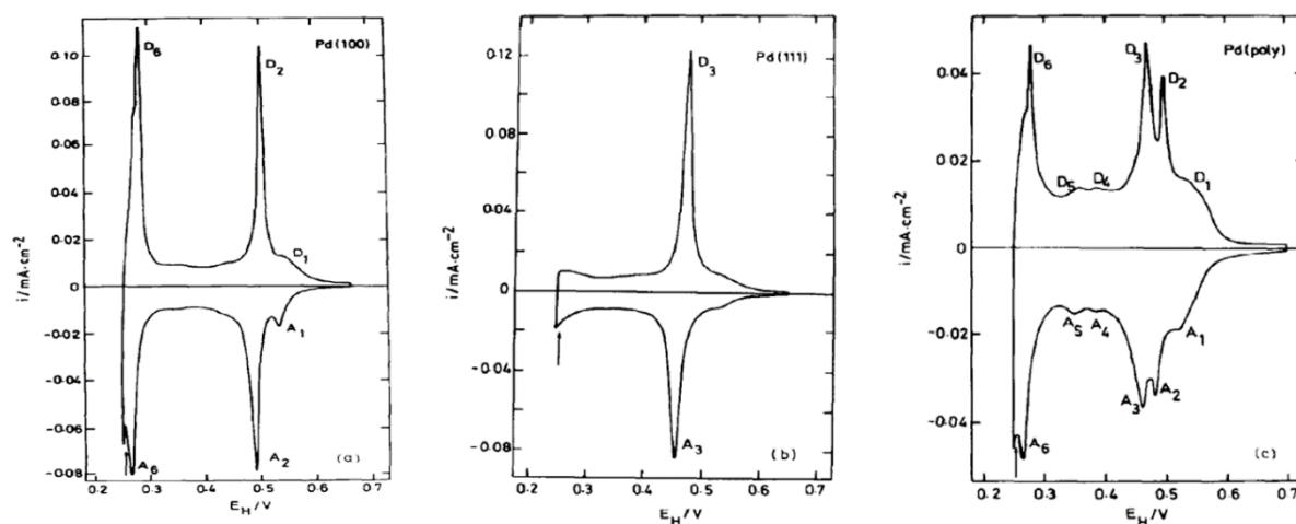
Figure III.14: Cyclic voltammograms of Pd single-crystal electrodes in 0.5 \text{ mol L}^{-1} \text{ NaClO}_4 + 0.01 \text{ mol L}^{-1} \text{ HClO}_4 + 1 \text{ mmol L}^{-1} \text{ Cu}^{2+} , at 10 \text{ mV s}^{-1} : a) Pd(100), b) Pd(111), c) polycrystalline Pd. Reprinted from reference [425]. Copyright (1988) with permission from Elsevier.
