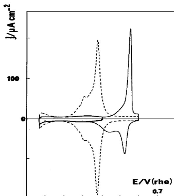
Figure III.13: Voltammograms of a Pt(100) surface fully covered with Ge (continuous line) and Pt(100) blank. Reprinted from. Reference [390]. Copyrights (1992) with permission from Elsevier.
