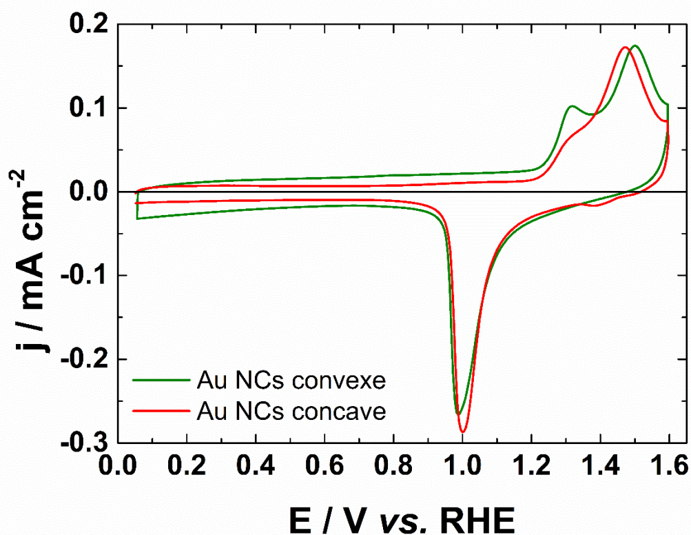
Figure VII.4: Cyclic voltammograms of Au NCs nanoparticles in 0.1 mol L -1 NaOH recorded at 50 mV s -1 at a temperature of 20°C.
