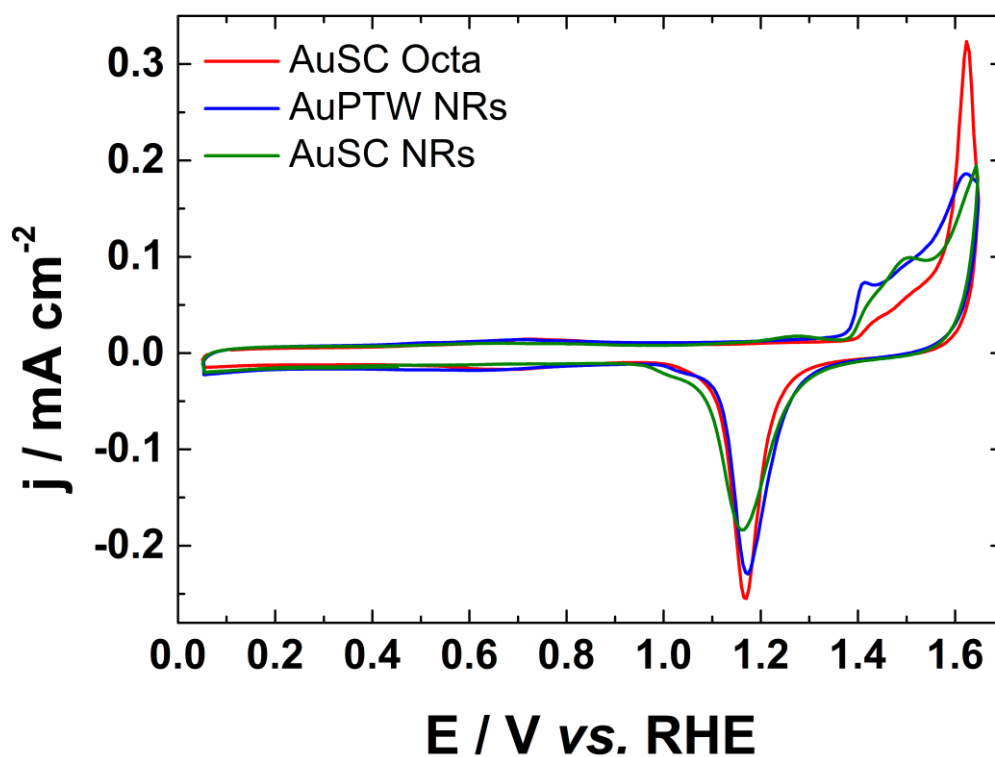
Figure V.5: Voltammograms of Au octahedrons (AuSC Octa), single Au crystal nanorods (AuSC NRs) and pentatwinned Au nanorods (AuPTW NRs) in 0.5 \text{ mol L}^{-1} \text{ H}_2\text{SO}_4 , recorded at 50 \text{ mV s}^{-1} and at a temperature of 25^\circ\text{C} .
