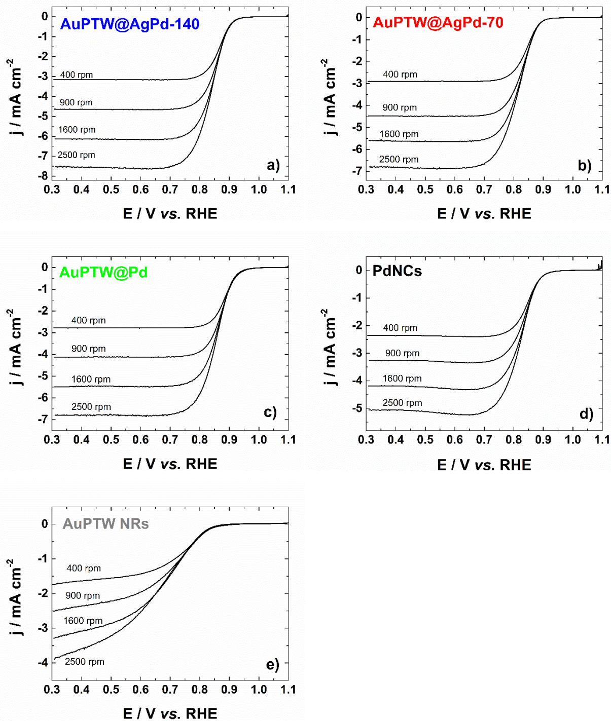
Figure VI.9: Linear polarizations of the different NPs at different rotation speeds in 0.1 mol L -1 KOH recorded at 5 mV s -1 and at a temperature of 20°C.
