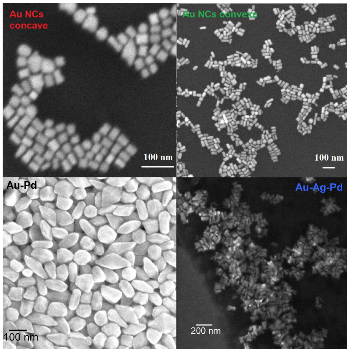
Figure VII.2: Scanning electron microscopy images of the nanoparticles: a) Au NCs concave, b) Au NCs convexe, c) Au–Pd NPs and d) Au–Ag–Pd NPs.
