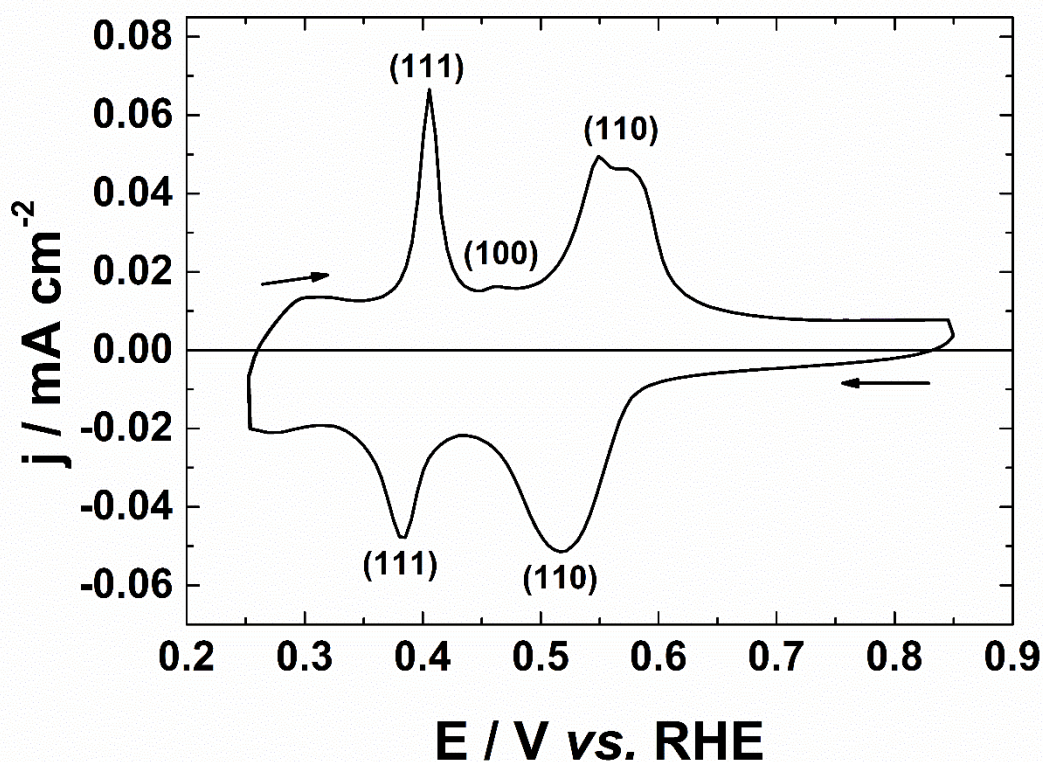
Figure IV.6: Voltammetric upd profile of AuNPs in 0.1 \text{ mol L}^{-1} \text{ NaOH} + 1 \text{ mmol L}^{-1} \text{ Pb}(\text{NO}_3)_2 recorded at 20 \text{ mV s}^{-1} at a temperature of 20^\circ\text{C} .
