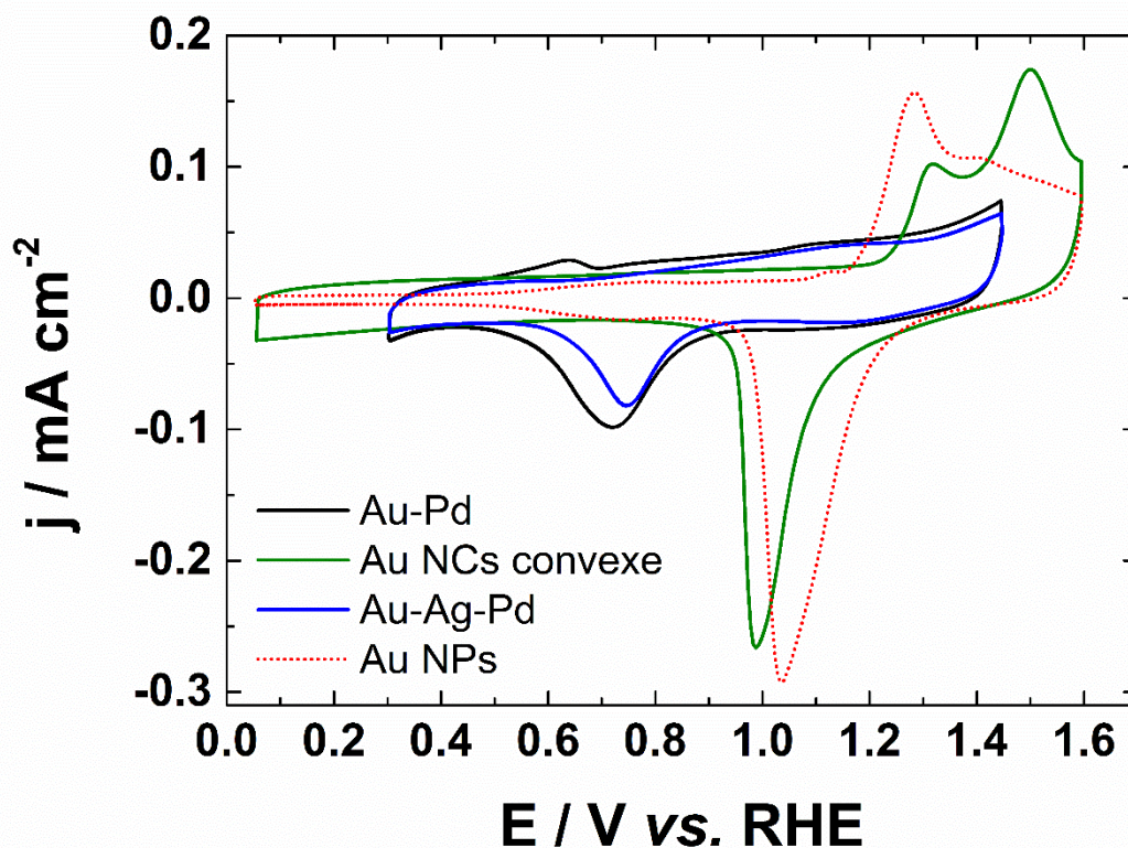
Figure VII.6: Cyclic voltammograms of gold and gold-based nanoparticles in 0.1 mol L -1 NaOH recorded at 50 mV s -1 at a temperature of 20°C.
