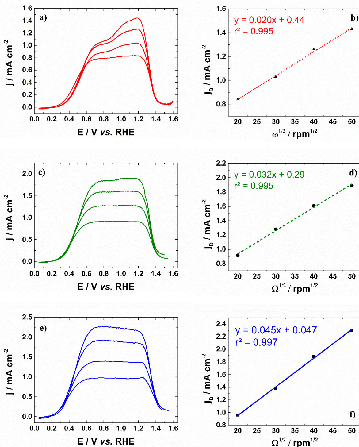
Figure IV.12: Cyclic voltammetry (forward scan) on AuNPs in CO-saturated 0.1 mol L -1 NaOH recorded at: a) 10 mV s -1 , c) 20 mV s -1 and e) 50 mV s -1 , at a temperature of 20°C and at different electrode rotation speeds (400, 900, 1600 and 2500 rpm); b), d), f) Levich curves plotted from the cyclic voltammograms showed at left, at 1.0 V vs. RHE, for forward scans at different scan rates.
