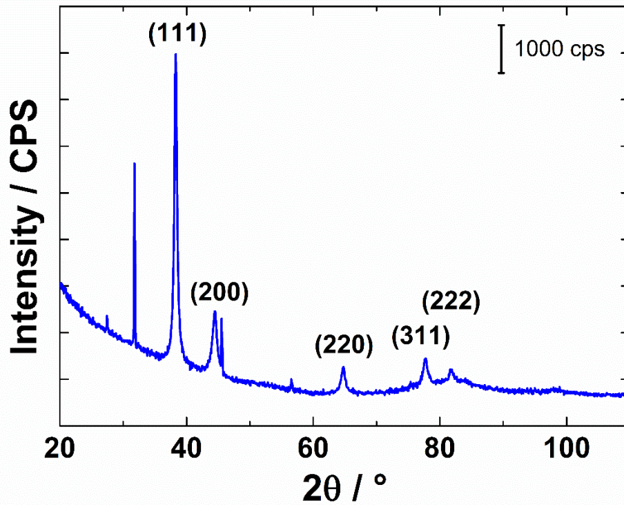
Figure IV.4: Diffractogram of AuNPs.
