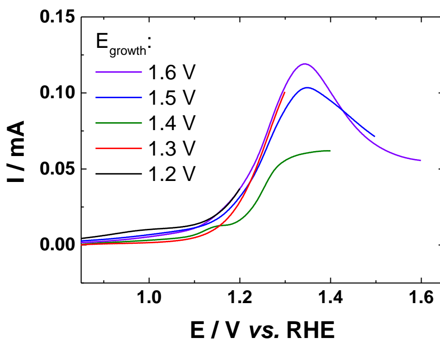
Figure IV.7: Linear polarization on AuNPs from 0.05 V vs. RHE to E_{\text{growth}} in 0.1 \text{ mol L}^{-1} NaOH recorded at 50 \text{ mV s}^{-1} at a temperature of 20^\circ\text{C} .
