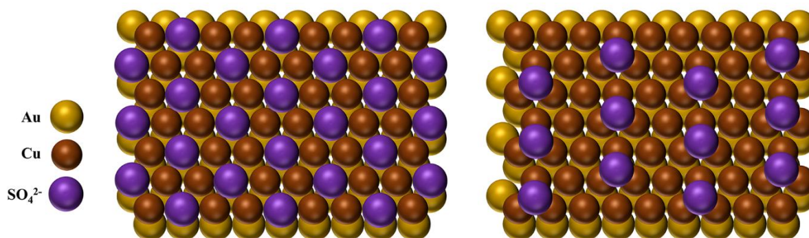
Figure III.3: Model of the (\sqrt{3} \times \sqrt{3}) sulfate structure with 2/3 of Cu monolayer (left) and (\sqrt{3} \times \sqrt{7}) sulfate structure on the first pseudomorphic monolayer of Cu underpotentially deposited (right) on Au (111).
