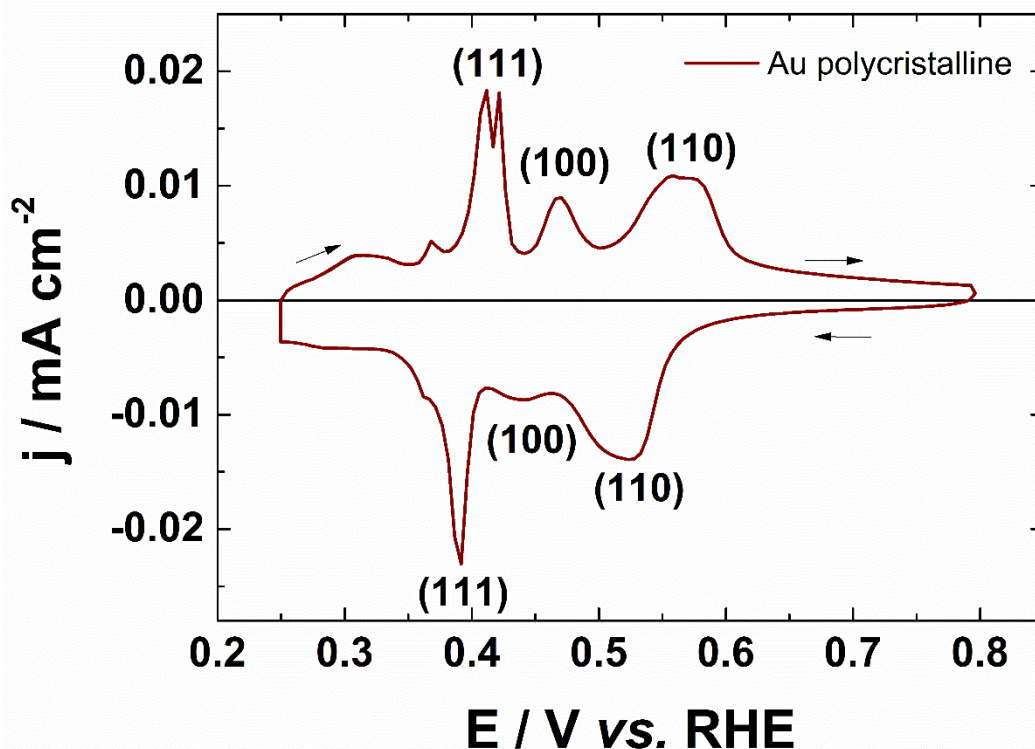
Figure III.7: Cyclic voltammogram of Au polycrystalline in 0.1 \text{ mol L}^{-1} \text{ NaOH} + 1 \text{ mmol L}^{-1} \text{ Pb}(\text{NO}_3)_2 , recorded at 20 \text{ mV s}^{-1} and at a temperature of 20^\circ\text{C} .
