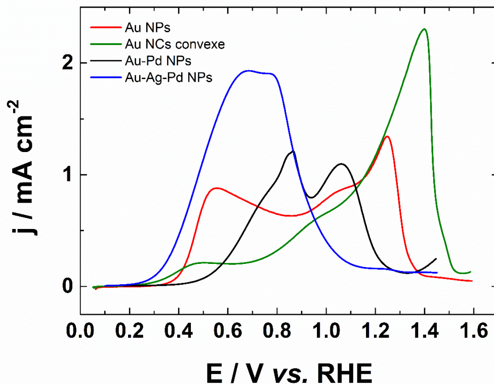
Figure VII.7: Cyclic voltammograms of gold and gold-based nanoparticles in 0.1 \text{ mol L}^{-1} NaOH + 10 \text{ mmol L}^{-1} glucose recorded at 20 \text{ mV s}^{-1} at a temperature of 20^\circ\text{C} .
