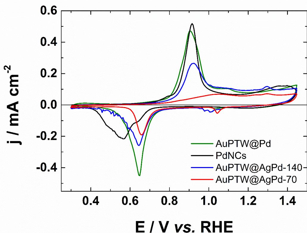
Figure VI.13: First cyclic voltammograms towards CO-stripping of the different NPs in 0.1 \text{ mol L}^{-1} \text{ NaOH} recorded at 20 \text{ mV s}^{-1} at a temperature of 20^\circ\text{C} .
