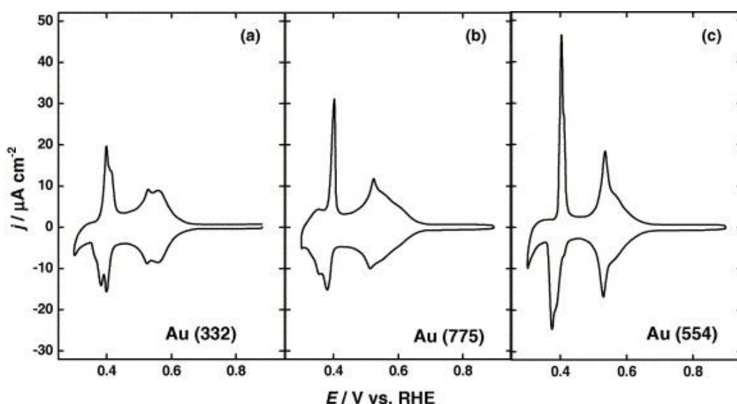
Figure III.4: Cyclic voltammograms of a) Au(332); b) Au(775); c) Au(554) in 0.05 \text{ mol L}^{-1} \text{ H}_2\text{SO}_4 + 1 \text{ mmol L}^{-1} \text{ CuSO}_4 at 5 \text{ mVs}^{-1} . Reprinted from reference [63]. Copyright (2004) with permission from Elsevier.
