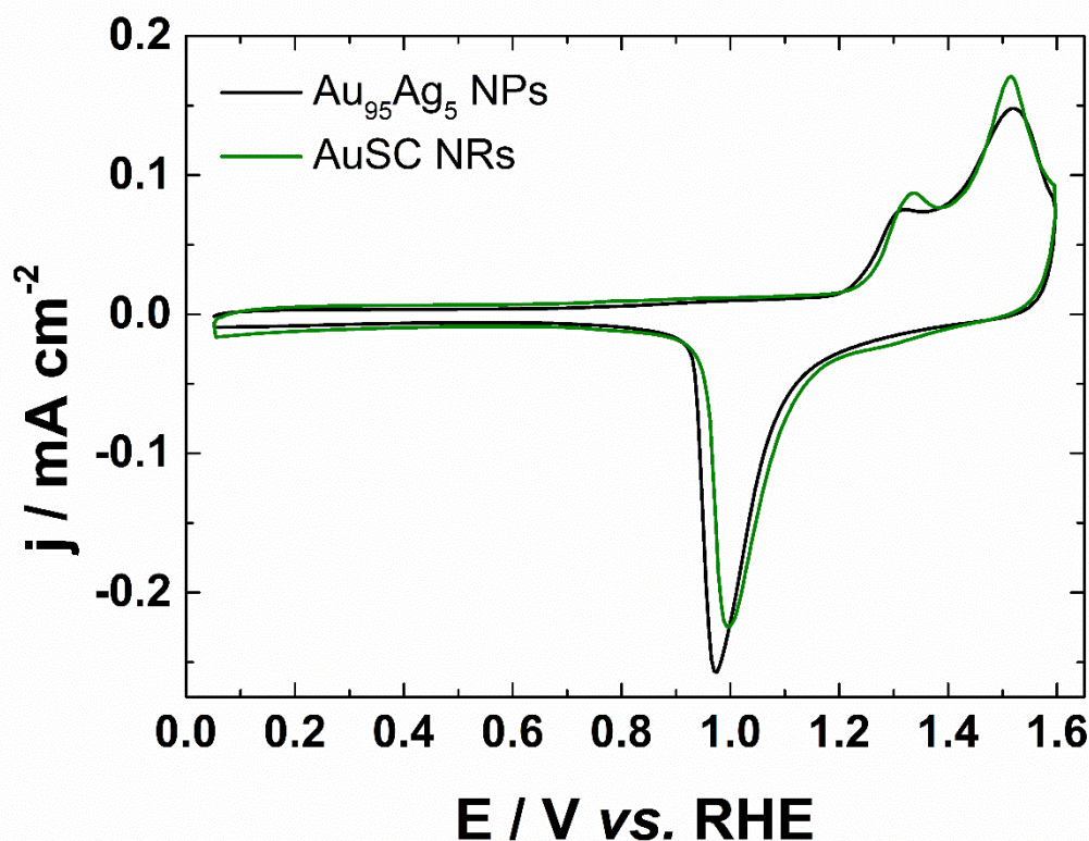
Figure V.4: Voltammograms of AuSC NRs and Au 95 Ag 5 NPs in 0.1 mol L -1 NaOH recorded at 50 mV s -1 at a temperature of 25°C.
