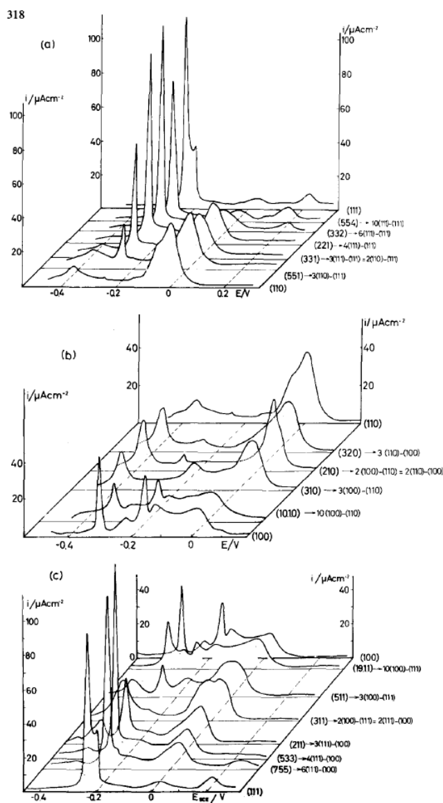
Figure III.8: Cyclic voltammograms for the stripping of \text{Pb}_{\text{upd}} on \text{Au}(\text{hkl}) electrodes in 10 \text{ mmol L}^{-1} \text{ HClO}_4 + 1 \text{ mmol L}^{-1} \text{ PbF}_2 . \text{Au}(\text{hkl}) surfaces are from the three main zones of the projected stereographic triangle: a ) (111)–(110) zone, b ) (110)–(100) zone, c ) (100)–(111) zone. All the surfaces are identified with Miller index notation and with the step notation. Reprinted from reference [85]. Copyright (1984) with permission from Elsevier.
