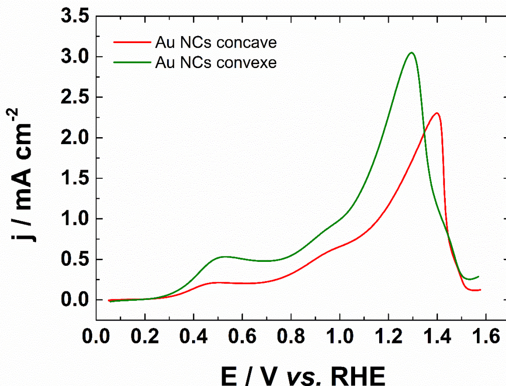
Figure VII.5: Cyclic voltammograms of Au NCs nanoparticles in 0.1 mol L -1 NaOH + 10 mmol L -1 glucose recorded at 20 mV s -1 at a temperature of 20°C.
