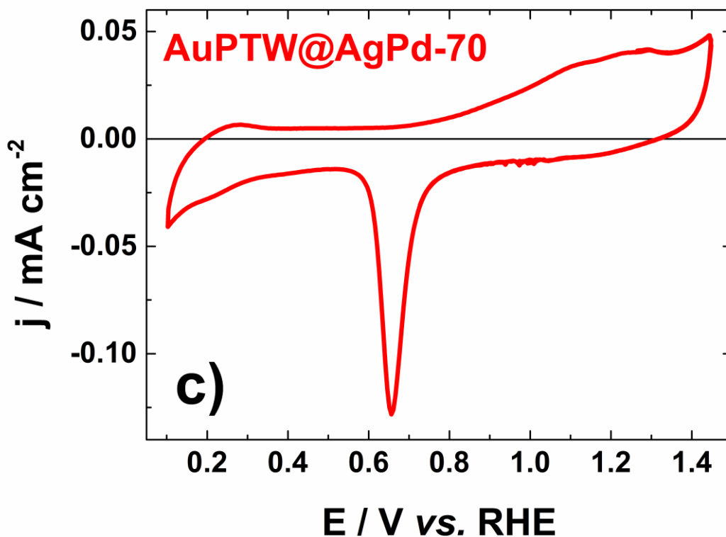
Figure VI.5: Cyclic Voltammograms of: a) AuPTW@Pd, b) AuPTW@AgPd-140, c) AuPTW@AgPd-70 in 0.1 mol L -1 KOH recorded at 20 mV s -1 and at a temperature of 20°C.
