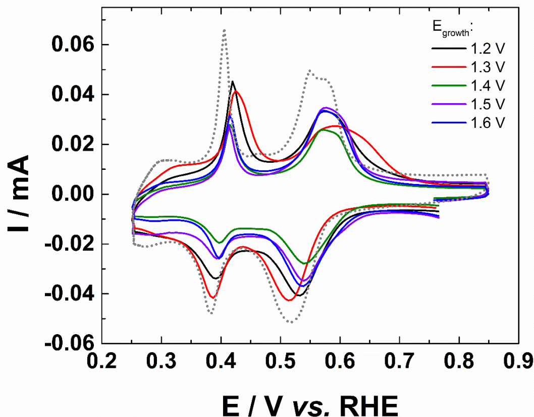
Figure VI.8: Voltammetric upd profiles of AuNPs in 0.1 \text{ mol L}^{-1} \text{ NaOH} + 1 \text{ mmol L}^{-1} \text{ Pb(NO}_3)_2 recorded at 20 \text{ mV s}^{-1} at a temperature of 20^\circ\text{C} after polarization at E_{\text{growth}} . Dashed line represents upd profile without the oxide growth step.
