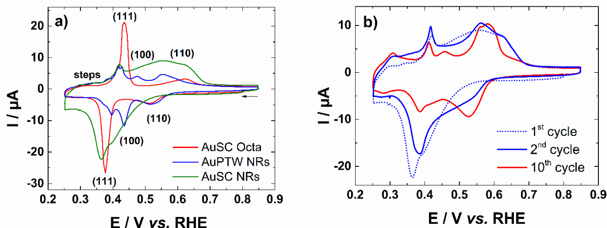
Figure V.6: a) Voltammetric upd profiles of Au octahedrons (AuSC Octa), single crystal Au nanorods (AuSC NRs) and pentatwinned Au nanorods (AuPTW NRs) in 0.1 \text{ mol L}^{-1} \text{ NaOH} + 1 \text{ mmol L}^{-1} \text{ Pb}(\text{NO}_3)_2 recorded at 20 \text{ mV s}^{-1} and at a temperature of 25^\circ\text{C} ; b) Different cycles of voltammetric upd profiles of AuSC NRs in 0.1 \text{ mol L}^{-1} \text{ NaOH} + 1 \text{ mmol L}^{-1} \text{ Pb}(\text{NO}_3)_2 recorded at 20 \text{ mV s}^{-1} and at a temperature of 25^\circ\text{C} .
