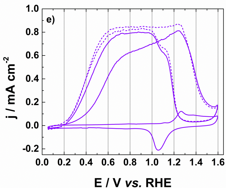
Figure IV.11: First cyclic voltammograms of AuNPs towards CO oxidation in 0.1 mol L -1 NaOH recorded at 50 mV s -1 at a temperature of 20°C and at 400 rpm according to the upper potential limit ( E_{\text{sup}} ): a) 0.8 V, b) 1.0 V, c) 1.2 V, d) 1.4 V, e) 1.6 V vs. RHE. Solid line is
