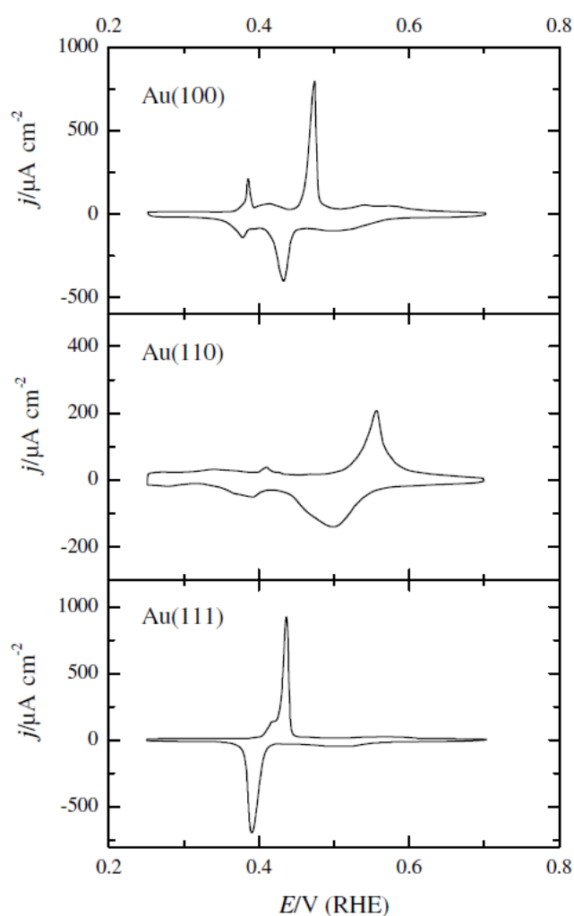
Figure III.9: Cyclic voltammograms of Au(100), Au(110) and Au(111) in 0.1 mol L -1 NaOH + 1 mmol L -1 Pb(NO 3 ) 2 at 50 mV s -1 . Reprinted from reference [253]. Copyright (2004) with permission from Elsevier.
