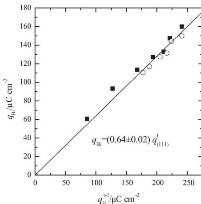
Figure III.12: Charge density values of the bismuth redox peak vs. the charge associated with the (111) sites on the terraces, assuming that one electron is exchanged per site
