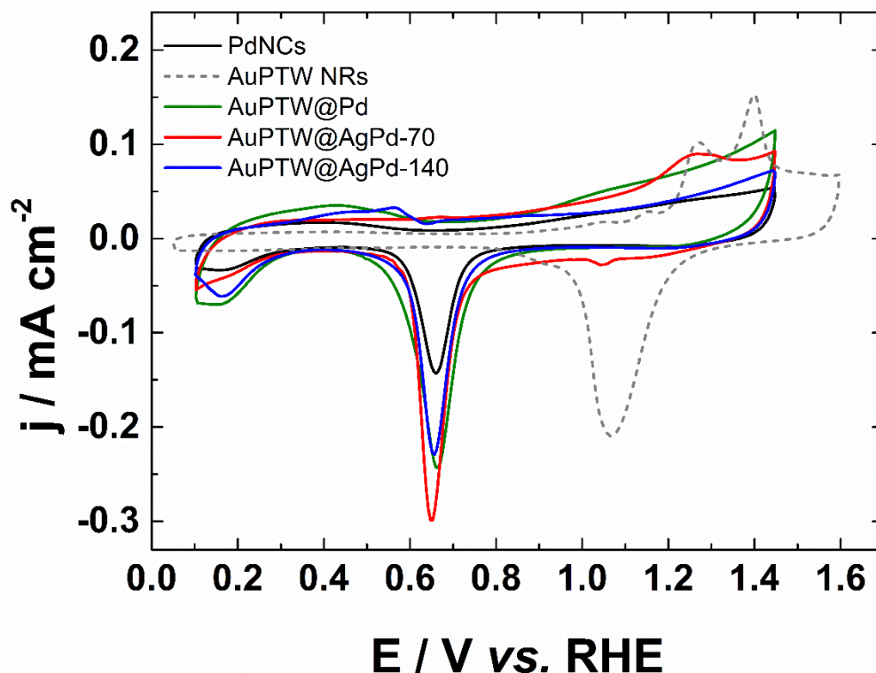
Figure VI.12: Cyclic voltammograms of the different nanoparticles in 0.1 \text{ mol L}^{-1} NaOH recorded at 50 \text{ mV s}^{-1} at a temperature of 20^\circ\text{C} .
