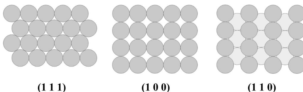
Figure III.2. Representation of the three low Miller indices for a faces centered cubic system.
