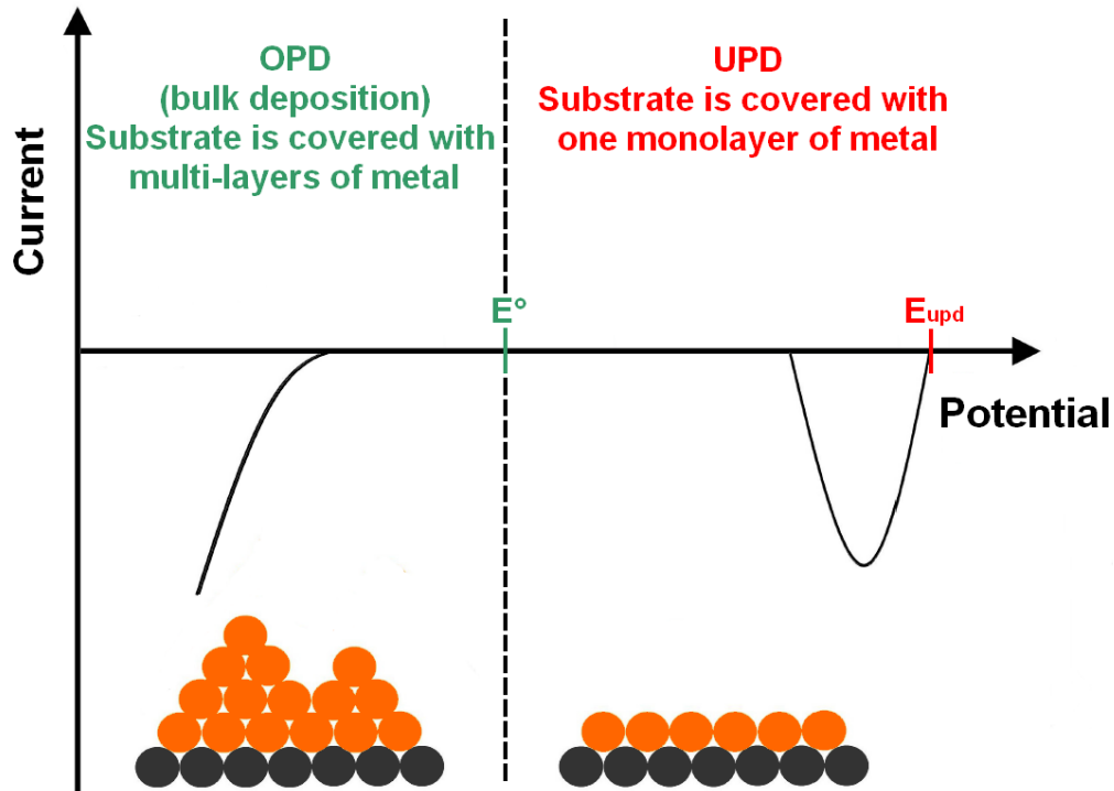
Figure III.1. Schematic profile of a voltammetric curve showing the upd and opd processes of a metal (in orange) on a foreign substrate (in black).
