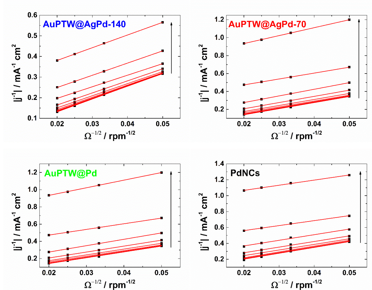
Figure VI.10: Koutecky-Levich plots obtained on each material for different values of potentials.
