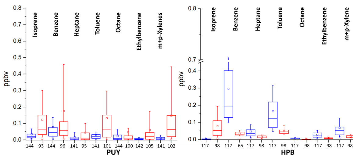
Figure III-15 Seasonal distribution of VOC concentrations (ppbv) in summer June and July (red boxplots) and in winter January and February (blue boxplots) 2012 and 2013 at PUY (A) and HPB (B) for VOC. The number of samples analyzed is indicated under each box plot. The bottom and top of box plots are the 25 th and 75 th percentiles, respectively. The full line and the open square represent the median and mean values, respectively. The “-” represents 10 th and 90 th percentiles.
