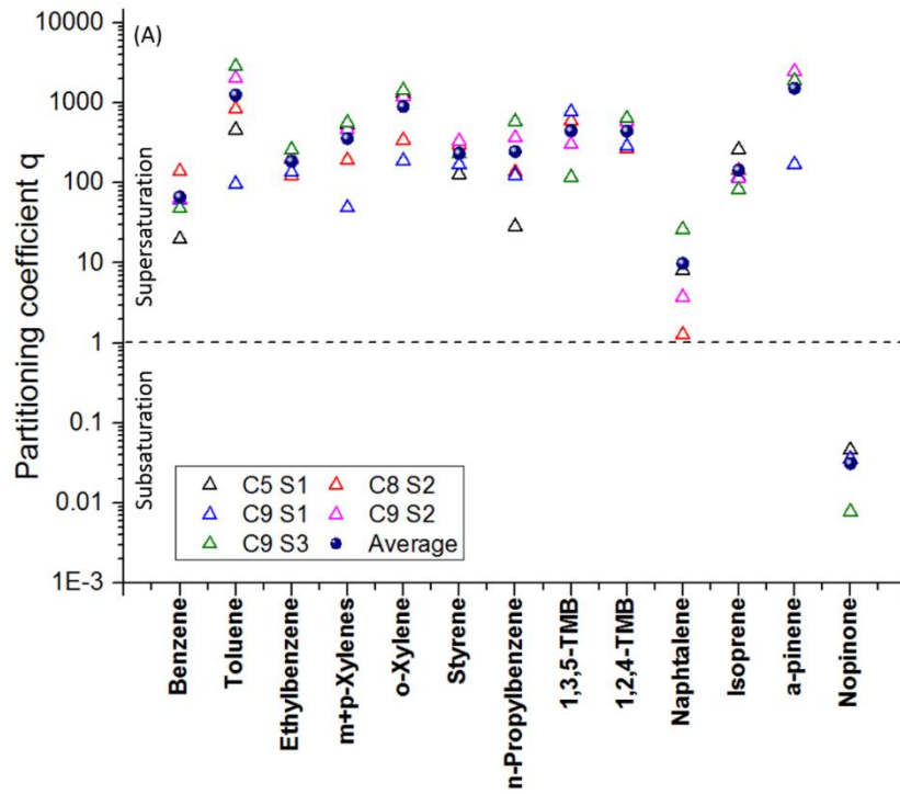
Figure III-19 q factors calculated for each cloud sample and for each chemical compound (blue circles correspond to mean values).
