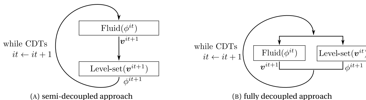
FIGURE 4.18 – Problem solving marching - iterative coupling strategy
