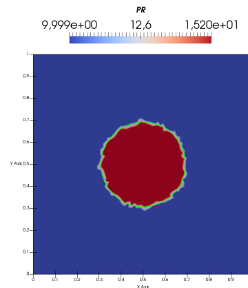
FIGURE 4.11 – Static bubble - Pressure field h_e = 1/50
