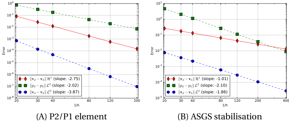
FIGURE 2.3 – Manufactured Solution for steady Navier Stokes- Convergence orders in the case of a turbulent flow with \mathcal{R}e = 5025
