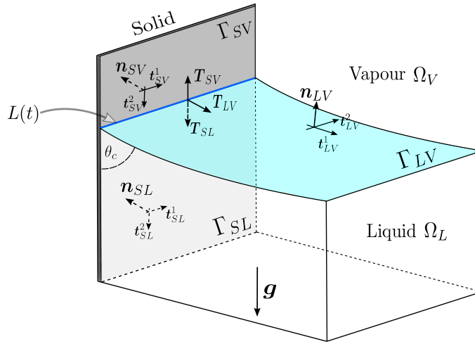
FIGURE 1.1 – Schematic description of notations for a capillary flow - a liquid meniscus against a rigid wall [58]
