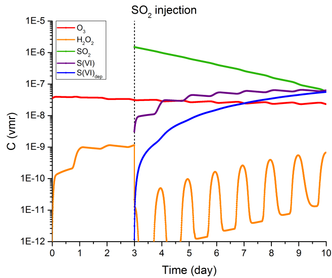
Figure 5.4: Gas-phase concentrations time evolution for \text{SO}_2 , its tropospheric oxidants and produced and deposited sulphates during C2 (see text); no halogens are released within the plume.
