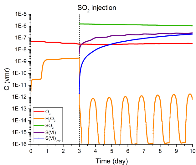
Figure 4.7: Time evolution in the gas-phase concentrations of \text{SO}_2 , its tropospheric oxidants and produced and deposited sulphates during S3. During S3 simulation the concentration of injected \text{SO}_2 drops from 1.5 ppmv to a final value of 1 ppmv.
