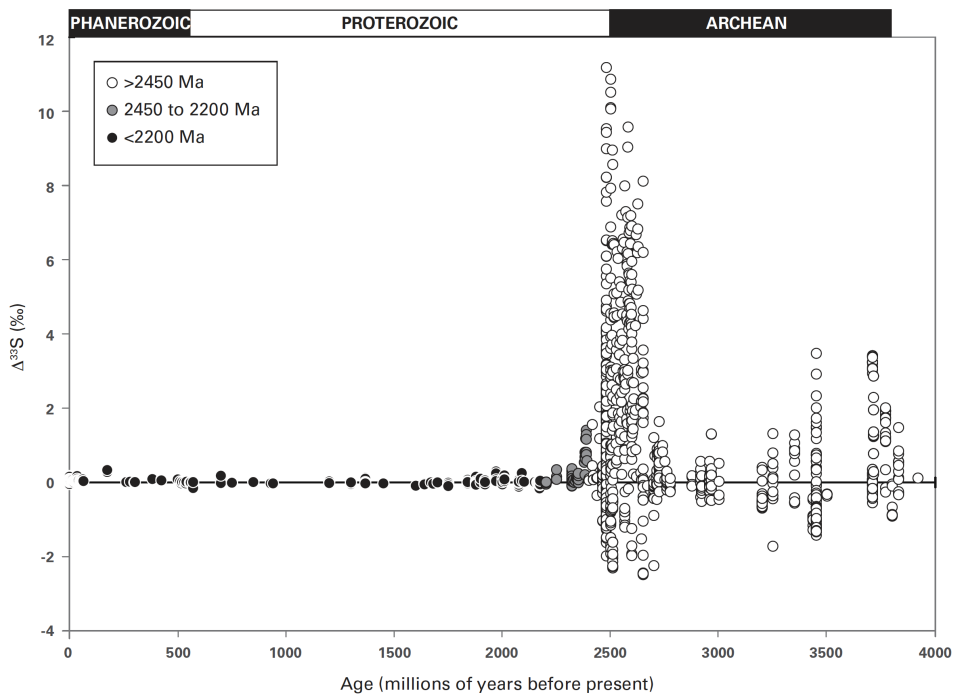
Figure 1.8: The upper figure shows the relation between \delta^{34}\text{S} and \delta^{33}\text{S} in terrestrial sulphur. Deviations from the TFL represent the magnitude of S-MIF. The lower plot shows the change in \Delta^{33}\text{S} reported in sulphides and sulphates collected from sediment rocks formed before and after the Archean era. Deviations from the terrestrial fractionation line (TFL) disappear at the advent of the Proterozoic era. Credits: (Farquhar and Wing, 2003).
